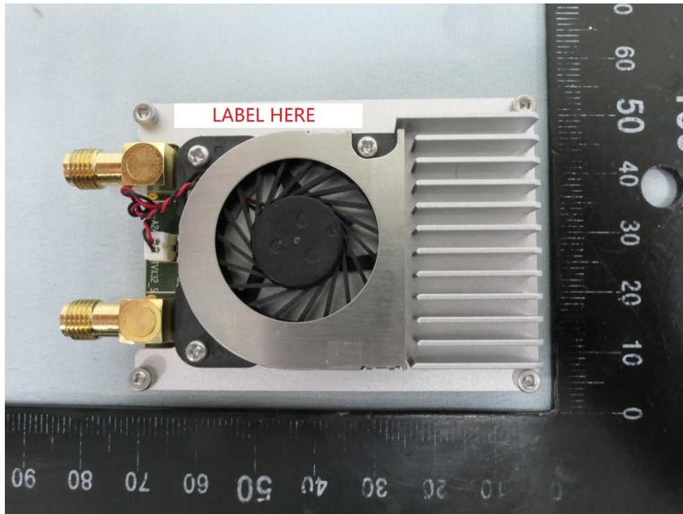
(8) EUT Photo (WVL-A2458J28TTVX32_S_US)
