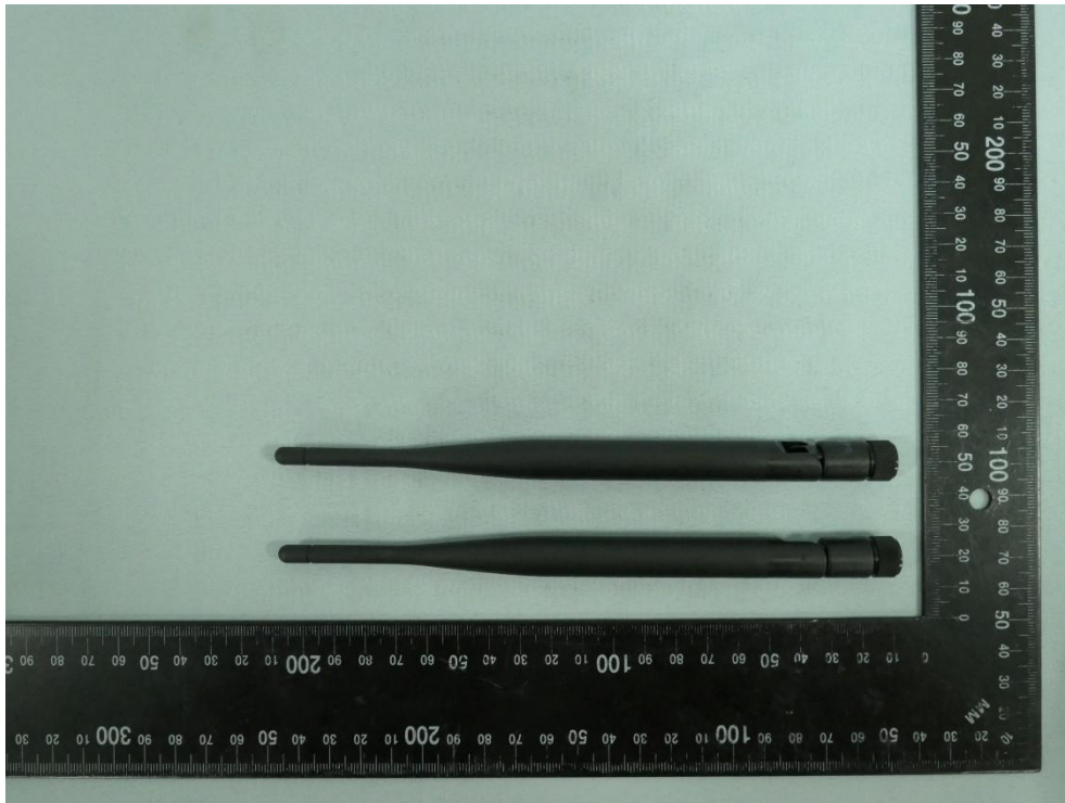
(13) Antenna Photo
