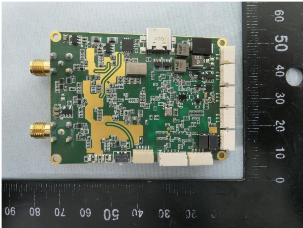
(22) EUT Photo (WVL-A2458J28TTVX32_S_US)
