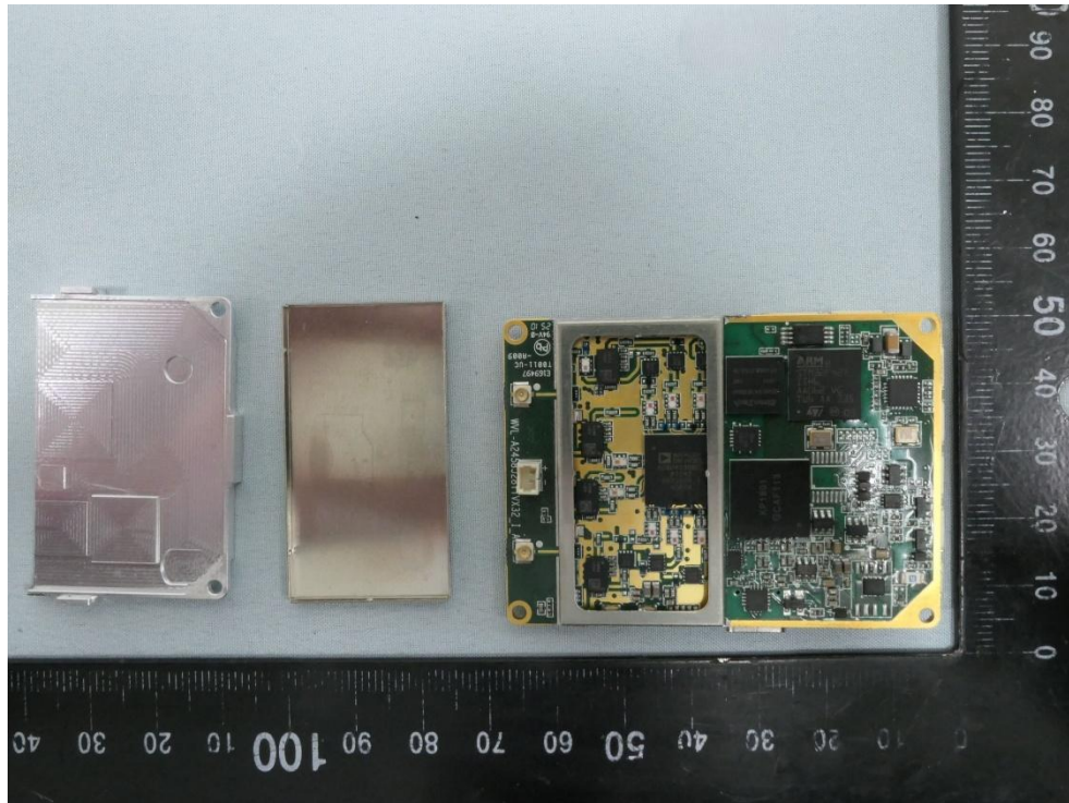
(2) EUT Photo (WVL-A2458J28TTVX32_I_US)
