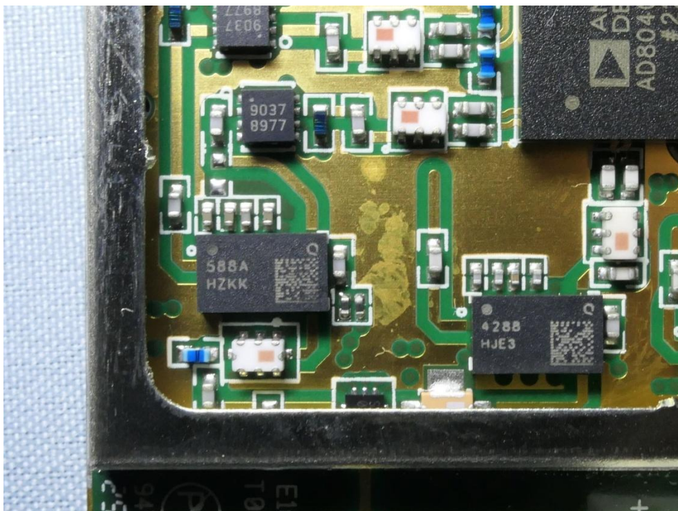
(4) EUT Photo (WVL-A2458J28TTVX32_I_US)
