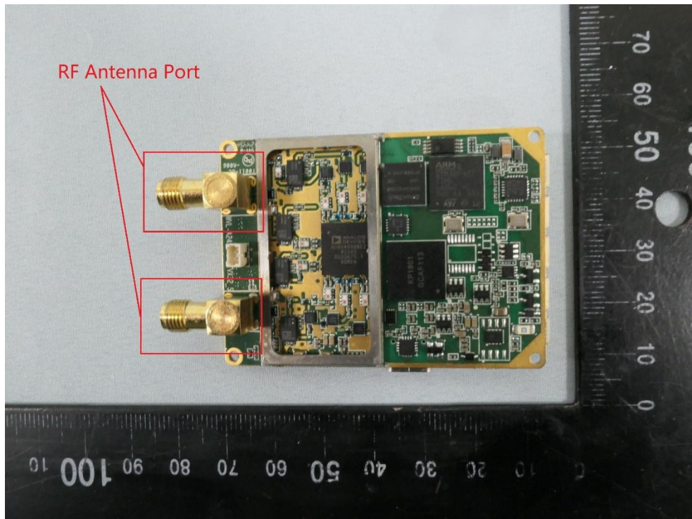
(14) EUT Photo (WVL-A2458J28TTVX32_S_US)
