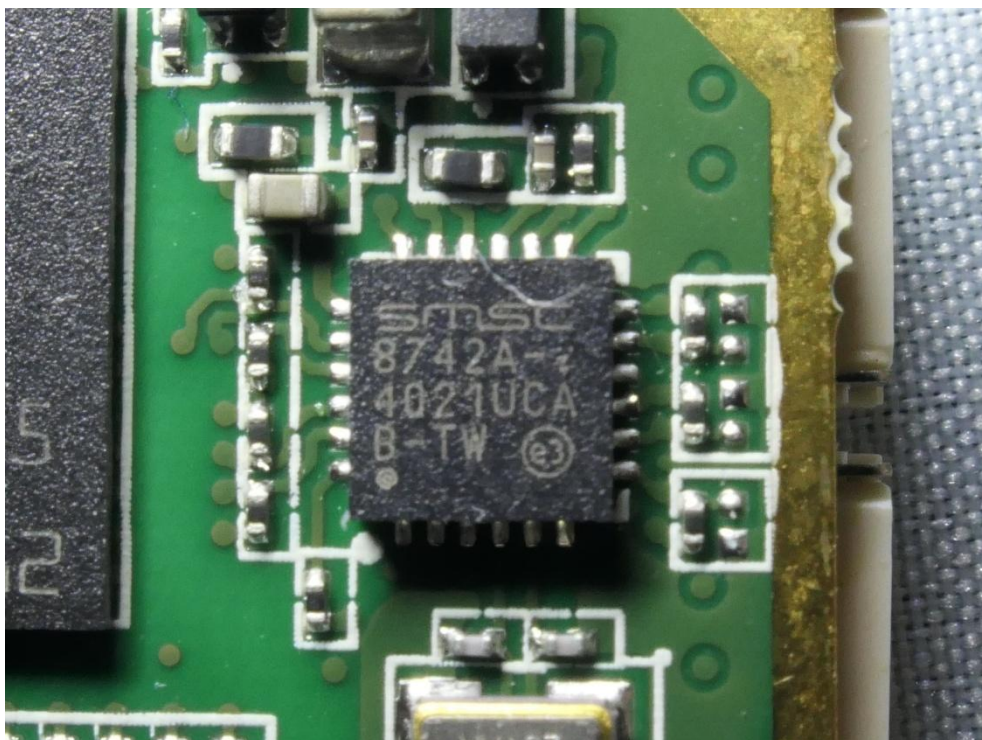
(20) EUT Photo (WVL-A2458J28TTVX32_S_US)
