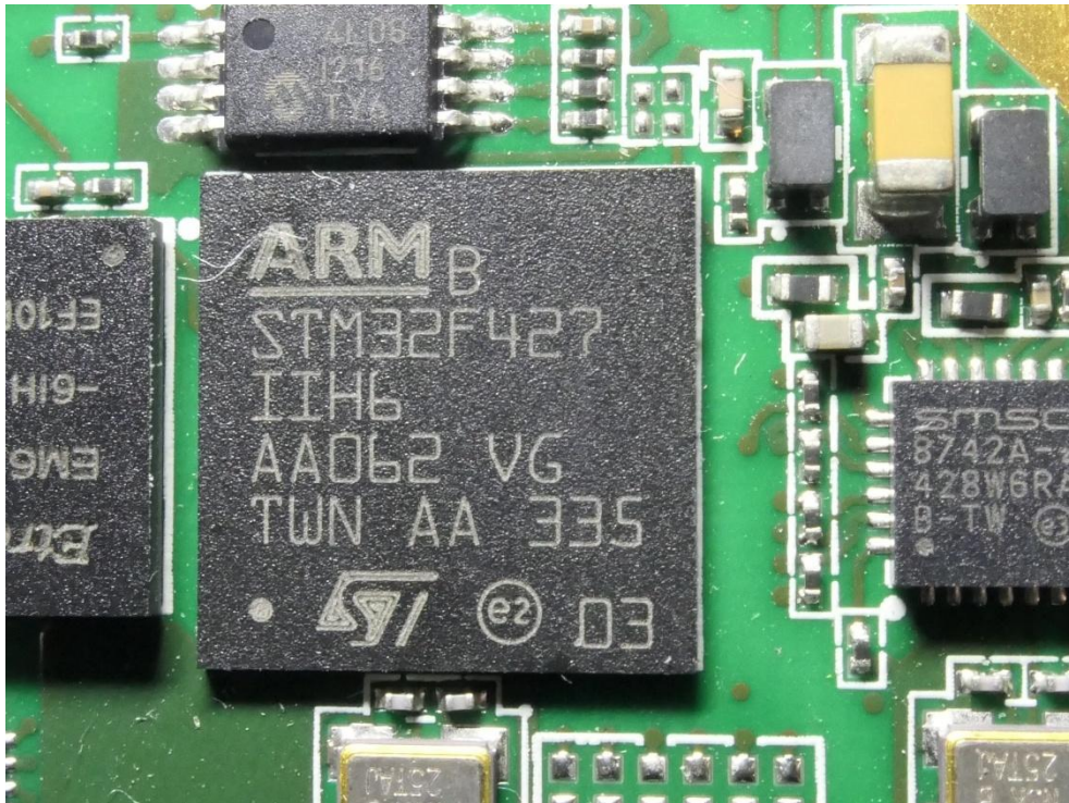
(8) EUT Photo (WVL-A2458J28TTVX32_I_US)
