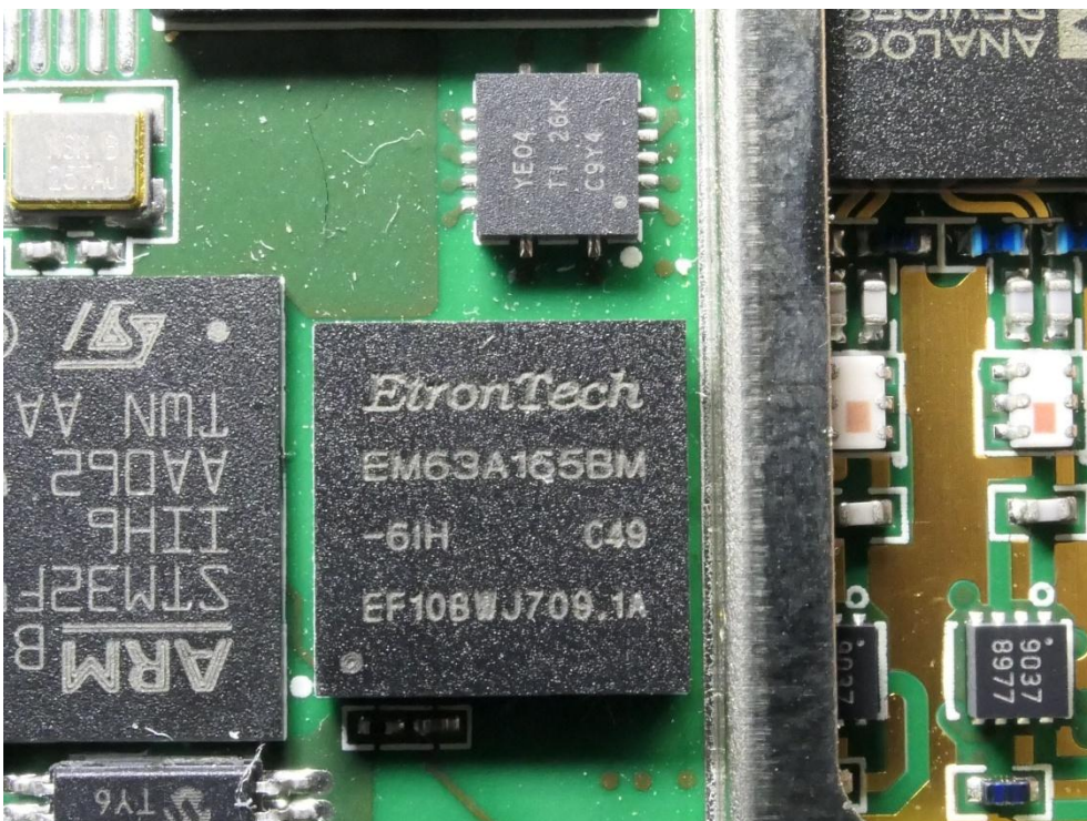
(6) EUT Photo (WVL-A2458J28TTVX32_I_US)
