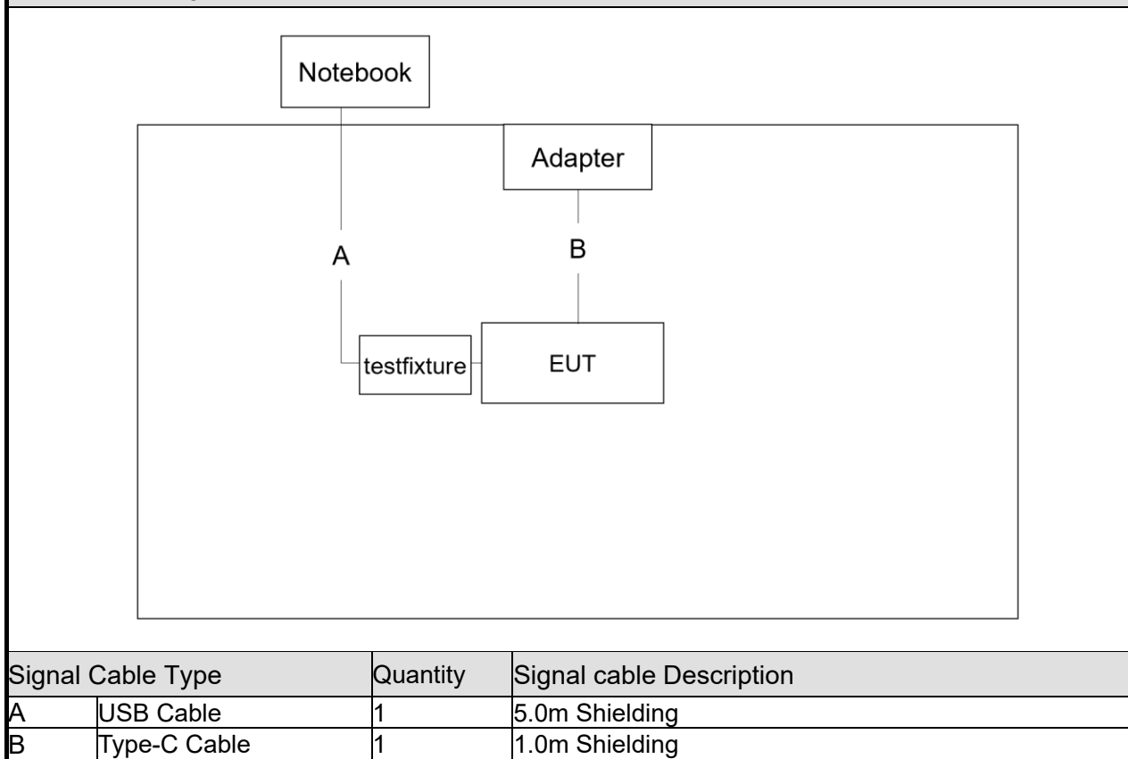
Connection Diagram
