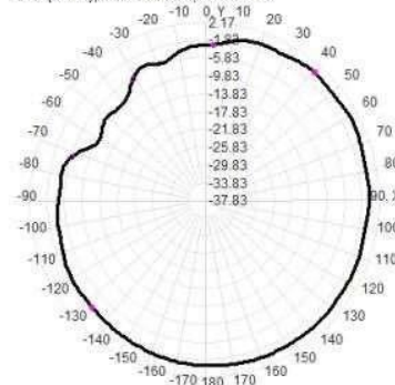
Total(H-XY), Max= 0.26dBi, CirD=10.50
