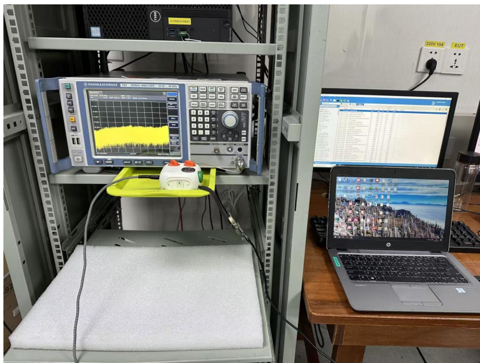
RF Conducted
