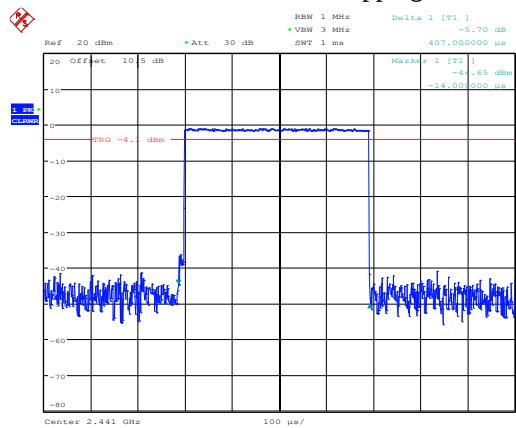
BDR_DH1_Hopping
