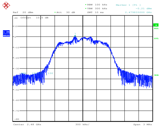
2EDR_DH1_High
