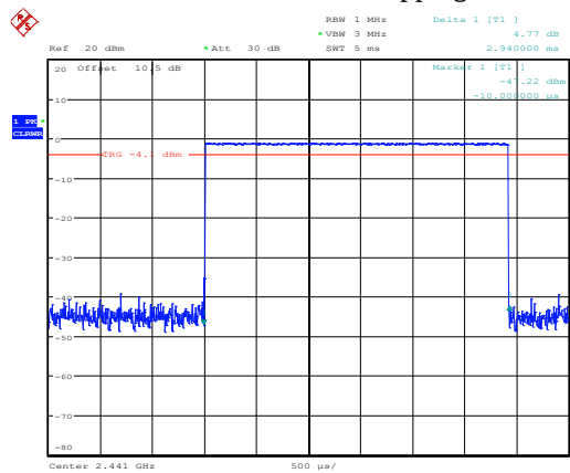
BDR_DH5_Hopping
