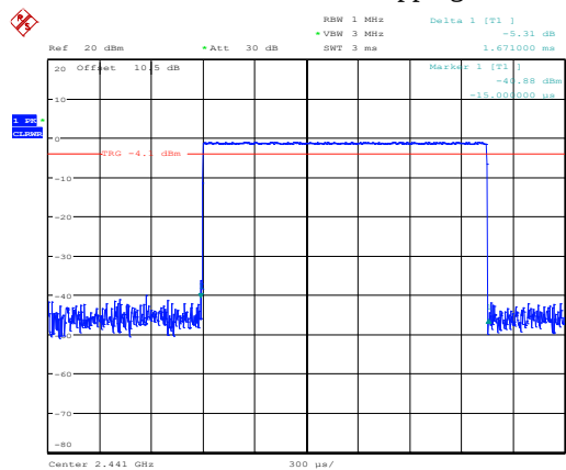
BDR_DH3_Hopping
