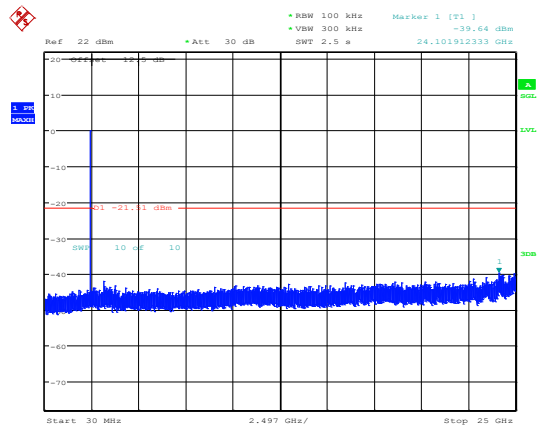
2EDR_DH1_Middle
