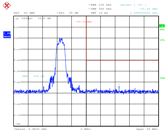
2EDR_DH1_High
