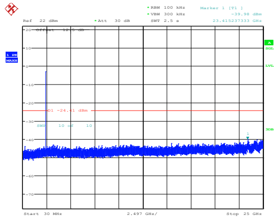
2EDR_DH1_Low
