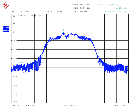
3EDR_DH1_Middle
