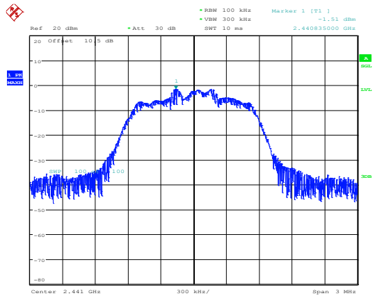
2EDR_DH1_Middle
