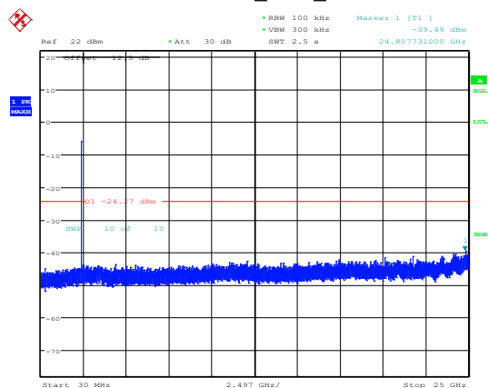
3EDR_DH1_Low
