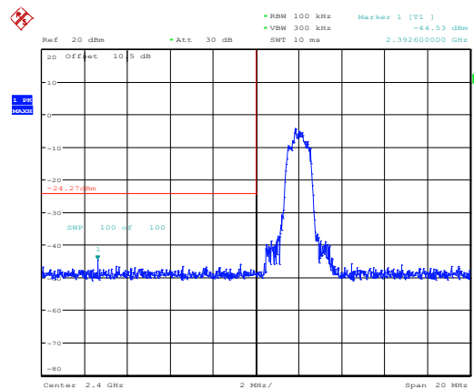
3EDR_DH1_Low
