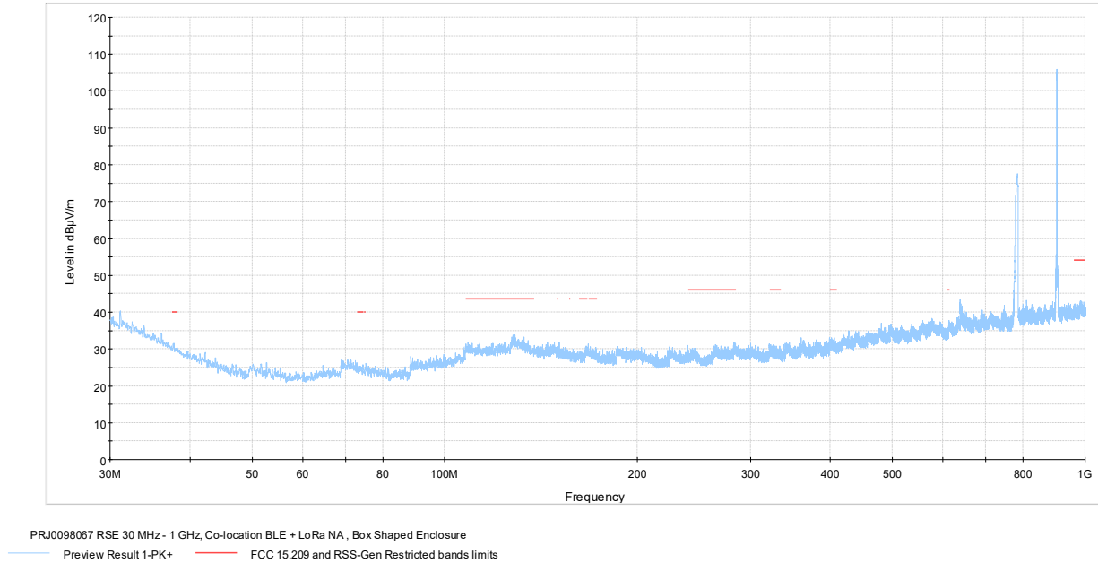
Figure 7.6-21: Radiated spurious emissions 30-1000 MHz, Pulse Mouse iQ TOTAL
