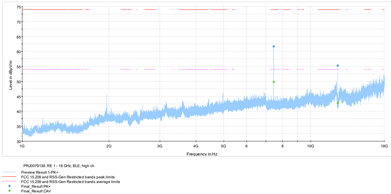
Figure 7.6-6: Radiated spurious emissions 1-18 GHz high channel
