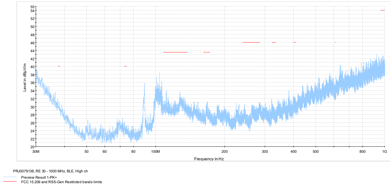
Figure 7.6-3: Radiated spurious emissions 30-1000 MHz high channel
