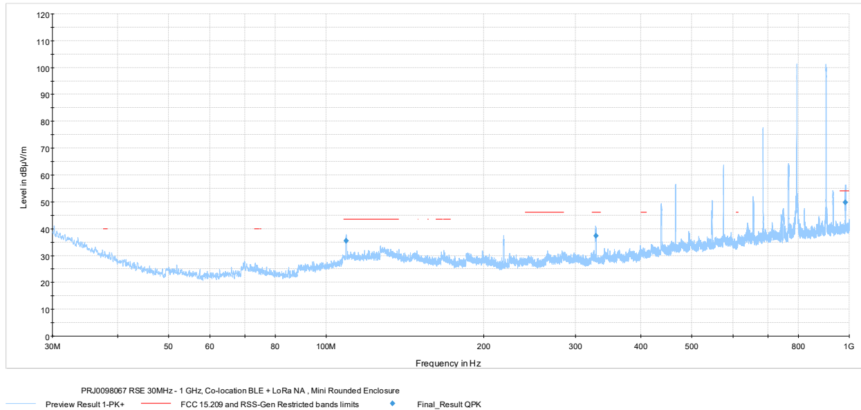
Figure 7.6-26: Radiated spurious emissions 30-1000 MHz, 24/7 iQ TOTAL
