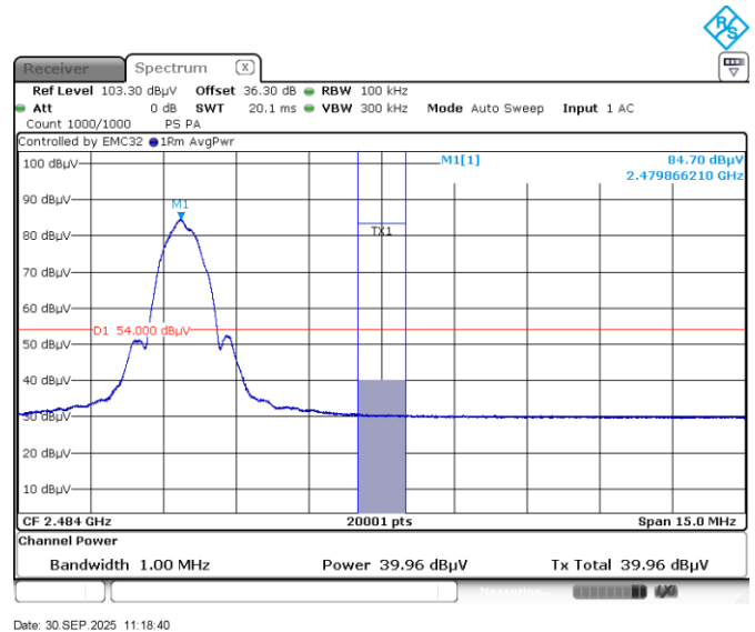
Figure 7.6-13: Radiated band edge spurious emissions at 2483.5 MHz Average
