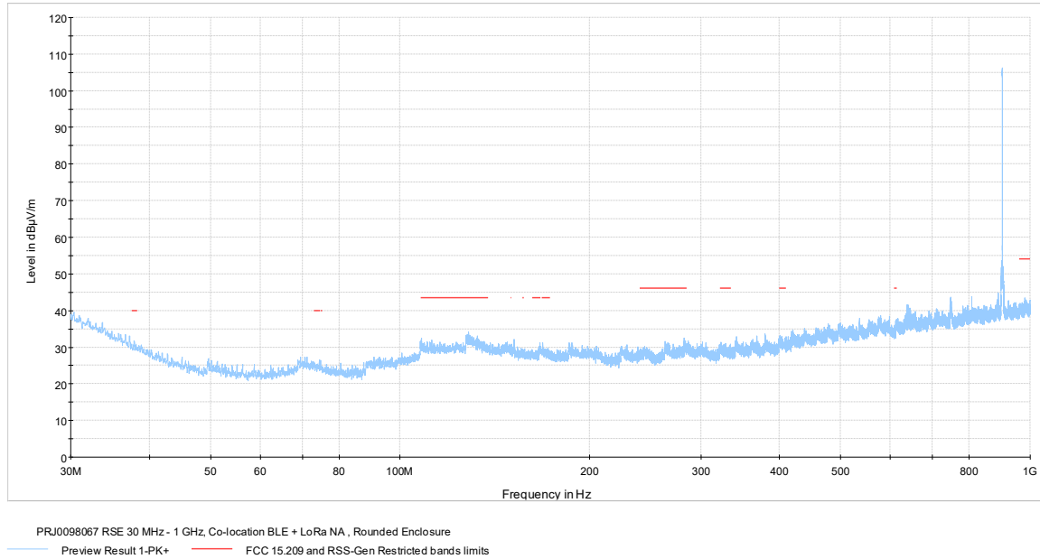
Figure 7.6-16: Radiated spurious emissions 30-1000 MHz, Pulse Rat iQ TOTAL
