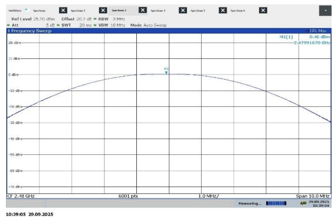
Figure 7.5-4: Output power on high channel
