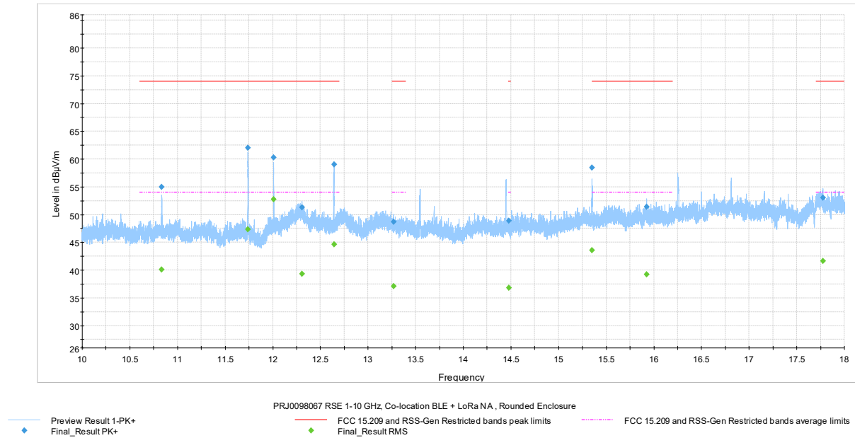
Figure 7.6-19: Radiated spurious emissions 10-18 GHz, Pulse Rat iQ TOTAL
