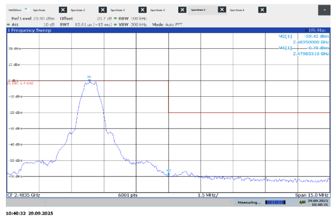
Figure 7.6-15: Conducted non-restricted band edge emissions at 2483.5 MHz
