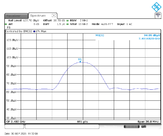
Figure 7.5-2: EIRP check on low channel
