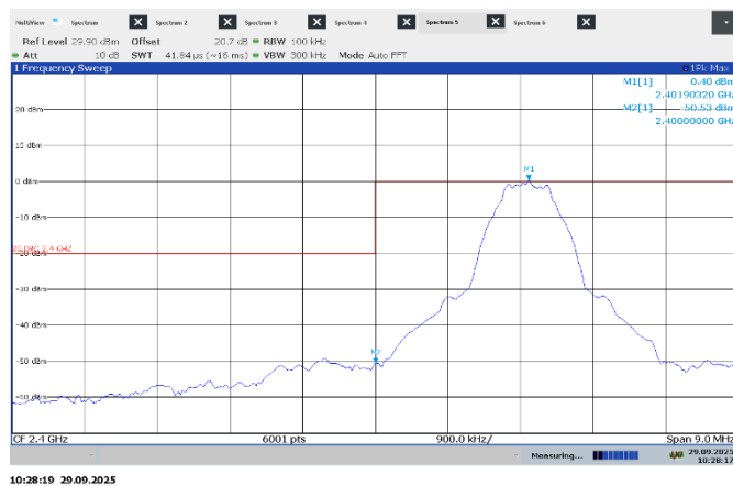
Figure 7.6-14: Conducted non-restricted band edge emissions at 2400 MHz
