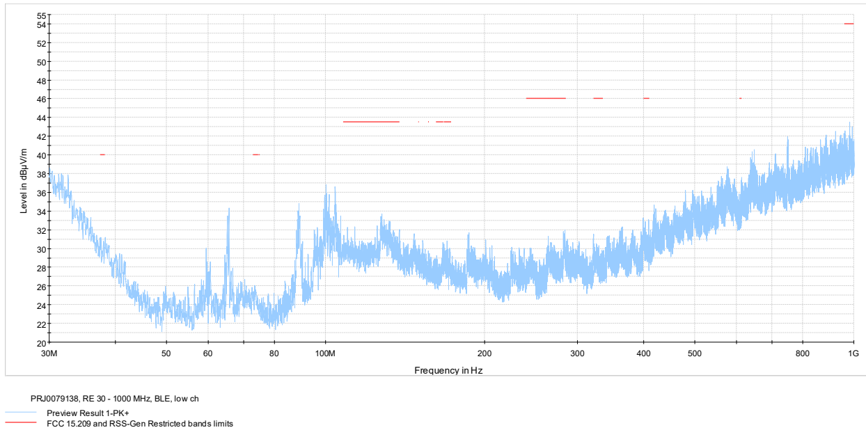
Figure 7.6-1: Radiated spurious emissions 30-1000 MHz low channel
