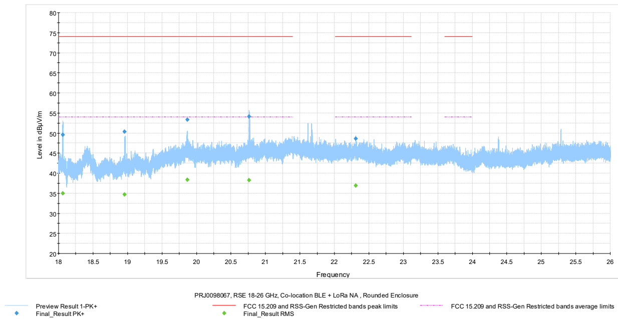
Figure 7.6-20: Radiated spurious emissions 18-26 GHz, Pulse Rat iQ TOTAL
