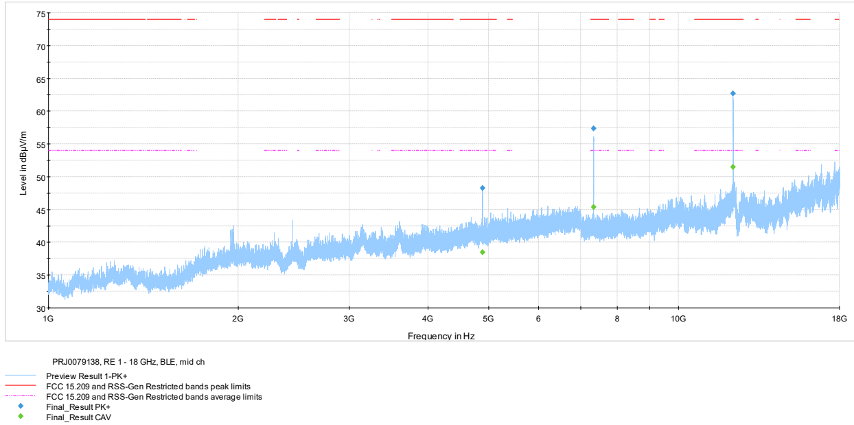
Figure 7.6-5: Radiated spurious emissions 1-18 GHz mid channel
