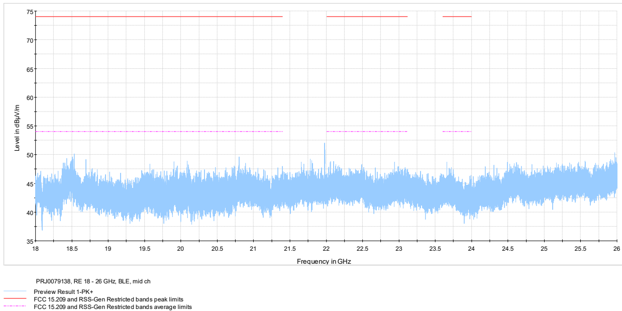
Figure 7.6-8: Radiated spurious emissions 18-26 GHz mid channel
