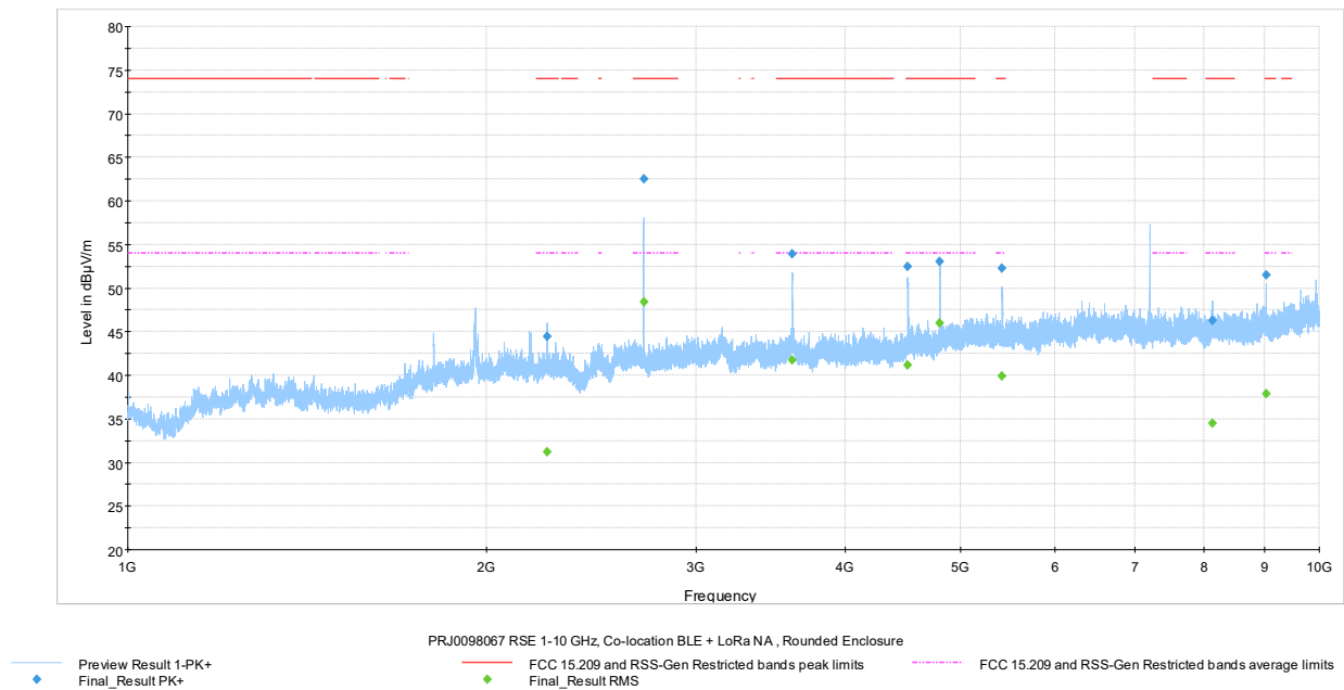
Figure 7.6-17: Radiated spurious emissions 1-10 GHz, Pulse Rat iQ TOTAL
