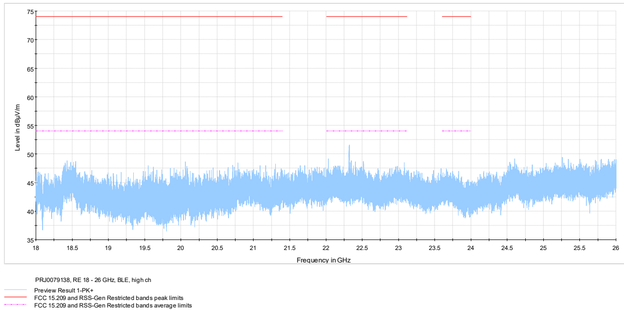
Figure 7.6-9: Radiated spurious emissions 18-26 GHz high channel
