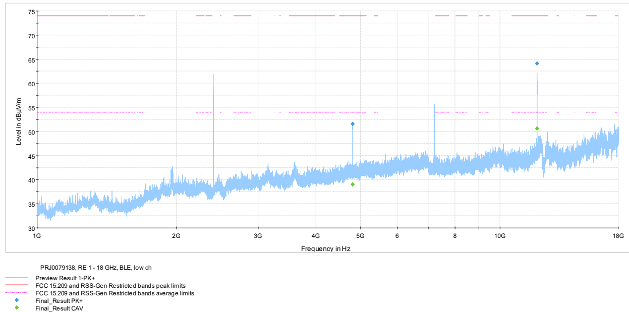
Figure 7.6-4: Radiated spurious emissions 1-18 GHz low channel
