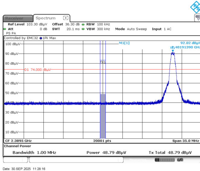
Figure 7.6-10: Radiated band edge spurious emissions at 2400 MHz Peak
