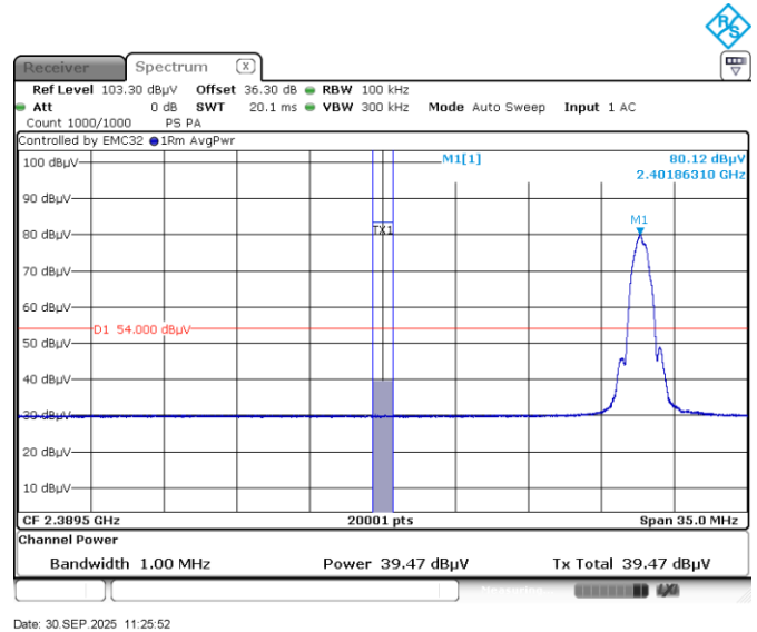
Figure 7.6-11: Radiated band edge spurious emissions at 2400 MHz Average
