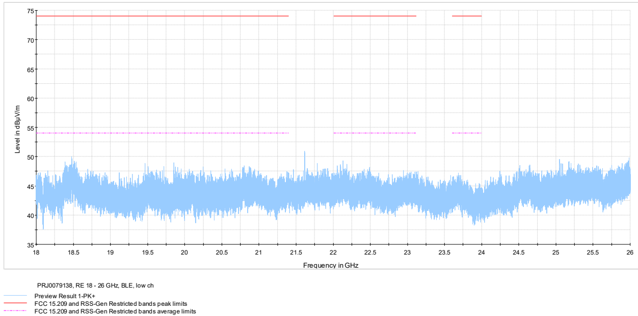
Figure 7.6-7: Radiated spurious emissions 18-26 GHz low channel
