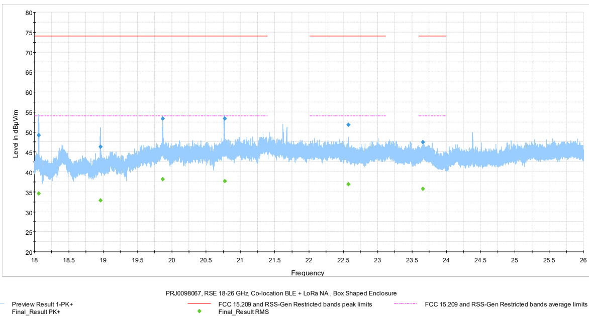
Figure 7.6-25: Radiated spurious emissions 18-26 GHz, Pulse Mouse iQ TOTAL
