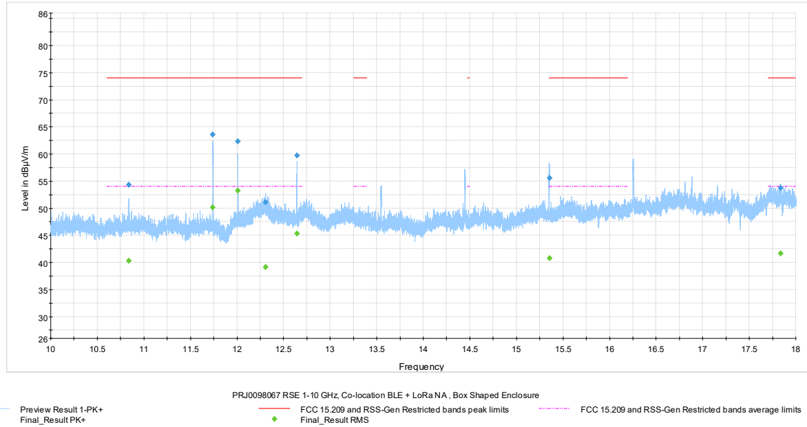
Figure 7.6-24: Radiated spurious emissions 10-18 GHz, Pulse Mouse iQ TOTAL
