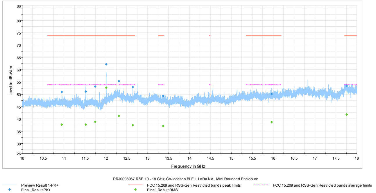
Figure 7.6-29: Radiated spurious emissions 10-18 GHz, 24/7 iQ TOTAL
