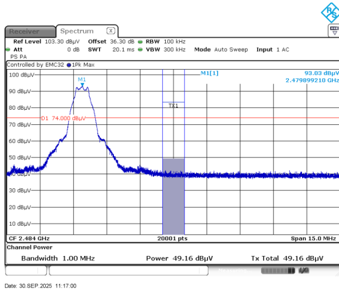
Figure 7.6-12: Radiated band edge spurious emissions at 2483.5 MHz Peak
