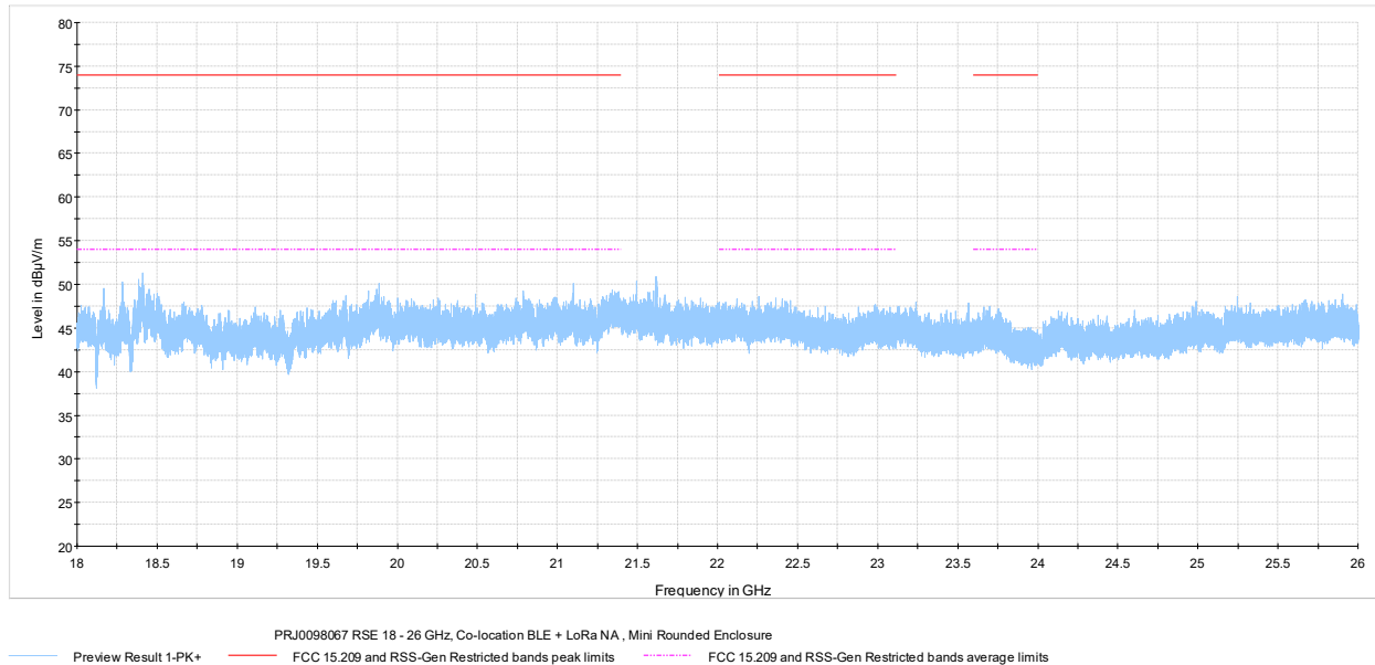
Figure 7.6-30: Radiated spurious emissions 18-26 GHz, 24/7 iQ TOTAL
