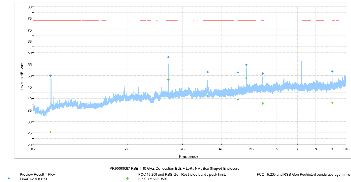
Figure 7.6-22: Radiated spurious emissions 1-10 GHz, Pulse Mouse iQ TOTAL
