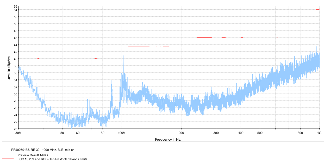
Figure 7.6-2: Radiated spurious emissions 30-1000 MHz mid channel
