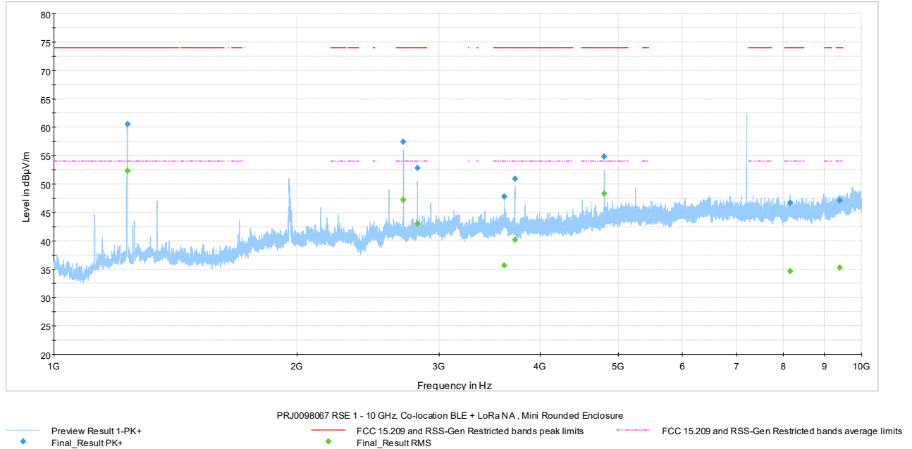
Figure 7.6-27: Radiated spurious emissions 1-10 GHz, 24/7 iQ TOTAL
