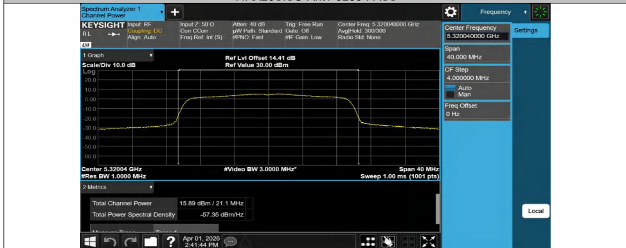
11AX20SISO-Ant1-5320-PASS
