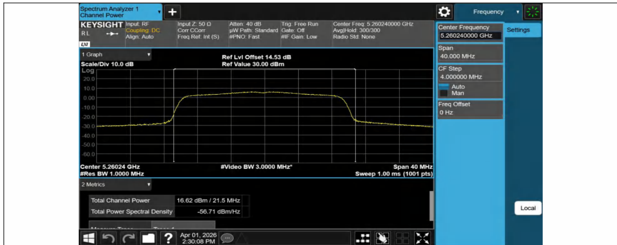
11AX20SISO-Ant1-5260-PASS
