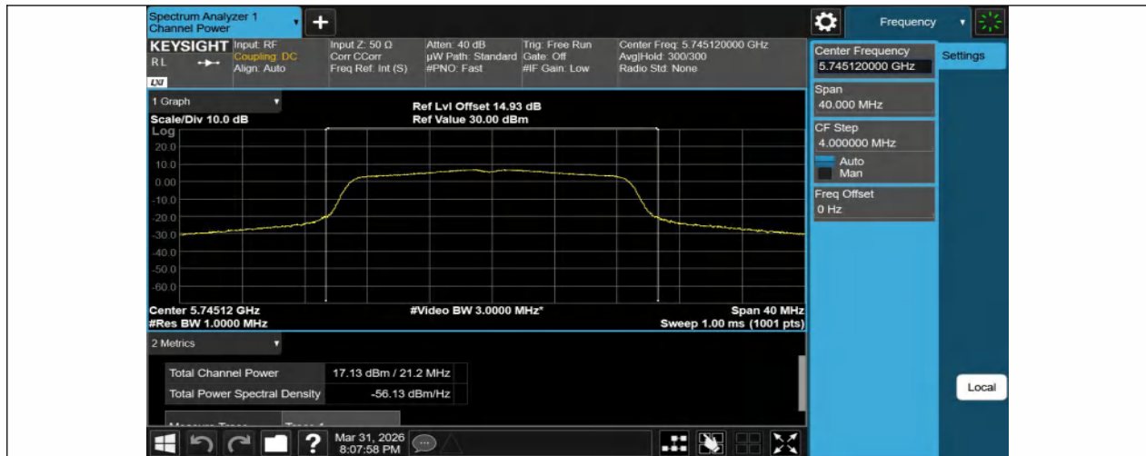
11N20SISO-Ant1-5745-PASS
