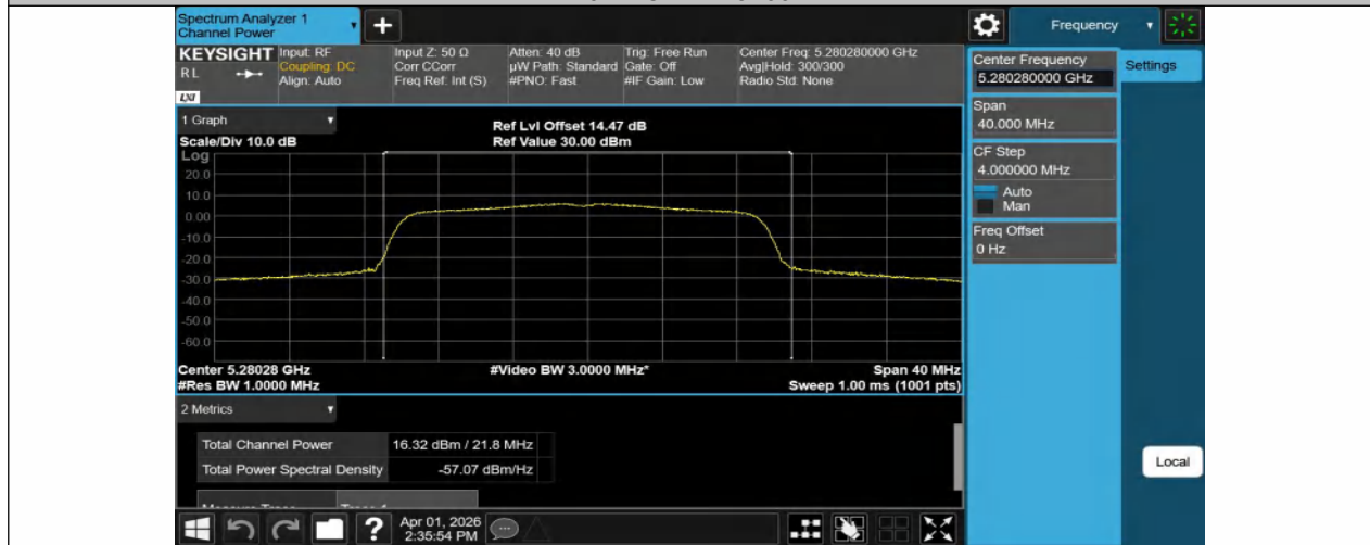
11AX20SISO-Ant1-5280-PASS
