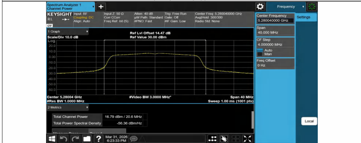
11N20SISO-Ant1-5280-PASS
