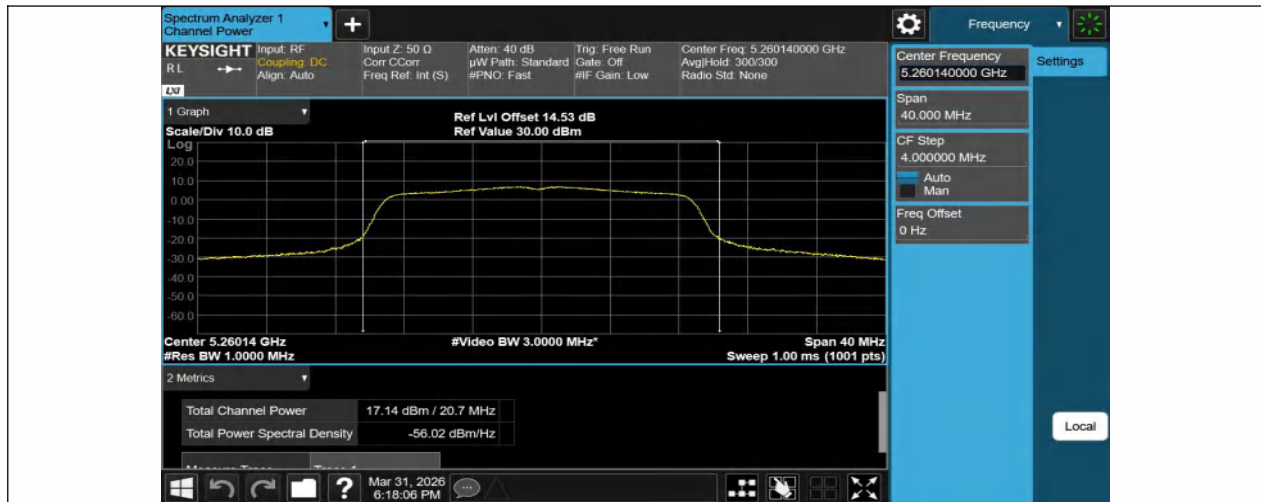
11N20SISO-Ant1-5260-PASS
