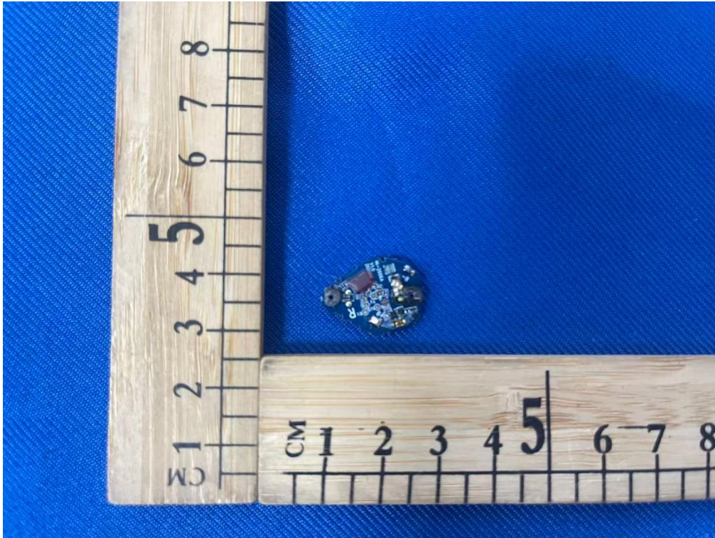
Internal Photos(Right)
