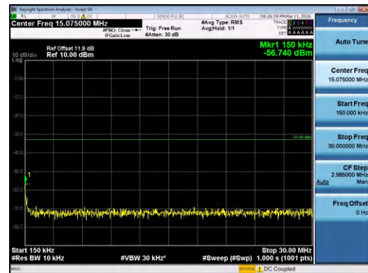
Band2-3MHz-QPSK-18615-15RB#0-0.15~30-PASS
