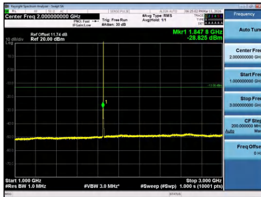
Band2-3MHz-QPSK-18615-1RB#14-1000~3000-PAS
