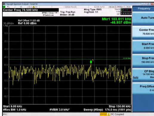
Band2-3MHz-QPSK-18615-15RB#0-0.009~0.15-PAS
