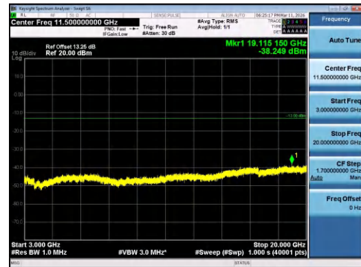
Band2-3MHz-QPSK-18615-1RB#14-3000~20000-PAS
