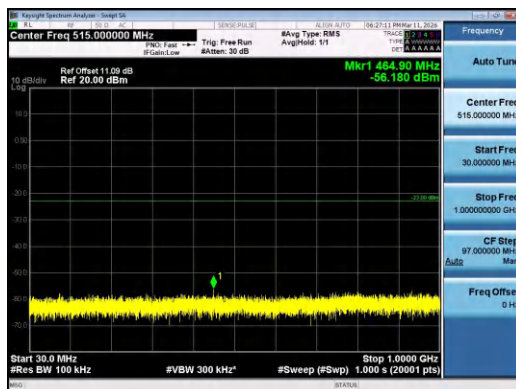
Band2-3MHz-QPSK-18615-15RB#0-30~1000-PASS
