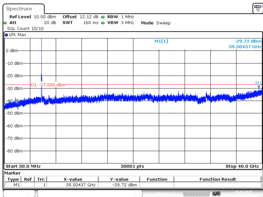
Tx. Spurious NVNT ax40 5795MHz Ant3 Emission
