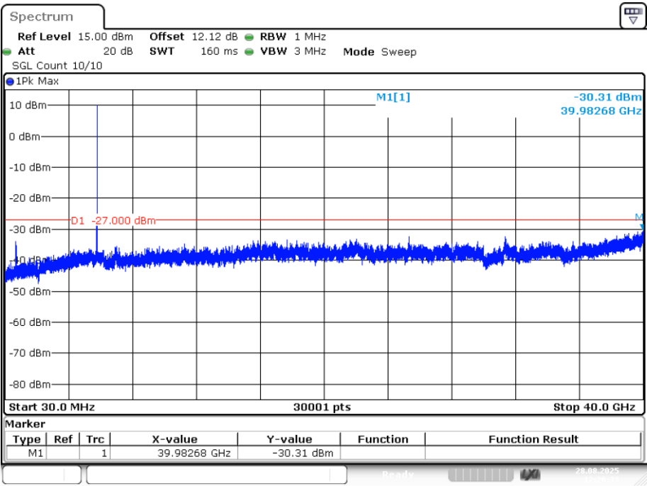
Tx. Spurious NVNT ac20 5825MHz Ant3 Emission
