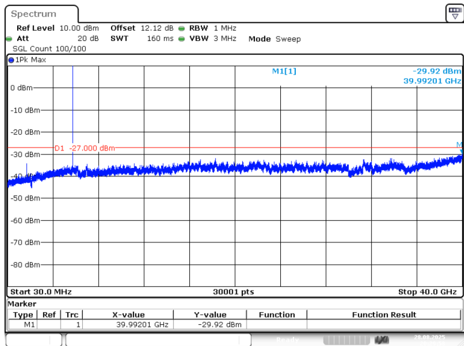
Tx. Spurious NVNT ax20 5745MHz Ant1 Emission
