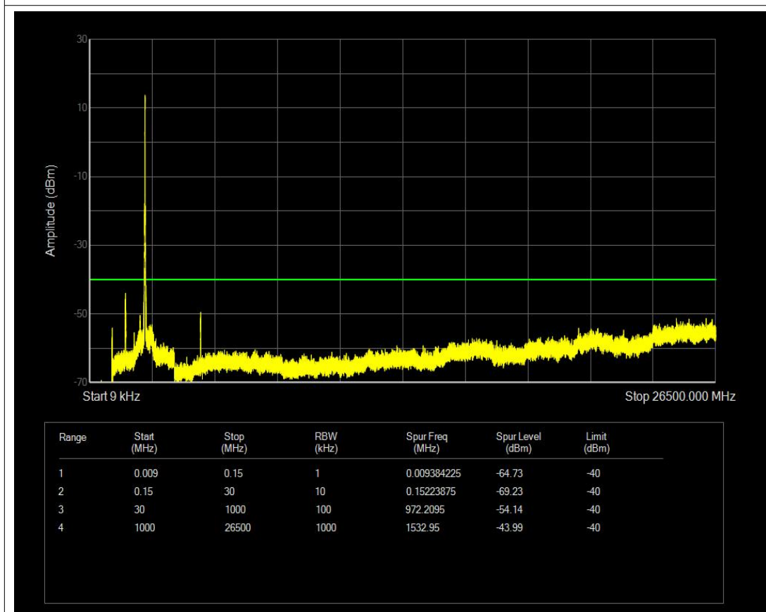
Band40(2350-2360) QPSK BW=10MHz Channel=39200 RB Size=50 Position=#0 NVNT
