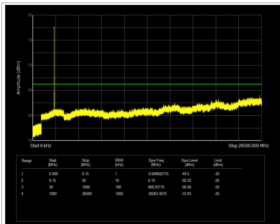
Band41 QPSK BW=5MHz Channel=39675 RB Size=25 Position=#0 NVNT
