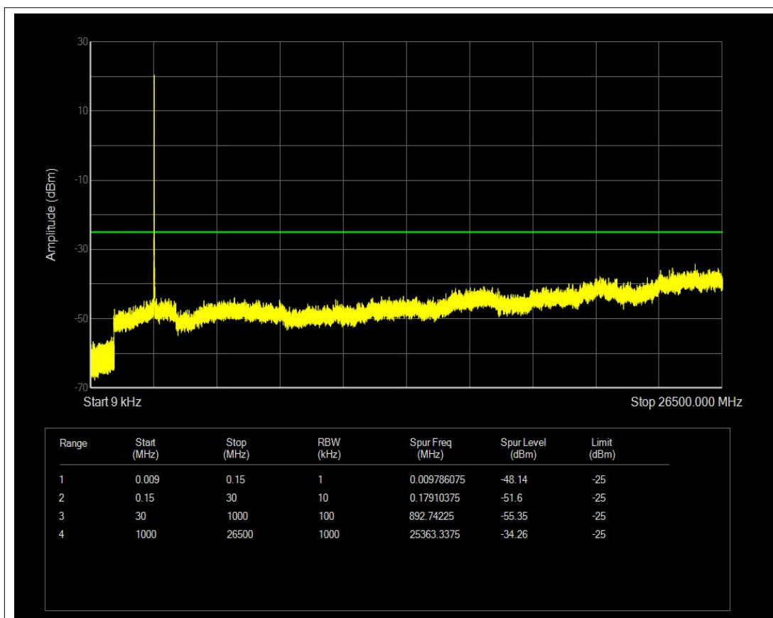
Band41 QPSK BW=5MHz Channel=41565 RB Size=25 Position=#0 NVNT
