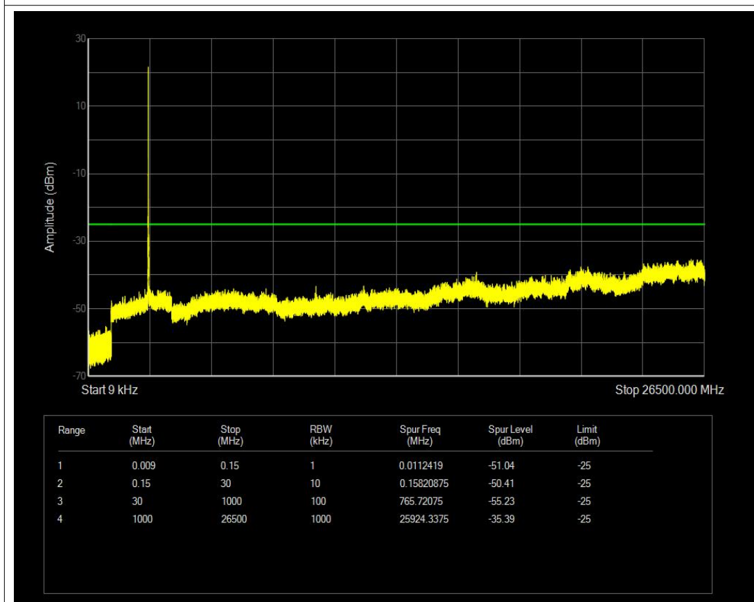
Band38 QPSK BW=5MHz Channel=38000 RB Size=25 Position=#0 NVNT
