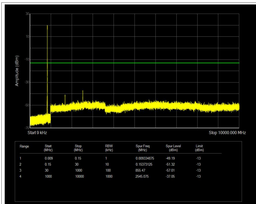
Band5 QPSK BW=1.4MHz Channel=20643 RB Size=6 Position=#0 NVNT
