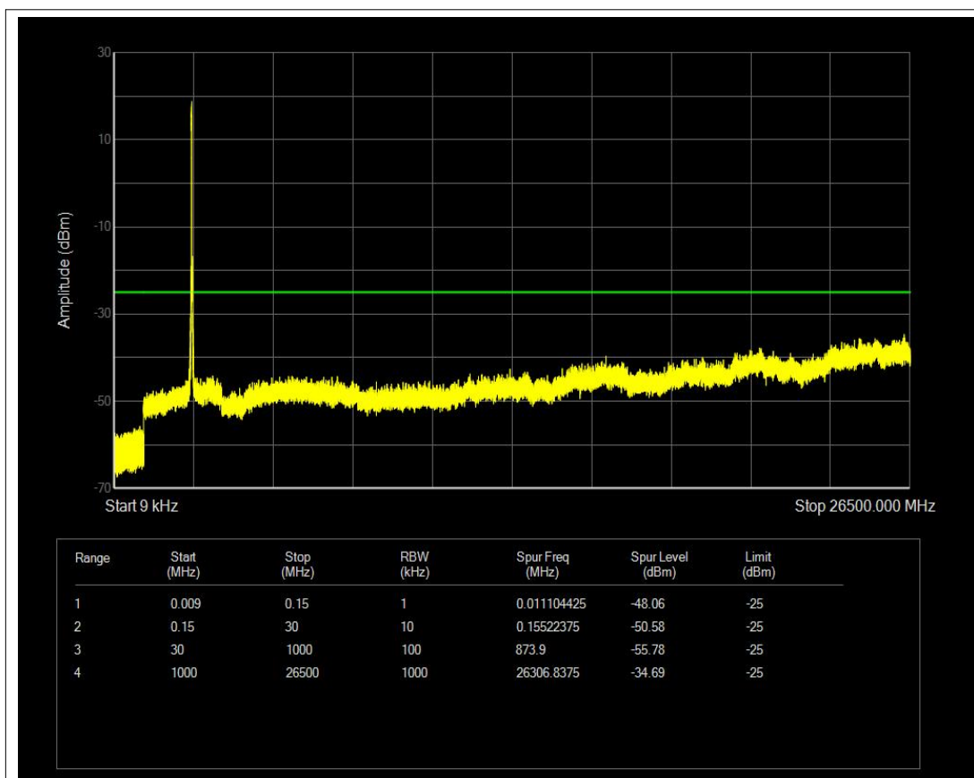
Band38 QPSK BW=20MHz Channel=38000 RB Size=100 Position=#0 NVNT
