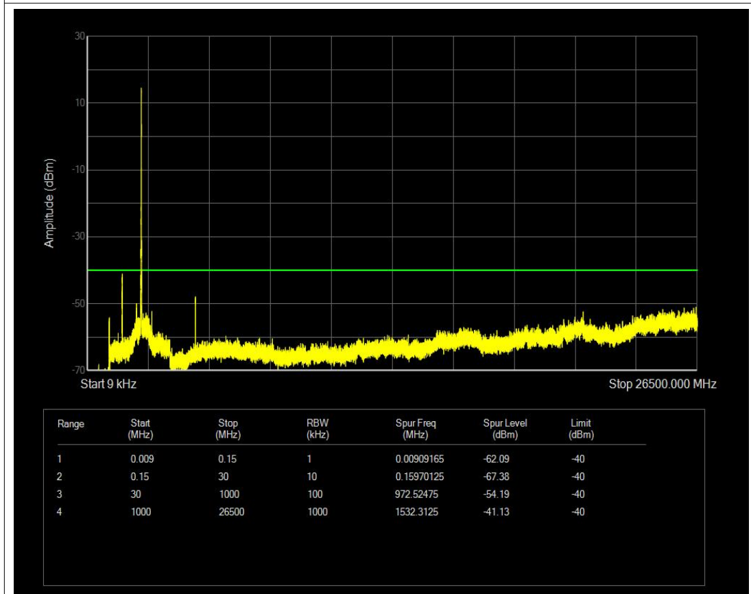
Band40(2350-2360) QPSK BW=5MHz Channel=39200 RB Size=25 Position=#0 NVNT
