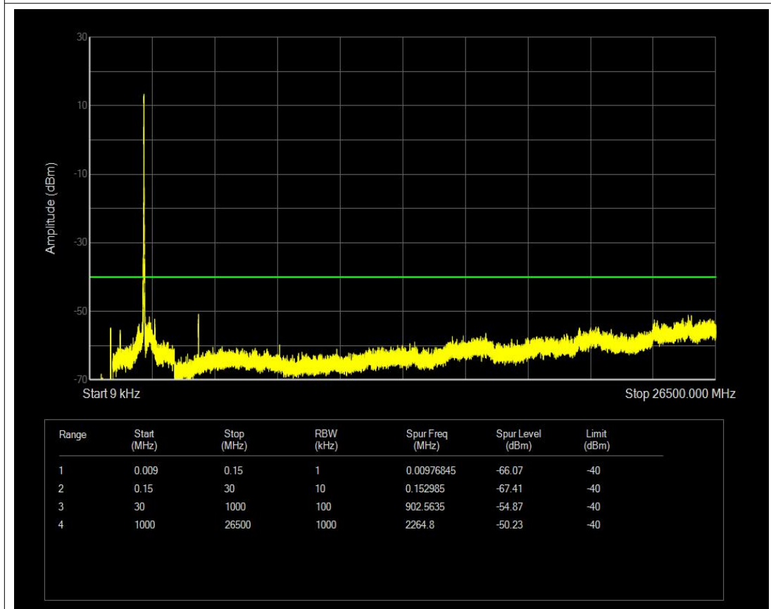
Band40(2305-2315) QPSK BW=10MHz Channel=38750 RB Size=50 Position=#0 NVNT
