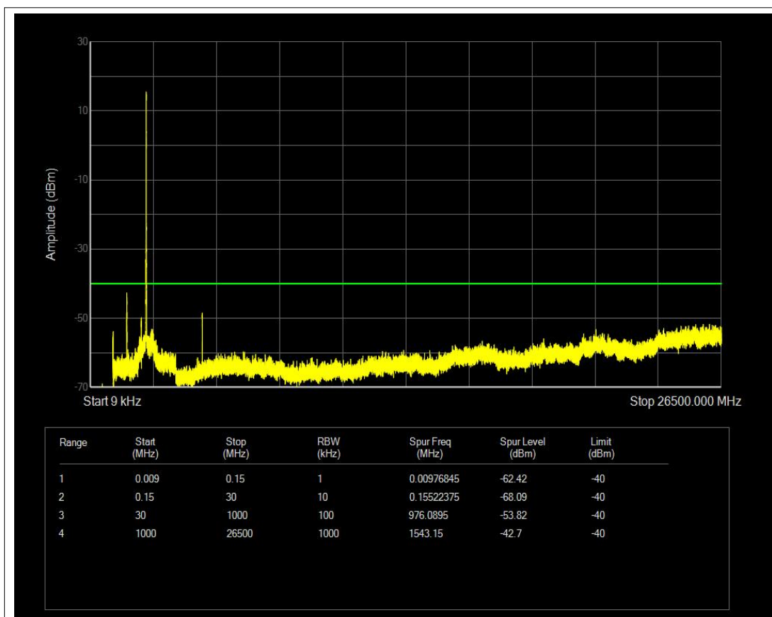
Band40(2350-2360) QPSK BW=5MHz Channel=39225 RB Size=25 Position=#0 NVNT
