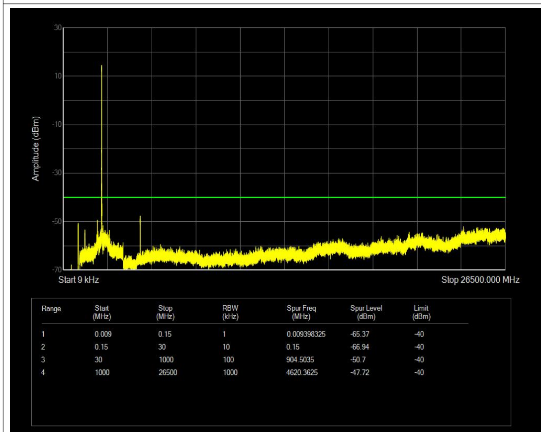
Band40(2305-2315) QPSK BW=5MHz Channel=38750 RB Size=25 Position=#0 NVNT
