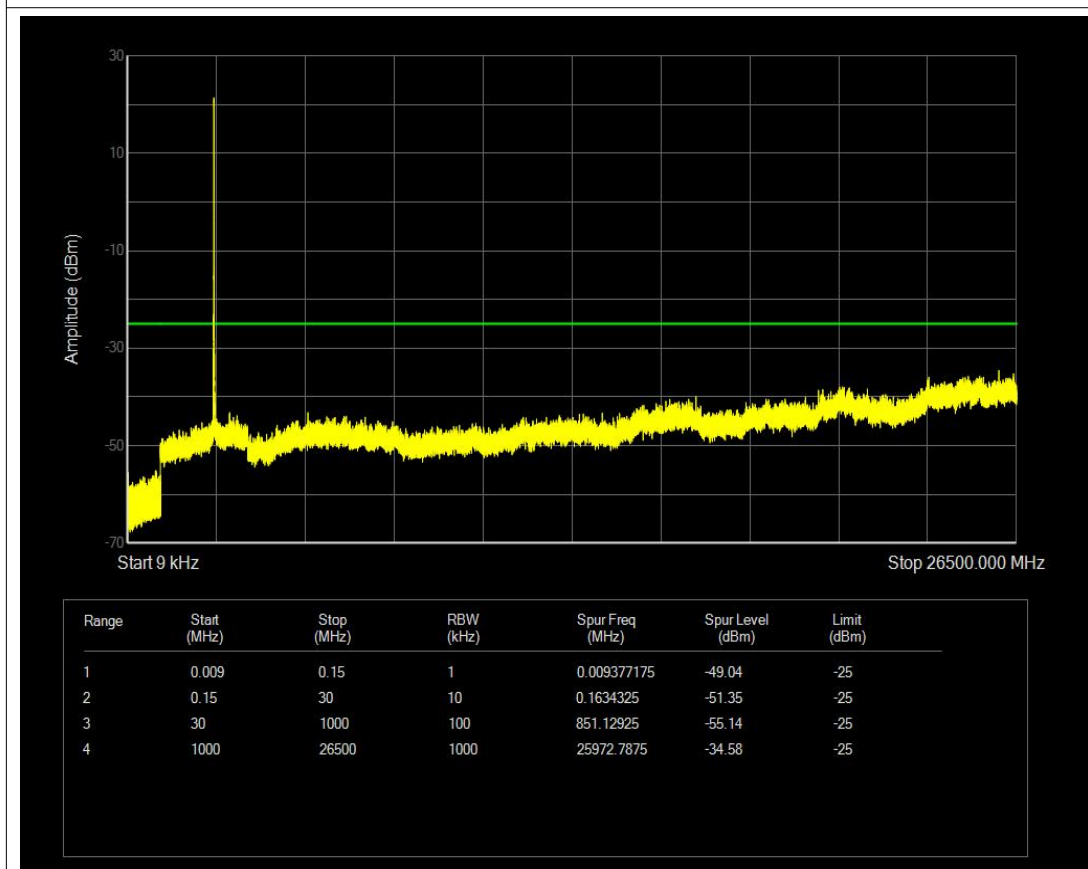
Band41 QPSK BW=5MHz Channel=40620 RB Size=25 Position=#0 NVNT
