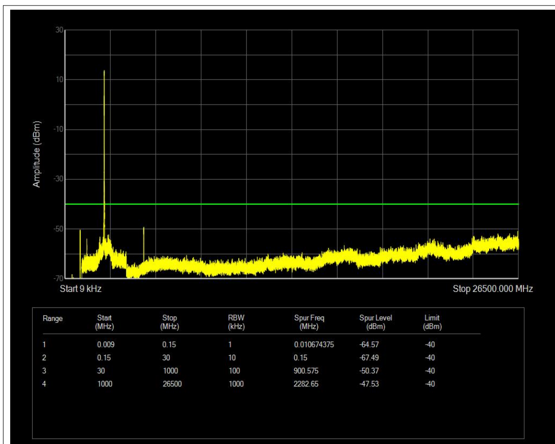
Band40(2305-2315) QPSK BW=5MHz Channel=38725 RB Size=25 Position=#0 NVNT
