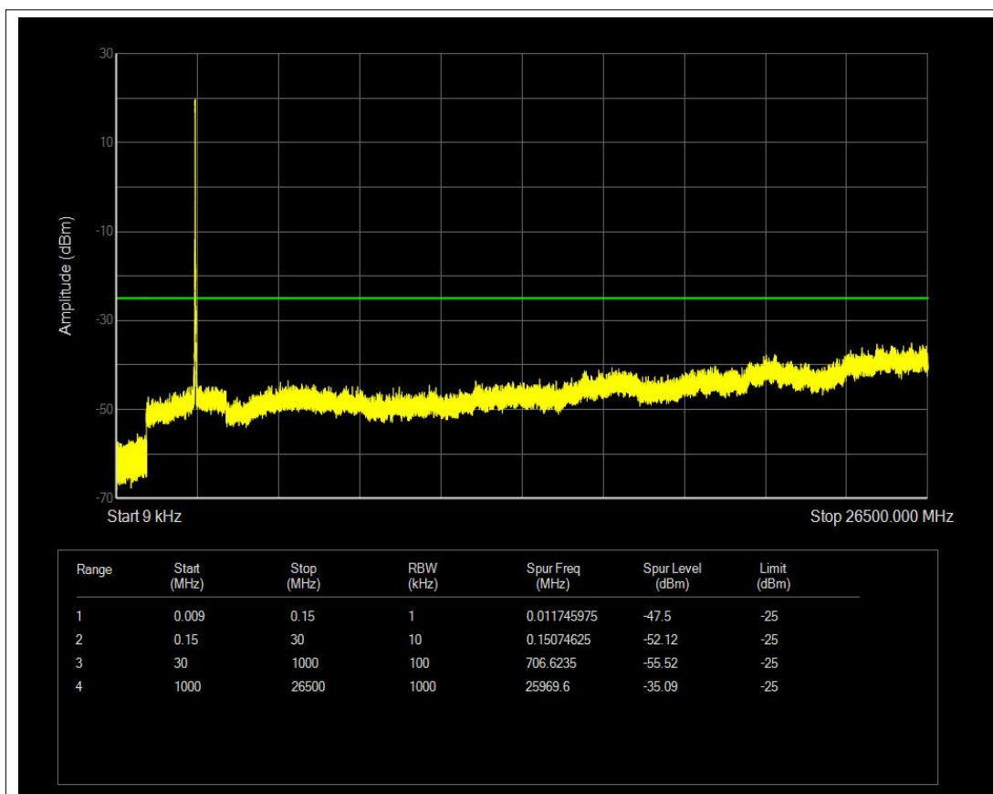
Band41 QPSK BW=10MHz Channel=40620 RB Size=50 Position=#0 NVNT
