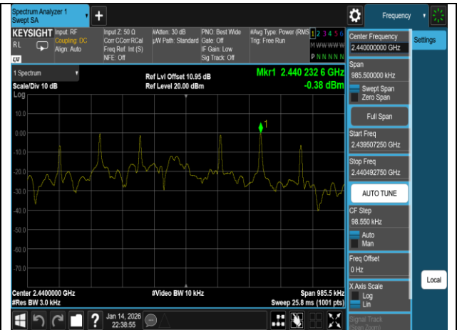
PSD_BLE 1M_MidCH19-2440MHz
