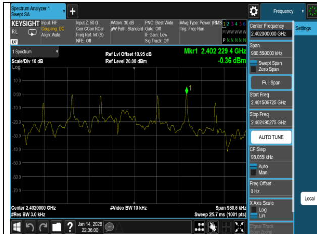
PSD_BLE 1M_LowCH00-2402MHz
