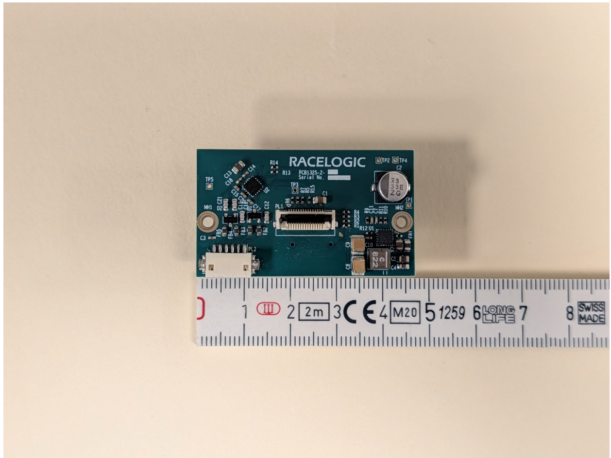
Top of IMU PCB
