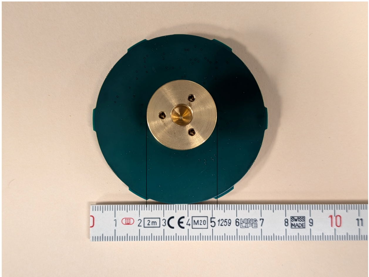
Top View of Antenna ( 5.2 - 2.3 = 2.9 cm Diameter)
