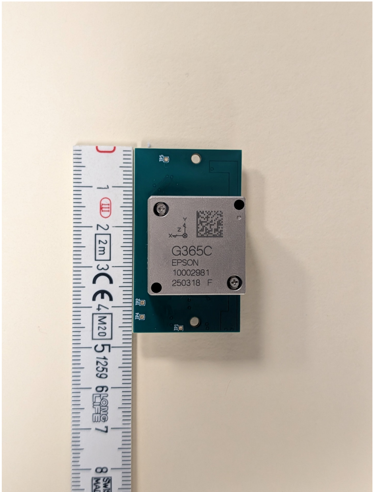
Bottom of IMU PCB
