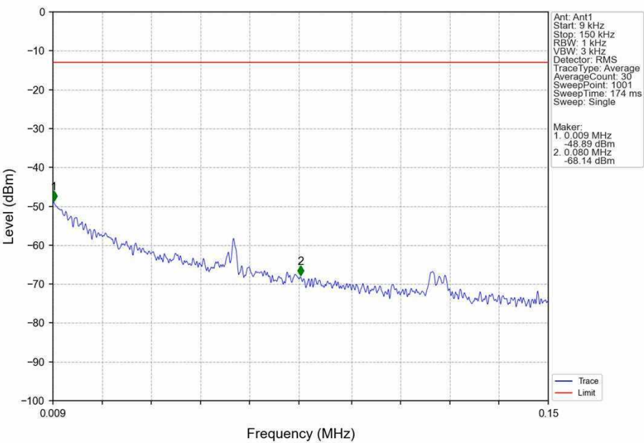
Band4 5MHz QPSK HCH 1752.5MHz RB 1 0 NTN
