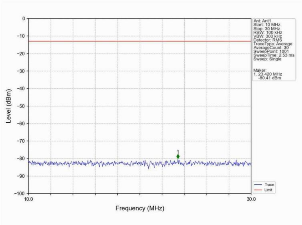
Band4 1.4MHz QPSK HCH 1754.3MHz RB 1 0 NTNV
