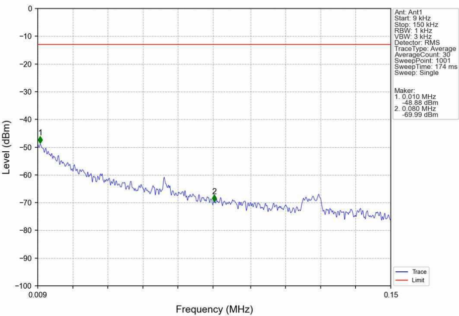
Band4 3MHz QPSK HCH 1753.5MHz RB 1 0 NTN
