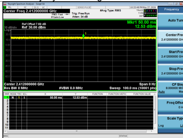
Duty Cycle NVNT n20 2412MHz Ant1
