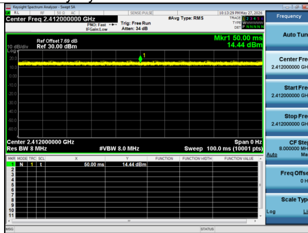
Duty Cycle NVNT g 2412MHz Ant1
