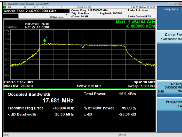
OBW NVNT n20 2462MHz Ant1
