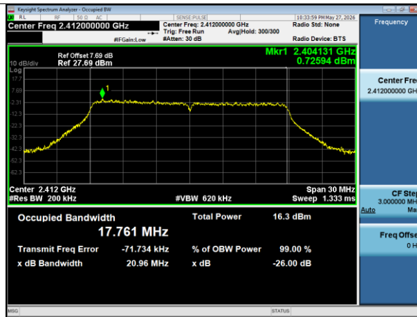
OBW NVNT n20 2412MHz Ant1
