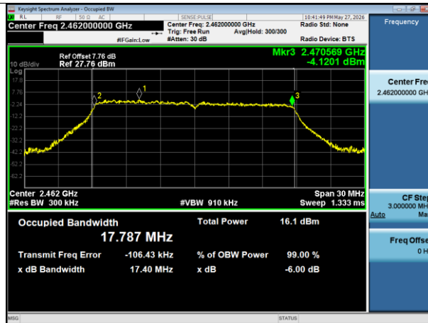
-6dB Bandwidth NVNT n20 2462MHz Ant1
