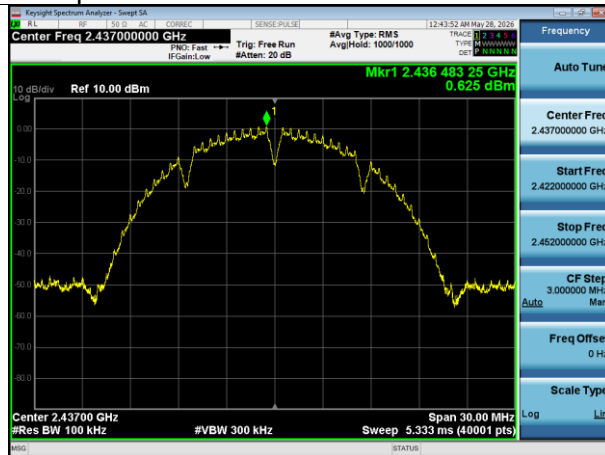
Tx. Spurious NVNT b 2437MHz Ant1 Ref
