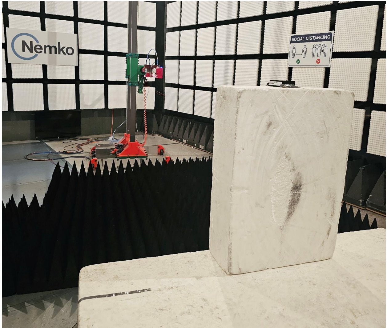
Photo 4 – Test Setup (View D). Alternate view of the same configuration
