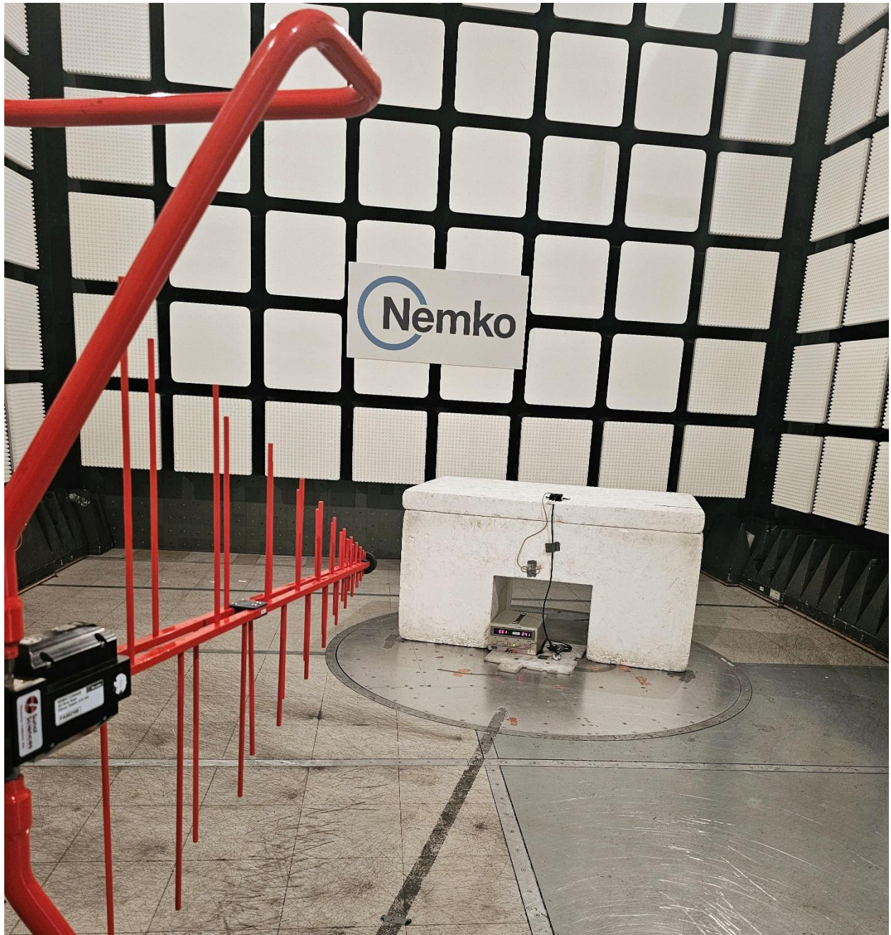
Photo 2 – Test Setup (View B). Alternate view of the same configuration.
