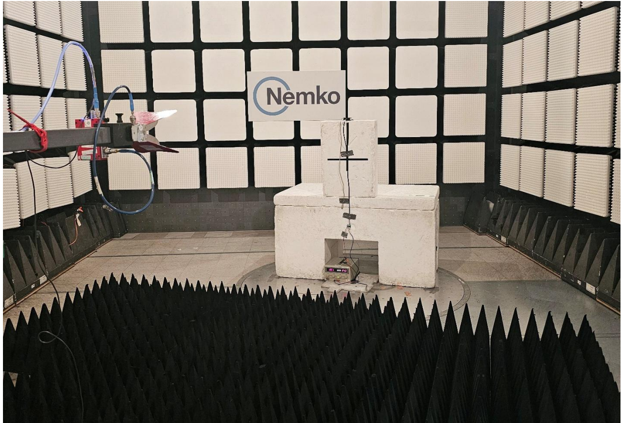
Photo 3 – Test Setup (View C). Above 1 GHz.
