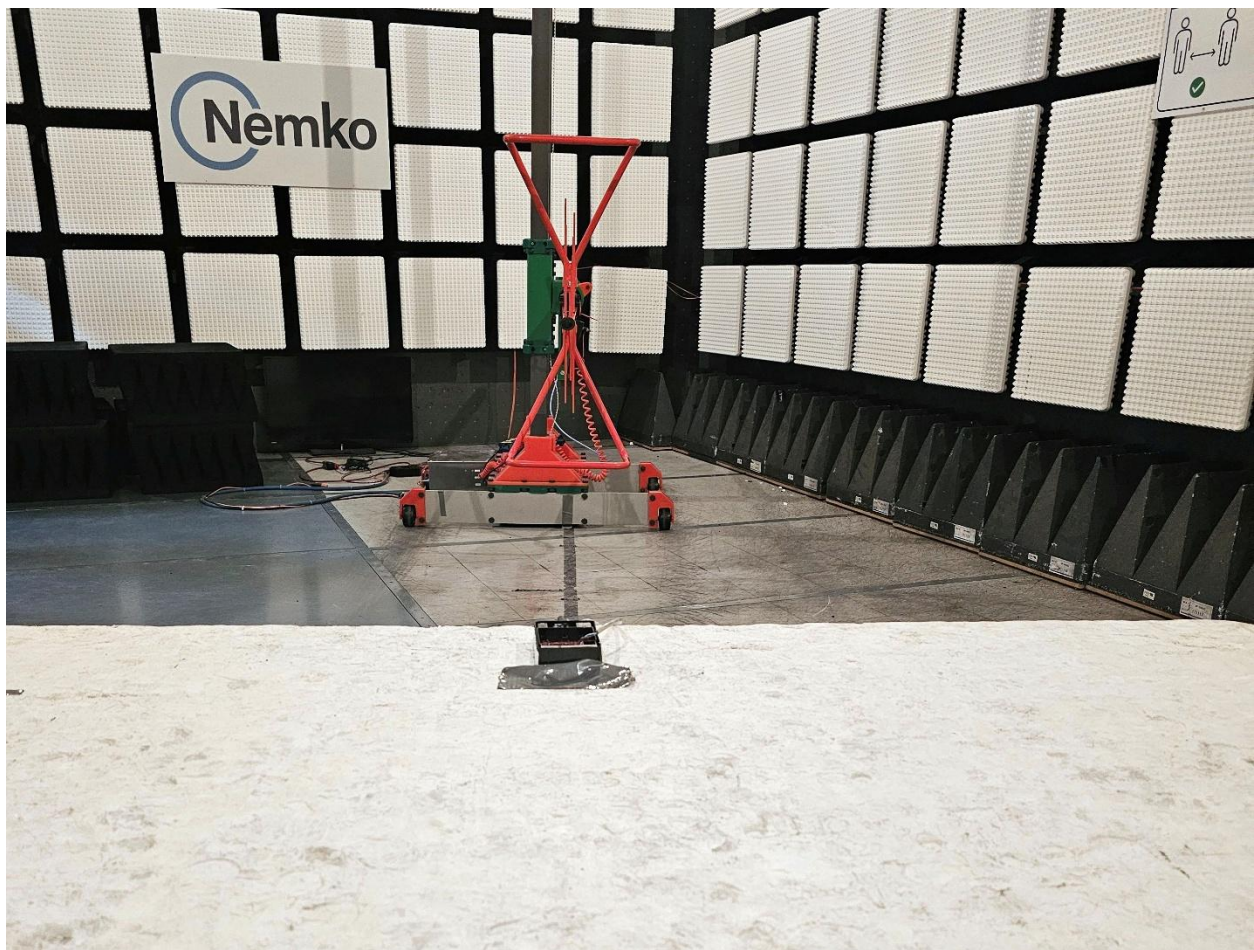
Photo 1 – Test Setup (View A). Below 1 GHz
