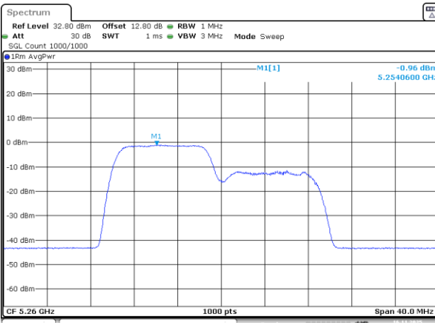
802.11be20_5260MHz_RU_106/53_Chain 3
