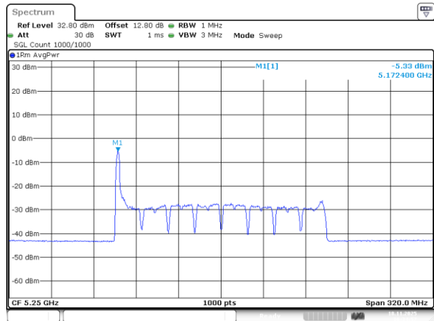
802.11be160_5250MHz_RU_26/0_Chain 1
