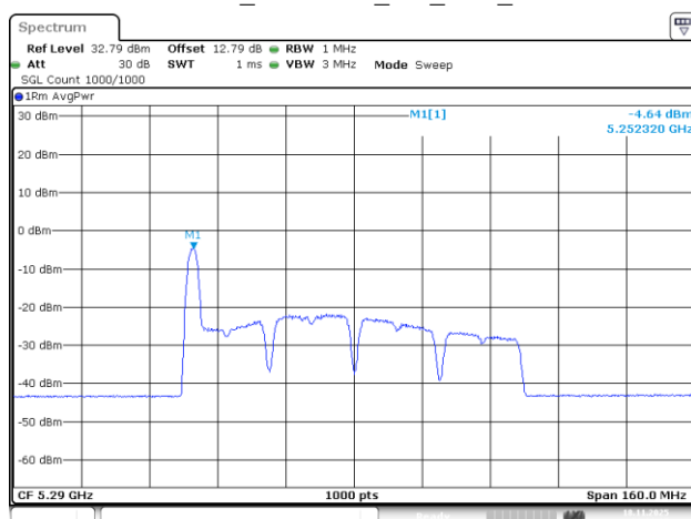
802.11be80_5290MHz_RU_26/0_Chain 3
