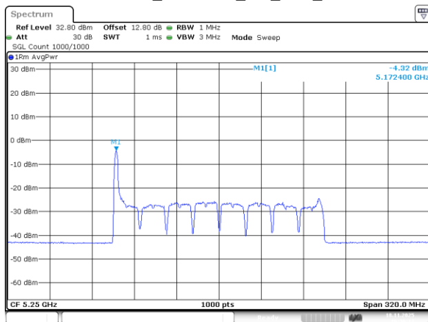
802.11be160_5250MHz_RU_26/0_Chain 2
