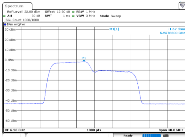
802.11be20_5260MHz_RU_106/53_Chain 0
