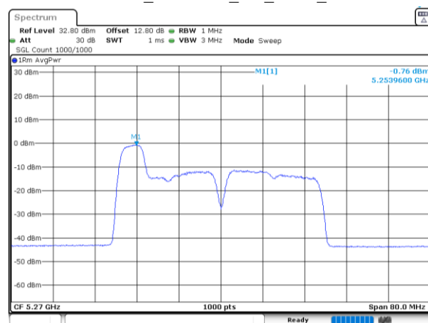
802.11be40_5270MHz_RU_52/37_Chain 2
