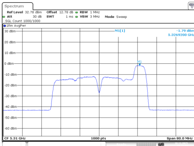
802.11be40_5310MHz_RU_52/44_Chain 1
