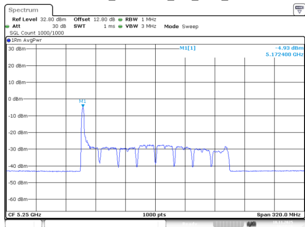
802.11be160_5250MHz_RU_26/0_Chain 3
