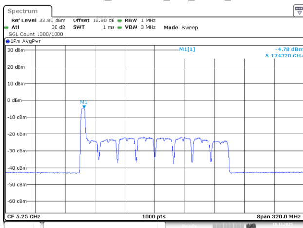
802.11be160_5250MHz_RU_52/37_Chain 2
