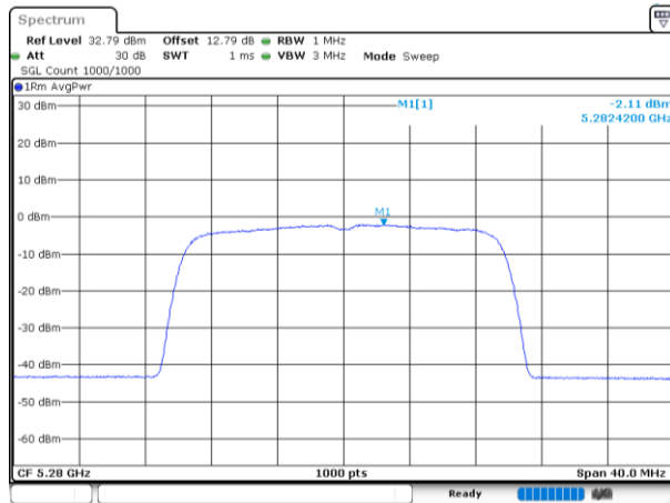
802.11be20_5280MHz_RU_242/61_Chain 1
