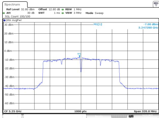
802.11ac160_5250MHz_Chain 1
