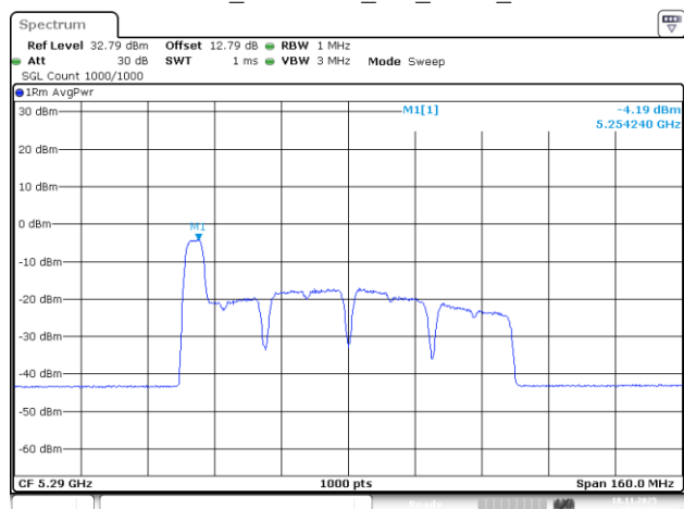
802.11be80_5290MHz_RU_52/37_Chain 3
