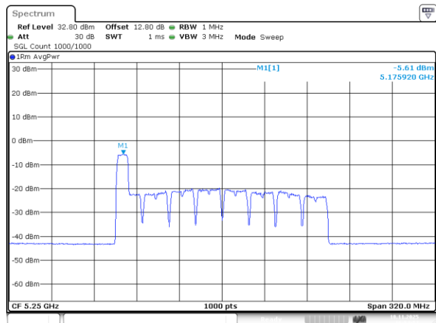
802.11be160_5250MHz_RU_106/53_Chain 1
