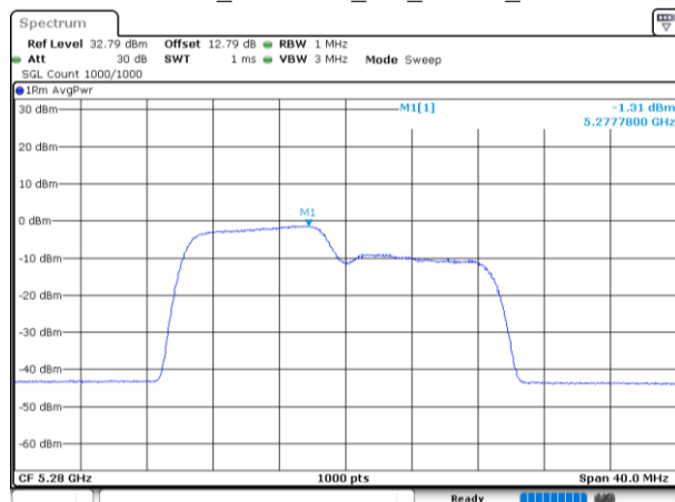
802.11be20_5280MHz_RU_106/53_Chain 1
