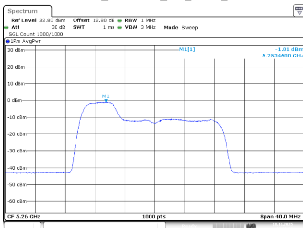
802.11be20_5260MHz_RU_52/37_Chain 3
