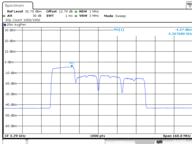
802.11be80_5290MHz_RU_242/61_Chain 0
