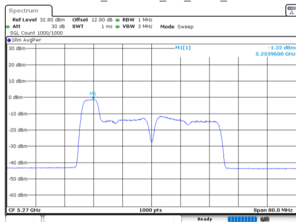
802.11be40_5270MHz_RU_52/37_Chain 0
