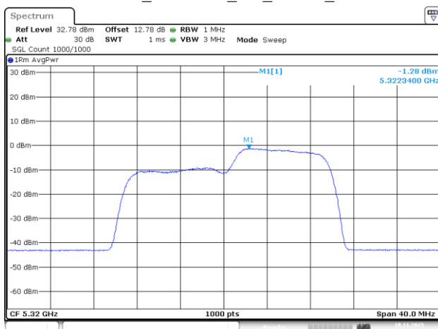
802.11be20_5320MHz_RU_106/54_Chain 1
