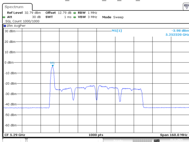
802.11be80_5290MHz_RU_26/0_Chain 0
