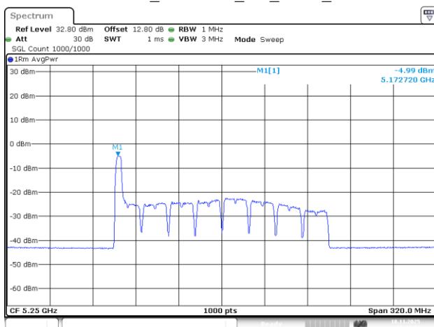
802.11be160_5250MHz_RU_52/37_Chain 3
