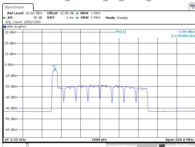
802.11be160_5250MHz_RU_106/53_Chain 2
