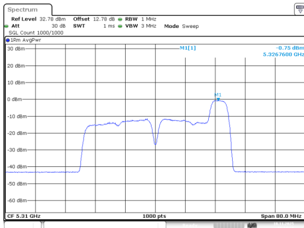
802.11be40_5310MHz_RU_52/44_Chain 0
