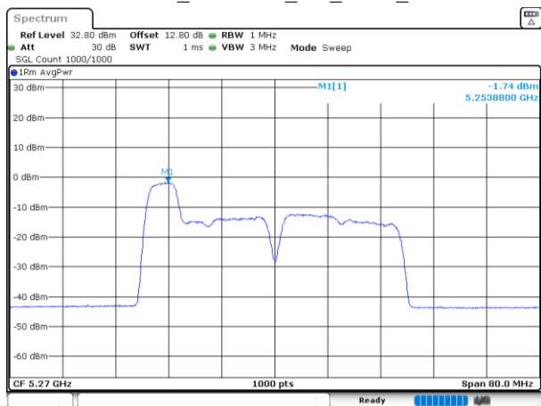
802.11be40_5270MHz_RU_52/37_Chain 1
