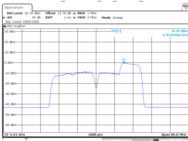
802.11be40_5310MHz_RU_106/56_Chain 2
