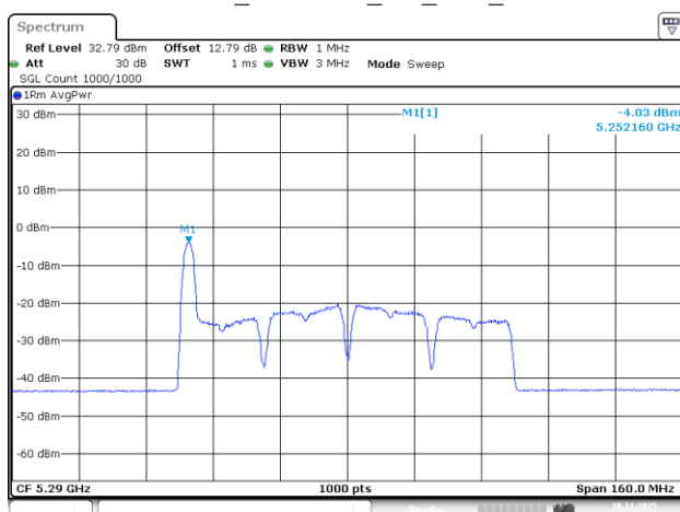
802.11be80_5290MHz_RU_26/0_Chain 2
