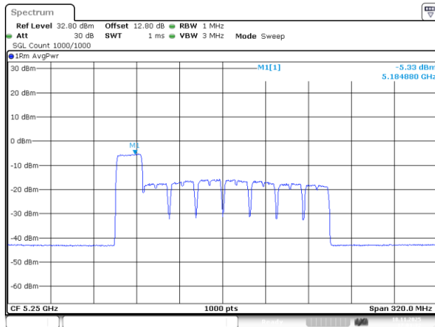
802.11be160_5250MHz_RU_242/61_Chain 0
