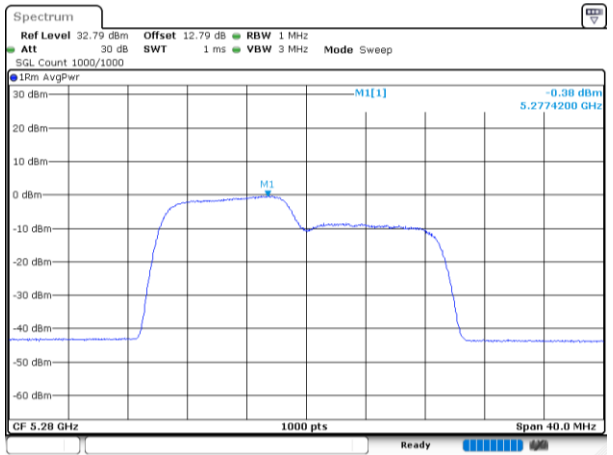
802.11be20_5280MHz_RU_106/53_Chain 2
