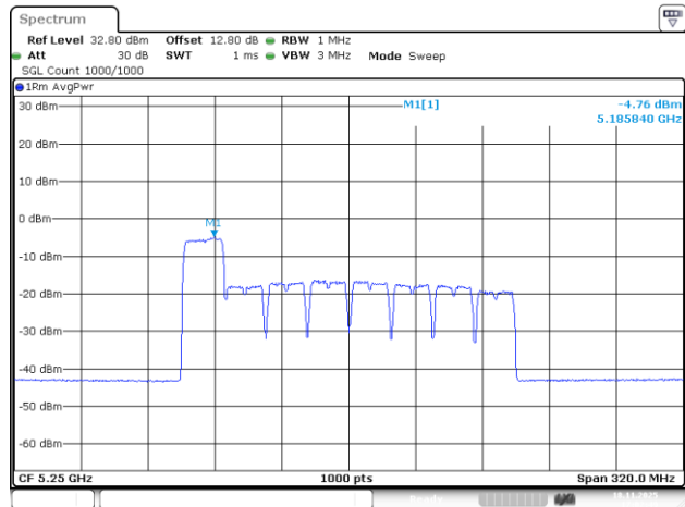
802.11be160_5250MHz_RU_242/61_Chain 1
