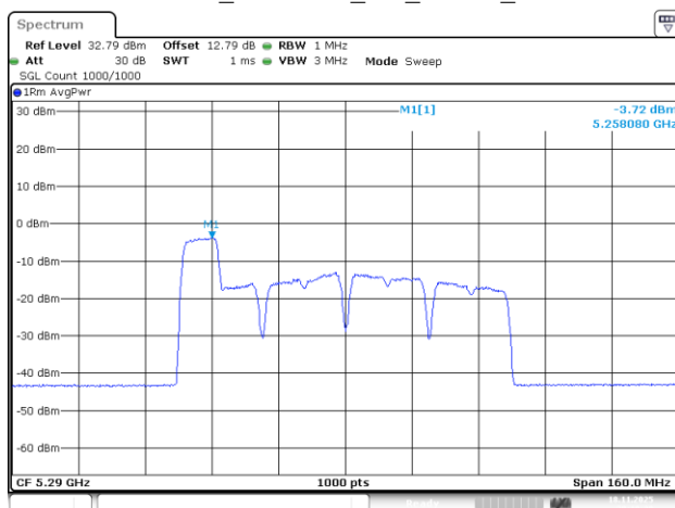
802.11be80_5290MHz_RU_106/53_Chain 2
