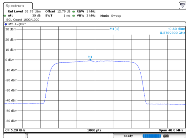
802.11be20_5280MHz_RU_242/61_Chain 2
