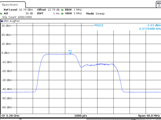
802.11be20_5280MHz_RU_106/53_Chain 3
