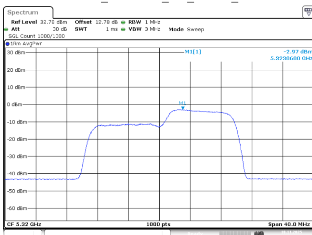
802.11be20_5320MHz_RU_106/54_Chain 3
