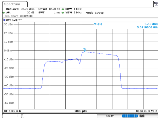
802.11be40_5310MHz_RU_242/62_Chain 0
