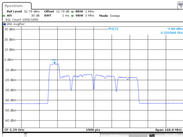
802.11be80_5290MHz_RU_106/53_Chain 0
