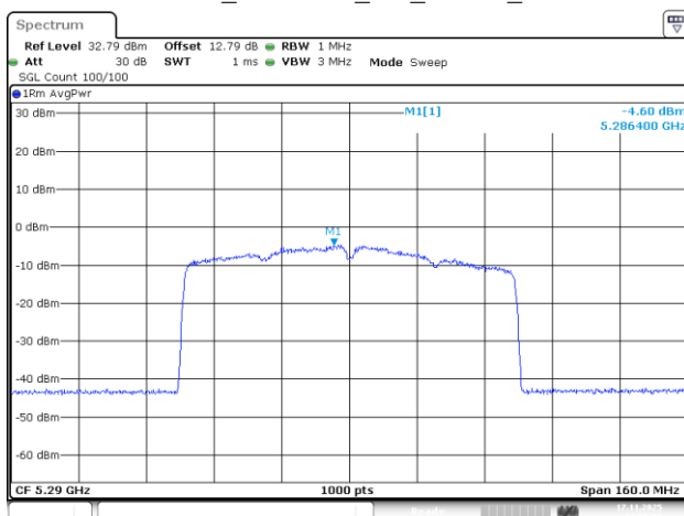
802.11be80_5290MHz_RU_996/67_Chain 3
