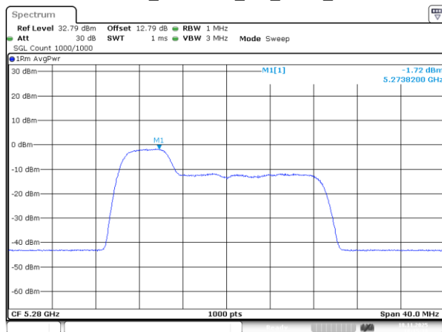
802.11be20_5280MHz_RU_52/37_Chain 1
