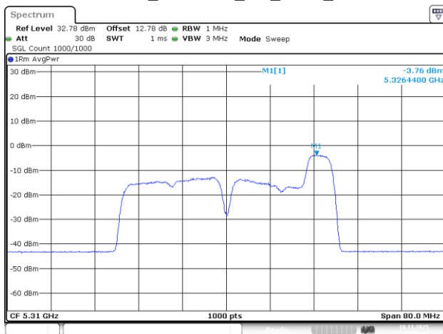
802.11be40_5310MHz_RU_52/44_Chain 3
