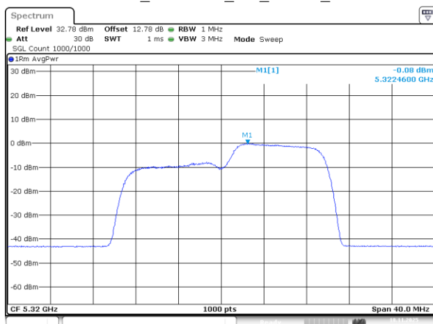
802.11be20_5320MHz_RU_106/54_Chain 0
