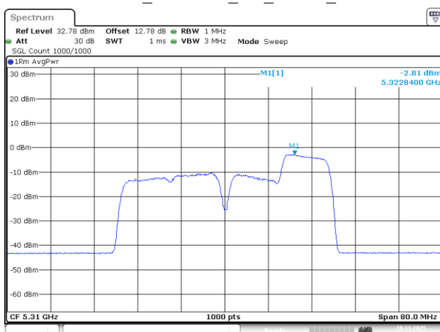
802.11be40_5310MHz_RU_106/56_Chain 3
