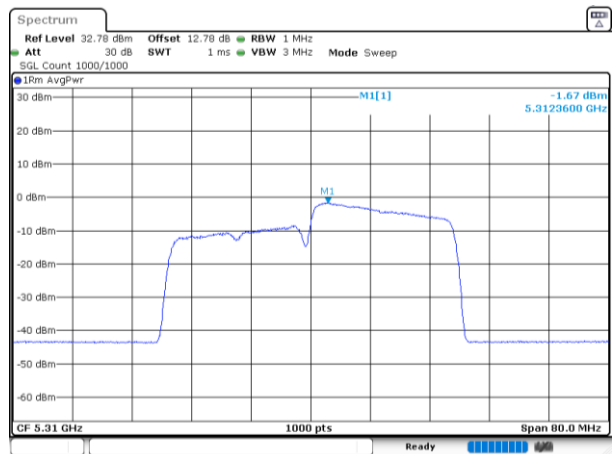
802.11be40_5310MHz_RU_242/62_Chain 3
