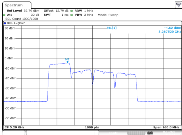
802.11be80_5290MHz_RU_242/61_Chain 1
