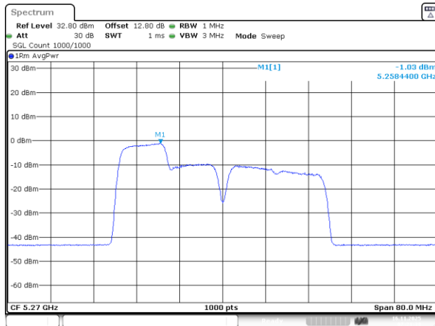
802.11be40_5270MHz_RU_106/53_Chain 0
