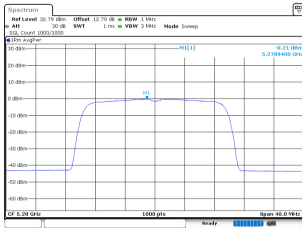
802.11be20_5280MHz_RU_242/61_Chain 3
