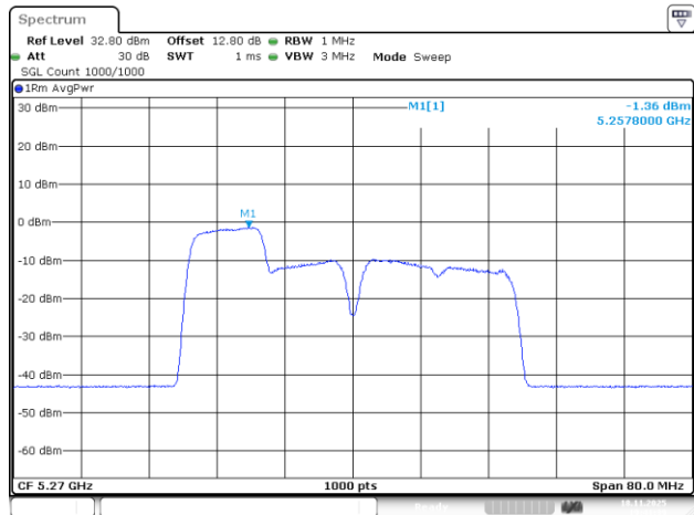
802.11be40_5270MHz_RU_106/53_Chain 1
