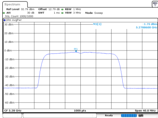
802.11be20_5280MHz_RU_242/61_Chain 0
