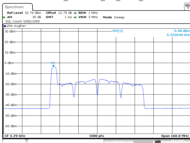
802.11be80_5290MHz_RU_52/37_Chain 2
