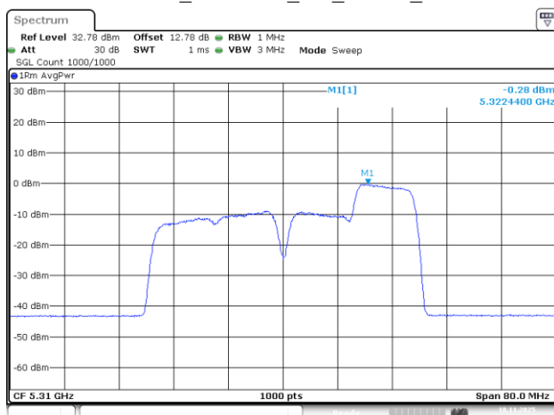
802.11be40_5310MHz_RU_106/56_Chain 0
