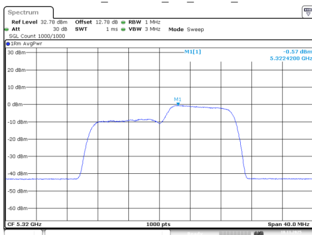
802.11be20_5320MHz_RU_106/54_Chain 2
