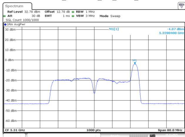
802.11be40_5310MHz_RU_26/17_Chain 3
