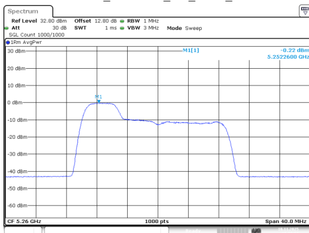
802.11be20_5260MHz_RU_52/37_Chain 2
