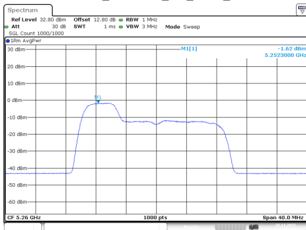
802.11be20_5260MHz_RU_52/37_Chain 1
