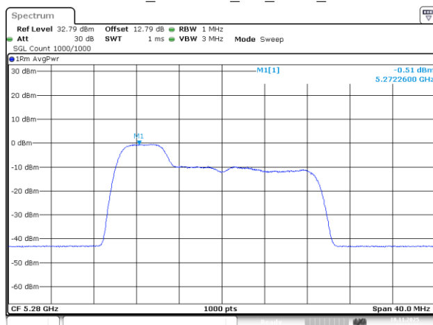
802.11be20_5280MHz_RU_52/37_Chain 2
