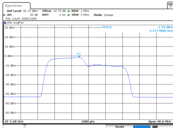
802.11be20_5280MHz_RU_106/53_Chain 0
