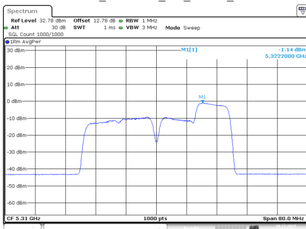
802.11be40_5310MHz_RU_106/56_Chain 1
