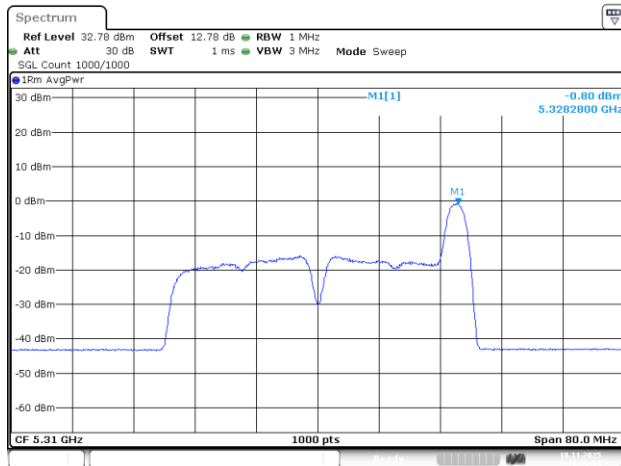
802.11be40_5310MHz_RU_26/17_Chain 0
