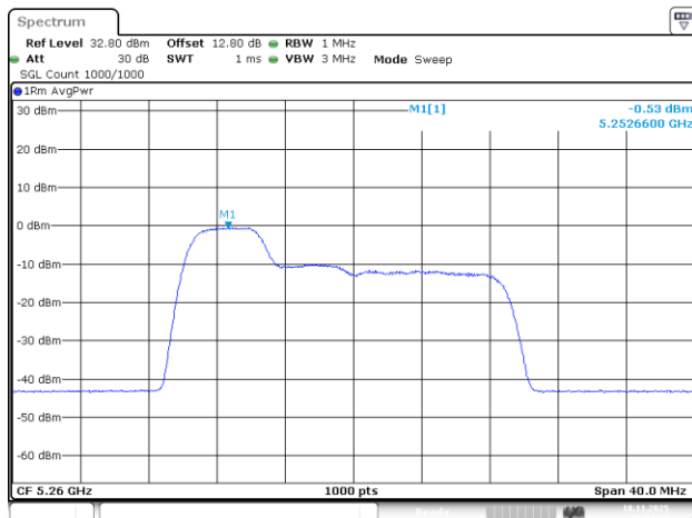
802.11be20_5260MHz_RU_52/37_Chain 0
