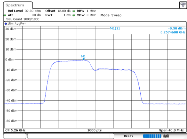
802.11be20_5260MHz_RU_106/53_Chain 2
