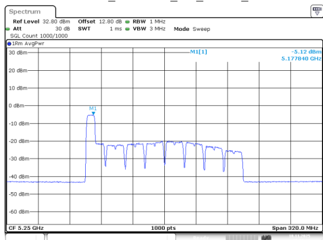
802.11be160_5250MHz_RU_106/53_Chain 3
