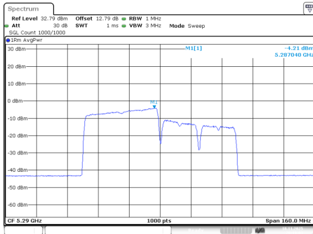
802.11be80_5290MHz_RU_484/65_Chain 0
