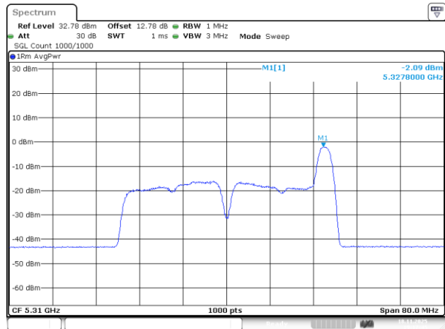
802.11be40_5310MHz_RU_26/17_Chain 1
