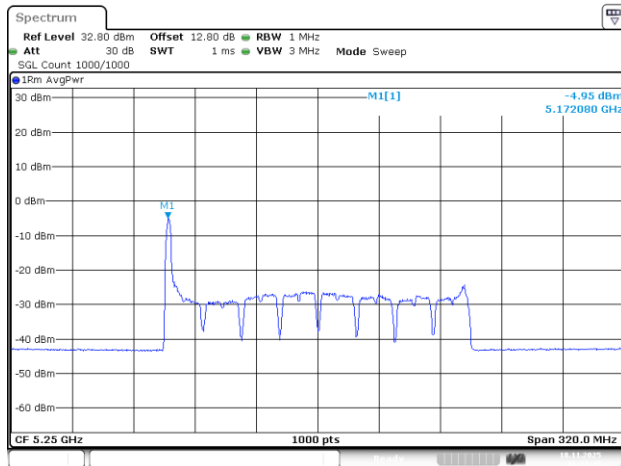
802.11be160_5250MHz_RU_26/0_Chain 0
