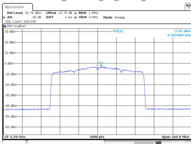
802.11be80_5290MHz_RU_996/67_Chain 2
