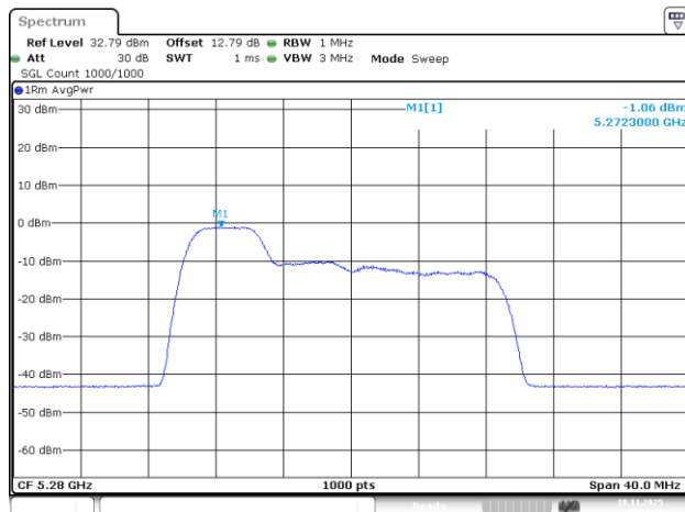
802.11be20_5280MHz_RU_52/37_Chain 0
