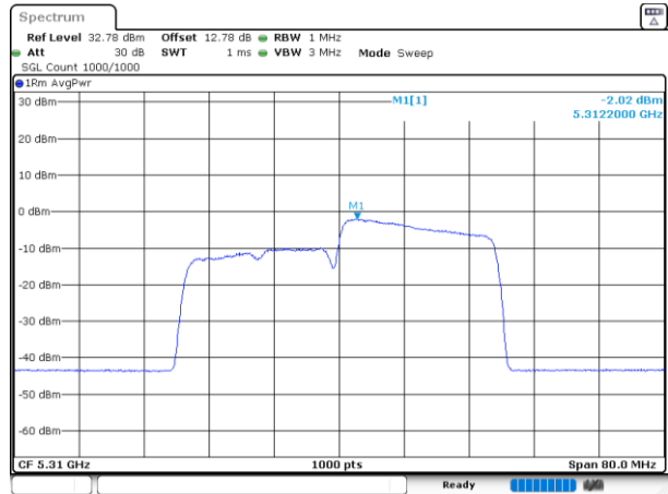
802.11be40_5310MHz_RU_242/62_Chain 1
