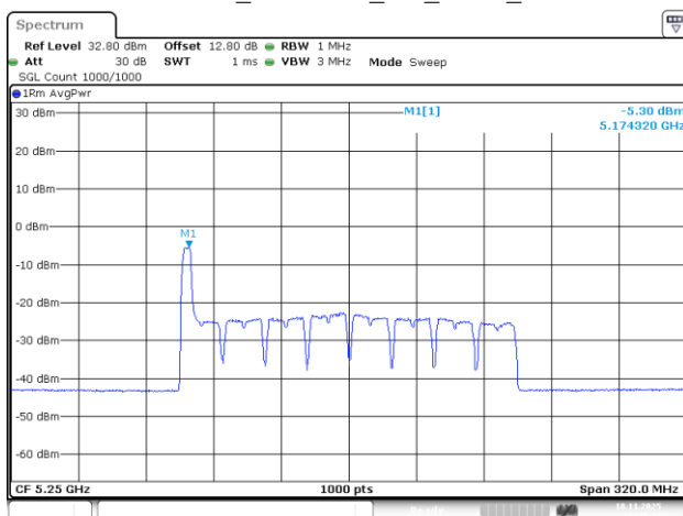
802.11be160_5250MHz_RU_52/37_Chain 1
