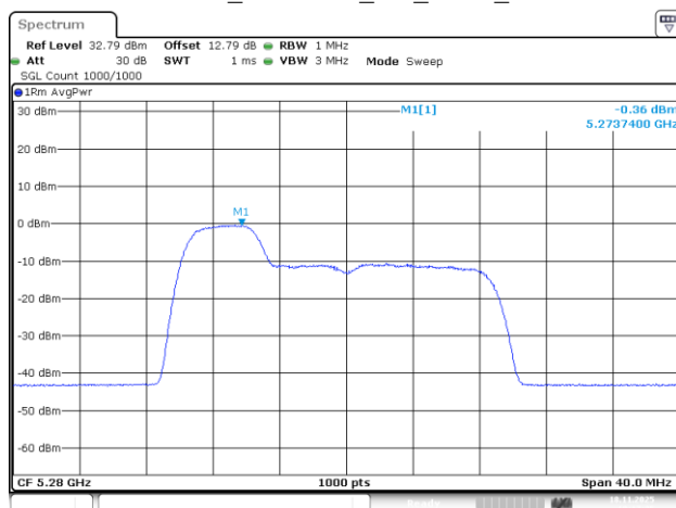
802.11be20_5280MHz_RU_52/37_Chain 3
