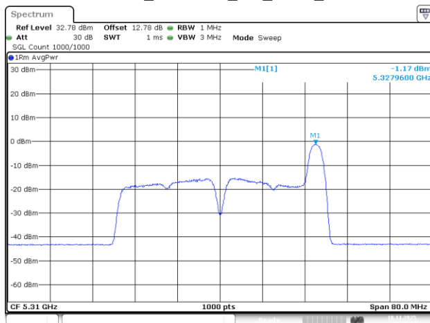
802.11be40_5310MHz_RU_26/17_Chain 2
