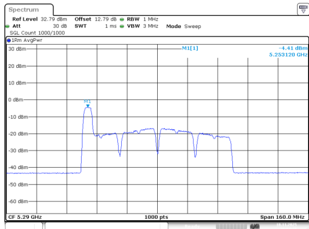
802.11be80_5290MHz_RU_52/37_Chain 1
