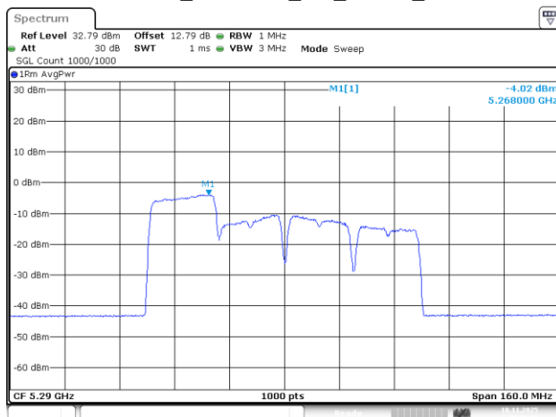
802.11be80_5290MHz_RU_242/61_Chain 2
