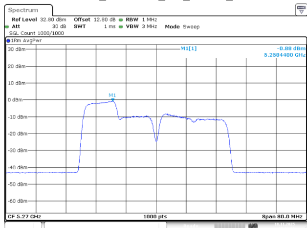
802.11be40_5270MHz_RU_106/53_Chain 3
