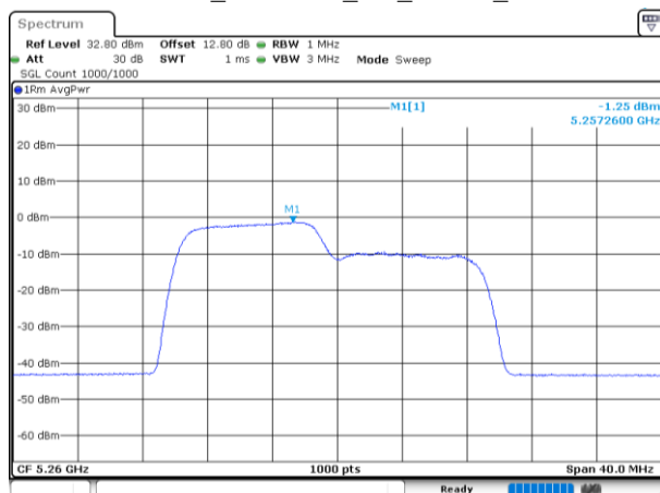
802.11be20_5260MHz_RU_106/53_Chain 1
