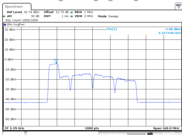
802.11be80_5290MHz_RU_106/53_Chain 3
