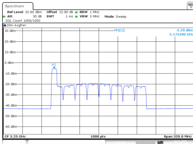
802.11be160_5250MHz_RU_106/53_Chain 0
