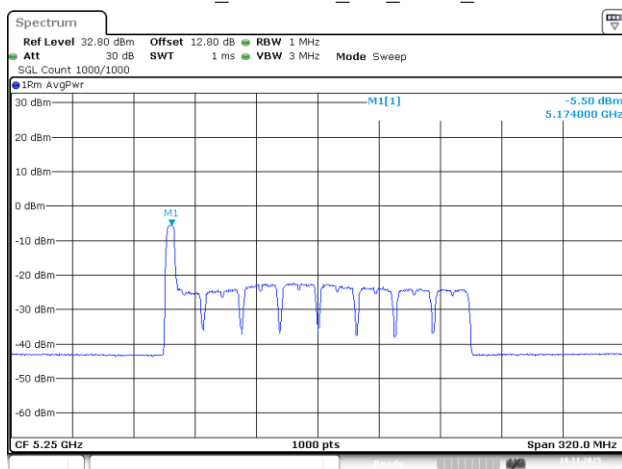
802.11be160_5250MHz_RU_52/37_Chain 0
