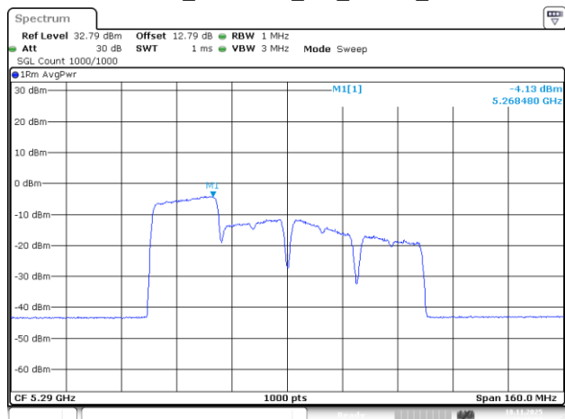
802.11be80_5290MHz_RU_242/61_Chain 3
