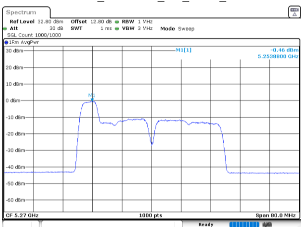
802.11be40_5270MHz_RU_52/37_Chain 3
