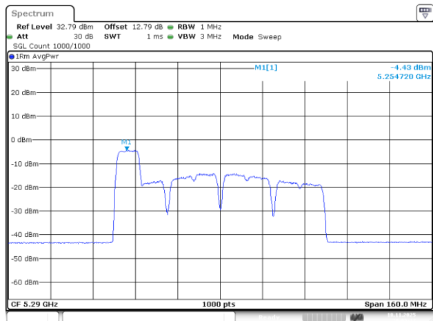
802.11be80_5290MHz_RU_106/53_Chain 1
