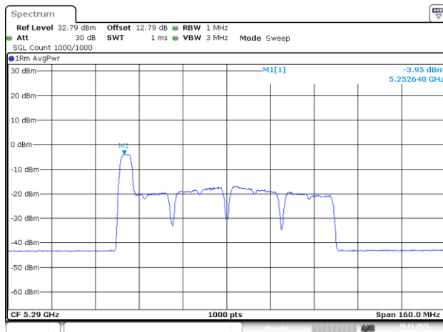
802.11be80_5290MHz_RU_52/37_Chain 0
