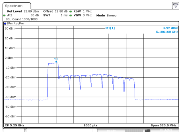
802.11be160_5250MHz_RU_242/61_Chain 3
