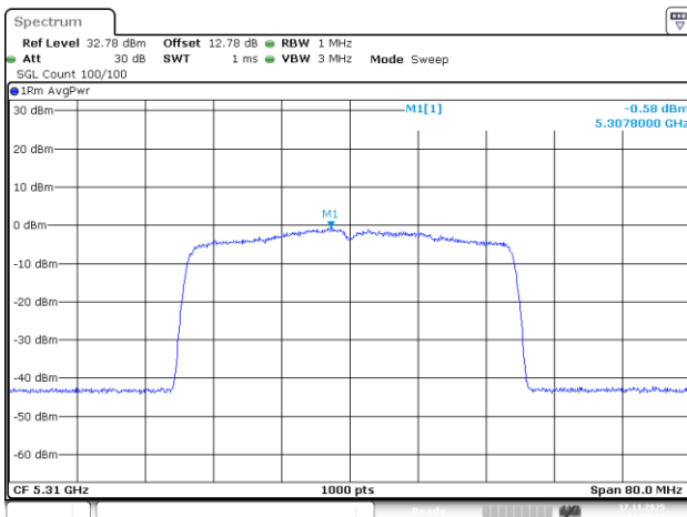
802.11be40_5310MHz_RU_484/65_Chain 0
