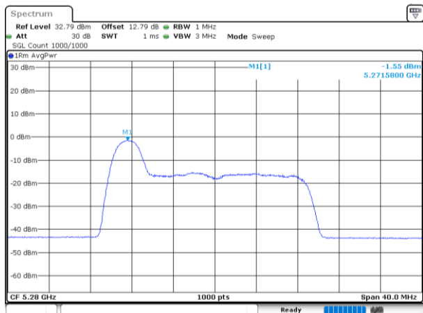
802.11be20_5280MHz_RU_26/0_Chain 0
