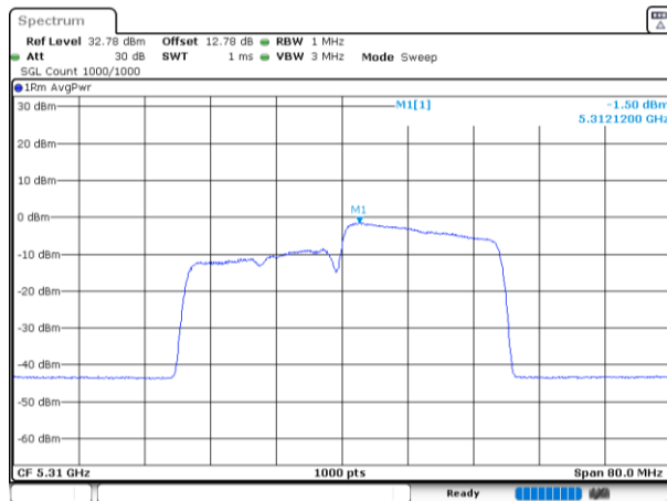
802.11be40_5310MHz_RU_242/62_Chain 2
