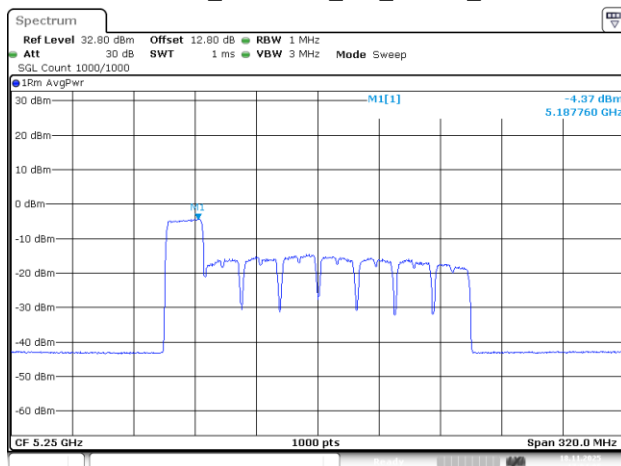
802.11be160_5250MHz_RU_242/61_Chain 2
