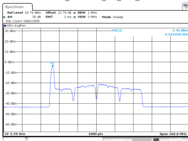
802.11be80_5290MHz_RU_26/0_Chain 1
