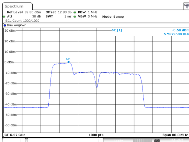
802.11be40_5270MHz_RU_106/53_Chain 2
