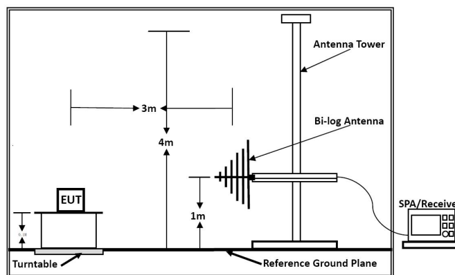
Below 1GHz
