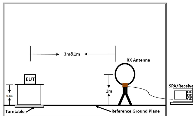
Below 30MHz
