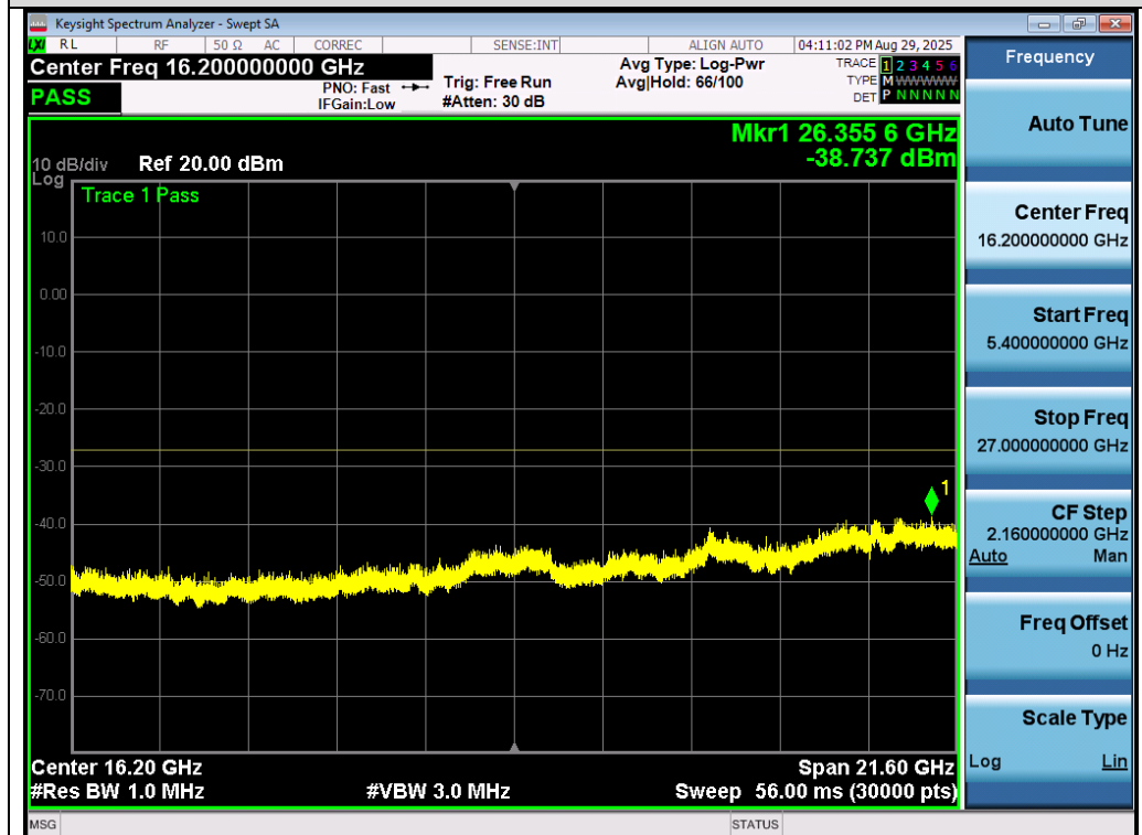
Test_Graph_802.11a_ANT1_5180_6Mbps_Frequency Band 4
