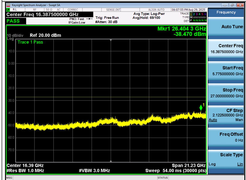
Test_Graph_802.11ac80_ANT1_5610_MCS0_Frequency Band 4
