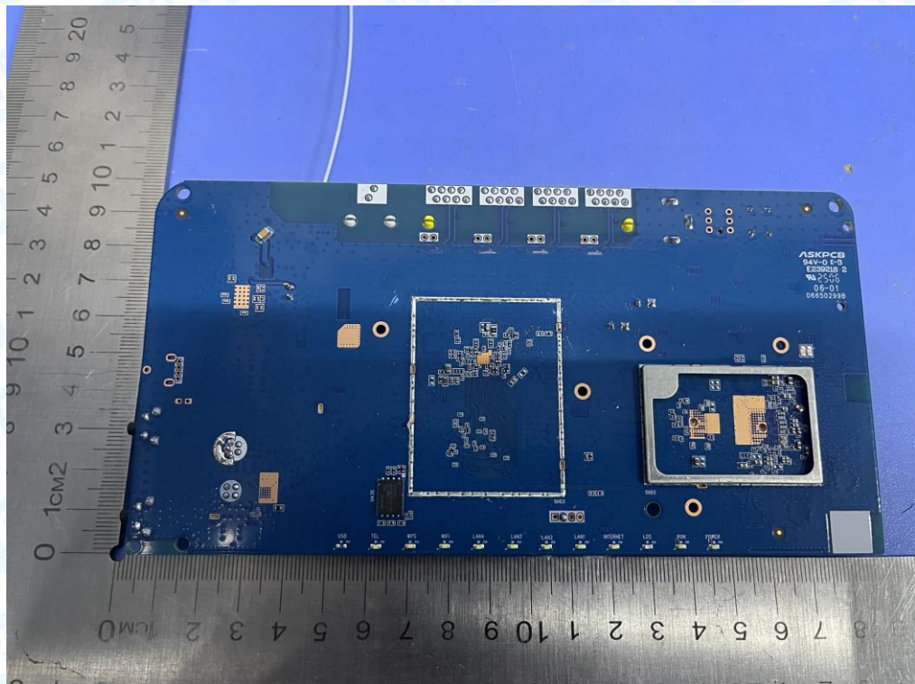
Photo 12 Appearance of PCB
