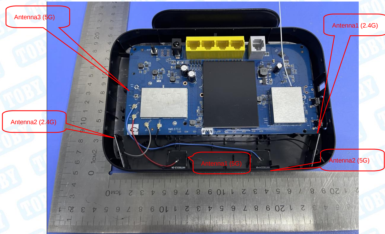
Photo 10 Internal of EUT
