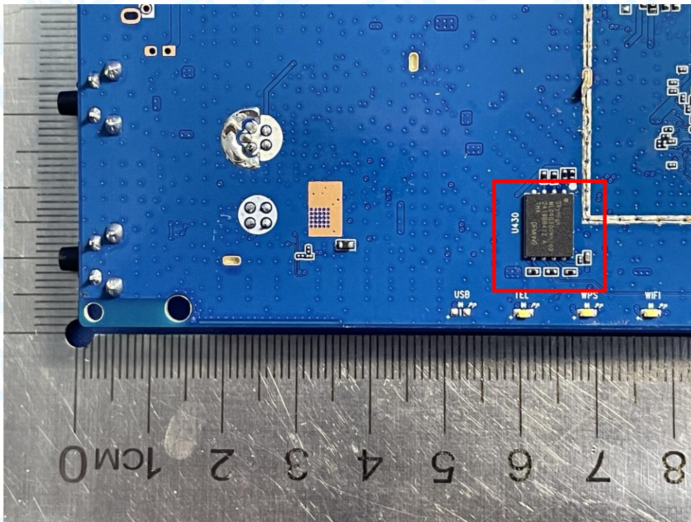
Photo 16 Appearance of PCB (Flash 2#)
