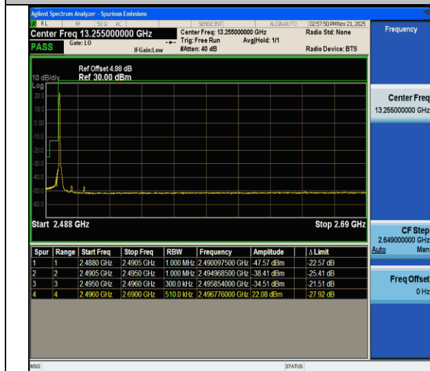
CA_41C-15MHz-15MHz-QPSK@QPSK-QPSK@QPSK-39725-39875-1RB#0@75RB#0-0RB#0@75RB#0-PASS
