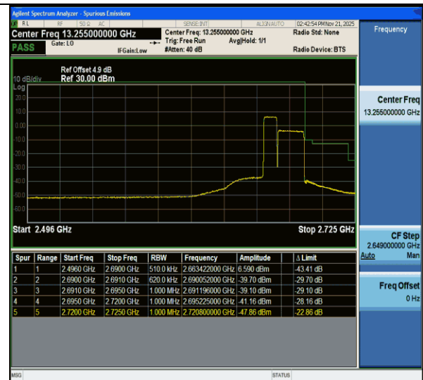
CA_41C-10MHz-20MHz-QPSK@QPSK-QPSK@QPSK-41346-41490-50RB#0@50RB#0-100RB#0@100RB#0-PASS
