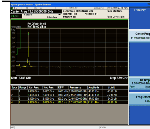
CA_41C-15MHz-20MHz-QPSK@QPSK-QPSK@QPSK-39728-39899-1RB#74@75RB#0-0RB#0@100RB#0-PASS
