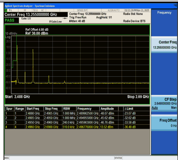
CA_41C-10MHz-15MHz-QPSK@QPSK-QPSK@QPSK-39703-39823-1RB#0@50RB#0-1RB#74@75RB#0-PASS
