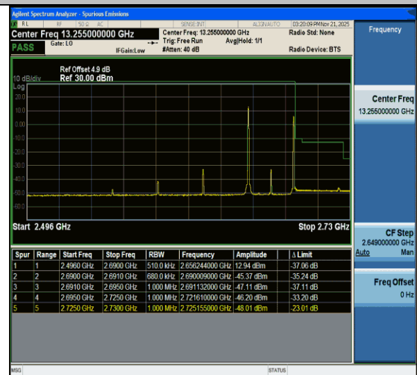
CA_41C-15MHz-20MHz-QPSK@QPSK-QPSK@QPSK-41319-41490-1RB#0@75RB#0-1RB#99@100RB#0-PASS
