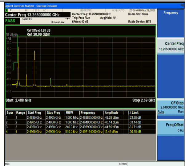
CA_41C-20MHz-5MHz-QPSK@QPSK-QPSK@QPSK-39750-39867-1RB#0@100RB#0-1RB#24@25RB#0-PASS
