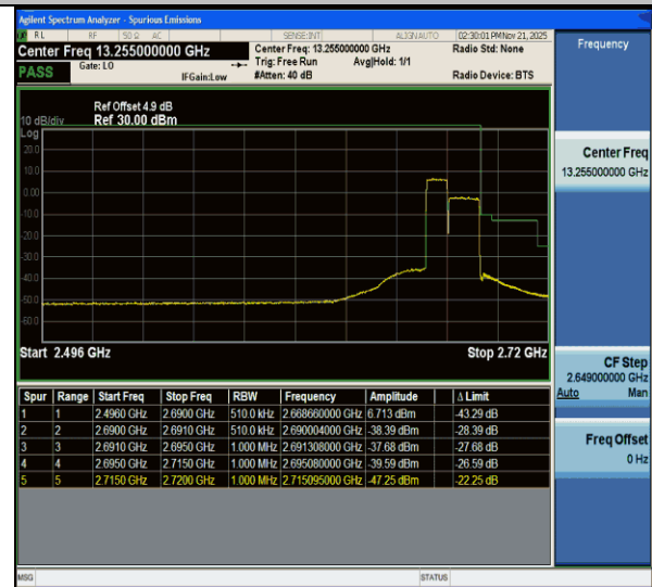
CA_41C-10MHz-15MHz-QPSK@QPSK-QPSK@QPSK-41395-41515-50RB#0@50RB#0-75RB#0@75RB#0-PASS
