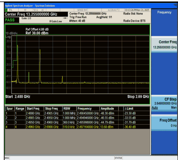
CA_41C-15MHz-20MHz-QPSK@QPSK-QPSK@QPSK-39728-39899-1RB#0@75RB#0-1RB#99@100RB#0-PASS
