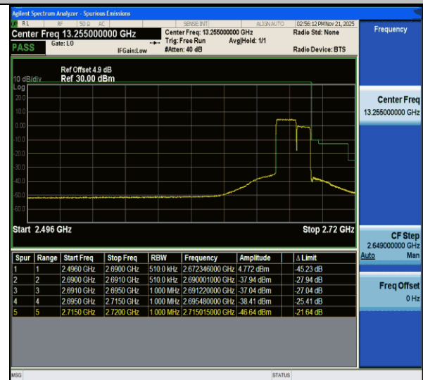
CA_41C-15MHz-10MHz-QPSK@QPSK-QPSK@QPSK-41417-41537-75RB#0@75RB#0-50RB#0@50RB#0-PASS
