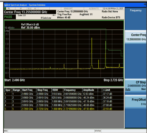
CA_41C-10MHz-20MHz-QPSK@QPSK-QPSK@QPSK-41346-41490-1RB#0@50RB#0-1RB#99@100RB#0-PASS
