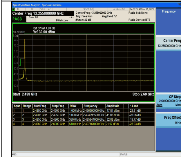
CA_41C-20MHz-20MHz-QPSK@QPSK-QPSK@QPSK-39750-39948-1RB#0@100RB#0-0RB#0@100RB#0-PASS
