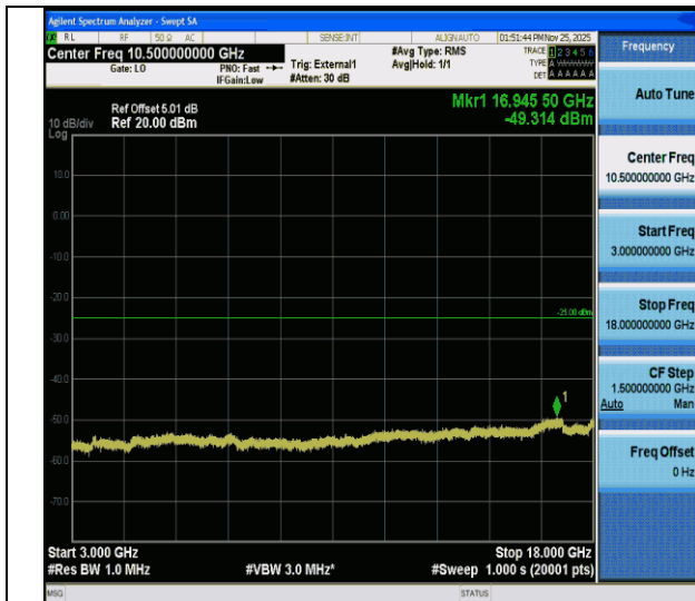
CA_41C-20MHz-20MHz-QPSK-QPSK-40521-40719-1RB#0- ORB#0-3000~18000MHz-PASS
