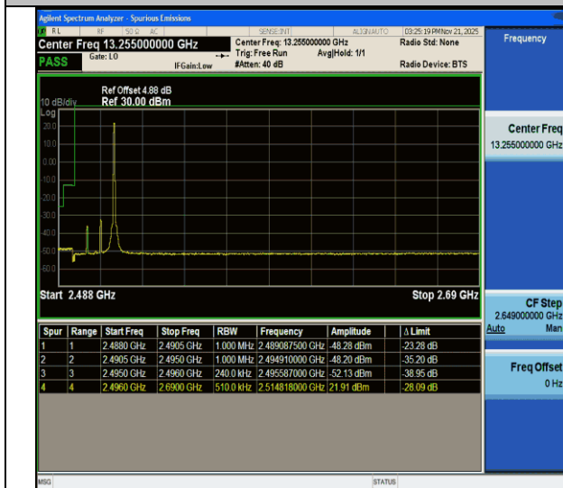
CA_41C-20MHz-5MHz-QPSK@QPSK-QPSK@QPSK-39750-39867-1RB#99@100RB#0-0RB#0@25RB#0-PASS
