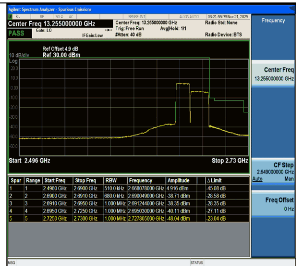
CA_41C-15MHz-20MHz-QPSK@QPSK-QPSK@QPSK-41319-41490-75RB#0@75RB#0-100RB#0@100RB#0-PASS
