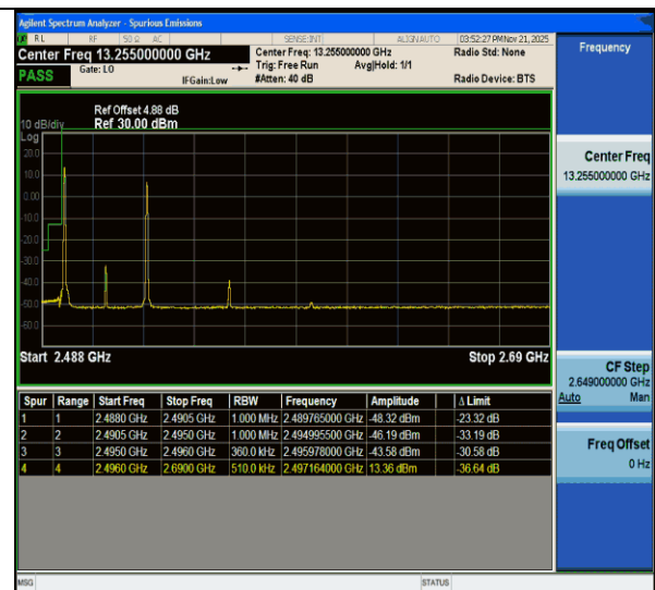
CA_41C-20MHz-15MHz-QPSK@QPSK-QPSK@QPSK-39750-39921-1RB#0@100RB#0-1RB#74@75RB#0-PASS
