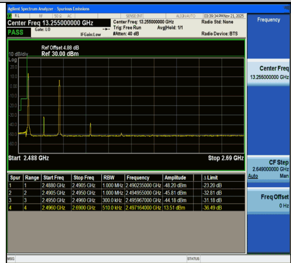
CA_41C-20MHz-10MHz-QPSK@QPSK-QPSK@QPSK-39750-39894-1RB#0@100RB#0-1RB#49@50RB#0-PASS
