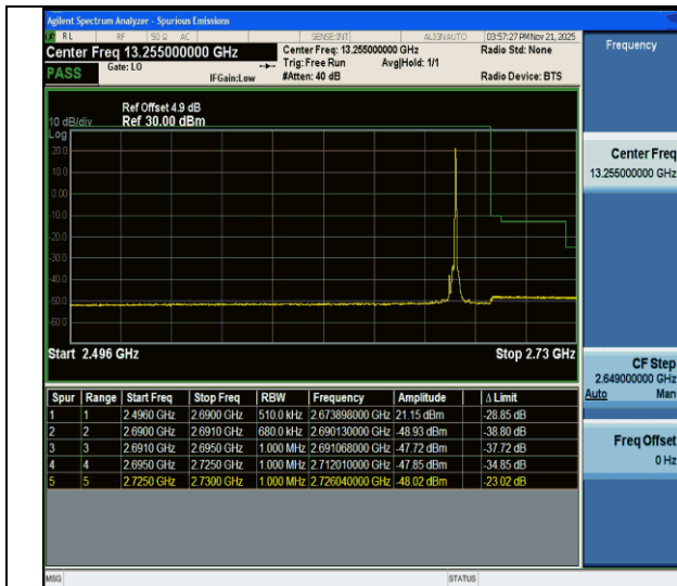
CA_41C-20MHz-15MHz-QPSK@QPSK-QPSK@QPSK-41341-41512-1RB#99@100RB#0-0RB#0@75RB#0-PASS
