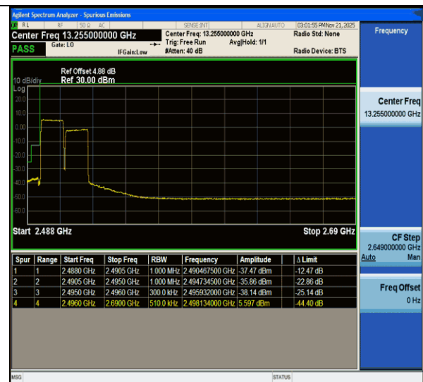
CA_41C-15MHz-15MHz-QPSK@QPSK-QPSK@QPSK-39725-39875-75RB#0@75RB#0-75RB#0@75RB#0-PASS
