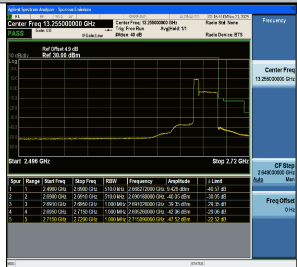
CA_41C-5MHz-20MHz-QPSK@QPSK-QPSK@QPSK-41373-41490-25RB#0@25RB#0-100RB#0@100RB#0-PASS
