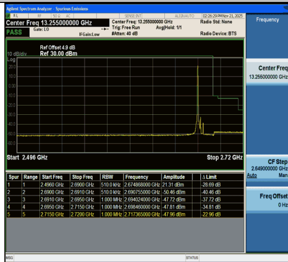
CA_41C-10MHz-15MHz-QPSK@QPSK-QPSK@QPSK-41395-41515-1RB#49@50RB#0-0RB#0@75RB#0-PASS
