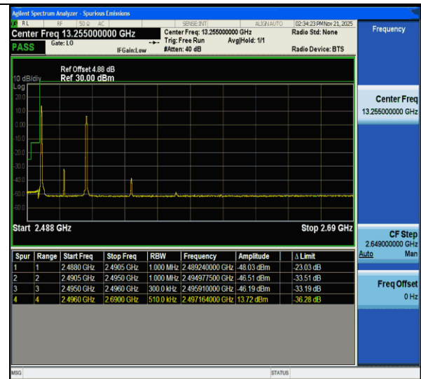
CA_41C-10MHz-20MHz-QPSK@QPSK-QPSK@QPSK-39705-39849-1RB#0@50RB#0-1RB#99@100RB#0-PASS
