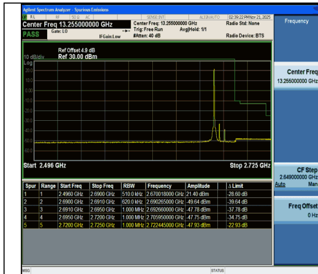
CA_41C-10MHz-20MHz-QPSK@QPSK-QPSK@QPSK-41346-41490-1RB#49@50RB#0-0RB#0@100RB#0-PASS
