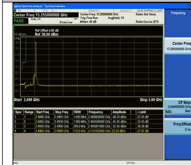
CA_41C-15MHz-10MHz-QPSK@QPSK-QPSK@QPSK-39725-39845-1RB#74@75RB#0-0RB#0@50RB#0-PASS
