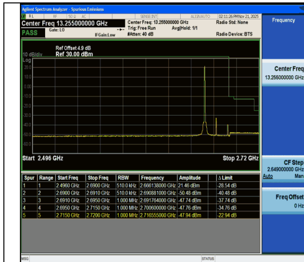
CA_41C-5MHz-20MHz-QPSK@QPSK-QPSK@QPSK-41373-41490-1RB#0@25RB#0-0RB#0@100RB#0-PASS
