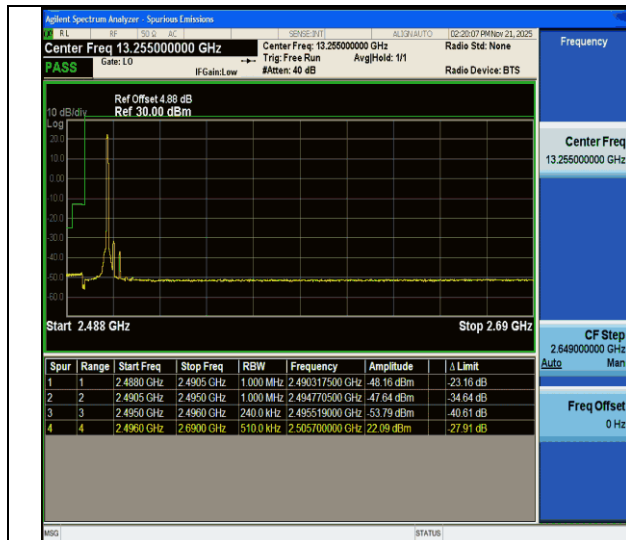
CA_41C-10MHz-15MHz-QPSK@QPSK-QPSK@QPSK-39703-39823-1RB#49@50RB#0-0RB#0@75RB#0-PASS
