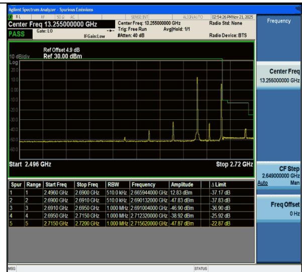
CA_41C-15MHz-10MHz-QPSK@QPSK-QPSK@QPSK-41417-41537-1RB#0@75RB#0-1RB#49@50RB#0-PASS
