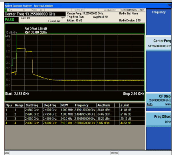
CA_41C-15MHz-10MHz-QPSK@QPSK-QPSK@QPSK-39725-39845-75RB#0@75RB#0-50RB#0@50RB#0-PASS
