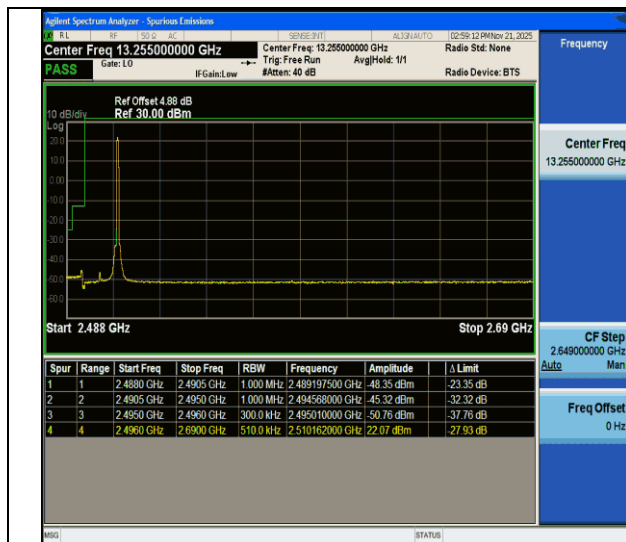
CA_41C-15MHz-15MHz-QPSK@QPSK-QPSK@QPSK-39725-39875-1RB#74@75RB#0-0RB#0@75RB#0-PASS
