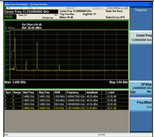
CA_41C-20MHz-20MHz-QPSK@QPSK-QPSK@QPSK-39750-39948-1RB#0@100RB#0-1RB#99@100RB#0-PASS
