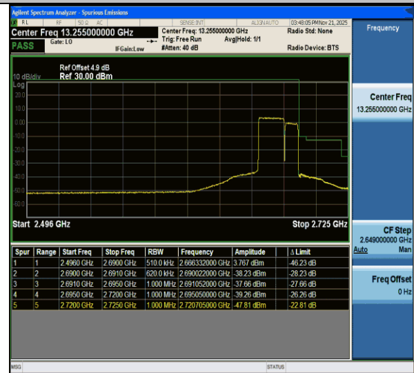
CA_41C-20MHz-10MHz-QPSK@QPSK-QPSK@QPSK-41391-41535-100RB#0@100RB#0-50RB#0@50RB#0-PASS
