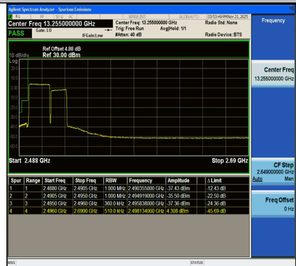
CA_41C-20MHz-15MHz-QPSK@QPSK-QPSK@QPSK-39750-39921-100RB#0@100RB#0-75RB#0@75RB#0-PASS
