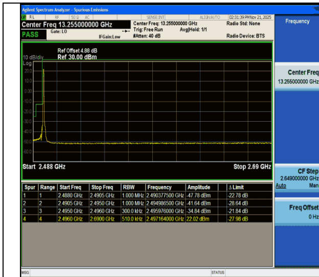
CA_41C-10MHz-20MHz-QPSK@QPSK-QPSK@QPSK-39705-39849-1RB#0@50RB#0-0RB#0@100RB#0-PASS
