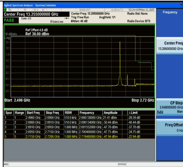
CA_41C-10MHz-15MHz-QPSK@QPSK-QPSK@QPSK-41395-41515-1RB#0@50RB#0-0RB#0@75RB#0-PASS
