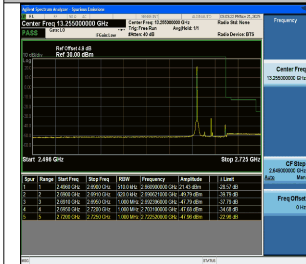
CA_41C-15MHz-15MHz-QPSK@QPSK-QPSK@QPSK-41365-41515-1RB#0@75RB#0-0RB#0@75RB#0-PASS
