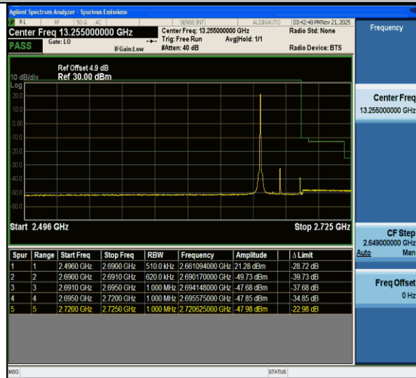
CA_41C-20MHz-10MHz-QPSK@QPSK-QPSK@QPSK-41391-41535-1RB#0@100RB#0-0RB#0@50RB#0-PASS
