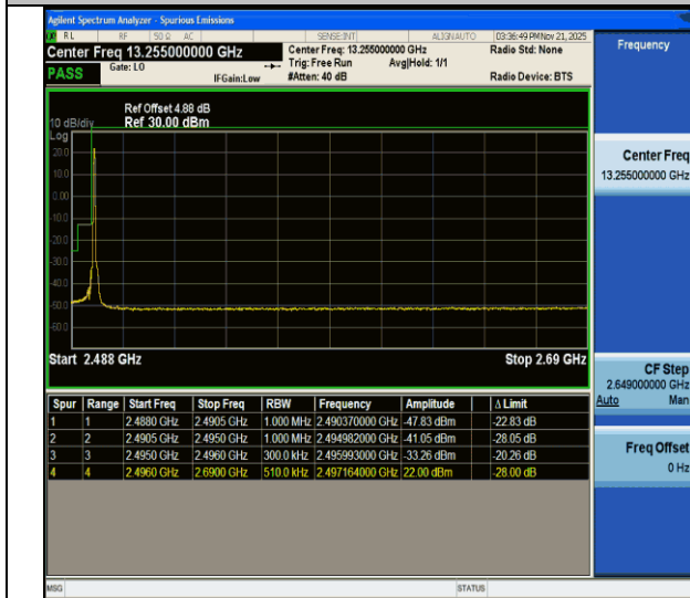
CA_41C-20MHz-10MHz-QPSK@QPSK-QPSK@QPSK-39750-39894-1RB#0@100RB#0-0RB#0@50RB#0-PASS
