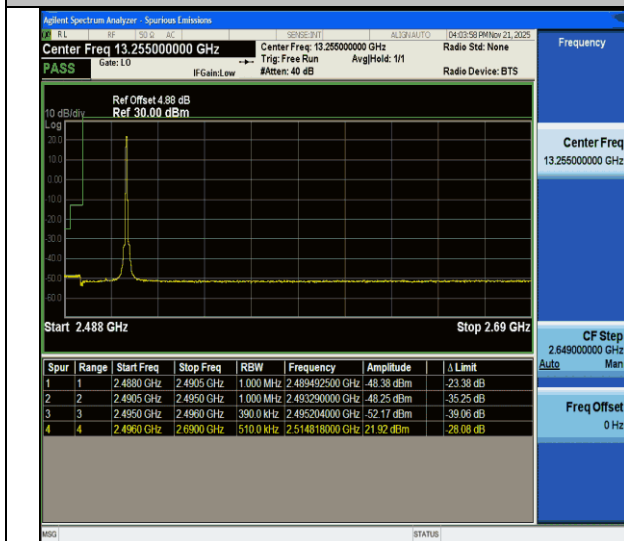
CA_41C-20MHz-20MHz-QPSK@QPSK-QPSK@QPSK-39750-39948-1RB#99@100RB#0-0RB#0@100RB#0-PASS
