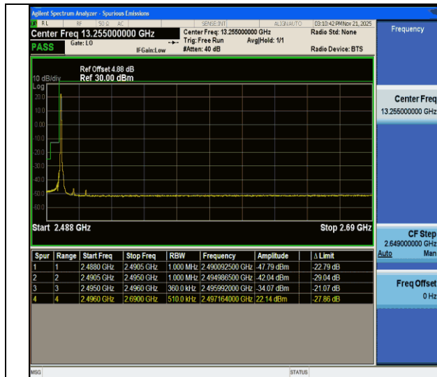
CA_41C-15MHz-20MHz-QPSK@QPSK-QPSK@QPSK-39728-39899-1RB#0@75RB#0-0RB#0@100RB#0-PASS
