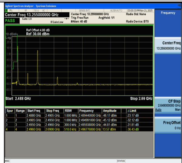
CA_41C-15MHz-15MHz-QPSK@QPSK-QPSK@QPSK-39725-39875-1RB#0@75RB#0-1RB#74@75RB#0-PASS
