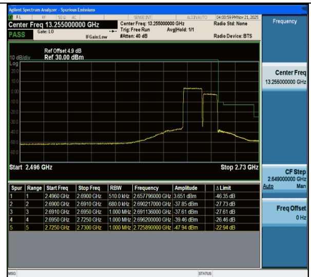
CA_41C-20MHz-15MHz-QPSK@QPSK-QPSK@QPSK-41341-41512-100RB#0@100RB#0-75RB#0@75RB#0-PASS
