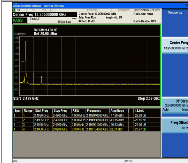
CA_41C-20MHz-5MHz-QPSK@QPSK-QPSK@QPSK-39750-39867-1RB#0@100RB#0-0RB#0@25RB#0-PASS
