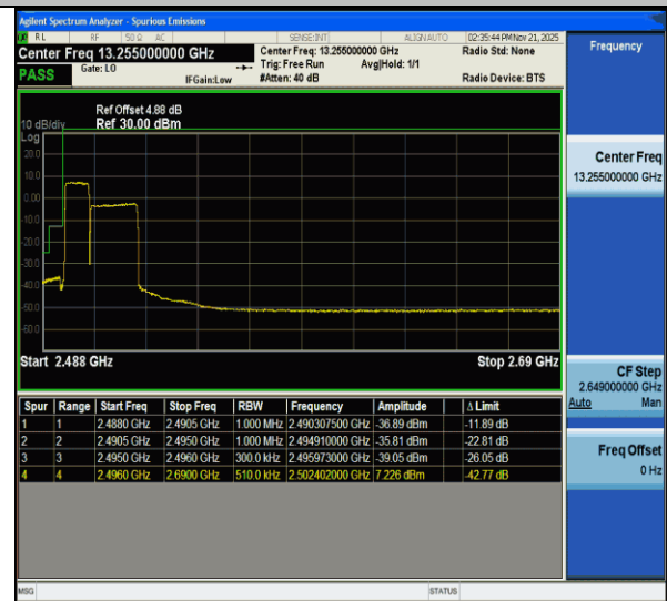
CA_41C-10MHz-20MHz-QPSK@QPSK-QPSK@QPSK-39705-39849-50RB#0@50RB#0-100RB#0@100RB#0-PASS
