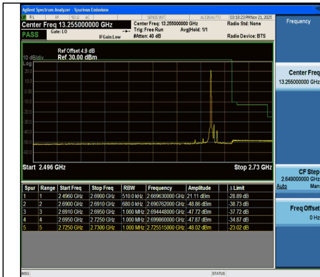
CA_41C-15MHz-20MHz-QPSK@QPSK-QPSK@QPSK-41319-41490-1RB#74@75RB#0-0RB#0@100RB#0-PASS
