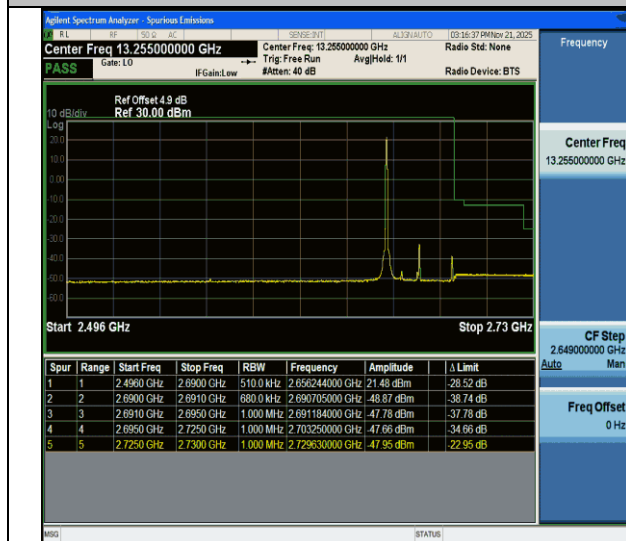
CA_41C-15MHz-20MHz-QPSK@QPSK-QPSK@QPSK-41319-41490-1RB#0@75RB#0-0RB#0@100RB#0-PASS
