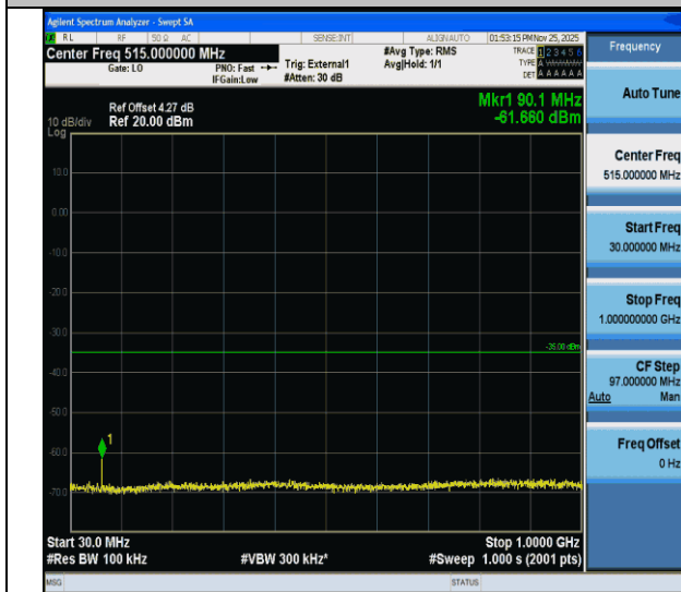
CA_41C-20MHz-20MHz-QPSK-QPSK-41292-41490-1RB#0- ORB#0-30~1000MHz-PASS
