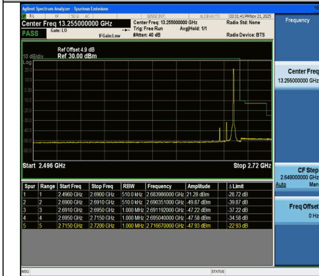
CA_41C-20MHz-5MHz-QPSK@QPSK-QPSK@QPSK-41440-41557-1RB#99@100RB#0-0RB#0@25RB#0-PASS
