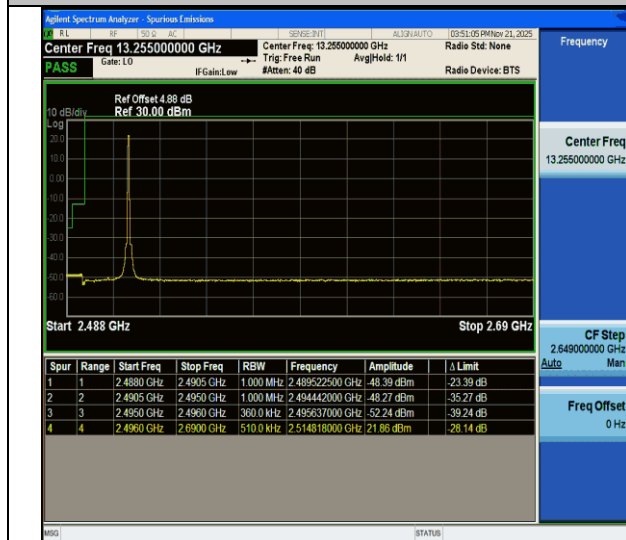
CA_41C-20MHz-15MHz-QPSK@QPSK-QPSK@QPSK-39750-39921-1RB#99@100RB#0-0RB#0@75RB#0-PASS
