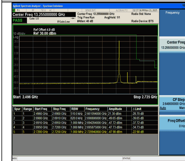
CA_41C-10MHz-20MHz-QPSK@QPSK-QPSK@QPSK-41346-41490-1RB#0@50RB#0-0RB#0@100RB#0-PASS
