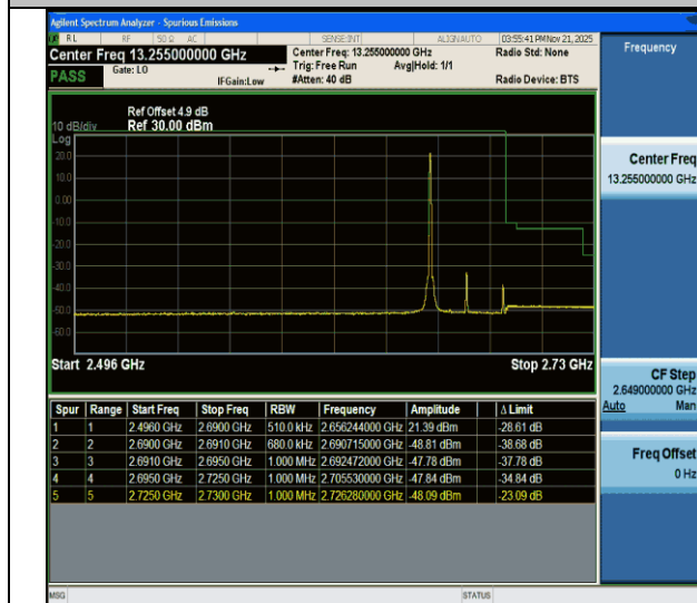
CA_41C-20MHz-15MHz-QPSK@QPSK-QPSK@QPSK-41341-41512-1RB#0@100RB#0-0RB#0@75RB#0-PASS
