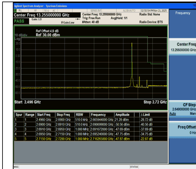
CA_41C-15MHz-10MHz-QPSK@QPSK-QPSK@QPSK-41417-41537-1RB#0@75RB#0-0RB#0@50RB#0-PASS
