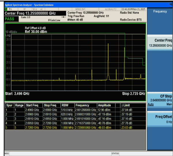
CA_41C-20MHz-10MHz-QPSK@QPSK-QPSK@QPSK-41391-41535-1RB#0@100RB#0-1RB#49@50RB#0-PASS
