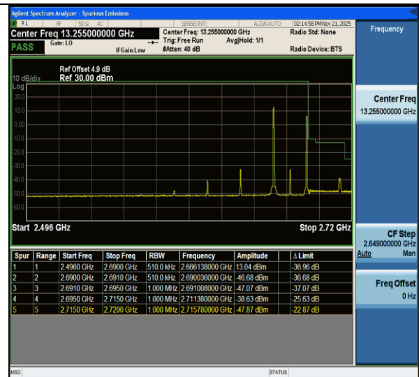
CA_41C-5MHz-20MHz-QPSK@QPSK-QPSK@QPSK-41373-41490-1RB#0@25RB#0-1RB#99@100RB#0-PASS
