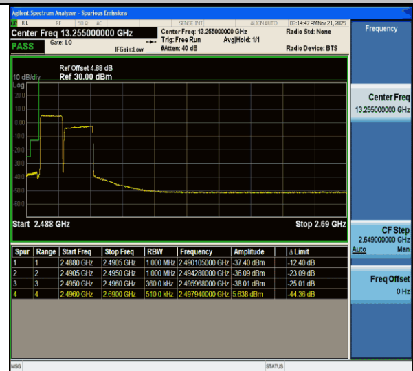
CA_41C-15MHz-20MHz-QPSK@QPSK-QPSK@QPSK-39728-39899-75RB#0@75RB#0-100RB#0@100RB#0-PASS
