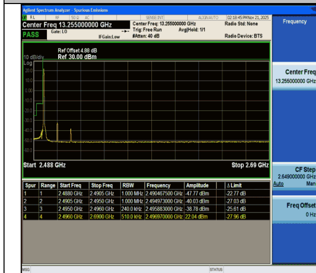
CA_41C-10MHz-15MHz-QPSK@QPSK-QPSK@QPSK-39703-39823-1RB#0@50RB#0-0RB#0@75RB#0-PASS
