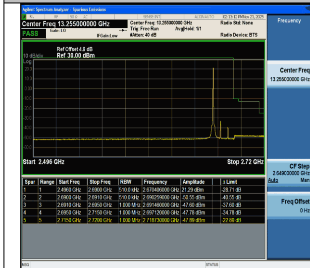
CA_41C-5MHz-20MHz-QPSK@QPSK-QPSK@QPSK-41373-41490-1RB#24@25RB#0-0RB#0@100RB#0-PASS
