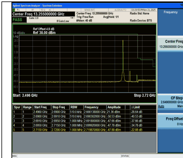
CA_41C-20MHz-5MHz-QPSK@QPSK-QPSK@QPSK-41440-41557-1RB#0@100RB#0-0RB#0@25RB#0-PASS
