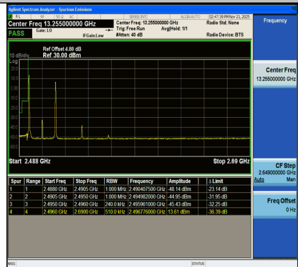
CA_41C-15MHz-10MHz-QPSK@QPSK-QPSK@QPSK-39725-39845-1RB#0@75RB#0-1RB#49@50RB#0-PASS
