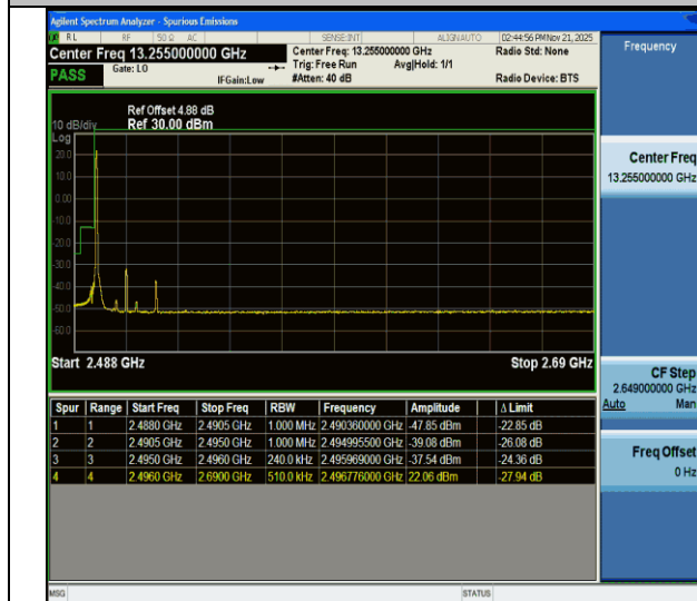
CA_41C-15MHz-10MHz-QPSK@QPSK-QPSK@QPSK-39725-39845-1RB#0@75RB#0-0RB#0@50RB#0-PASS
