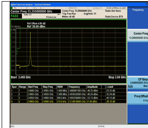
CA_41C-20MHz-10MHz-QPSK@QPSK-QPSK@QPSK-39750-39894-1RB#99@100RB#0-0RB#0@50RB#0-PASS
