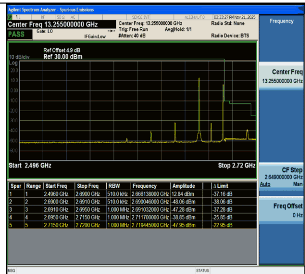
CA_41C-20MHz-5MHz-QPSK@QPSK-QPSK@QPSK-41440-41557-1RB#0@100RB#0-1RB#24@25RB#0-PASS
