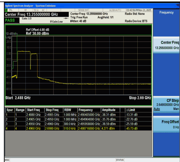
CA_41C-20MHz-10MHz-QPSK@QPSK-QPSK@QPSK-39750-39894-100RB#0@100RB#0-50RB#0@50RB#0-PASS
