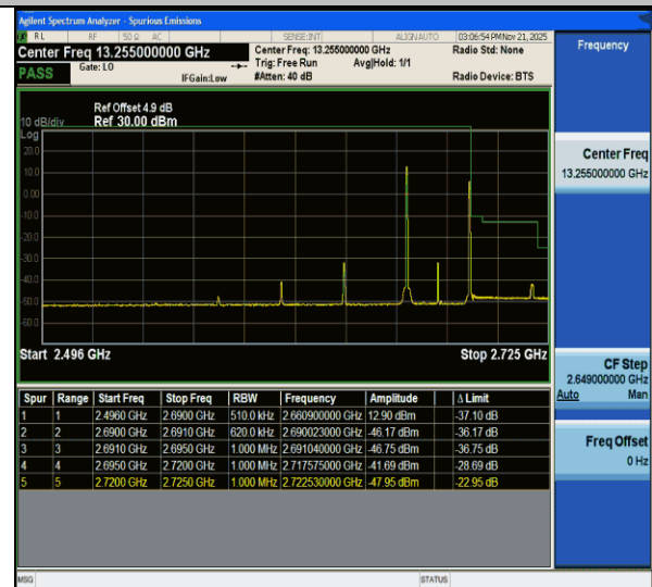
CA_41C-15MHz-15MHz-QPSK@QPSK-QPSK@QPSK-41365-41515-1RB#0@75RB#0-1RB#74@75RB#0-PASS
