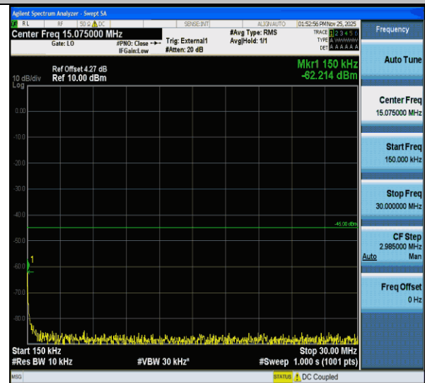
CA_41C-20MHz-20MHz-QPSK-QPSK-41292-41490-1RB#0- ORB#0-0.15~30MHz-PASS
