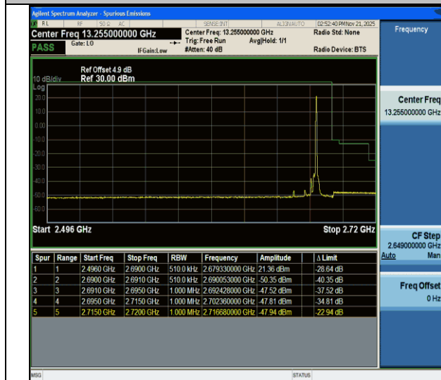
CA_41C-15MHz-10MHz-QPSK@QPSK-QPSK@QPSK-41417-41537-1RB#74@75RB#0-0RB#0@50RB#0-PASS
