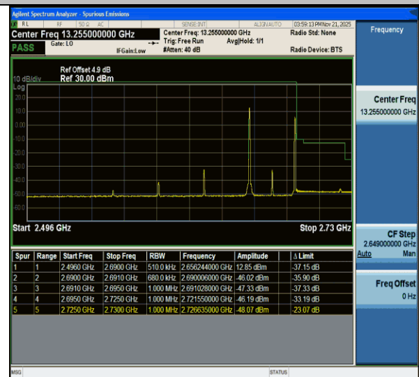
CA_41C-20MHz-15MHz-QPSK@QPSK-QPSK@QPSK-41341-41512-1RB#0@100RB#0-1RB#74@75RB#0-PASS
