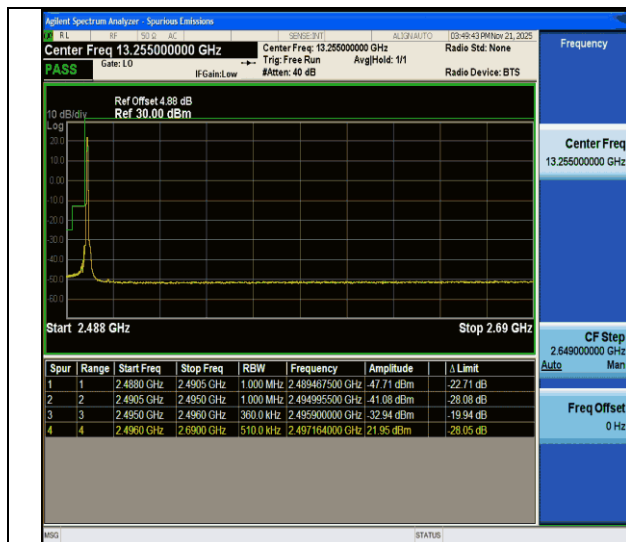
CA_41C-20MHz-15MHz-QPSK@QPSK-QPSK@QPSK-39750-39921-1RB#0@100RB#0-0RB#0@75RB#0-PASS
