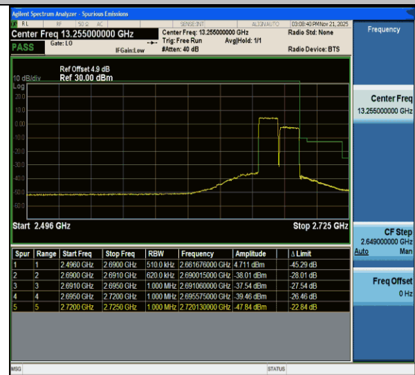
CA_41C-15MHz-15MHz-QPSK@QPSK-QPSK@QPSK-41365-41515-75RB#0@75RB#0-75RB#0@75RB#0-PASS
