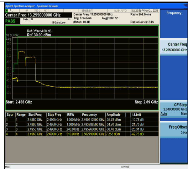
CA_41C-10MHz-15MHz-QPSK@QPSK-QPSK@QPSK-39703-39823-50RB#0@50RB#0-75RB#0@75RB#0-PASS
