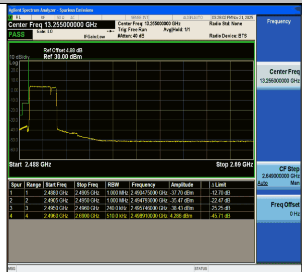
CA_41C-20MHz-5MHz-QPSK@QPSK-QPSK@QPSK-39750-39867-100RB#0@100RB#0-25RB#0@25RB#0-PASS
