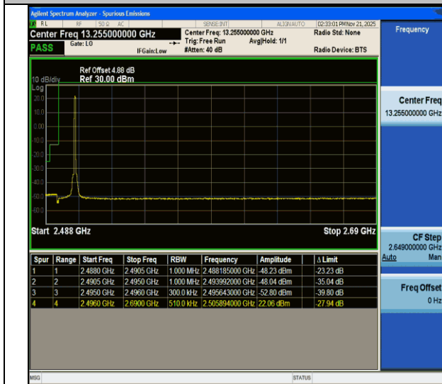
CA_41C-10MHz-20MHz-QPSK@QPSK-QPSK@QPSK-39705-39849-1RB#49@50RB#0-0RB#0@100RB#0-PASS
