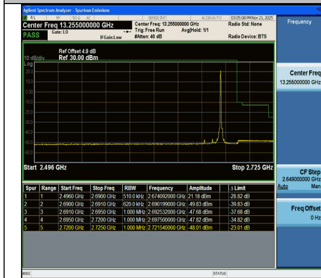
CA_41C-15MHz-15MHz-QPSK@QPSK-QPSK@QPSK-41365-41515-1RB#74@75RB#0-0RB#0@75RB#0-PASS
