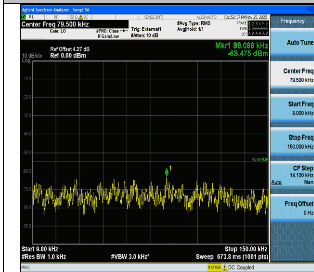
CA_41C-20MHz-20MHz-QPSK-QPSK-41292-41490-1RB#0- ORB#0-0.009~0.15MHz-PASS
