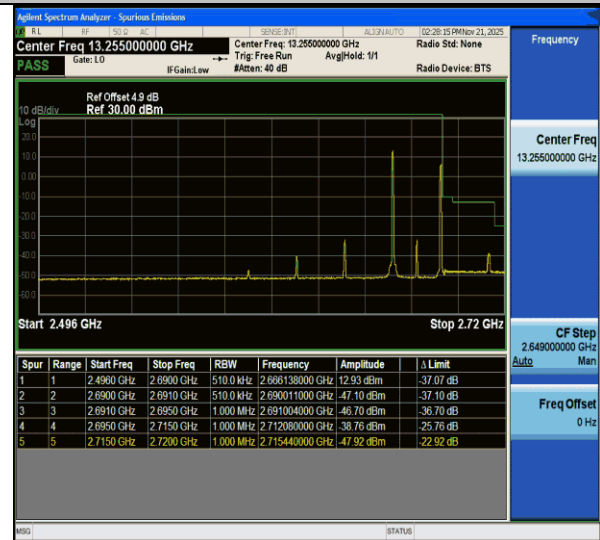
CA_41C-10MHz-15MHz-QPSK@QPSK-QPSK@QPSK-41395-41515-1RB#0@50RB#0-1RB#74@75RB#0-PASS
