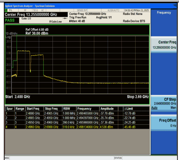
CA_41C-20MHz-20MHz-QPSK@QPSK-QPSK@QPSK-39750-39948-100RB#0@100RB#0-100RB#0@100RB#0-PASS
