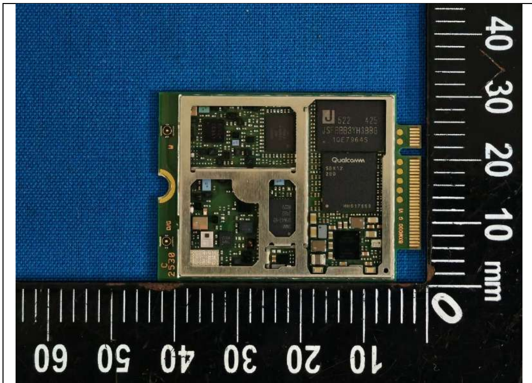
LTE Chip
