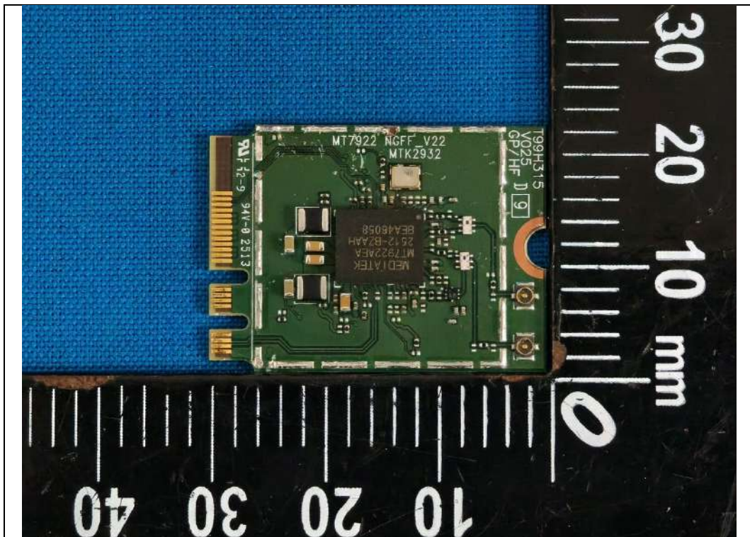
Wifi Chip
