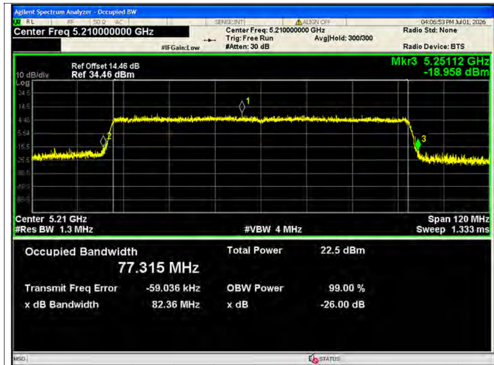
-26dB Bandwidth NVNT ax80 5210MHz Ant1 SISO
