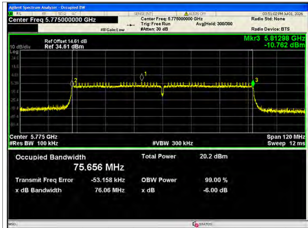
-6dB Bandwidth NVNT ac80 5775MHz Ant1 SISO
