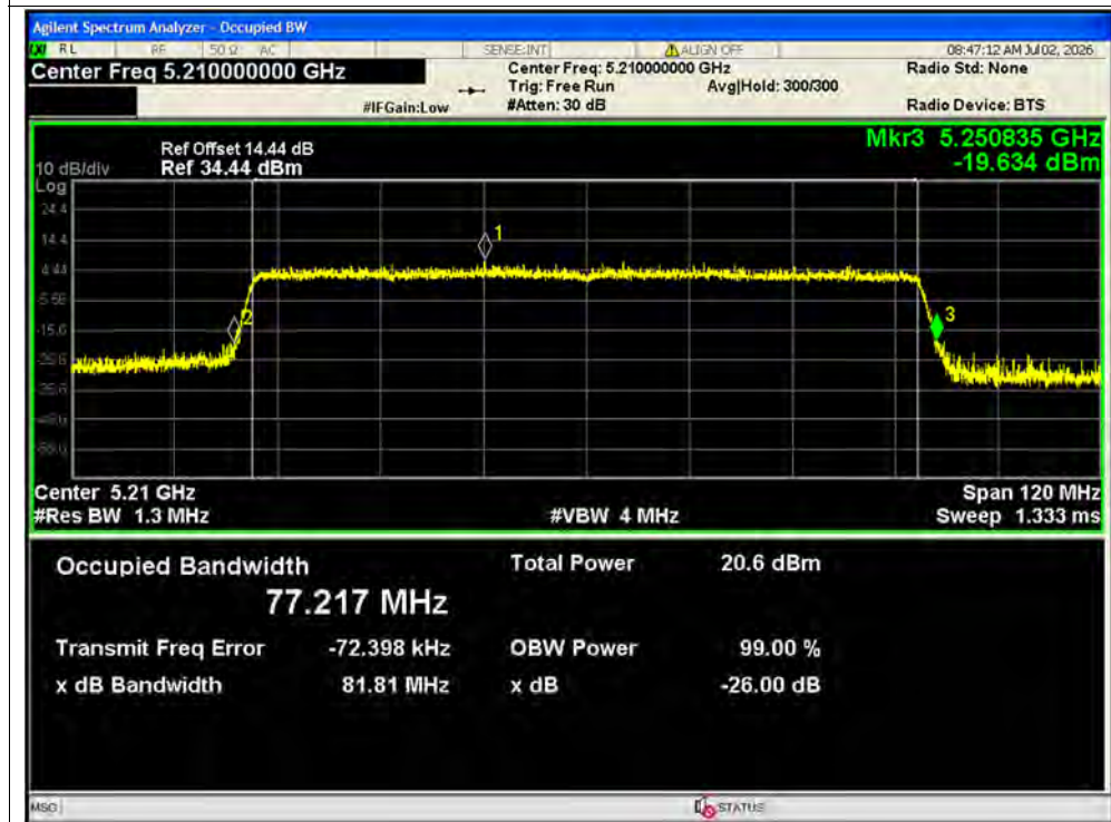
-26dB Bandwidth NVNT ax80 5210MHz Ant2 SISO
