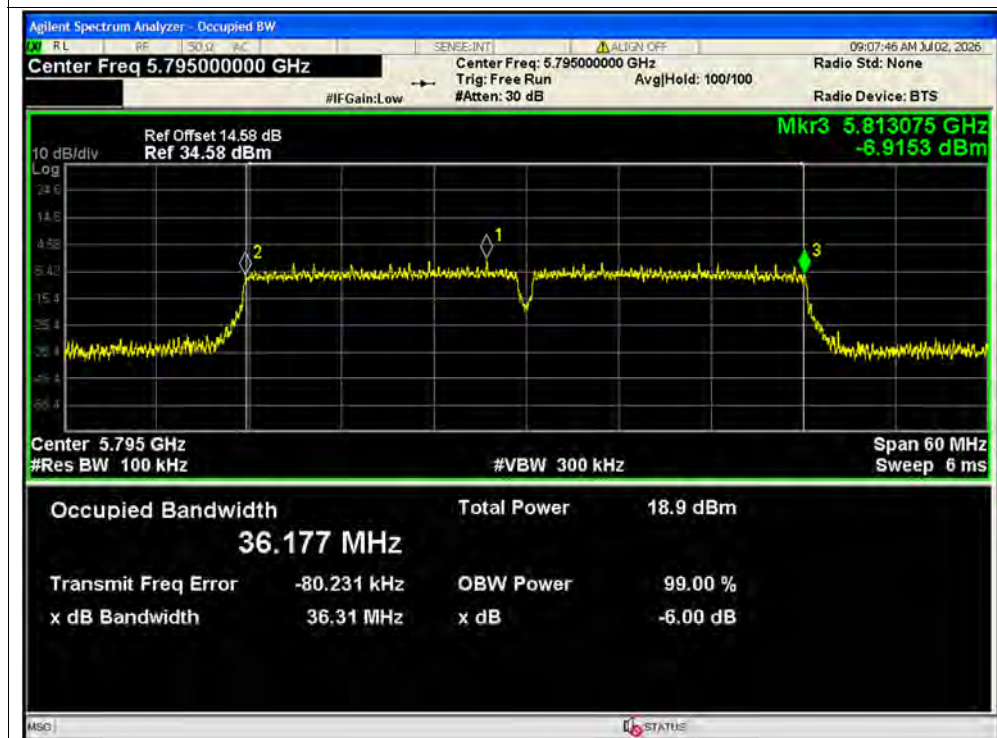
-6dB Bandwidth NVNT n40 5795MHz Ant2 MIMO
