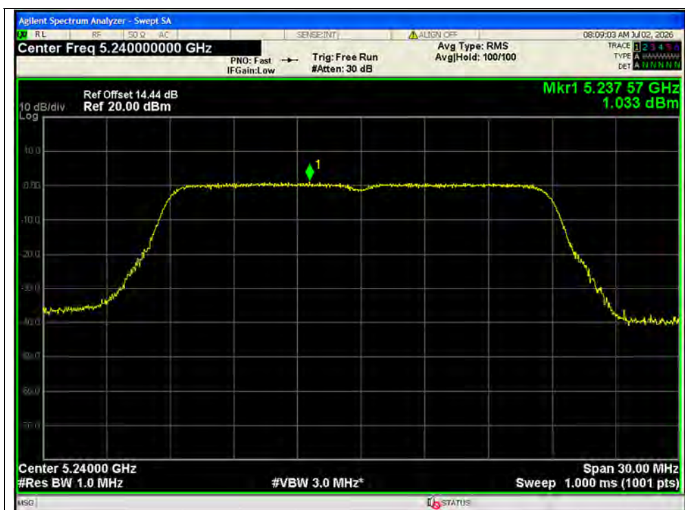
PSD NVNT n20 5240MHz Ant2 SISO
