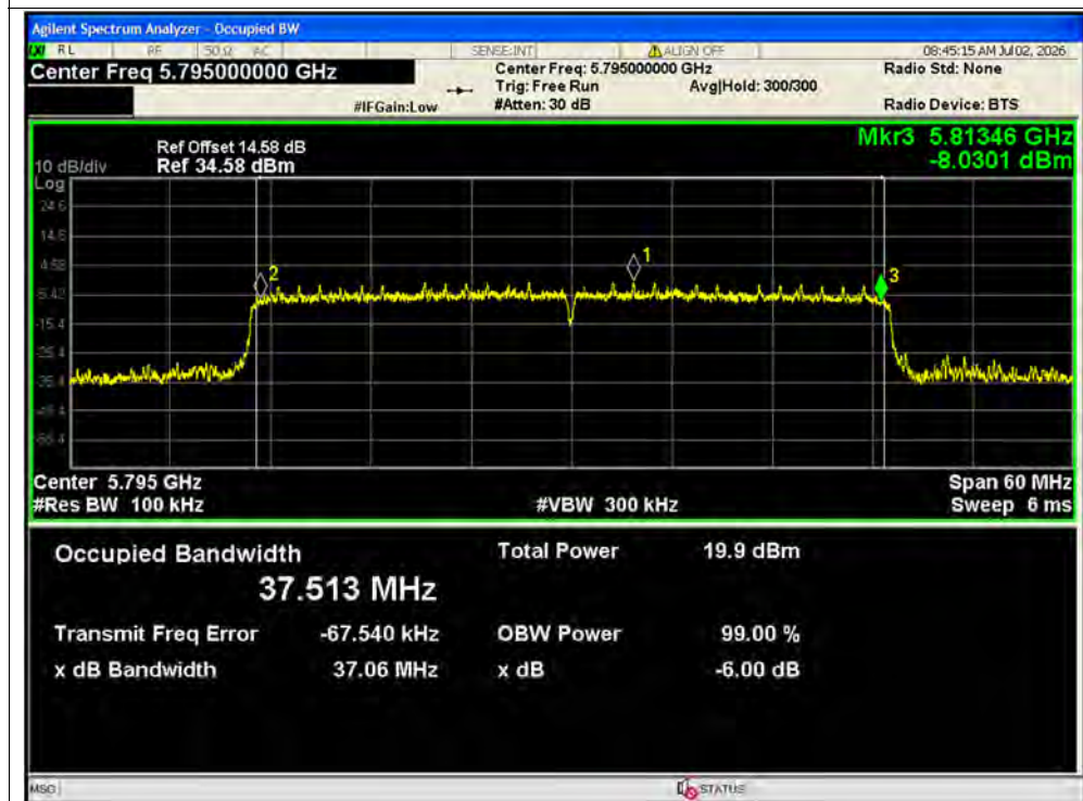
-6dB Bandwidth NVNT ax40 5795MHz Ant2 SISO
