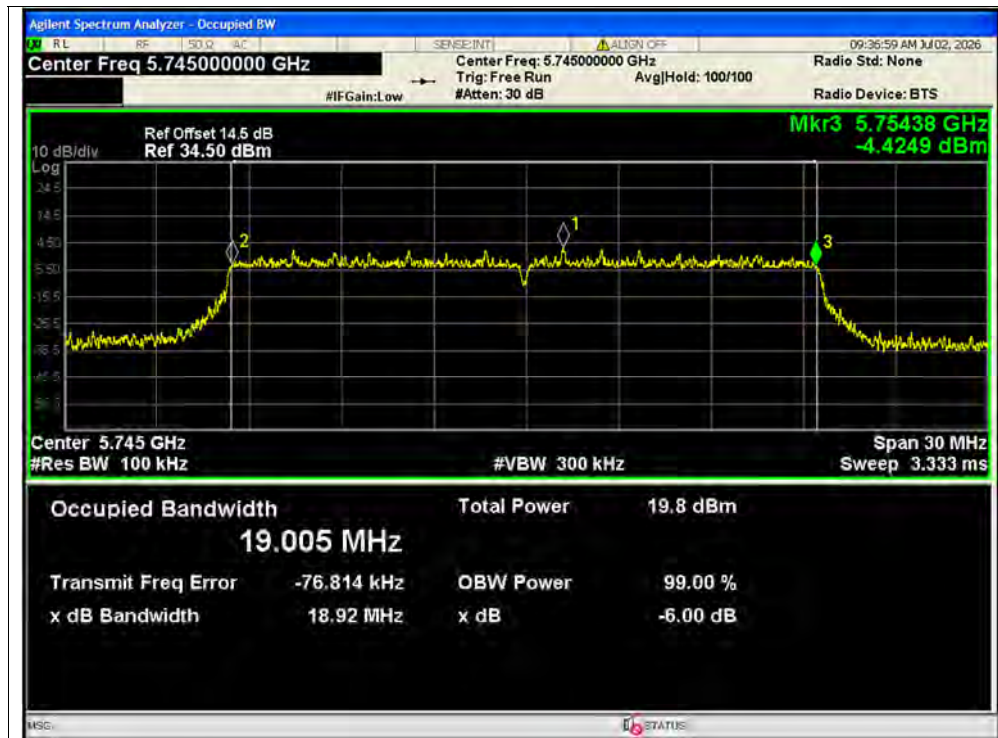
-6dB Bandwidth NVNT ax20 5745MHz Ant1 MIMO
