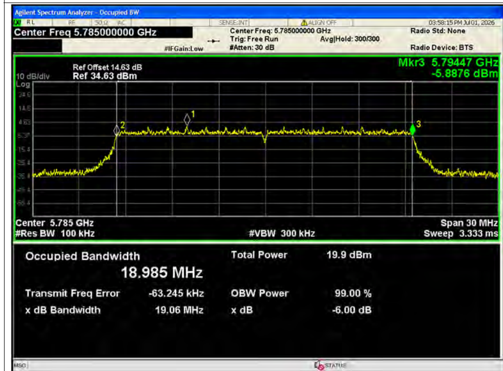
-6dB Bandwidth NVNT ax20 5785MHz Ant1 SISO
