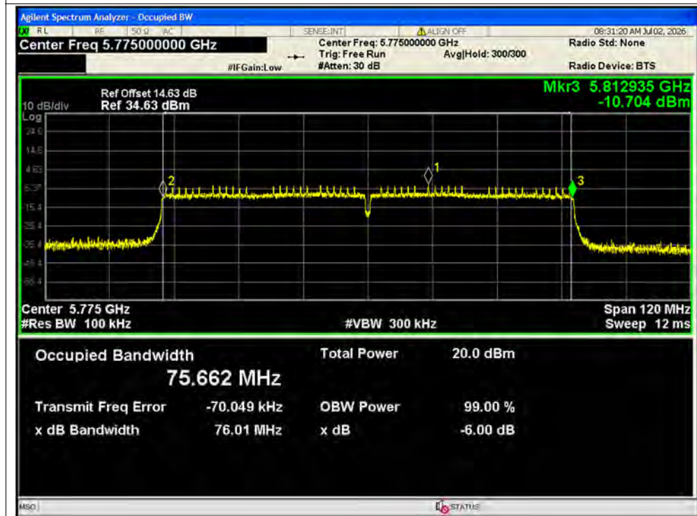
-6dB Bandwidth NVNT ac80 5775MHz Ant2 SISO
