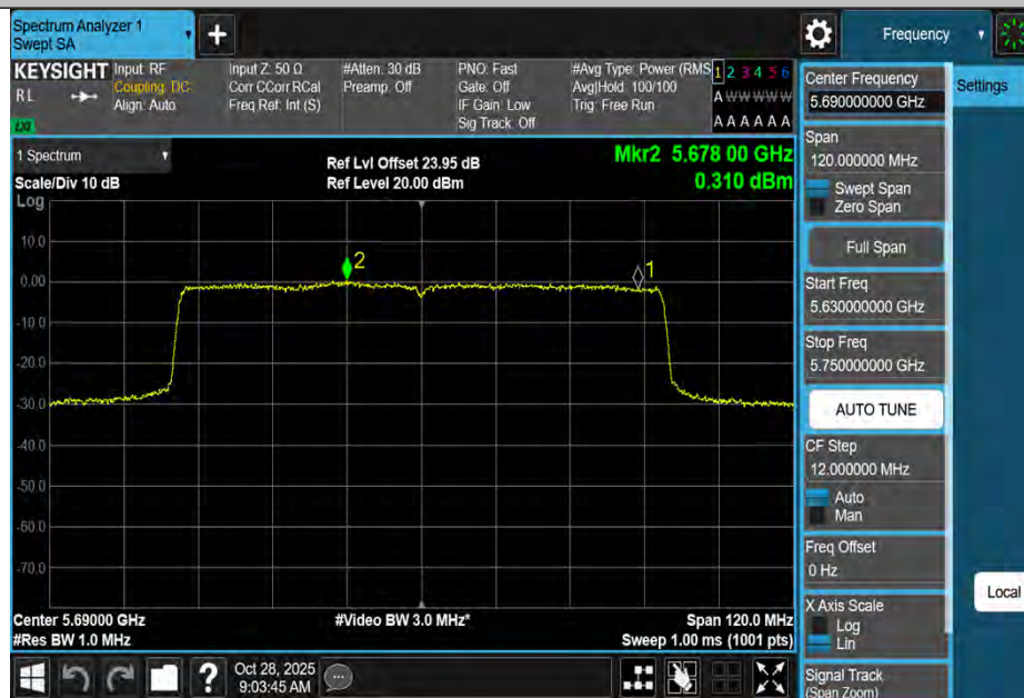
11AC80MIMO-Ant2-5690_UNII-2C-PASS
