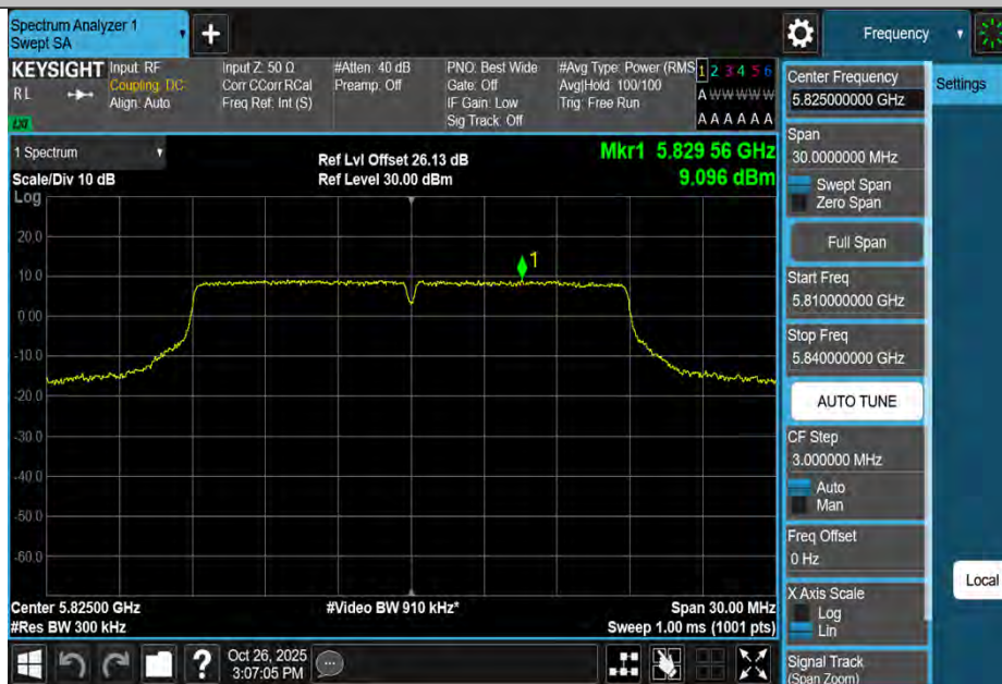
11AC20MIMO-Ant2-5825-PASS
