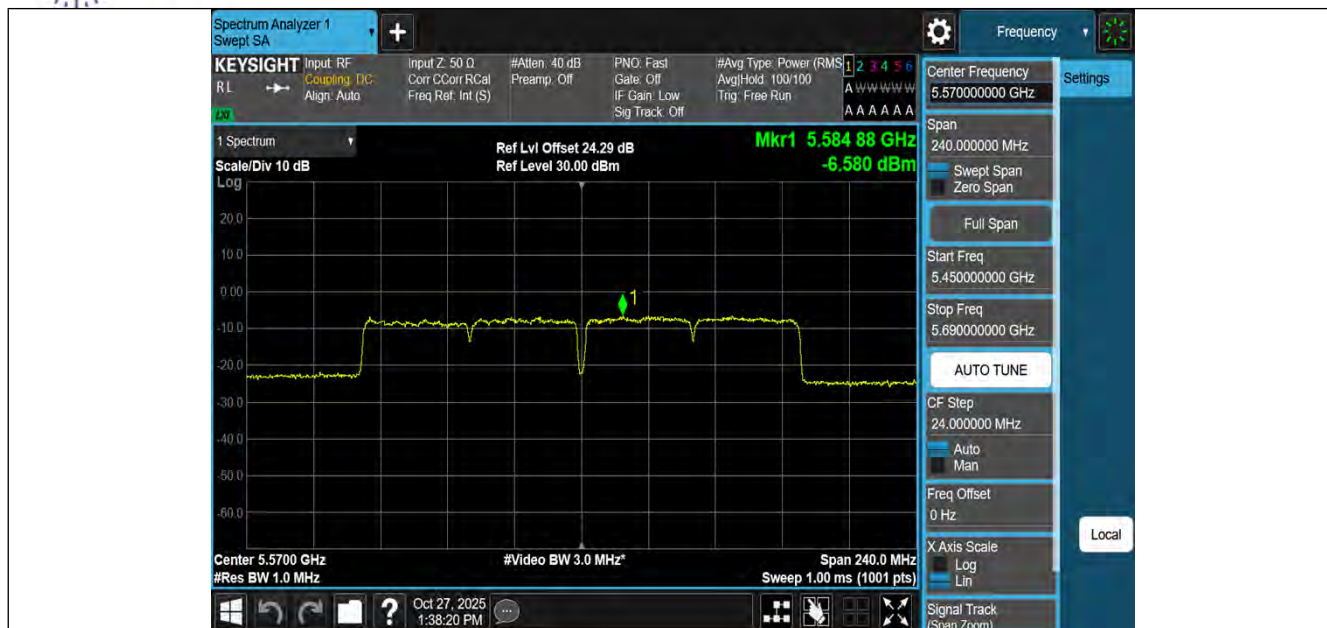
11AC160MIMO-Ant3-5570-PASS
