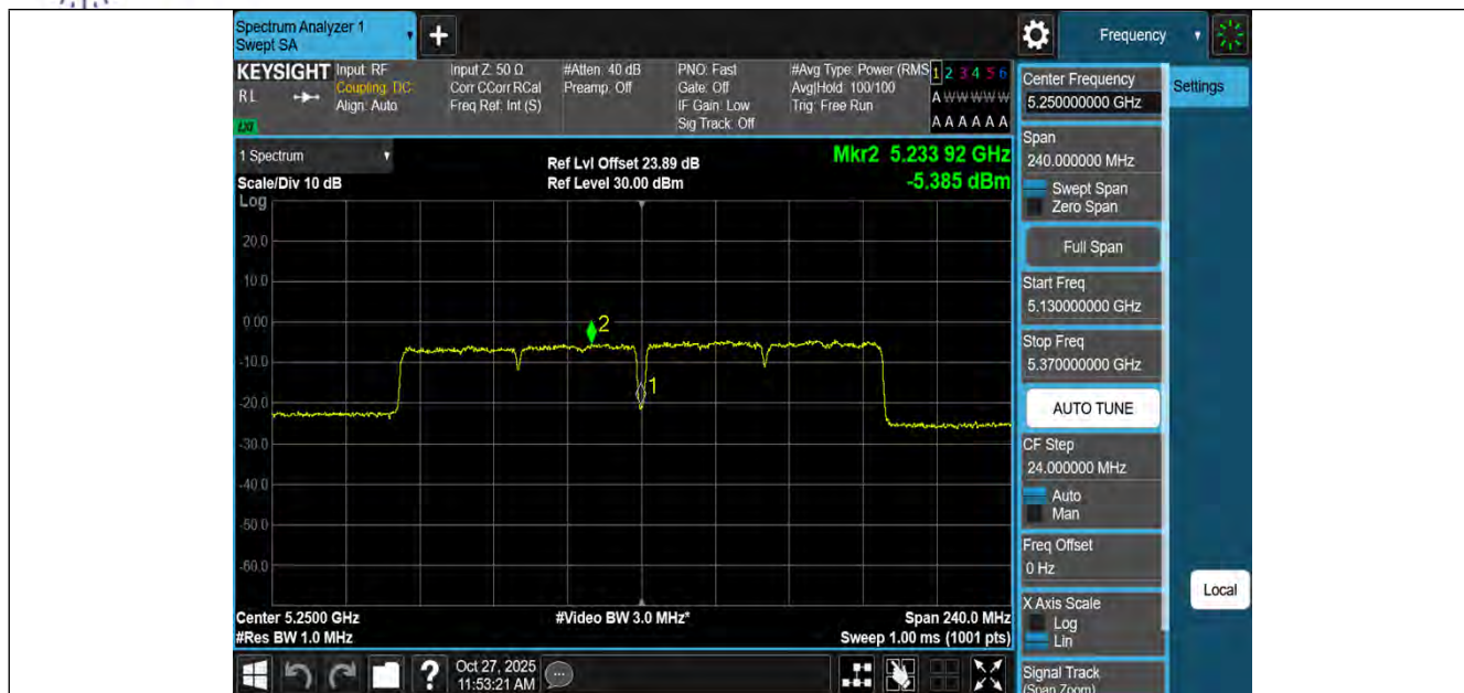
11AC160MIMO-Ant3-5250_UNII-1-PASS
