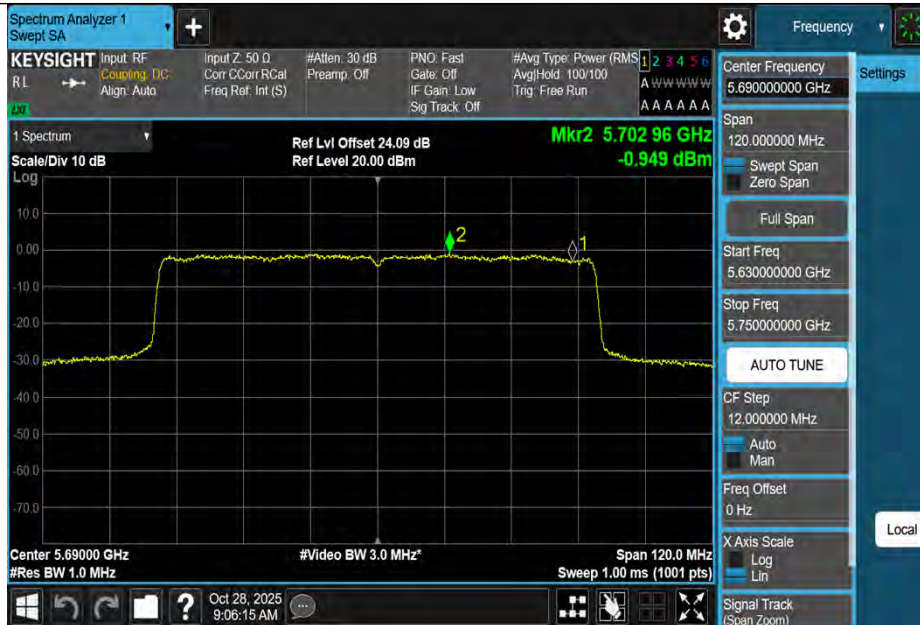
11AC80MIMO-Ant3-5690_UNII-2C-PASS
