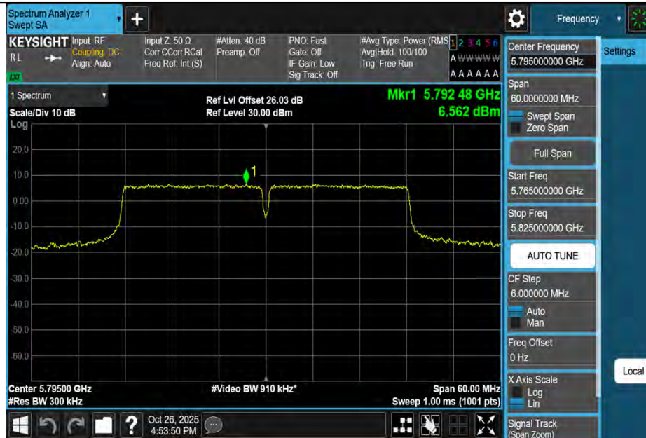
11AC40MIMO-Ant1-5795-PASS
