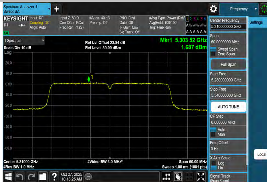
11AC40MIMO-Ant2-5310-PASS
