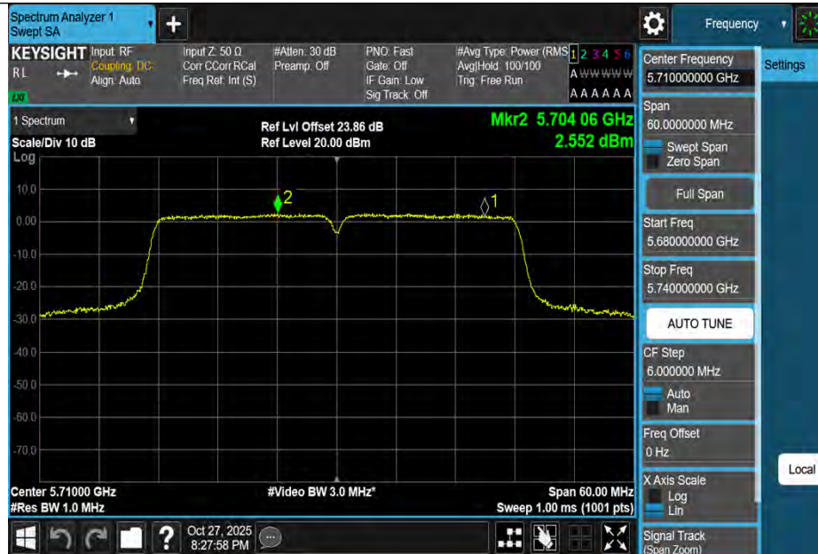
11AC40MIMO-Ant3-5710_UNII-2C-PASS
