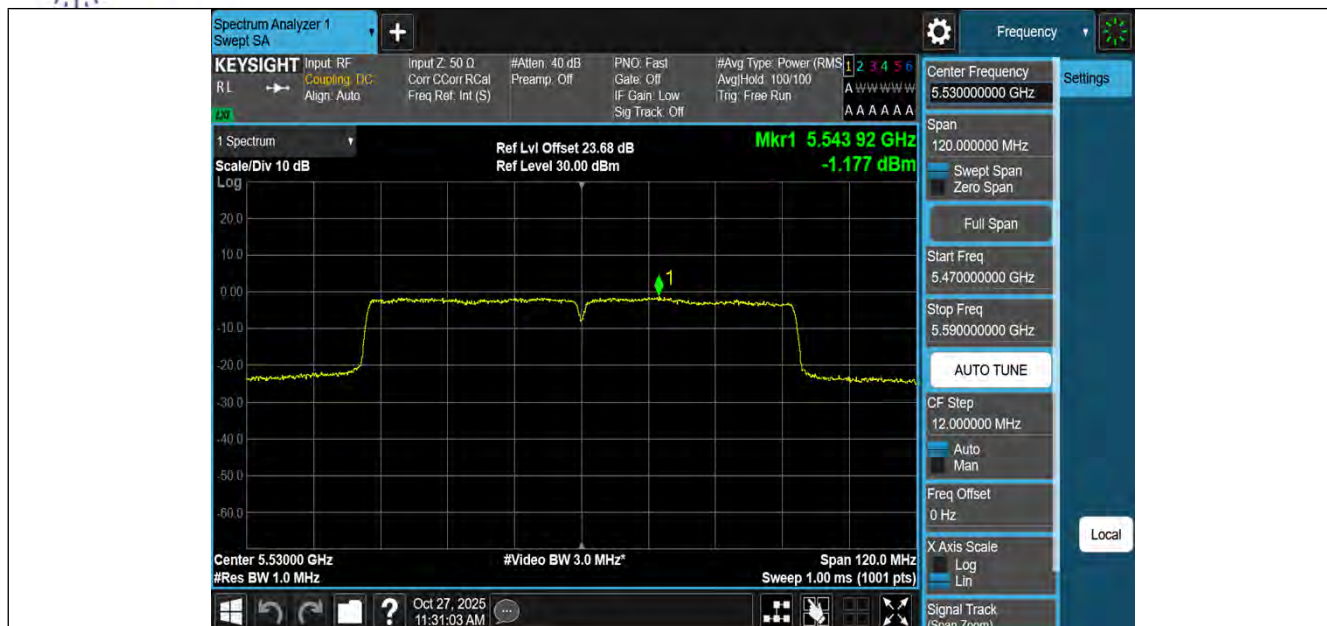
11AC80MIMO-Ant1-5530-PASS
