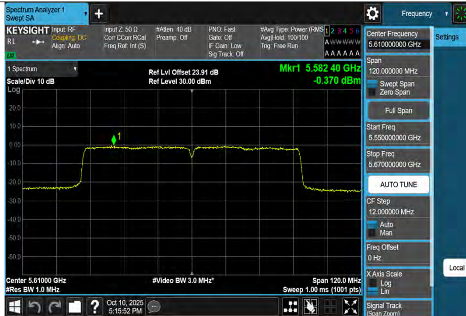
11AC80MIMO-Ant1-5610-PASS
