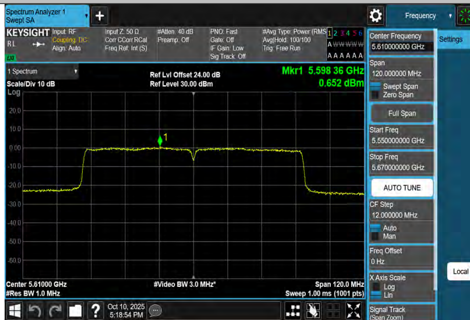
11AC80MIMO-Ant4-5610-PASS
