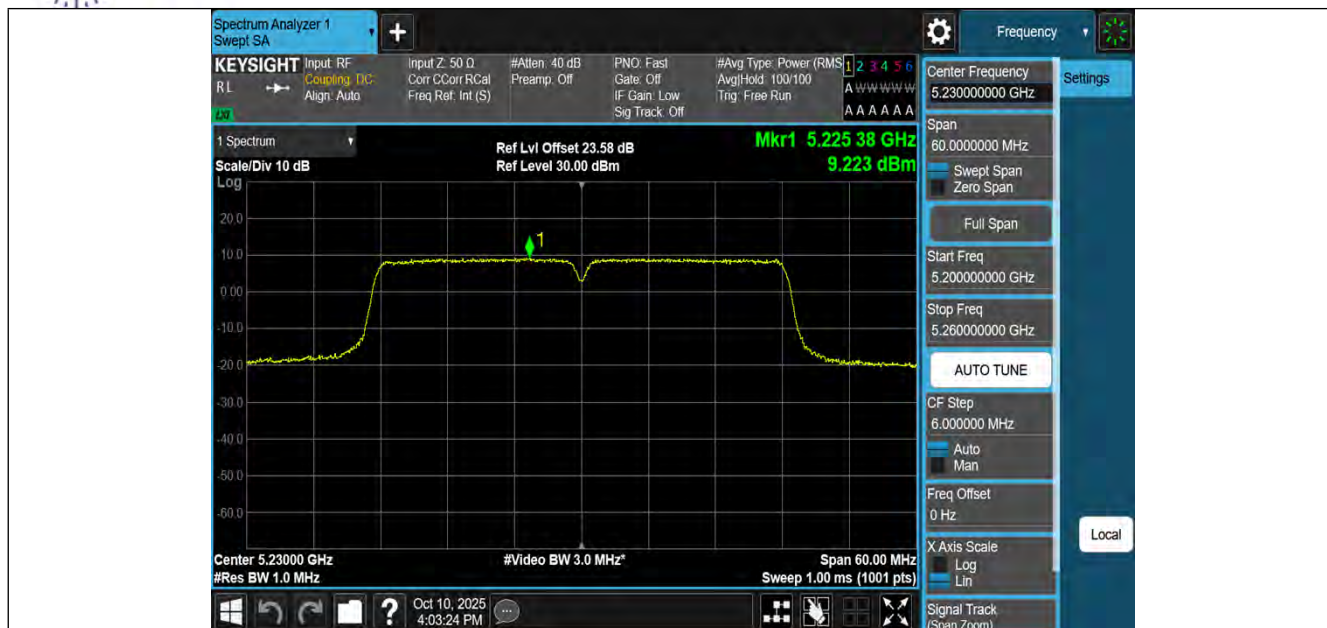
11AC40MIMO-Ant1-5230-PASS
