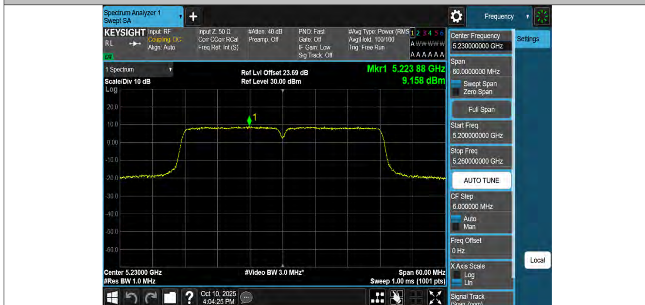
11AC40MIMO-Ant2-5230-PASS
