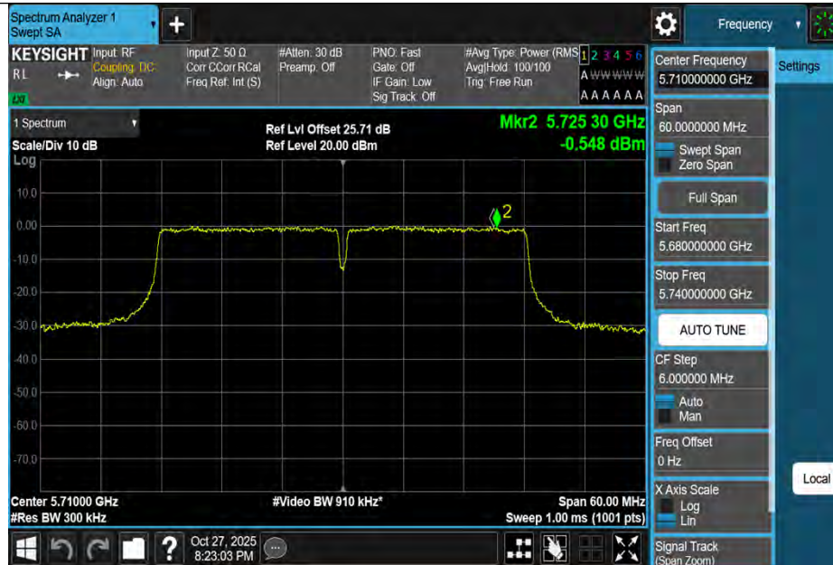
11AC40MIMO-Ant1-5710_UNII-3-PASS
