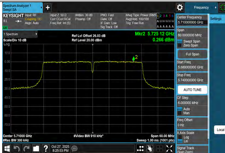
11AC40MIMO-Ant2-5710_UNII-3-PASS
