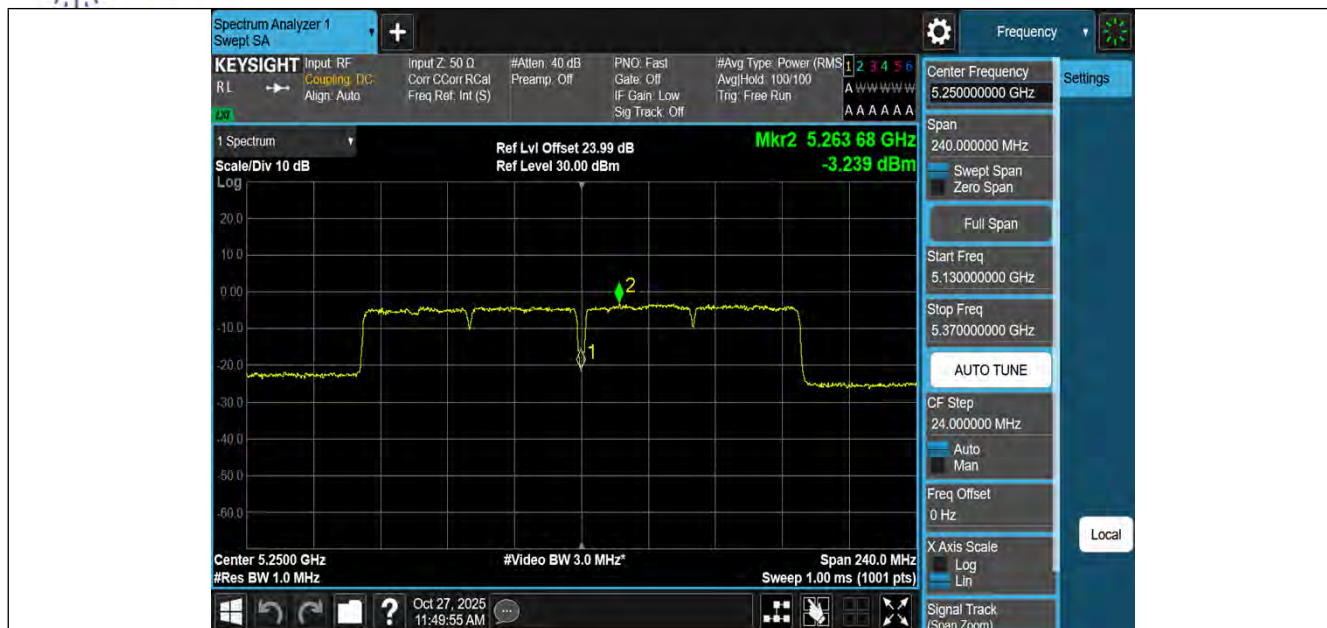
11AC160MIMO-Ant1-5250_UNII-2A-PASS
