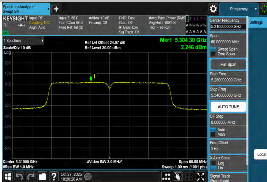
11AC40MIMO-Ant4-5310-PASS
