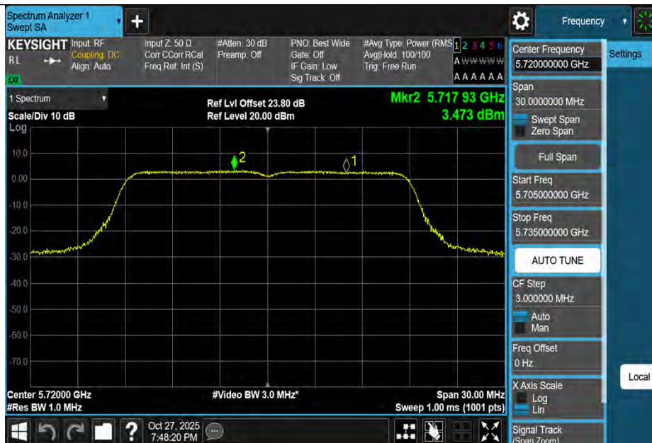
11AC20MIMO-Ant3-5720_UNII-2C-PASS
