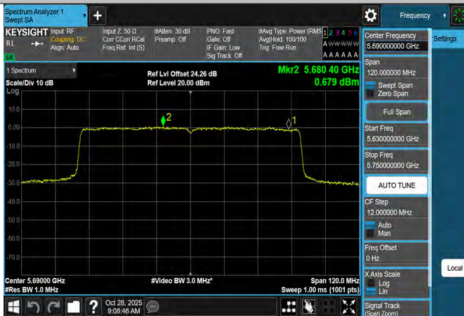
11AC80MIMO-Ant4-5690_UNII-2C-PASS
