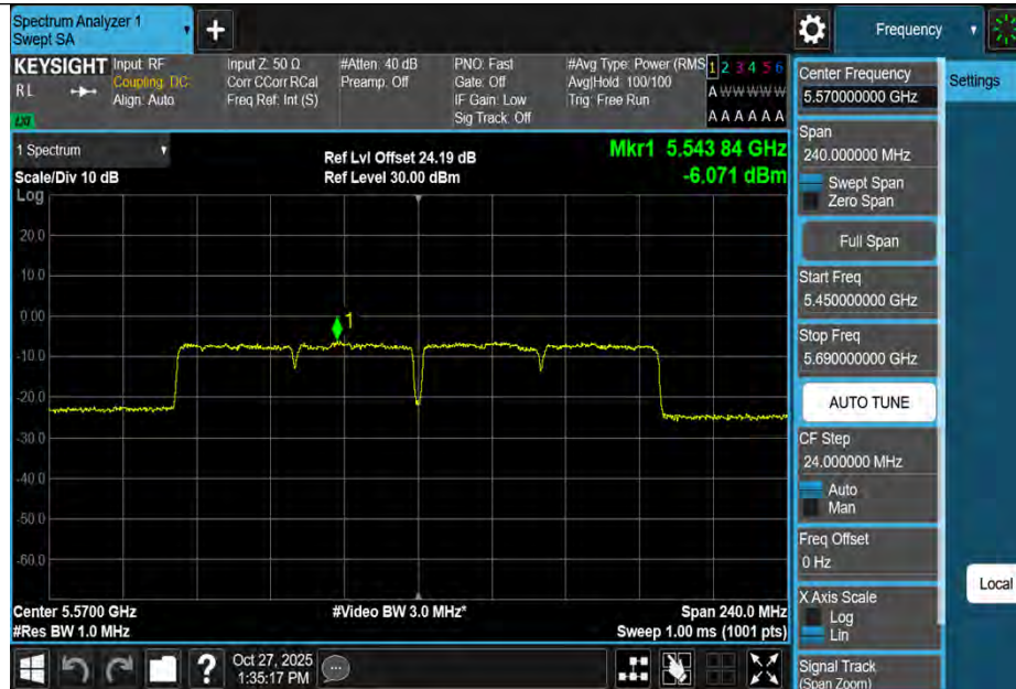
11AC160MIMO-Ant1-5570-PASS
