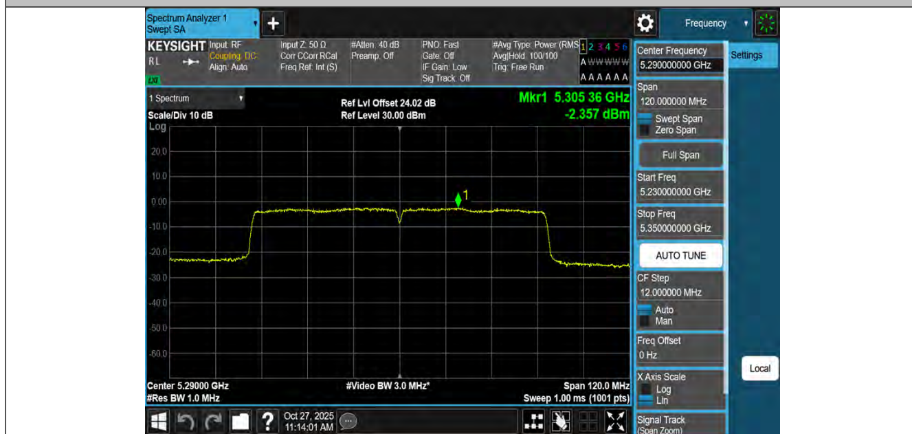
11AC80MIMO-Ant2-5290-PASS
