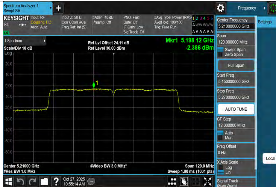
11AC80MIMO-Ant1-5210-PASS
