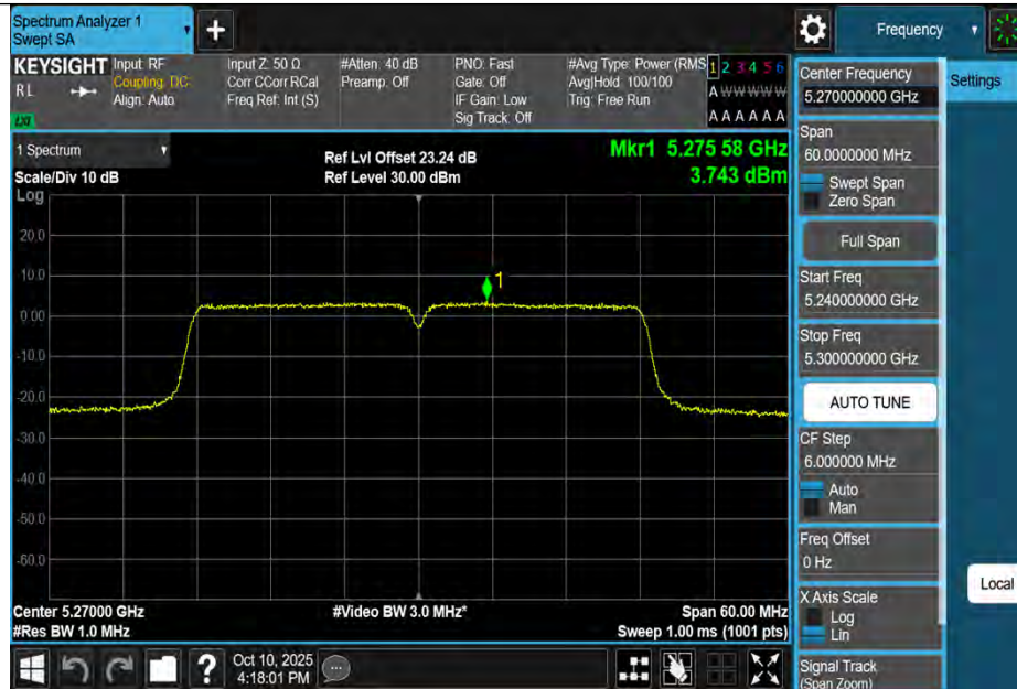
11AC40MIMO-Ant1-5270-PASS
