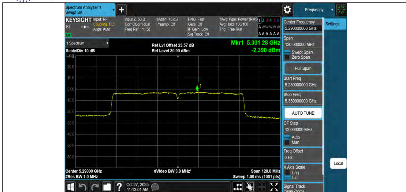
11AC80MIMO-Ant1-5290-PASS
