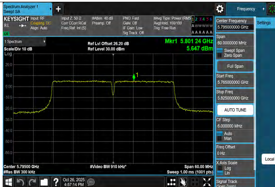
11AC40MIMO-Ant3-5795-PASS
