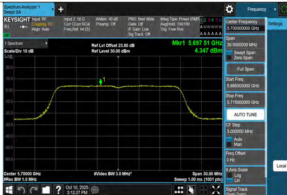
11AC20MIMO-Ant3-5700-PASS
