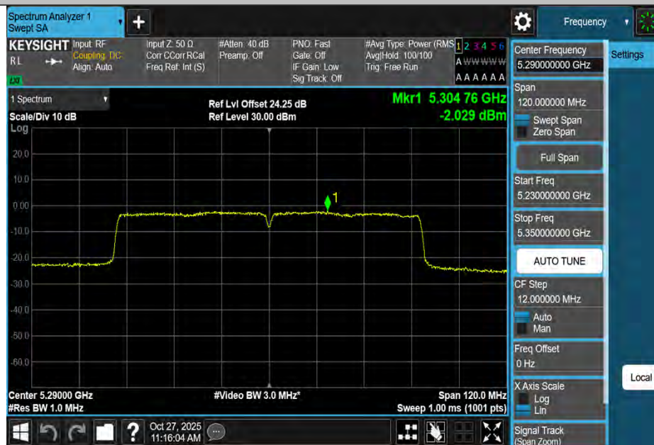
11AC80MIMO-Ant4-5290-PASS
