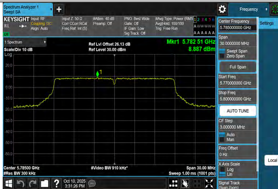
11AC20MIMO-Ant2-5785-PASS
