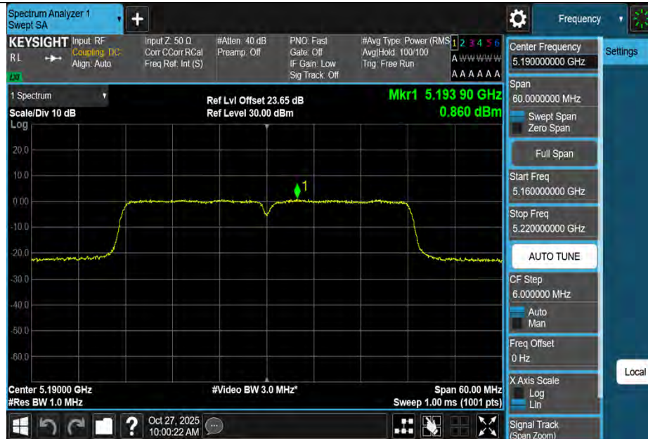
11AC40MIMO-Ant3-5190-PASS
