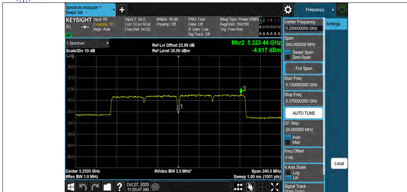
11AC160MIMO-Ant3-5250_UNII-2A-PASS
