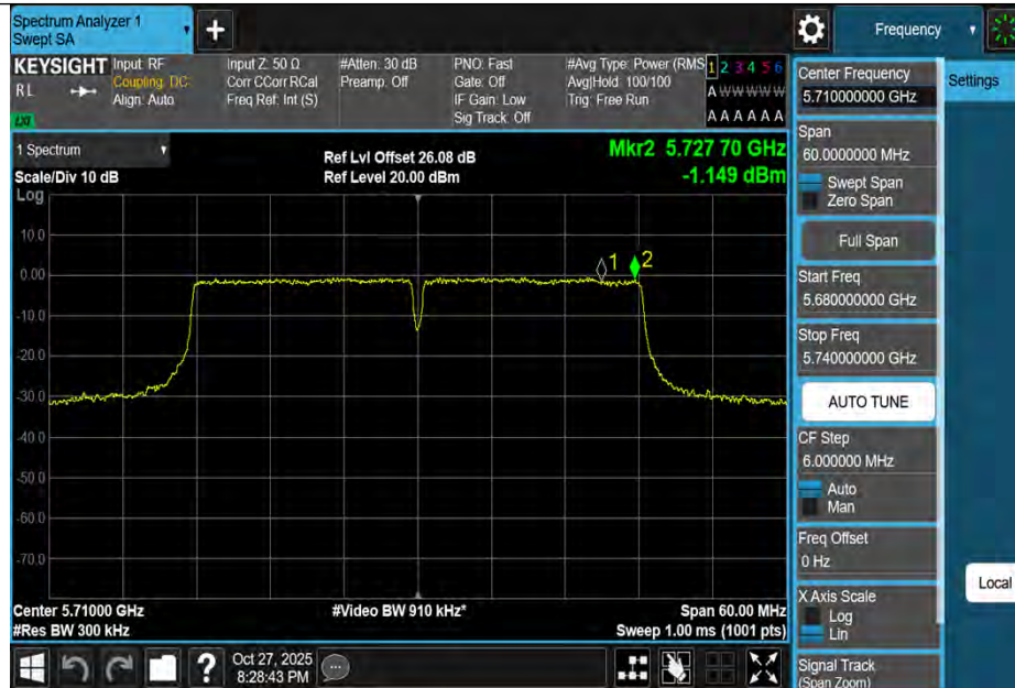
11AC40MIMO-Ant3-5710_UNII-3-PASS
