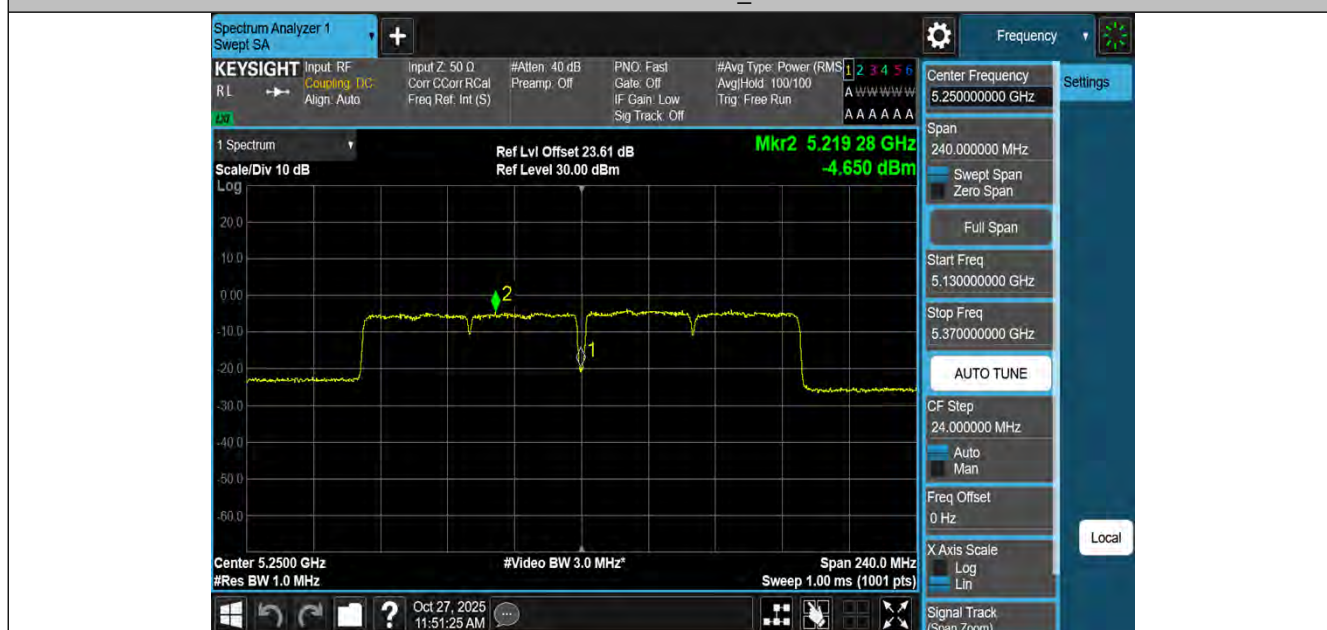
11AC160MIMO-Ant2-5250_UNII-1-PASS
