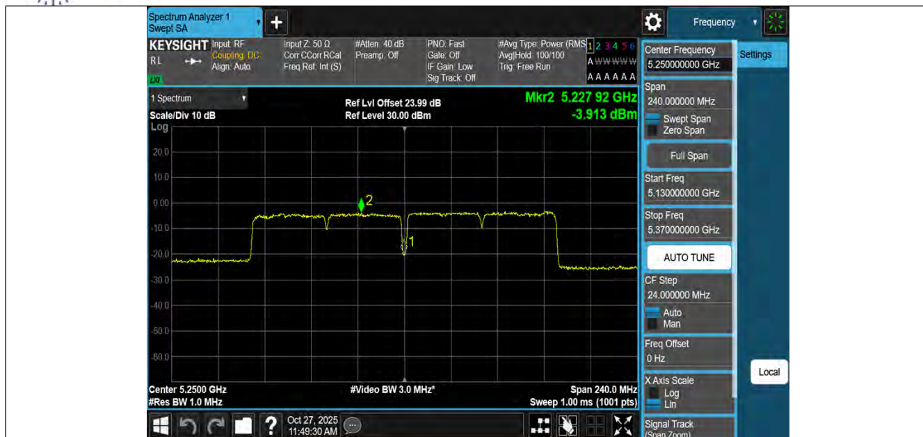
11AC160MIMO-Ant1-5250_UNII-1-PASS
