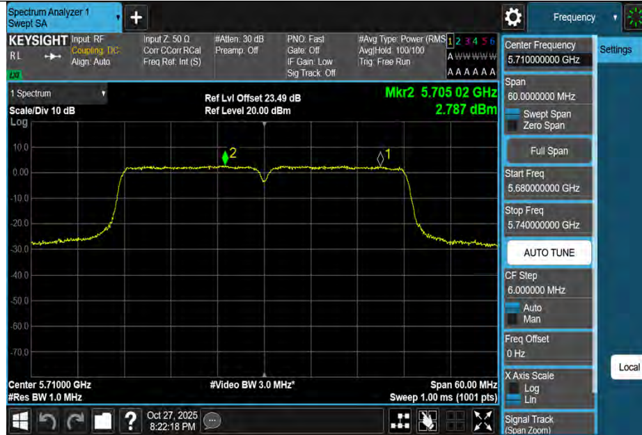
11AC40MIMO-Ant1-5710_UNII-2C-PASS
