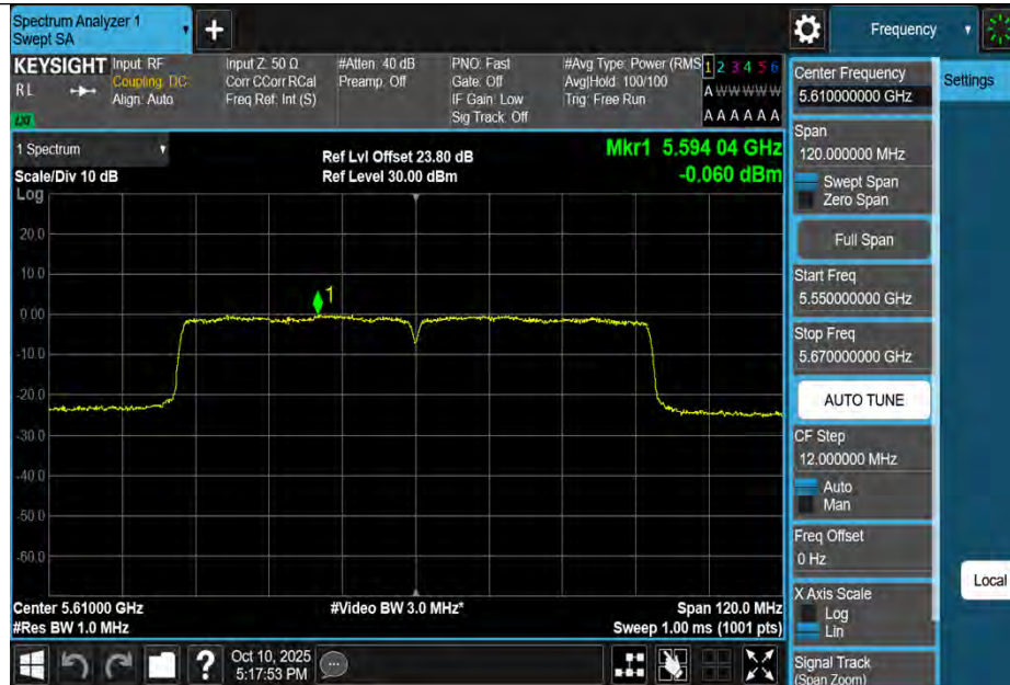
11AC80MIMO-Ant3-5610-PASS
