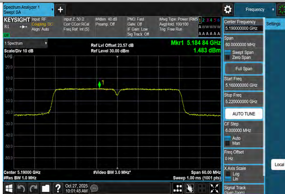
11AC40MIMO-Ant4-5190-PASS
