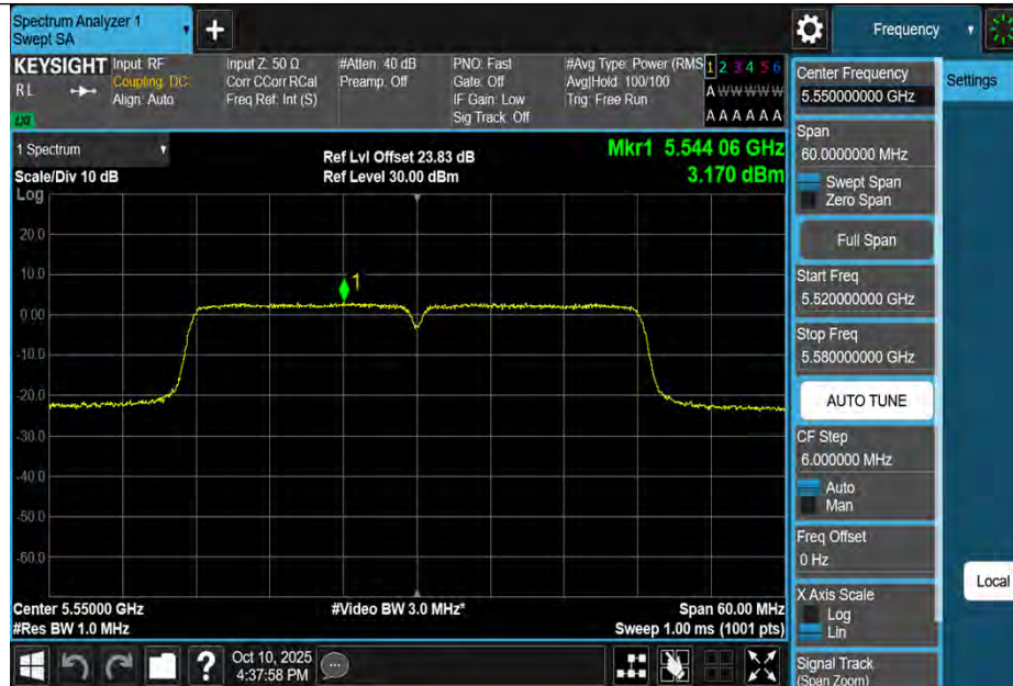
11AC40MIMO-Ant3-5550-PASS
