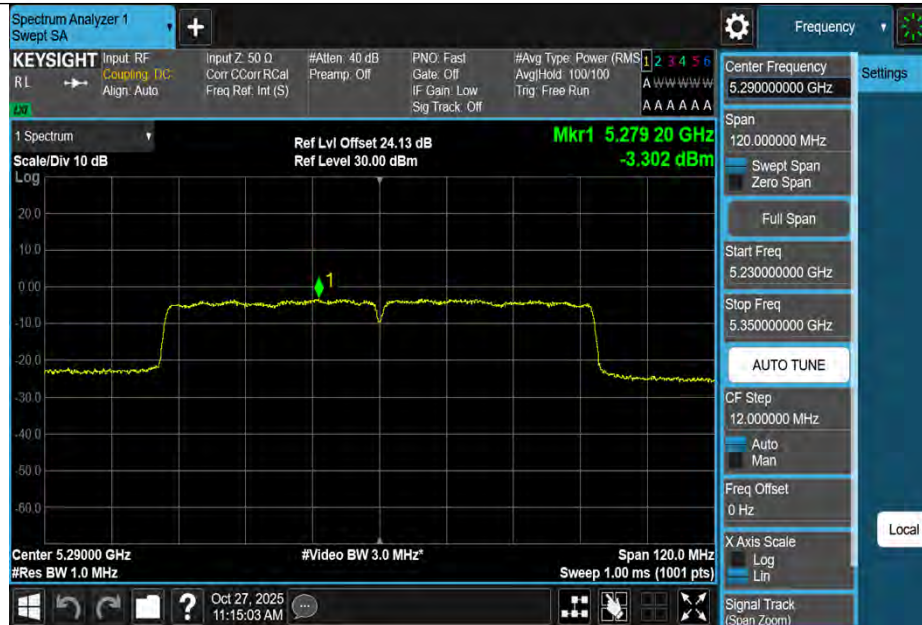
11AC80MIMO-Ant3-5290-PASS
