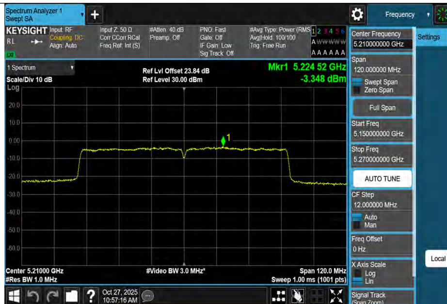
11AC80MIMO-Ant3-5210-PASS
