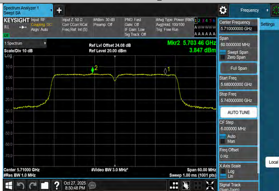
11AC40MIMO-Ant4-5710_UNII-2C-PASS
