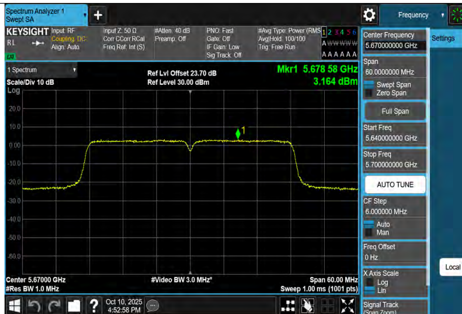
11AC40MIMO-Ant3-5670-PASS
