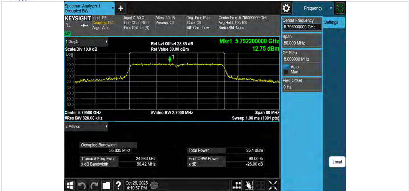
11AC40MIMO-Ant3-5795
