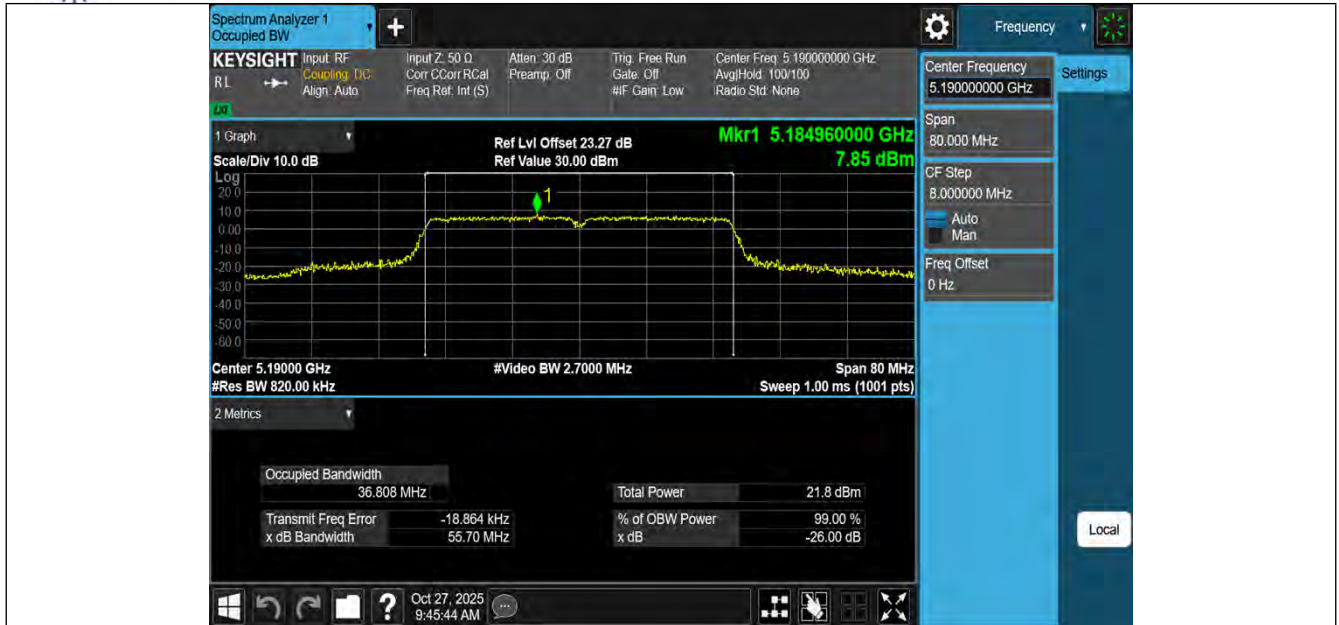
11AC40MIMO-Ant1-5190
