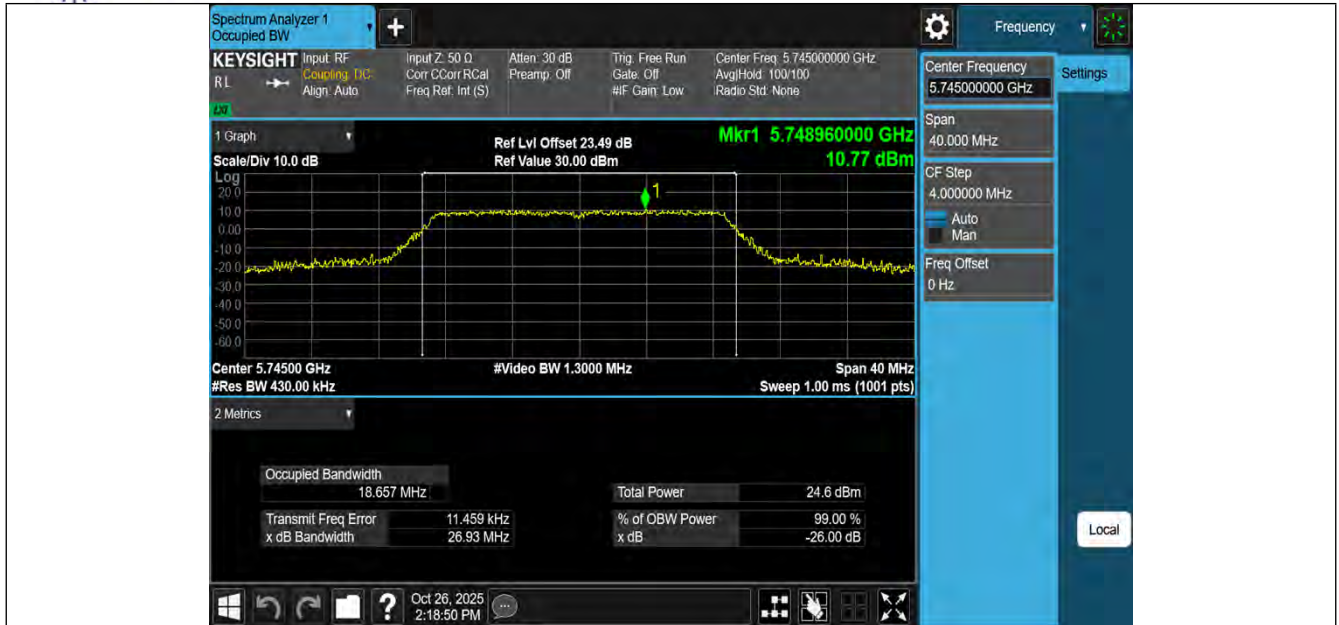
11AC20MIMO-Ant1-5745
