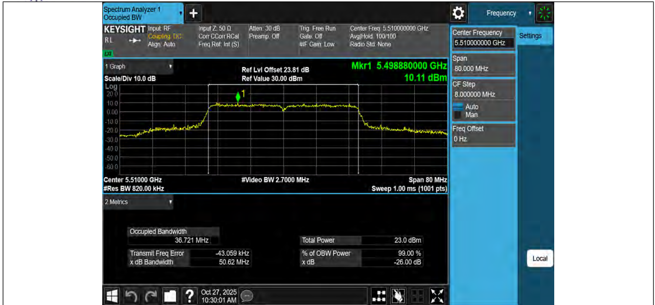
11AC40MIMO-Ant3-5510
