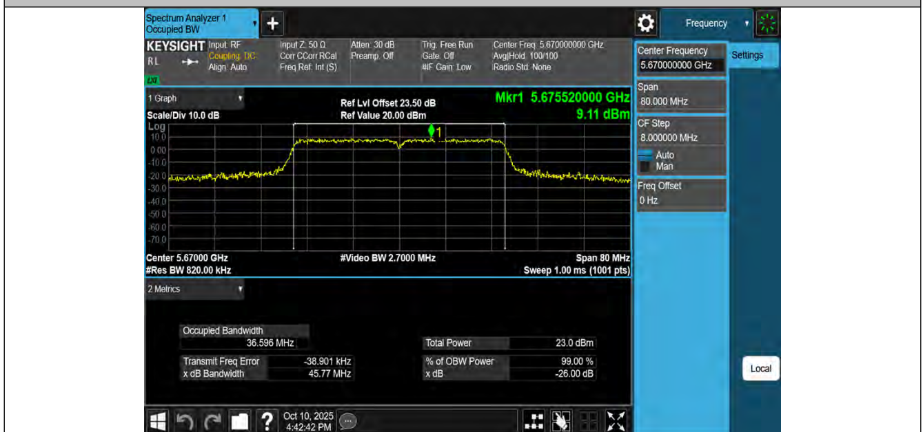
11AC40MIMO-Ant2-5670
