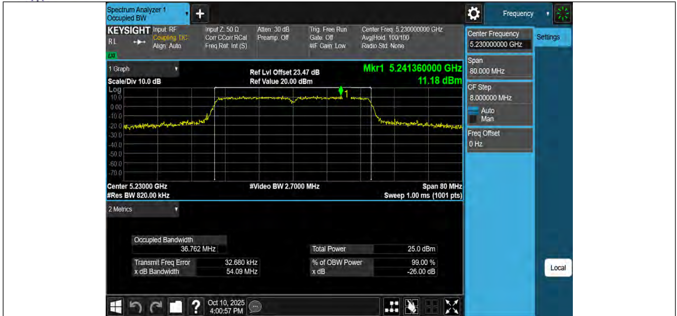
11AC40MIMO-Ant3-5230
