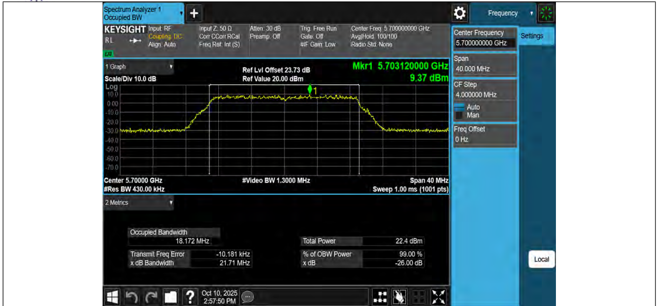
11AC20MIMO-Ant3-5700
