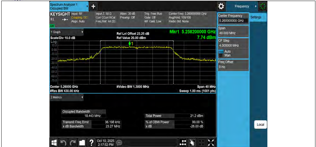
11AC20MIMO-Ant3-5260
