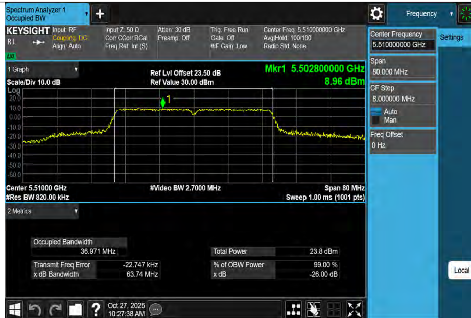
11AC40MIMO-Ant1-5510
