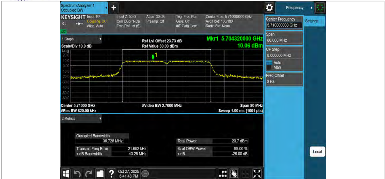
11N40MIMO-Ant3-5710
