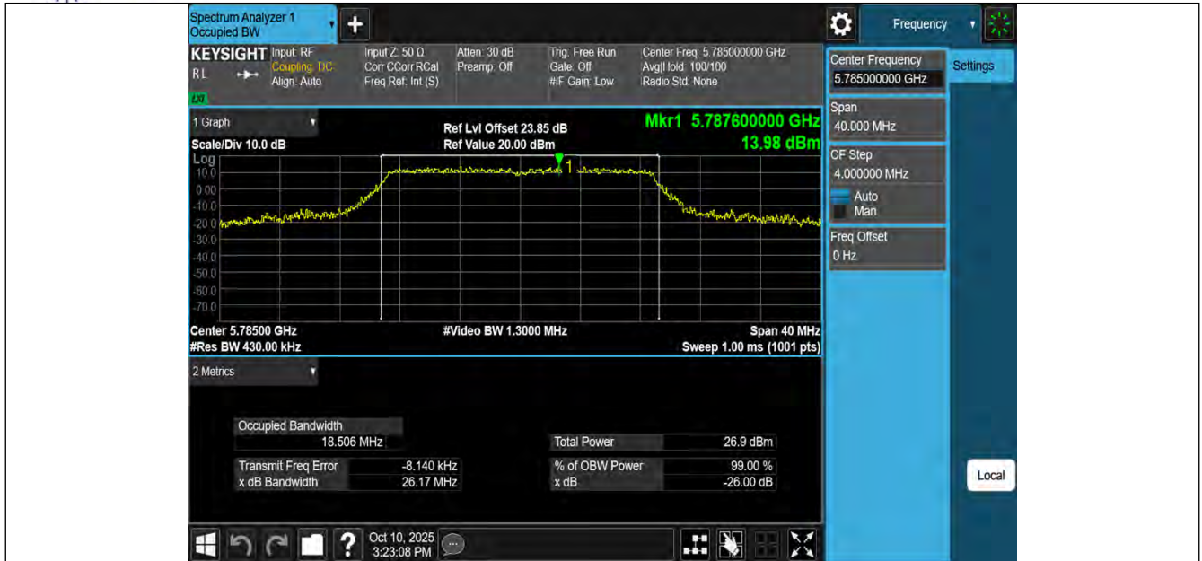
11AC20MIMO-Ant3-5785
