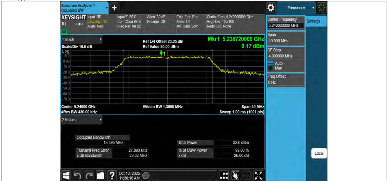
11AC20MIMO-Ant3-5240
