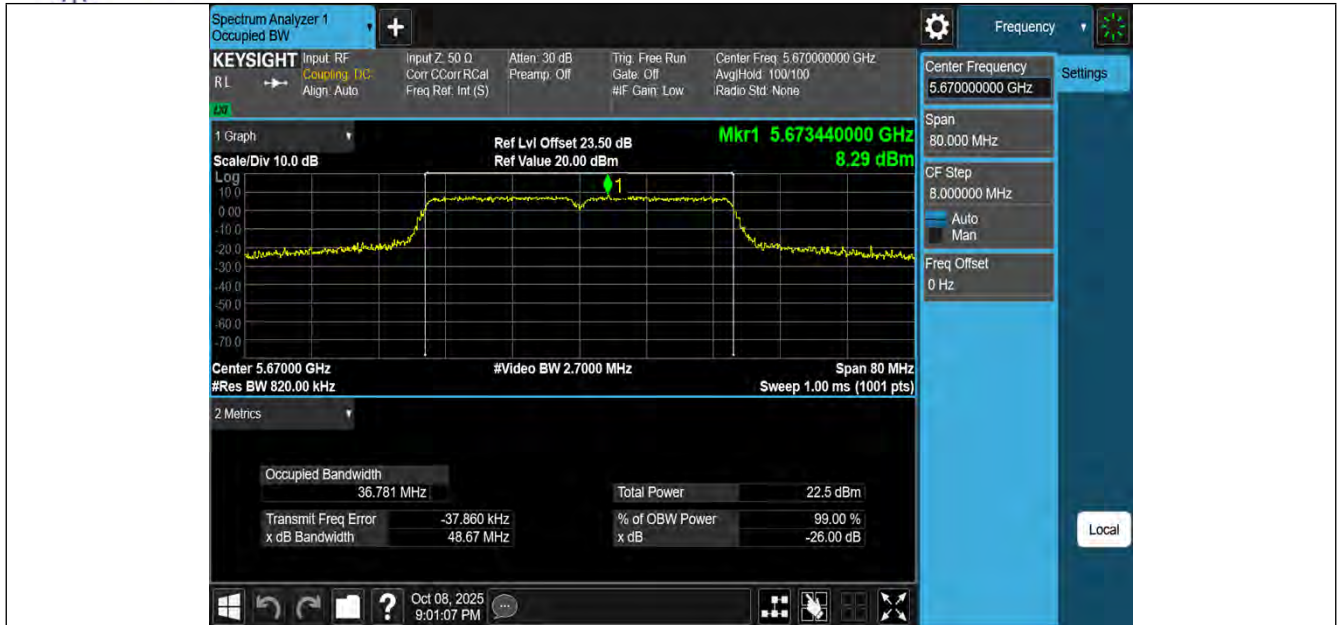
11N40MIMO-Ant1-5670
