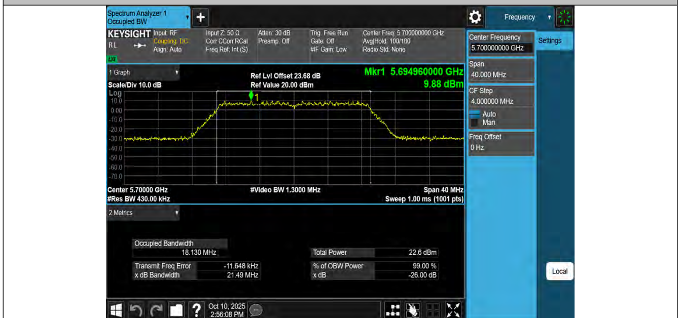
11AC20MIMO-Ant2-5700
