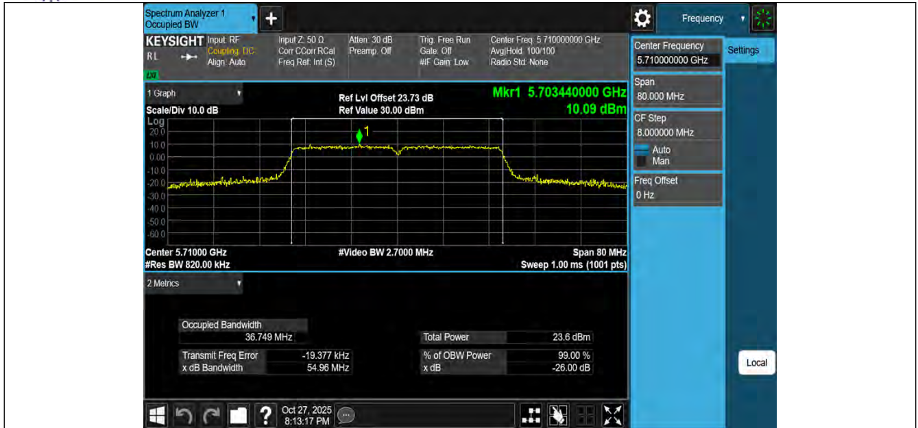
11AC40MIMO-Ant3-5710
