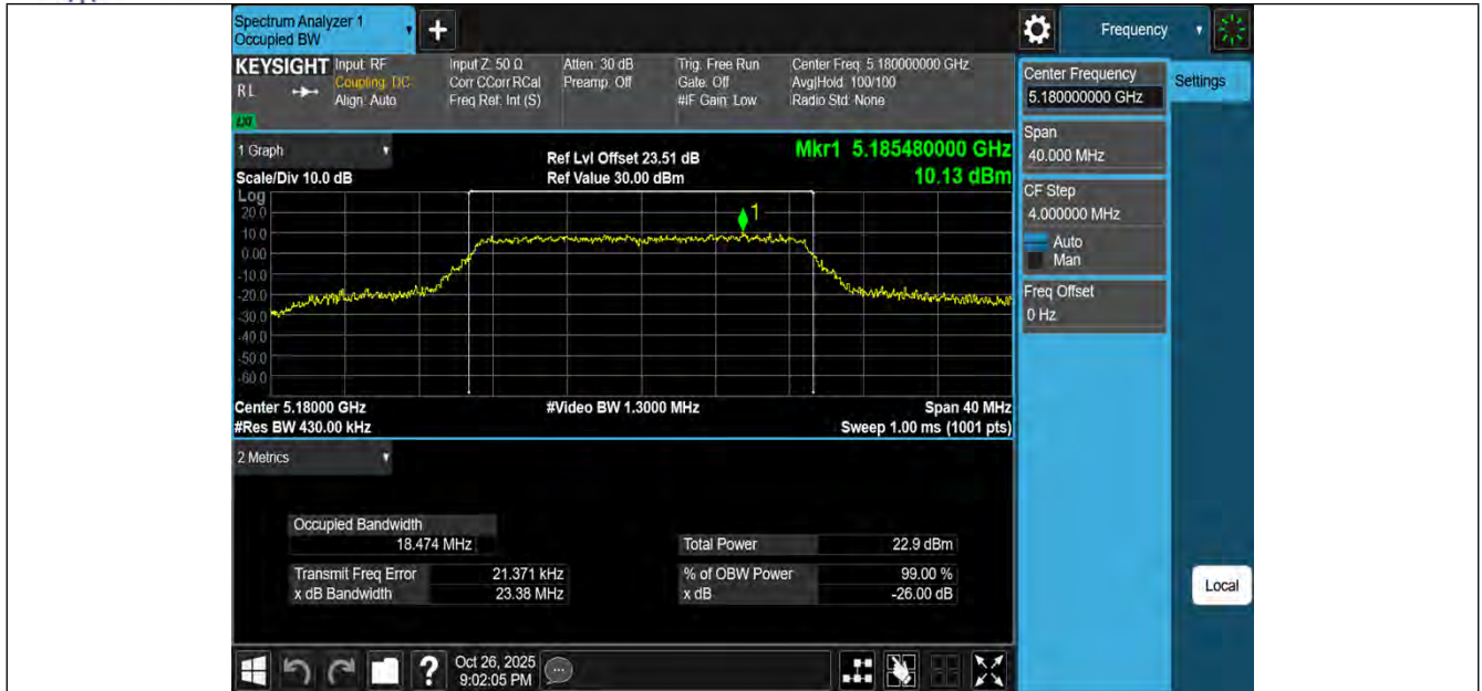
11AC20MIMO-Ant3-5180
