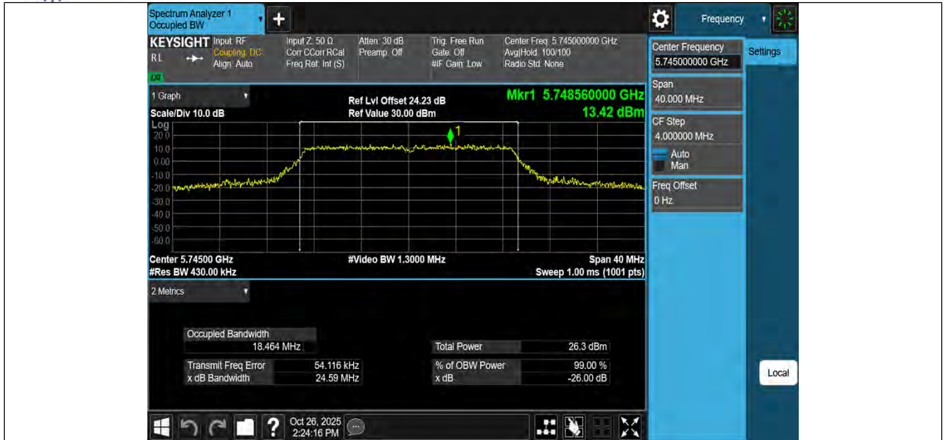
11AC20MIMO-Ant3-5745
