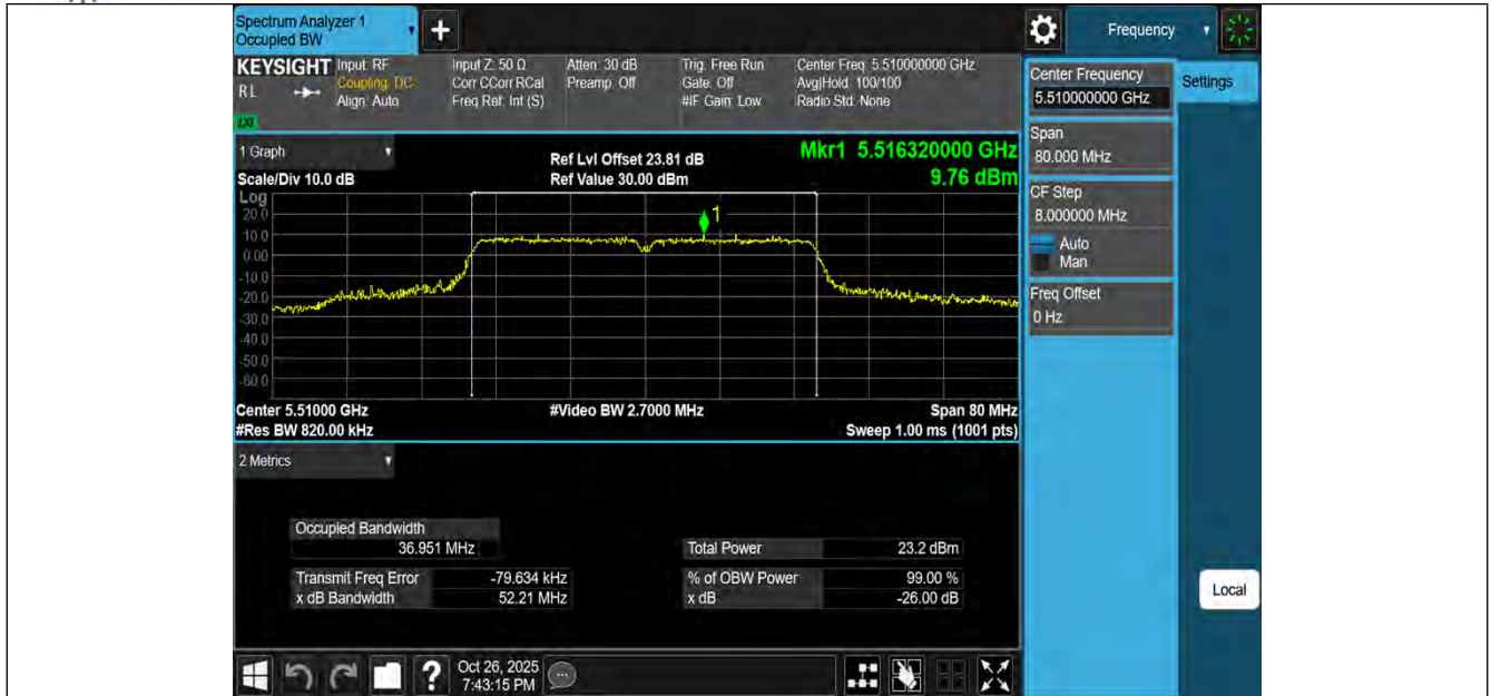
11N40MIMO-Ant3-5510
