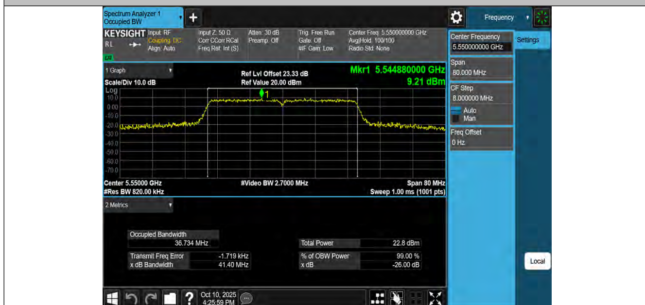
11AC40MIMO-Ant2-5550
