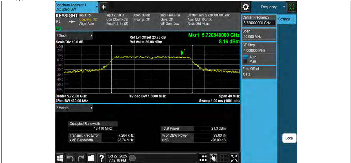
11AC20MIMO-Ant3-5720
