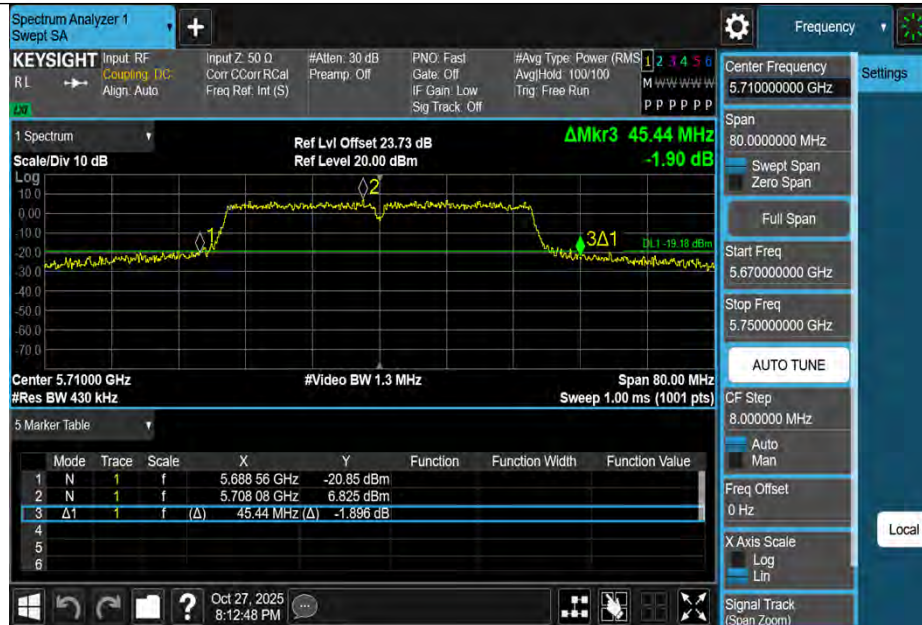
11AC40MIMO-Ant3-5710
