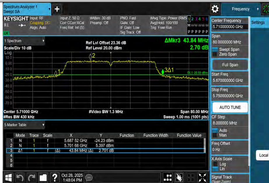
11AC40MIMO-Ant1-5710
