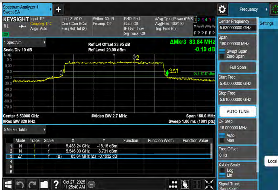
11AC80MIMO-Ant4-5530
