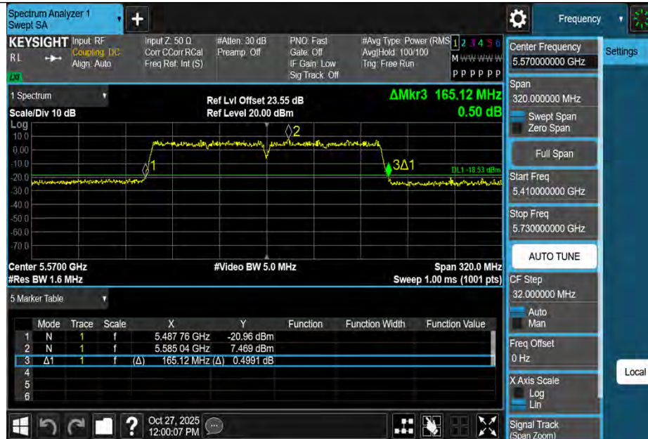
11AC160MIMO-Ant1-5570
