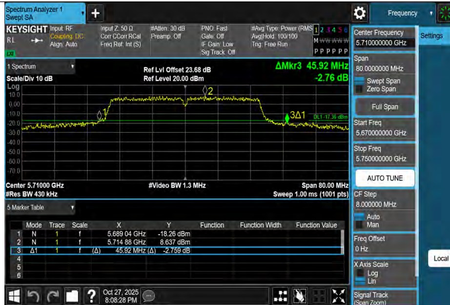
11AC40MIMO-Ant2-5710
