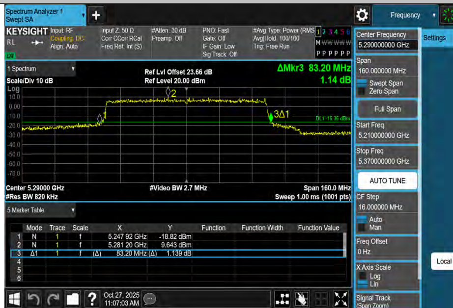
11AC80MIMO-Ant2-5290
