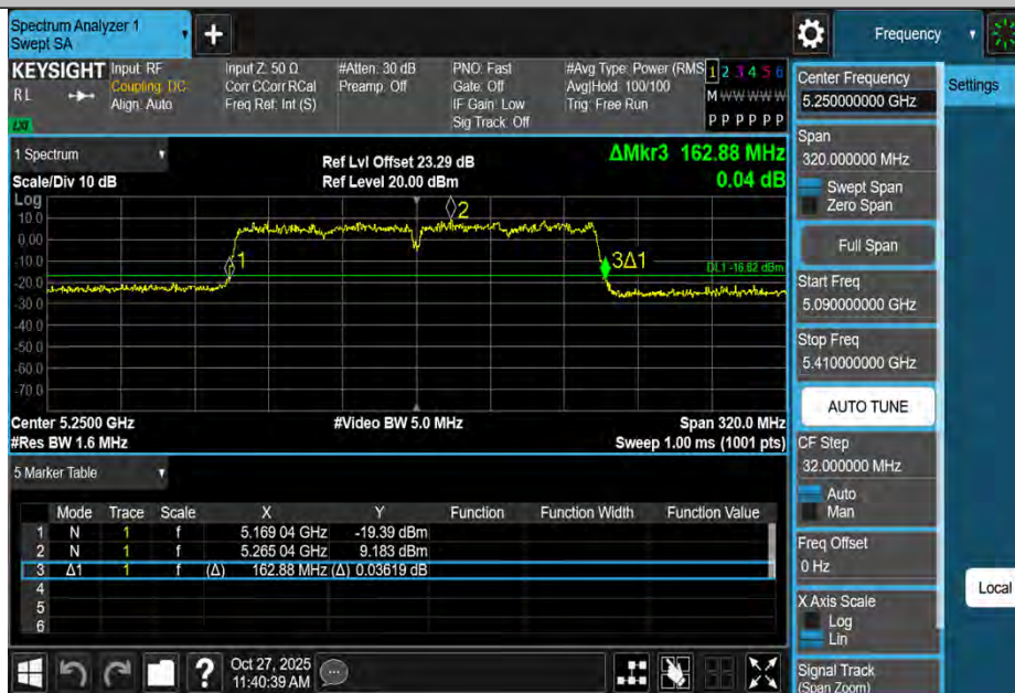
11AC160MIMO-Ant4-5250
