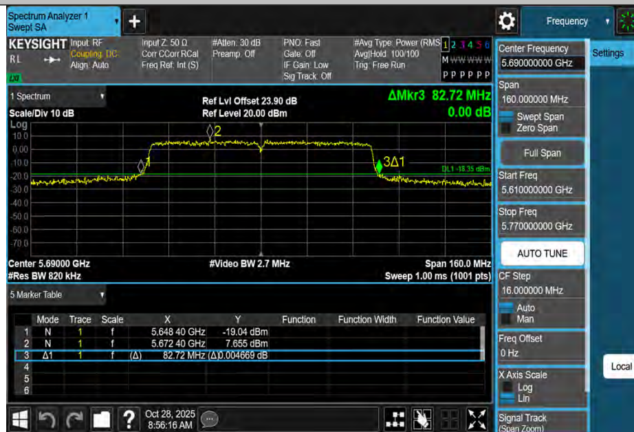
11AC80MIMO-Ant4-5690
