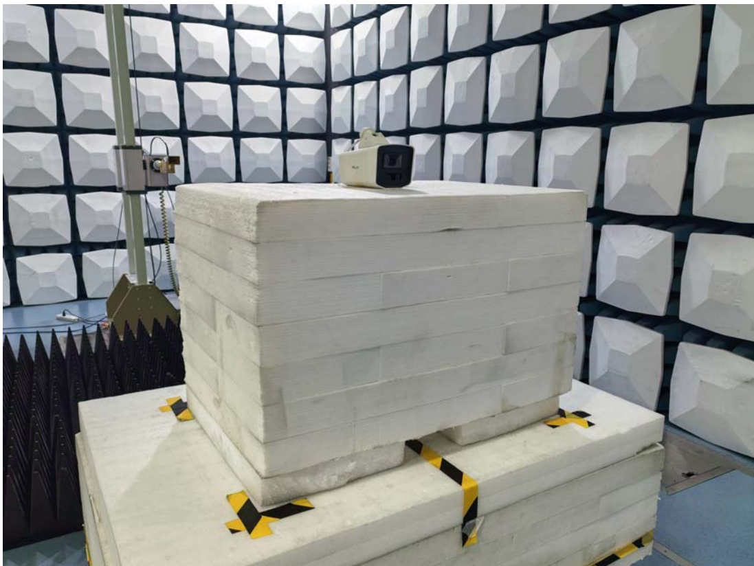
Radiated Emission Above 1GHz View 18-25G
