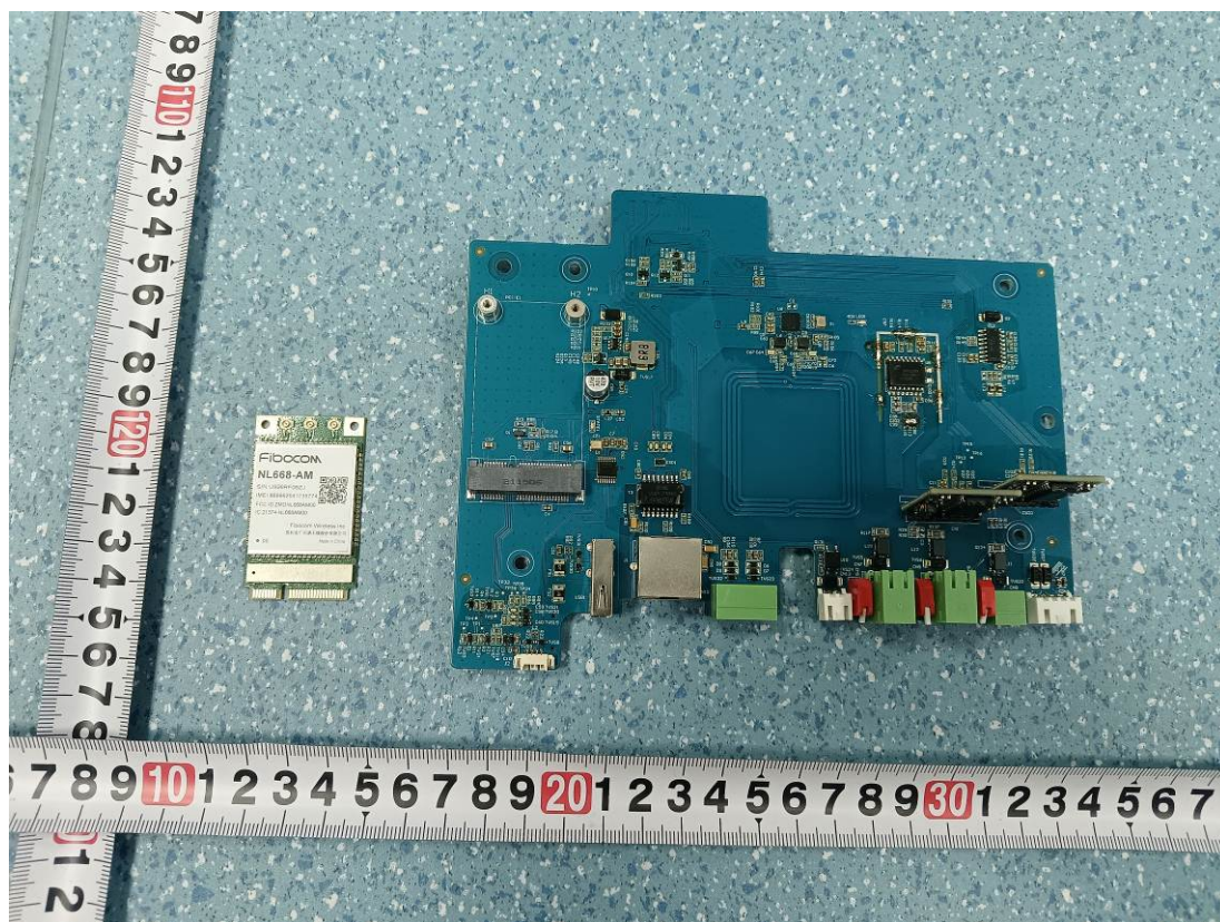
Contain WWAN Module, FCC ID:ZMONL668AM00, IC:21374-NL668AM00
