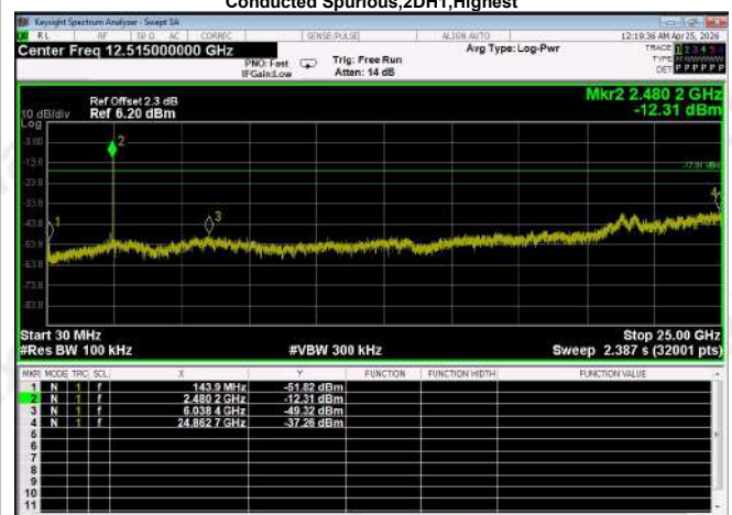
Conducted_Spurious,2DH1,Highest
