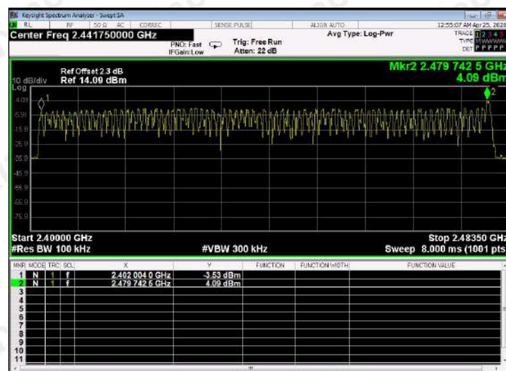
8-DPSK Modulation
