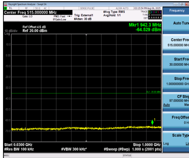
Band38_15MHz_16QAM_38175_1RB#0_30~1000_30~1000
