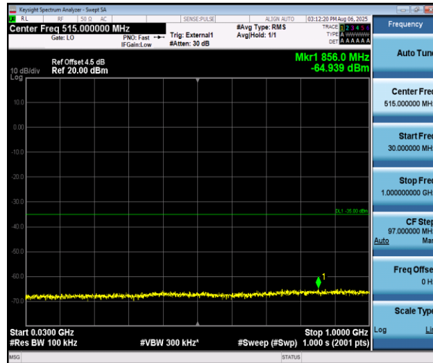
Band38_15MHz_QPSK_38000_1RB#0_30~1000_30~1000
