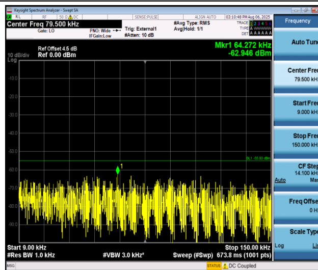
Band38_15MHz_16QAM_37825_1RB#0_0.009~0.15_0.009~0.15
