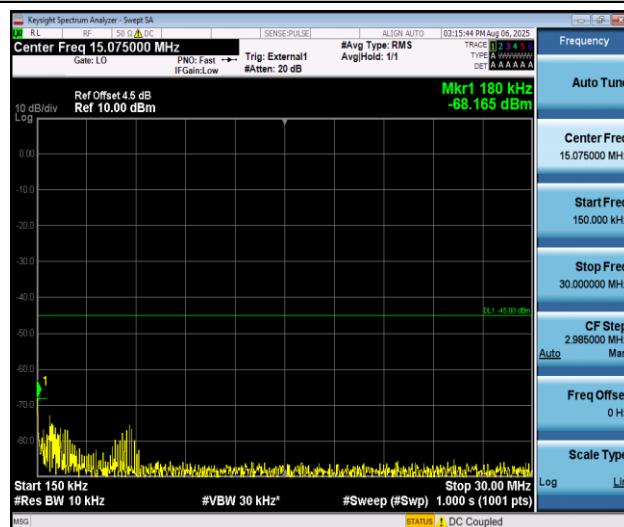
Band38_15MHz_16QAM_38175_1RB#0_0.15~30_0.15~30
