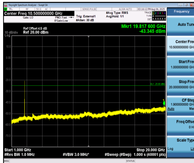
Band38_15MHz_16QAM_38175_1RB#0_1000~20000_1000~20000
