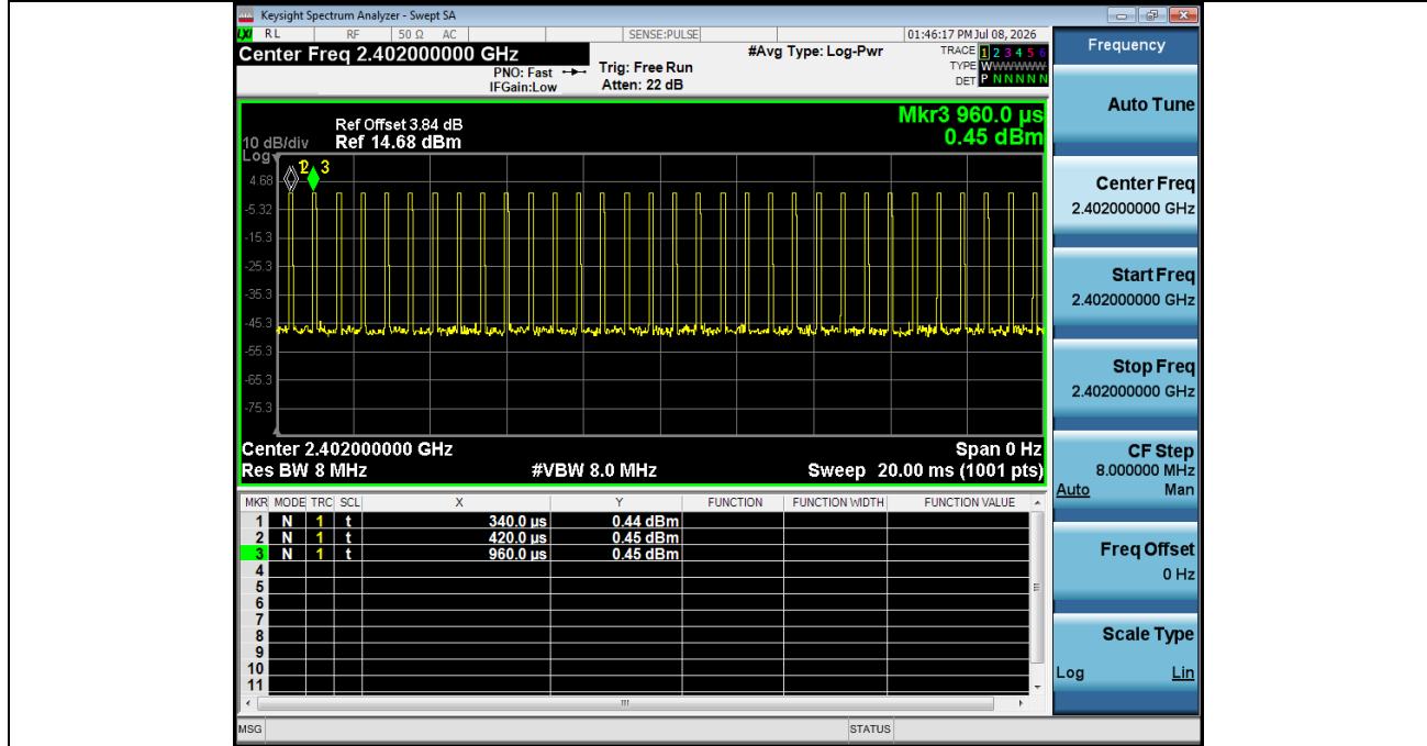
Duty Cycle NVNT_ANT1_1Mbps_2402
