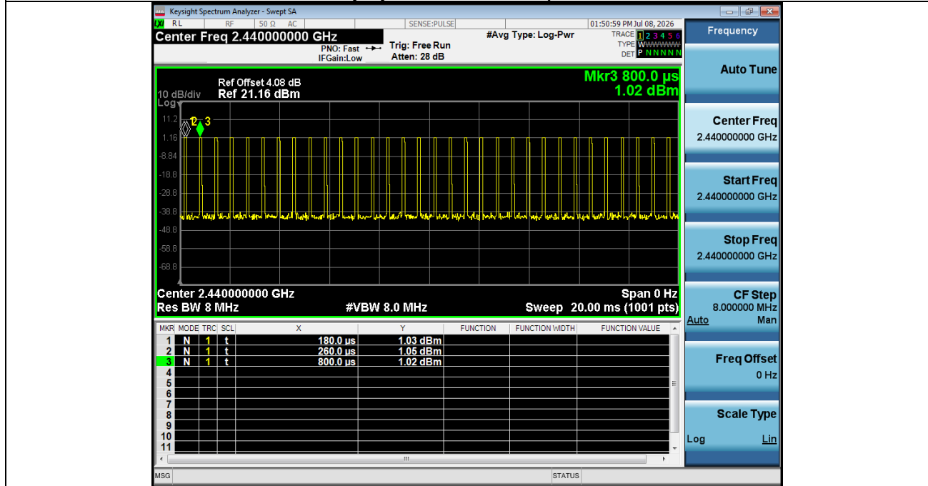
Duty Cycle NVNT_ANT1_1Mbps_2440
