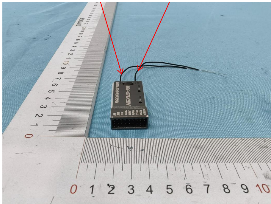
2.4G ANT2
