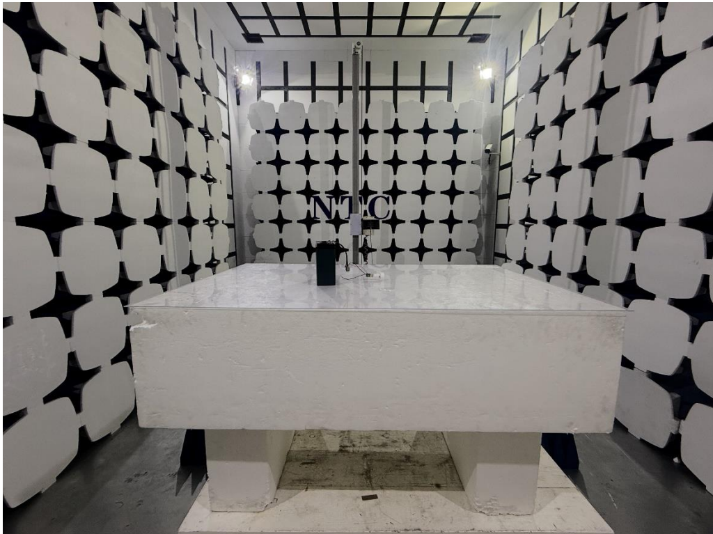
Photos of radiated emission test Above 1GHz
