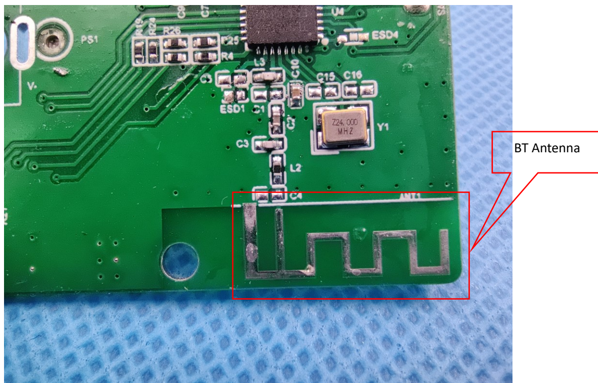
Internal view-3 of EUT
