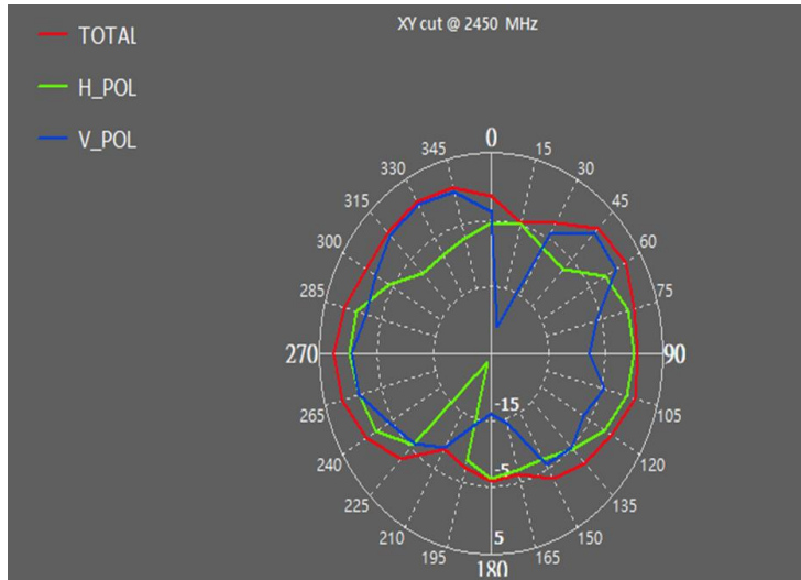
Radiation Pattern of WIFI3(2450 MHz)
