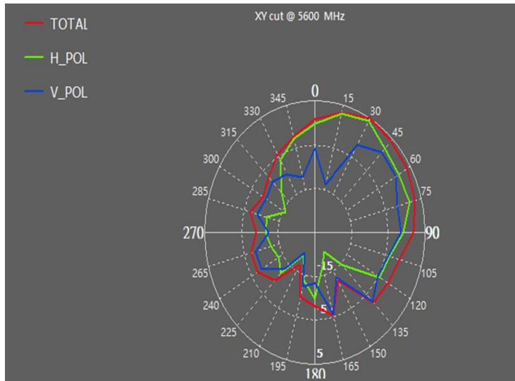
Radiation Pattern of WIFI3(5600 MHz)
