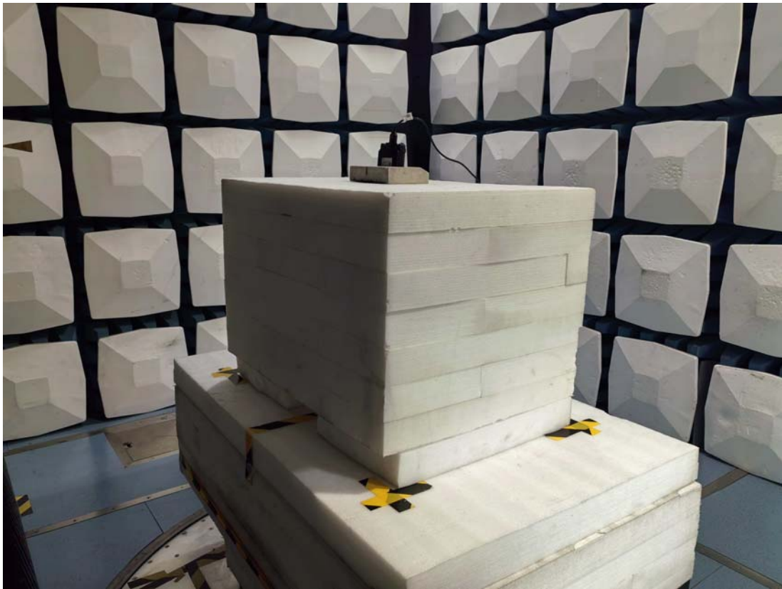
Radiated Emission Above 1GHz View 90-140G
