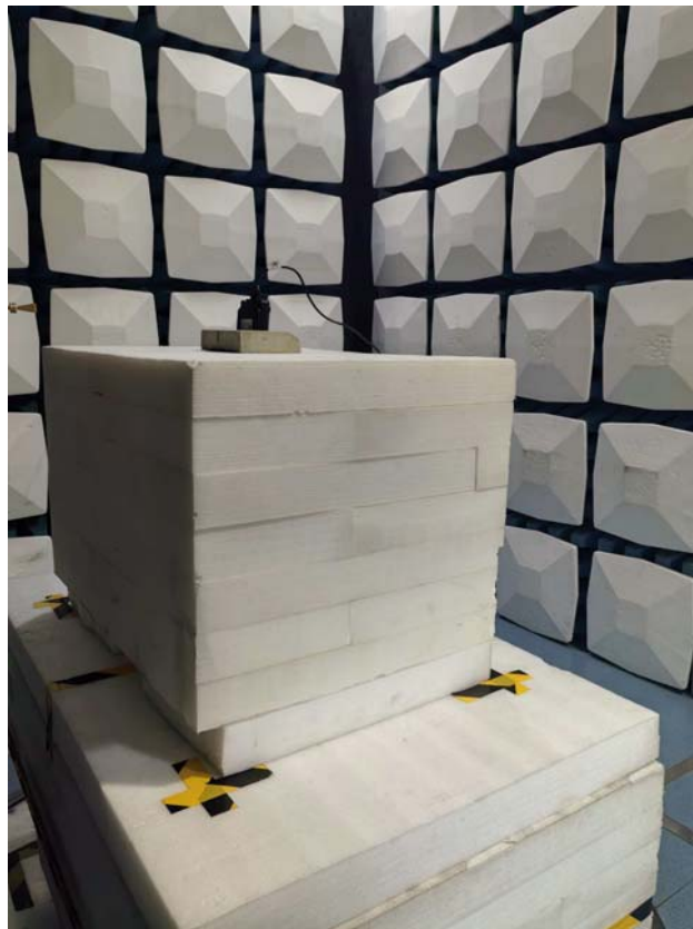
Radiated Emission Above 1GHz View 90-140G
