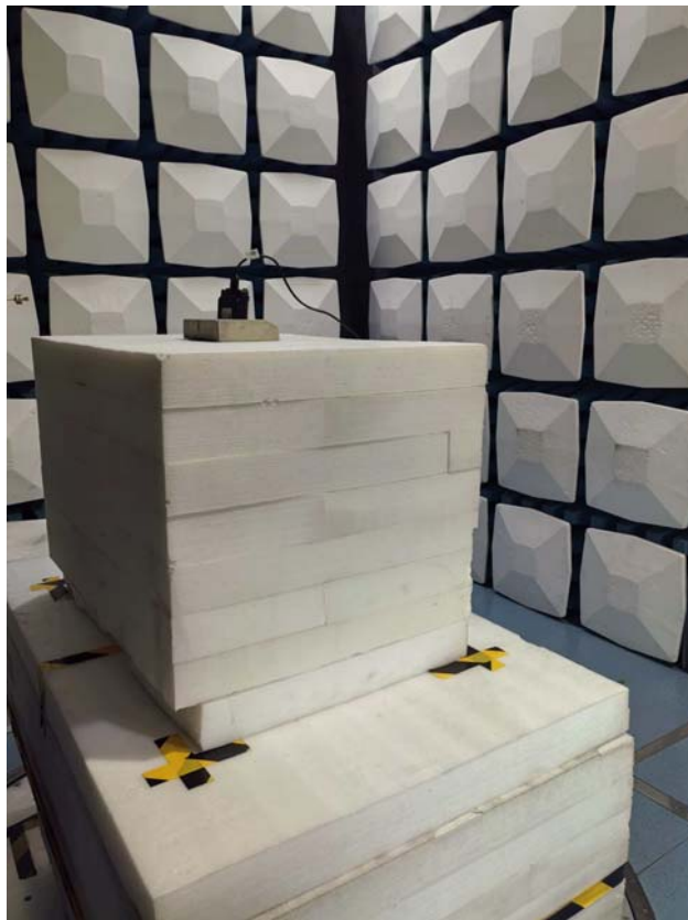
Radiated Emission Above 1GHz View 220-231G
