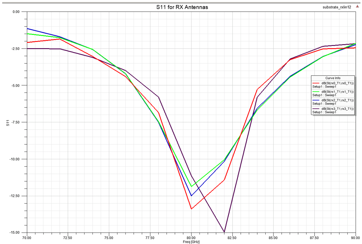
Figure 5 S11 for RX Antennas
