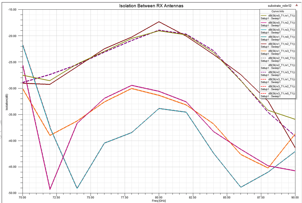
Figure 6 Isolation between RX Antennas
