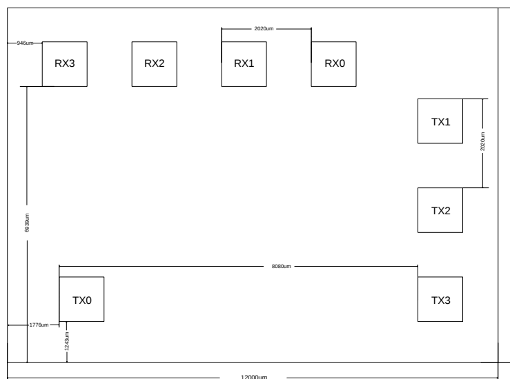
Figure 1 Configuration of RC7711C-AIP
