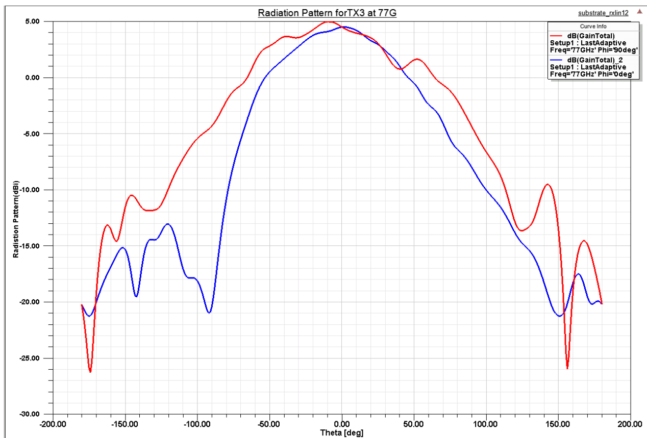
Figure 4 Radiation Pattern for TX Antennas at 77GHz
