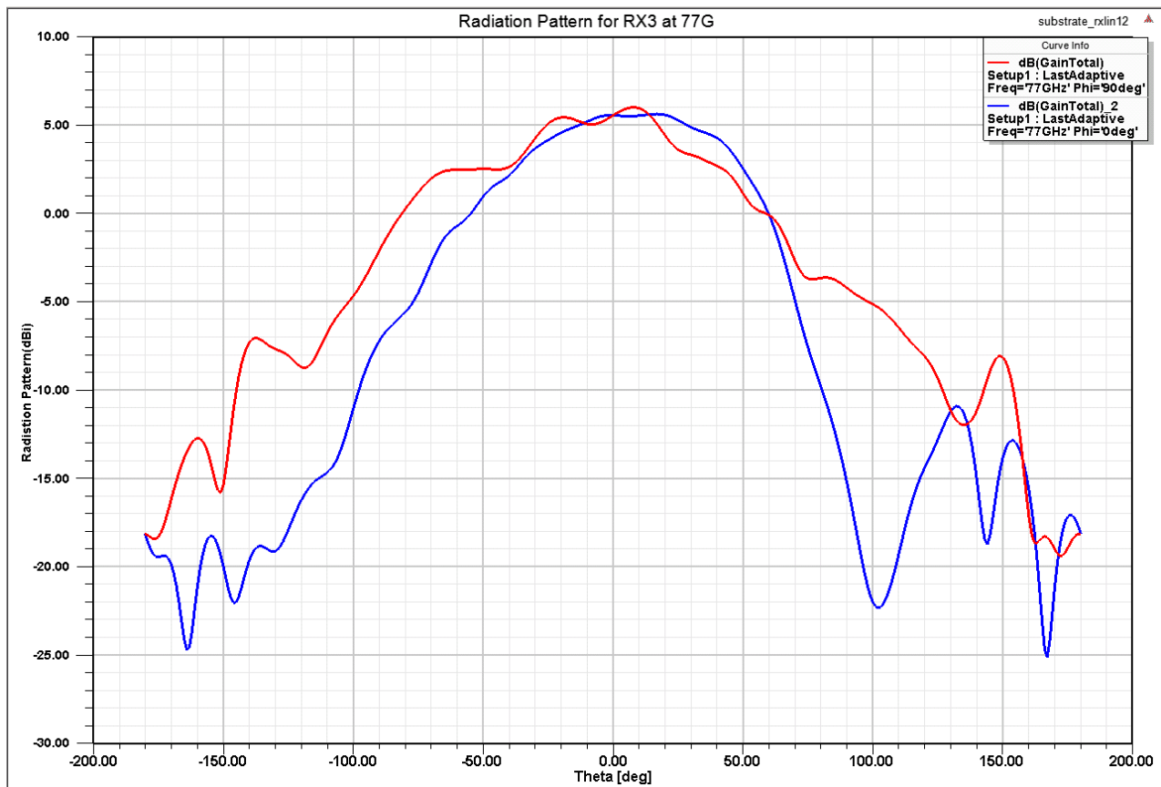
Figure 7 Radiation Pattern for RX Antennas at 77GHz
