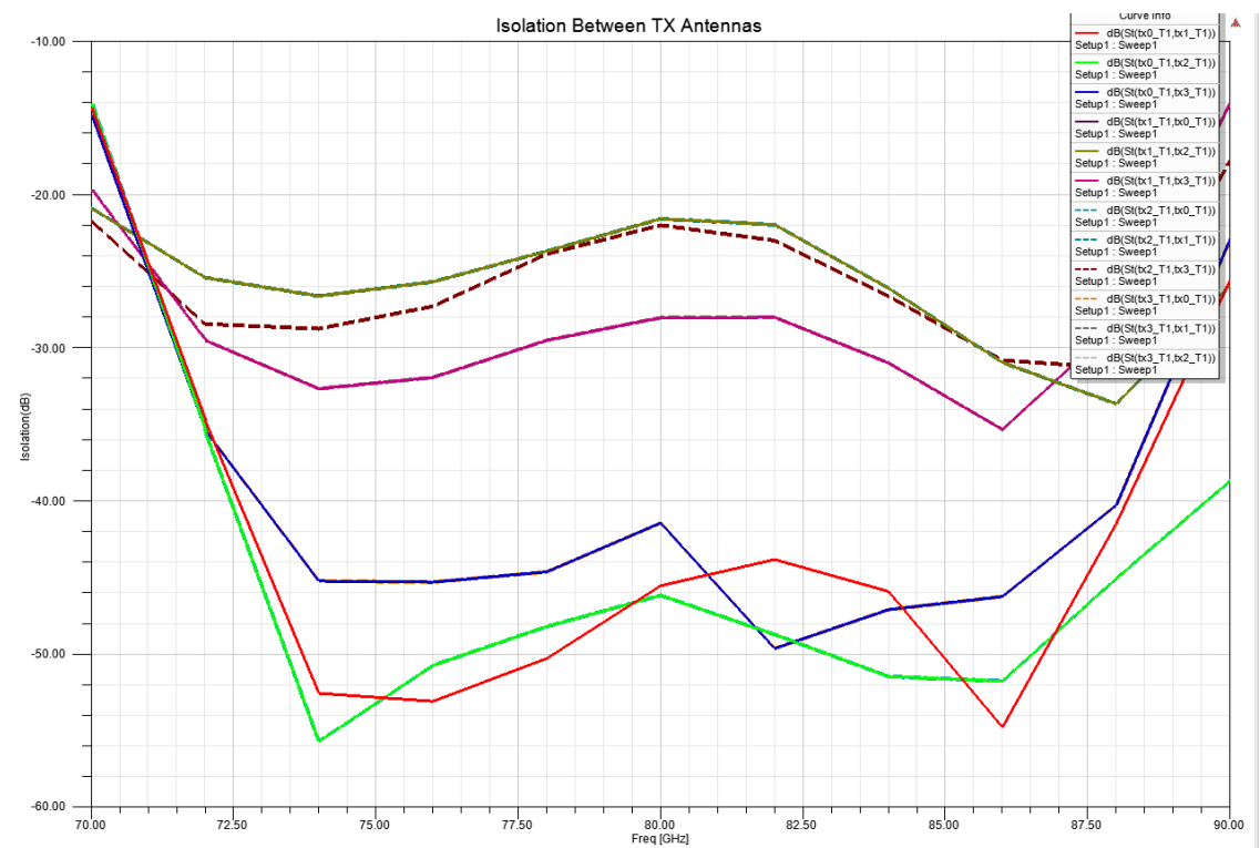
Figure 3 Isolation between TX Antennas
