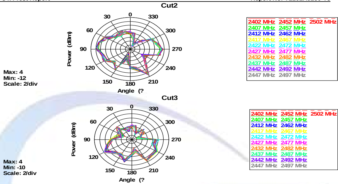
2402MHz ~2502 MHz Wi-Fi 2.4G 3D Gain
