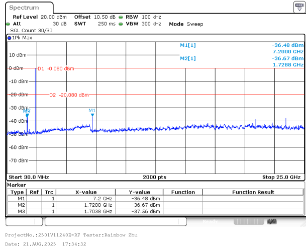
BLE_1M_High_Channel
