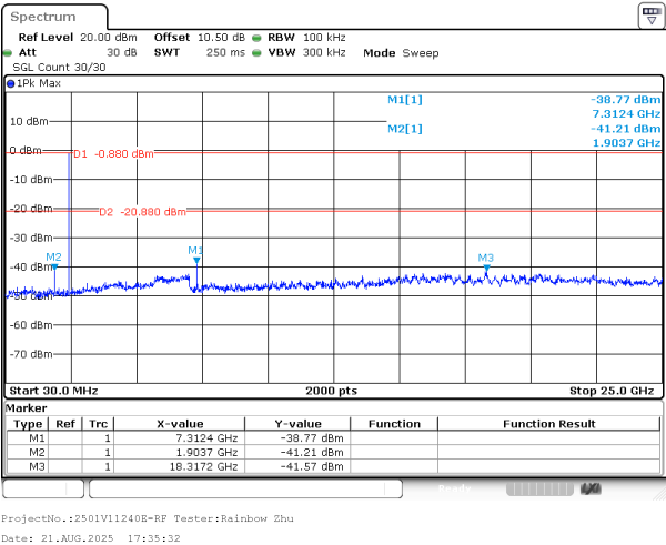
BLE_1M_Middle_Channel
