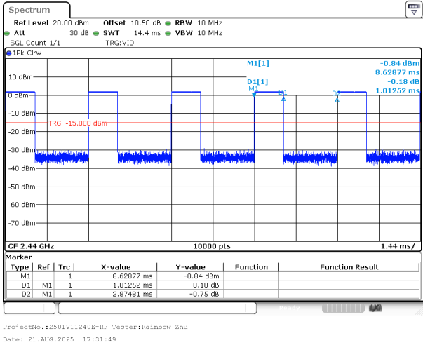
BLE_1M_Middle_Channel
