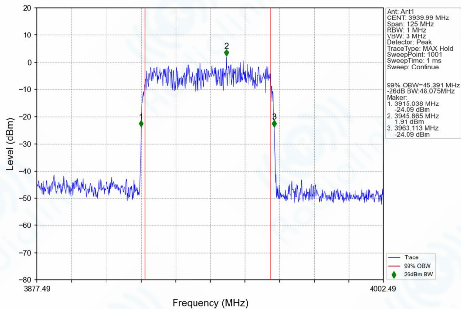
n77h_30kHz_SISO_NTNV_50MHz_DFT-s-OFDM_256_QAM_3939.99MHz_Outer_Full_Ant1
