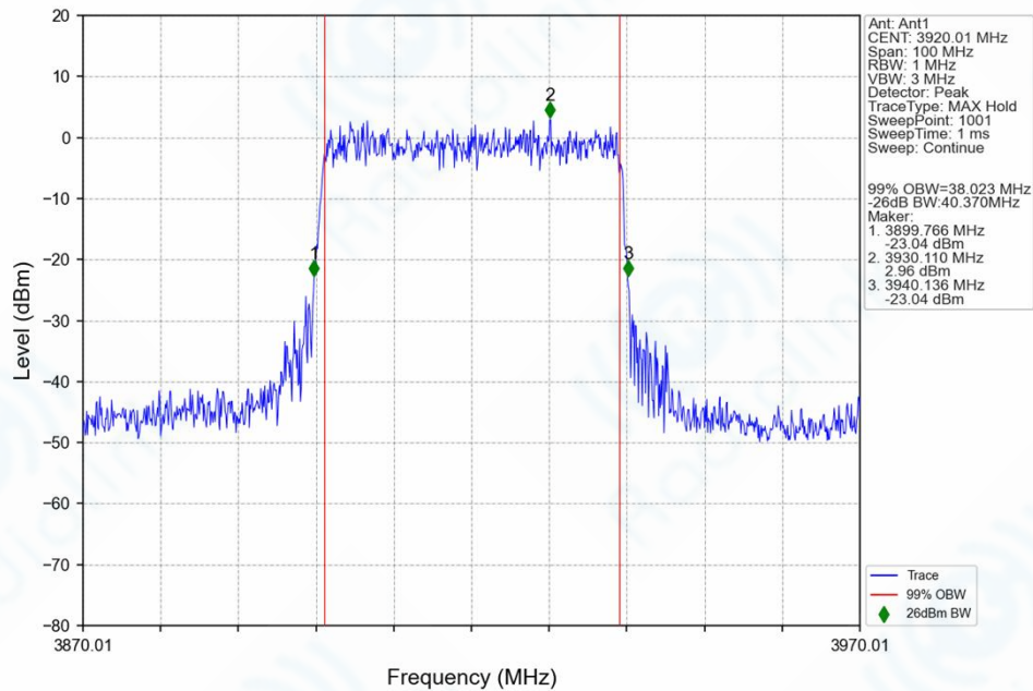
n77h_30kHz_SISO_NTNV_40MHz_CP-OFDM_64 QAM_3920.01MHz_Outer_Full_Ant1
