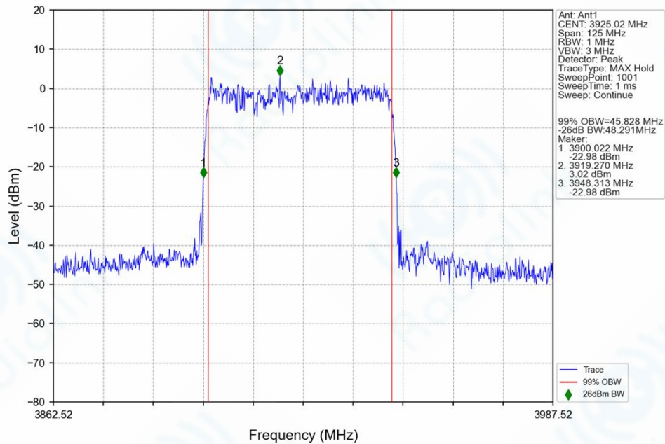
n77h_30kHz_SISO_NTNV_50MHz_DFT-s-OFDM_64_QAM_3925.02MHz_Outer_Full_Ant1
