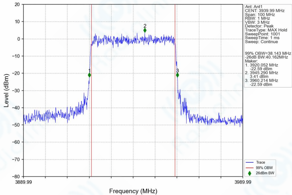
n77h_30kHz_SISO_NTNV_40MHz_CP-OFDM_16_QAM_3939.99MHz_Outer_Full_Ant1
