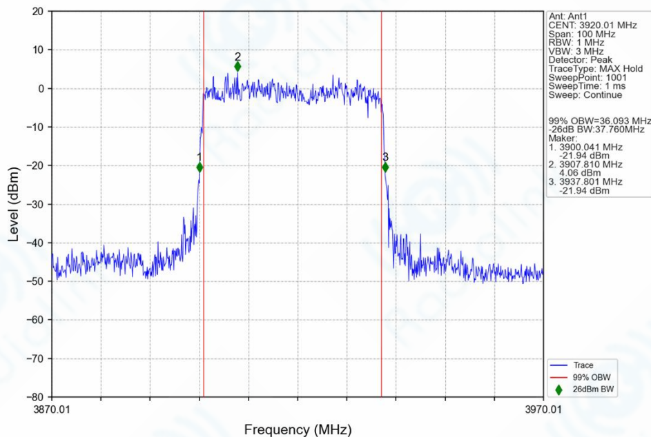
n77h_30kHz_SISO_NTNV_40MHz_DFT-s-OFDM_64_QAM_3920.01MHz_Outer_Full_Ant1
