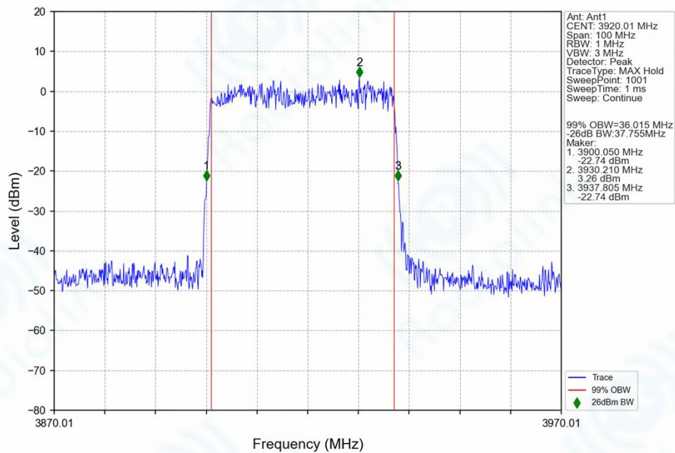
n77h_30kHz_SISO_NTNV_40MHz_DFT-s-OFDM QPSK_3920.01MHz_Outer_Full_Ant1
