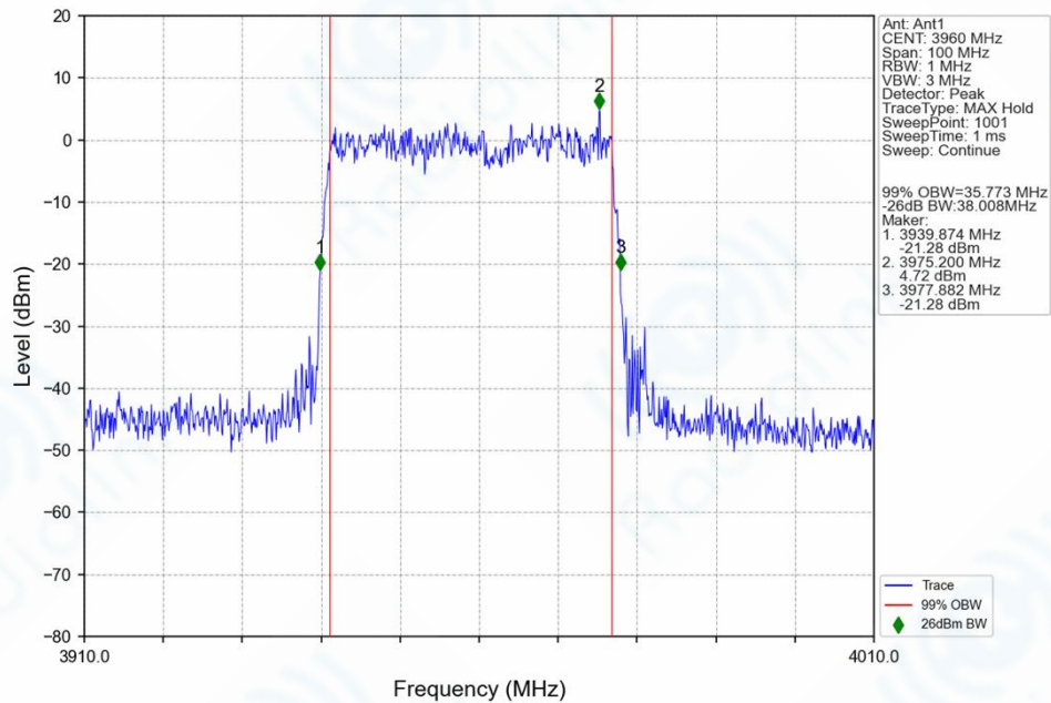
n77h_30kHz_SISO_NTNV_40MHz_DFT-s-OFDM_64_QAM_3960MHz_Outer_Full_Ant1
