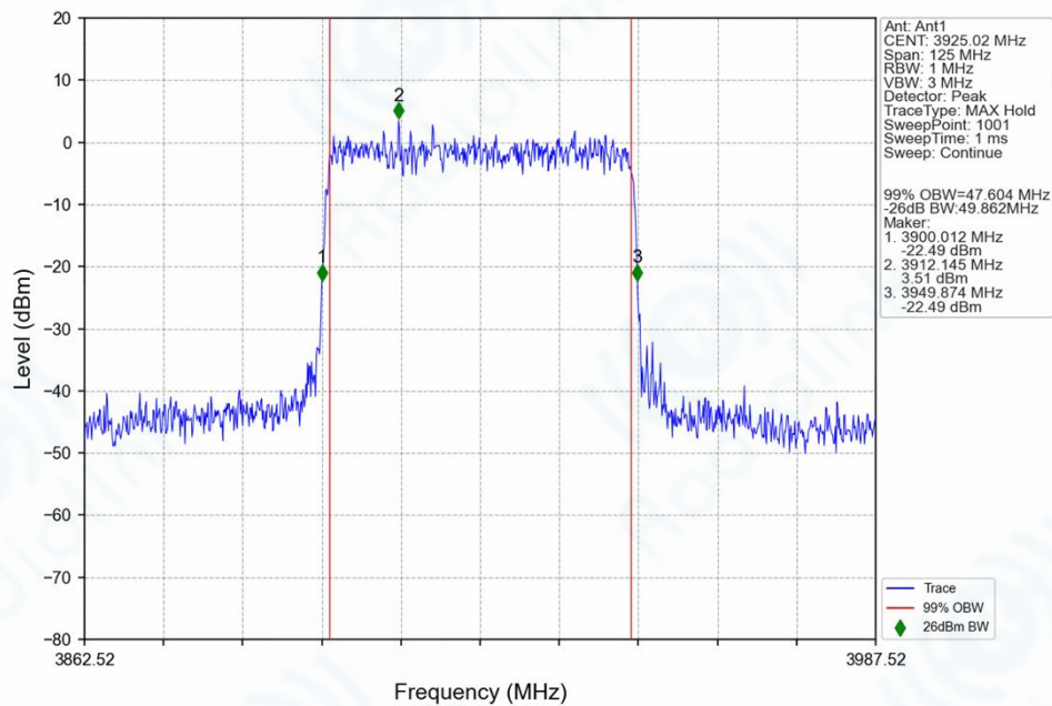
n77h_30kHz_SISO_NTNV_50MHz_CP-OFDM_QPSK_3925.02MHz_Outer_Full_Ant1
