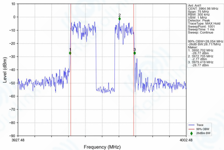
n77h_30kHz_SISO_NTNV_30MHz_CP-OFDM_64_QAM_3964.98MHz_Outer_Full_Ant1
