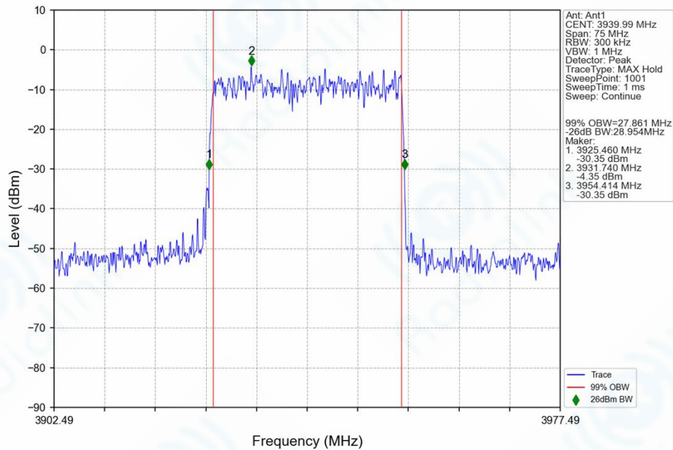
n77h_30kHz_SISO_NTNV_30MHz_CP-OFDM_256_QAM_3939.99MHz_Outer_Full_Ant1
