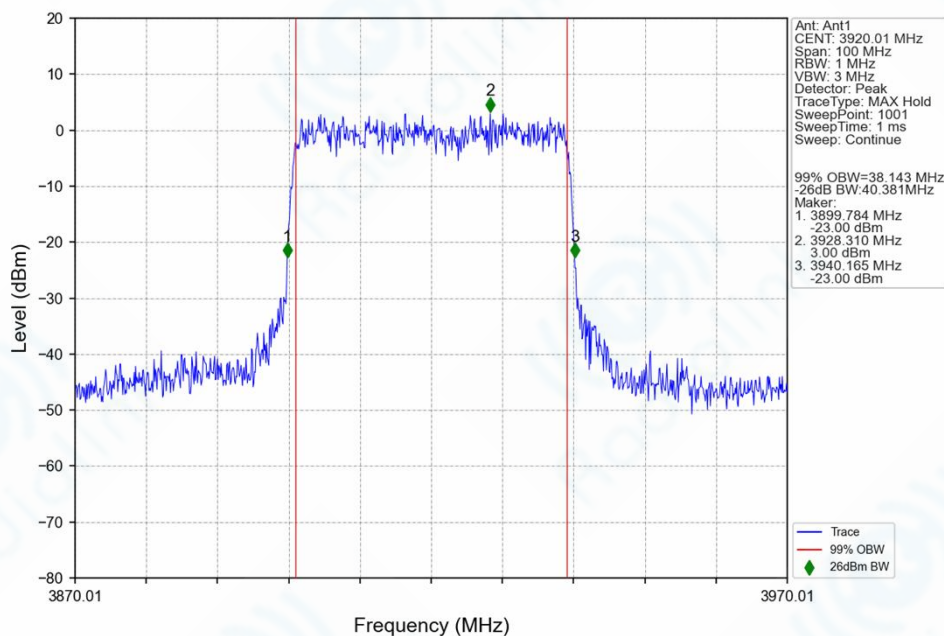
n77h_30kHz_SISO_NTNV_40MHz_CP-OFDM_QPSK_3920.01MHz_Outer_Full_Ant1
