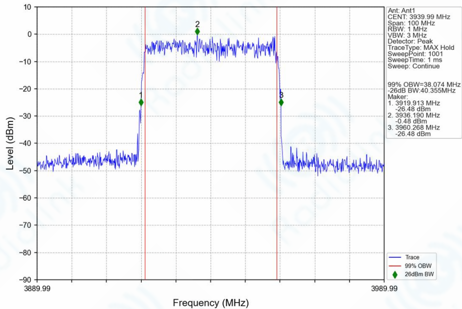
n77h_30kHz_SISO_NTNV_40MHz_CP-OFDM_256_QAM_3939.99MHz_Outer_Full_Ant1
