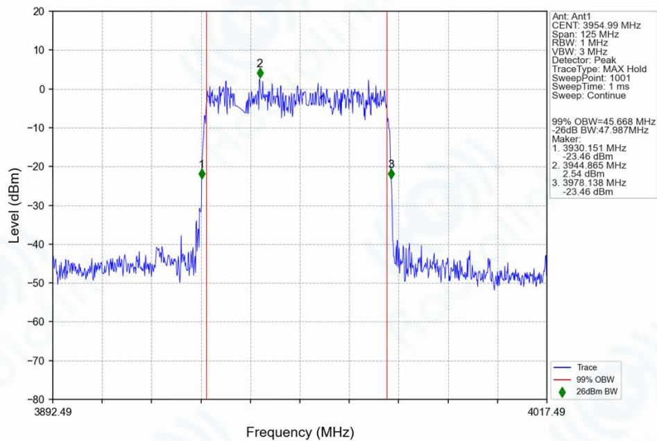
n77h_30kHz_SISO_NTNV_50MHz_DFT-s-OFDM_QPSK_3954.99MHz_Outer_Full_Ant1
