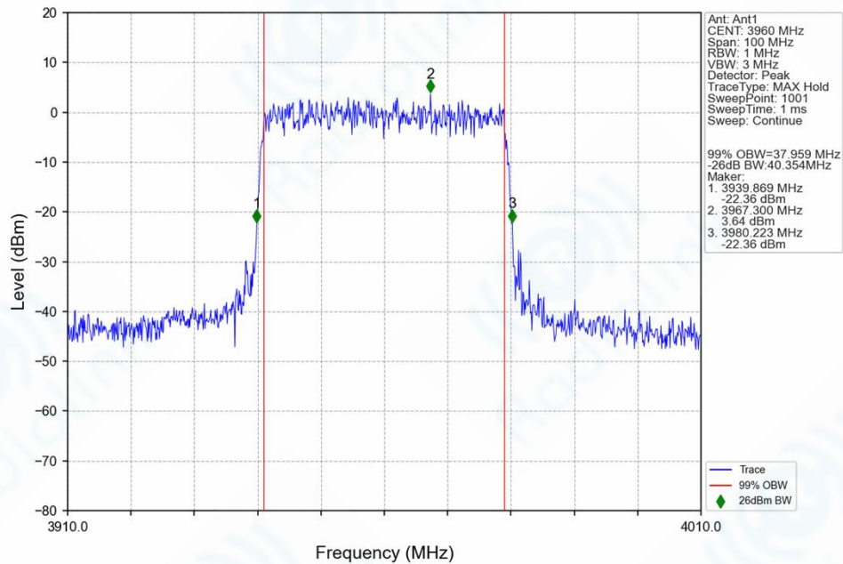
n77h_30kHz_SISO_NTNV_40MHz_CP-OFDM_QPSK_3960MHz_Outer_Full_Ant1
