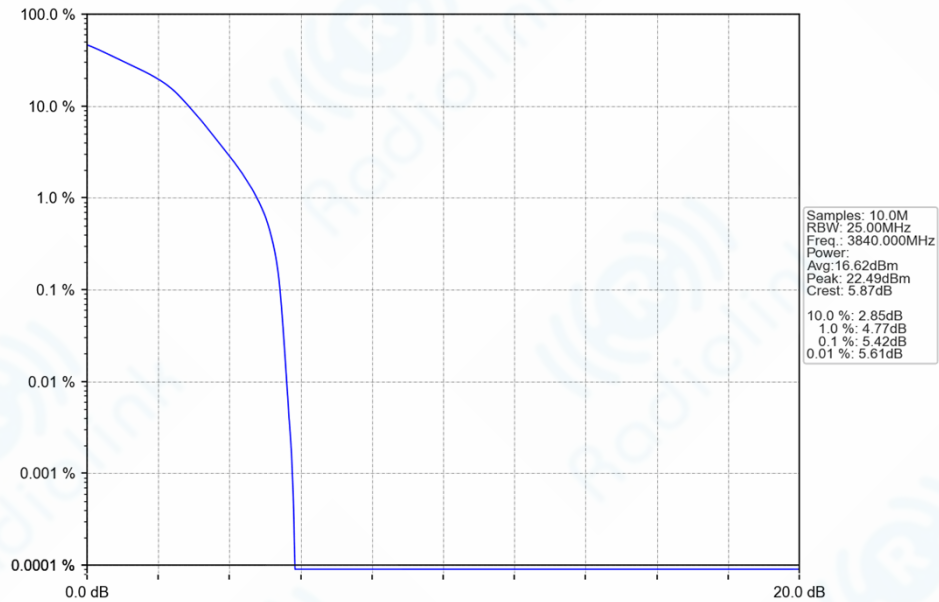
n77a_30kHz_SISO_NTNV_20MHz_DFT-s-OFDM_16_QAM_3840MHz_Outer_Full_Ant1
