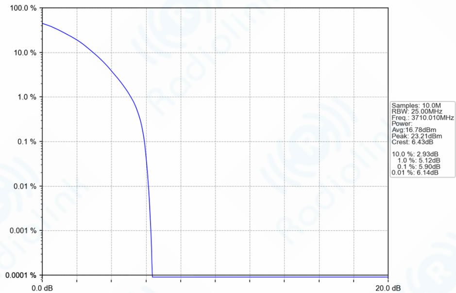
n77a_30kHz_SISO_NTNV_20MHz_DFT-s-OFDM_64_QAM_3710.01MHz_Outer_Full_Ant1
