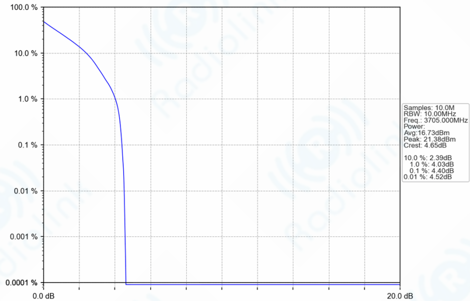
n77a_30kHz_SISO_NTNV_10MHz_DFT-s-OFDM QPSK_3705MHz_Outer_Full_Ant1
