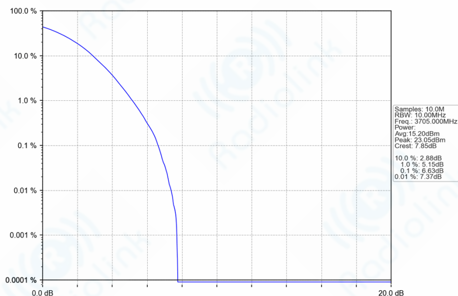
n77a_30kHz_SISO_NTNV_10MHz_DFT-s-OFDM_256_QAM_3705MHz_Outer_Full_Ant1
