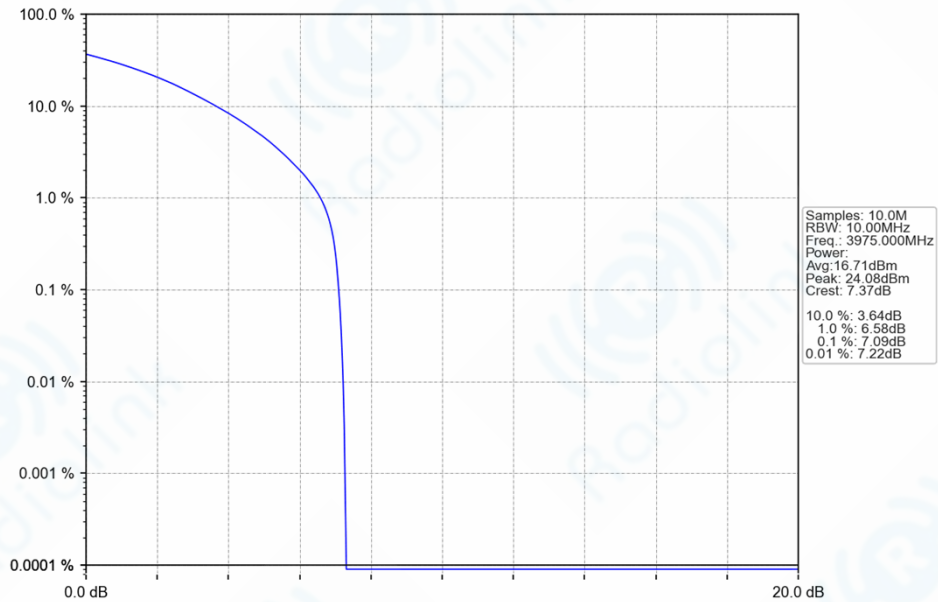
n77a_30kHz_SISO_NTNV_10MHz_CP-OFDM_64_QAM_3975MHz_Outer_Full_Ant1
