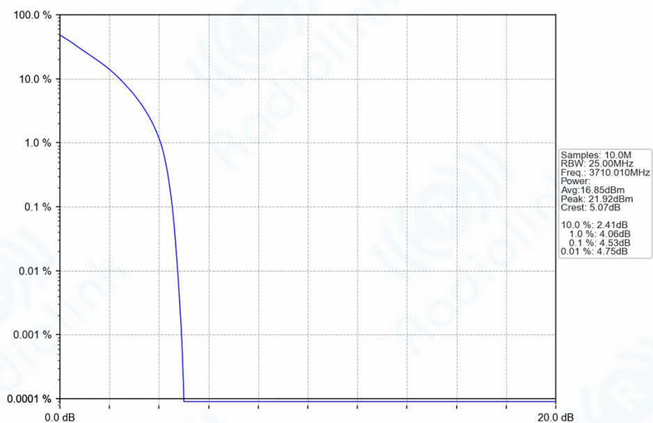
n77a_30kHz_SISO_NTNV_20MHz_DFT-s-OFDM_QPSK_3710.01MHz_Outer_Full_Ant1
