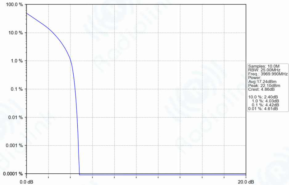
n77a_30kHz_SISO_NTNV_20MHz_DFT-s-OFDM_QPSK_3969.99MHz_Outer_Full_Ant1
