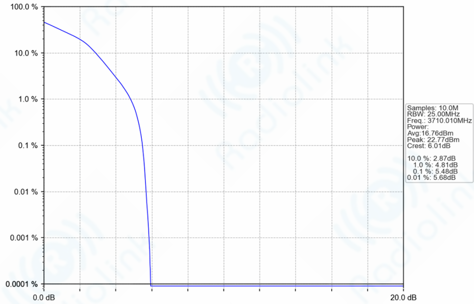
n77a_30kHz_SISO_NTNV_20MHz_DFT-s-OFDM_16_QAM_3710.01MHz_Outer_Full_Ant1
