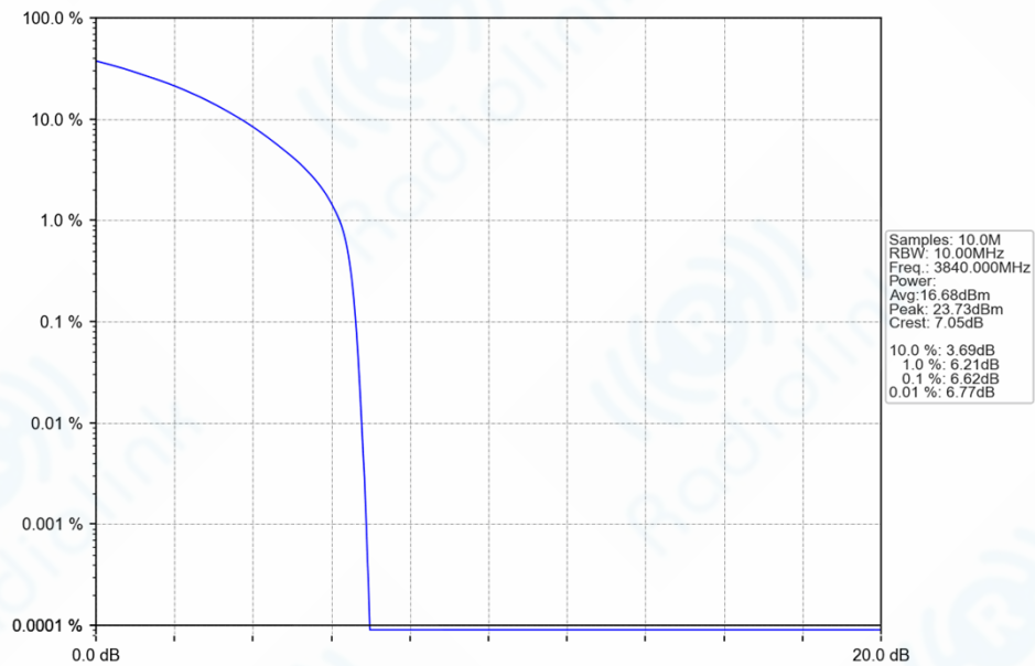
n77a_30kHz_SISO_NTNV_10MHz_CP-OFDM_16_QAM_3840MHz_Outer_Full_Ant1
