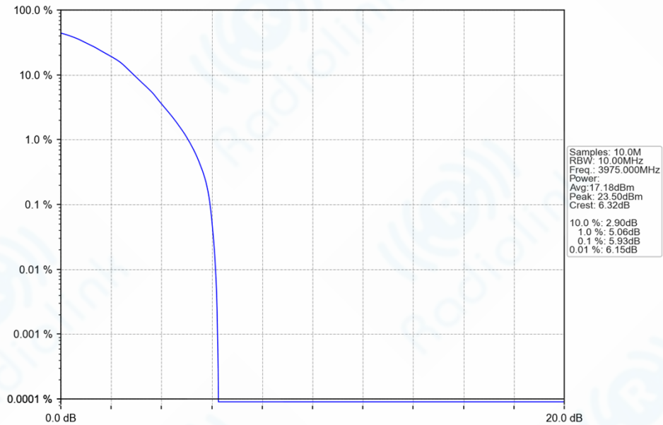
n77a_30kHz_SISO_NTNV_10MHz_DFT-s-OFDM_64_QAM_3975MHz_Outer_Full_Ant1
