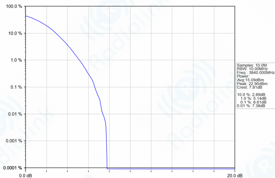
n77a_30kHz_SISO_NTNV_10MHz_DFT-s-OFDM_256_QAM_3840MHz_Outer_Full_Ant1
