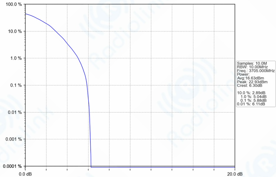
n77a_30kHz_SISO_NTNV_10MHz_DFT-s-OFDM_64_QAM_3705MHz_Outer_Full_Ant1
