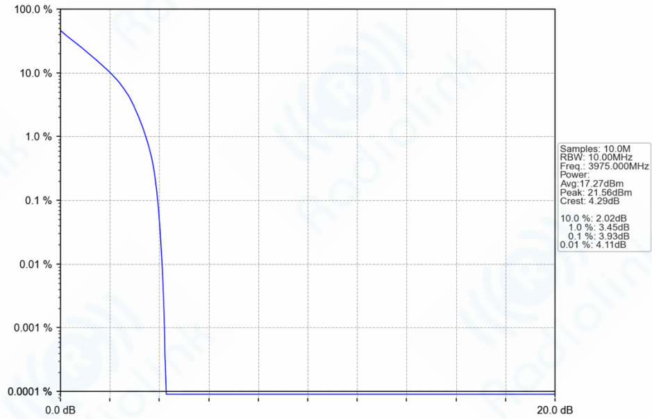
n77a_30kHz_SISO_NTNV_10MHz_DFT-s-OFDM PI/2 BPSK_3975MHz_Outer_Full_Ant1
