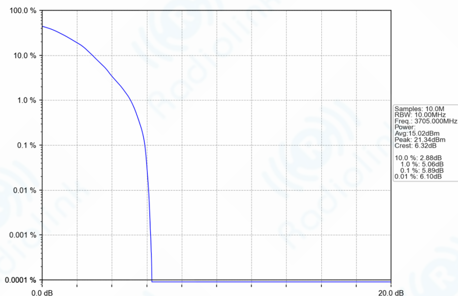
n78a_30kHz_SISO_NTNV_10MHz_DFT-s-OFDM_64_QAM_3705MHz_Outer_Full_Ant1
