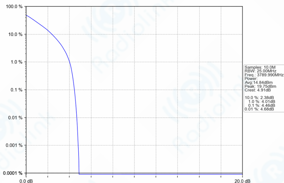
n78a_30kHz_SISO_NTNV_20MHz_DFT-s-OFDM_QPSK_3789.99MHz_Outer_Full_Ant1
