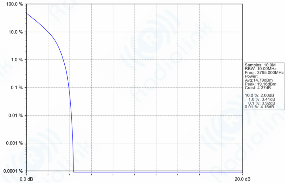
n78a_30kHz_SISO_NTNV_10MHz_DFT-s-OFDM PI/2 BPSK_3795MHz_Outer_Full_Ant1
