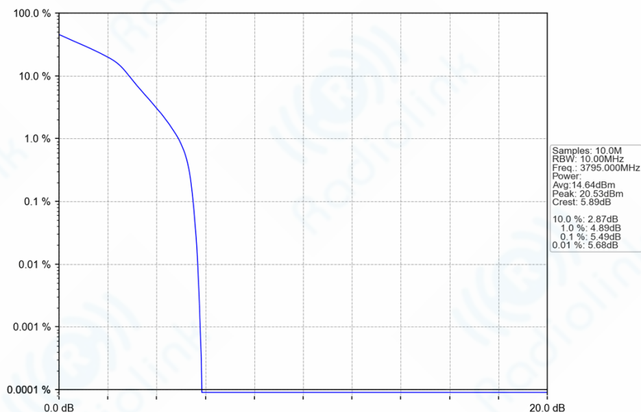
n78a_30kHz_SISO_NTNV_10MHz_DFT-s-OFDM_16_QAM_3795MHz_Outer_Full_Ant1
