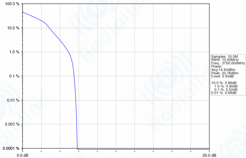
n78a_30kHz_SISO_NTNV_10MHz_DFT-s-OFDM_16_QAM_3750MHz_Outer_Full_Ant1
