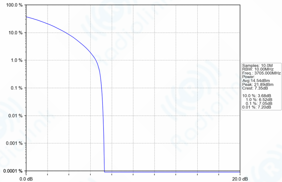
n78a_30kHz_SISO_NTNV_10MHz_CP-OFDM 64 QAM 3705MHz_Outer_Full_Ant1
