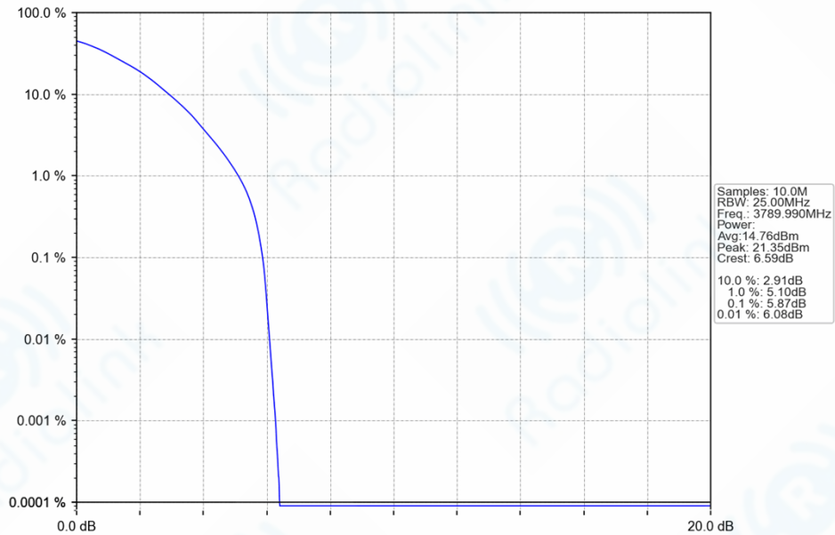
n78a_30kHz_SISO_NTNV_20MHz_DFT-s-OFDM_64_QAM_3789.99MHz_Outer_Full_Ant1
