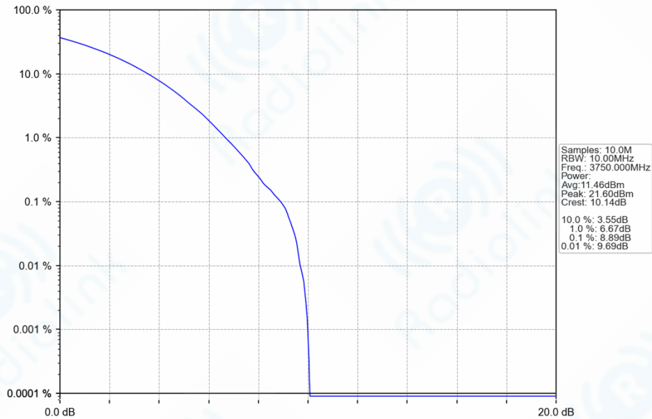
n78a_30kHz_SISO_NTNV_10MHz_CP-OFDM_256_QAM_3750MHz_Outer_Full_Ant1
