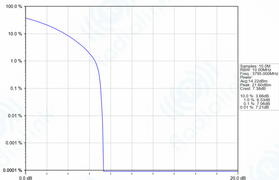
n78a_30kHz_SISO_NTNV_10MHz_CP-OFDM_64_QAM_3795MHz_Outer_Full_Ant1
