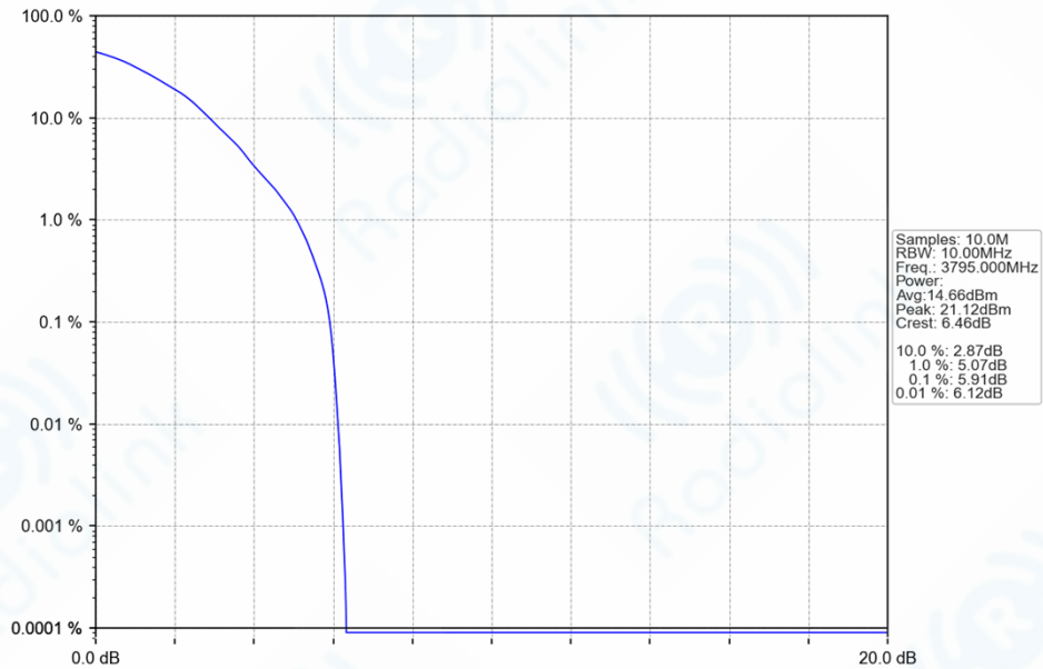
n78a_30kHz_SISO_NTNV_10MHz_DFT-s-OFDM_64_QAM_3795MHz_Outer_Full_Ant1
