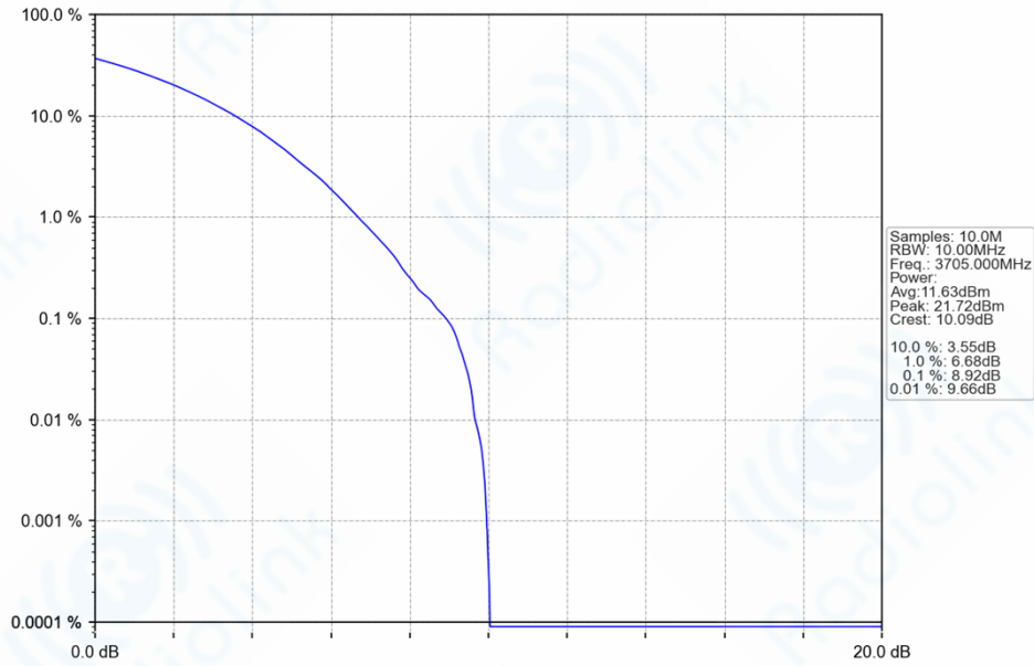
n78a_30kHz_SISO_NTNV_10MHz_CP-OFDM_256_QAM_3705MHz_Outer_Full_Ant1
