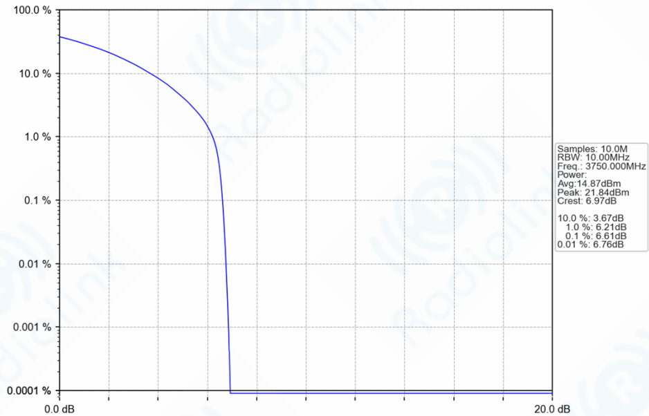
n78a_30kHz_SISO_NTNV_10MHz_CP-OFDM_16_QAM_3750MHz_Outer_Full_Ant1
