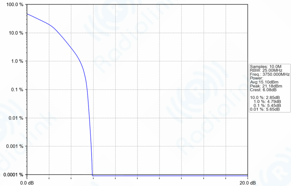
n78a_30kHz_SISO_NTNV_20MHz_DFT-s-OFDM_16_QAM_3750MHz_Outer_Full_Ant1
