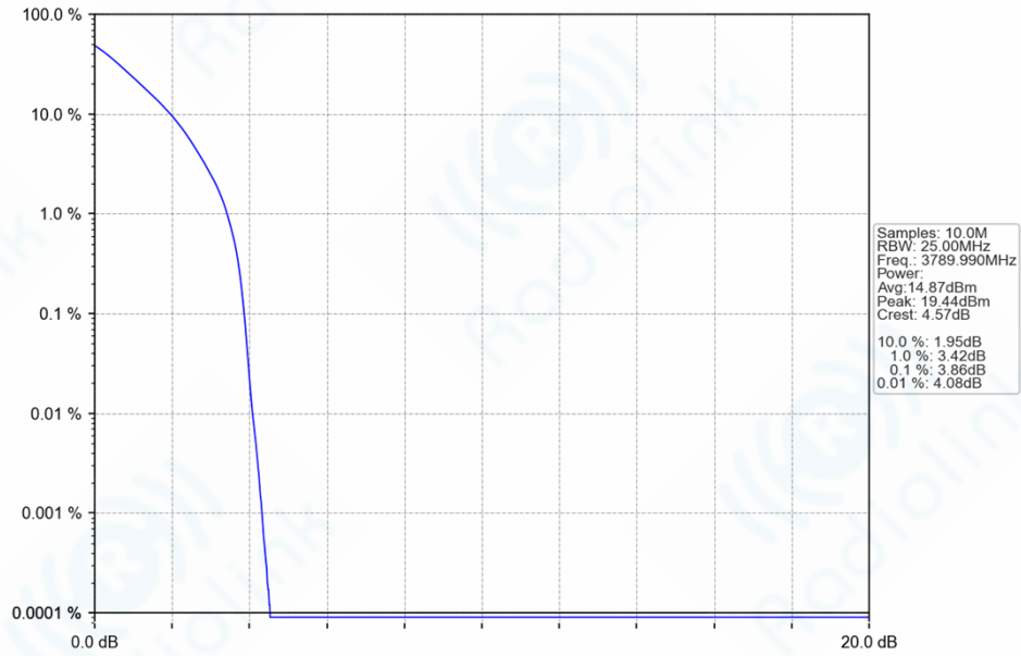
n78a_30kHz_SISO_NTNV_20MHz_DFT-s-OFDM_PI/2_BPSK_3789.99MHz_Outer_Full_Ant1
