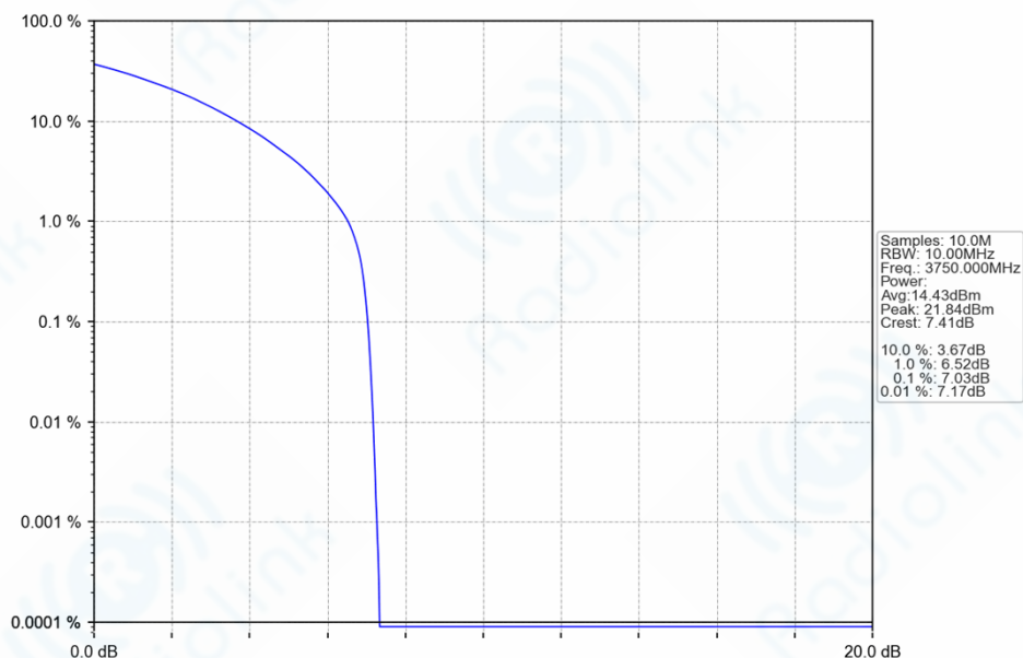
n78a_30kHz_SISO_NTNV_10MHz_CP-OFDM_64_QAM_3750MHz_Outer_Full_Ant1
