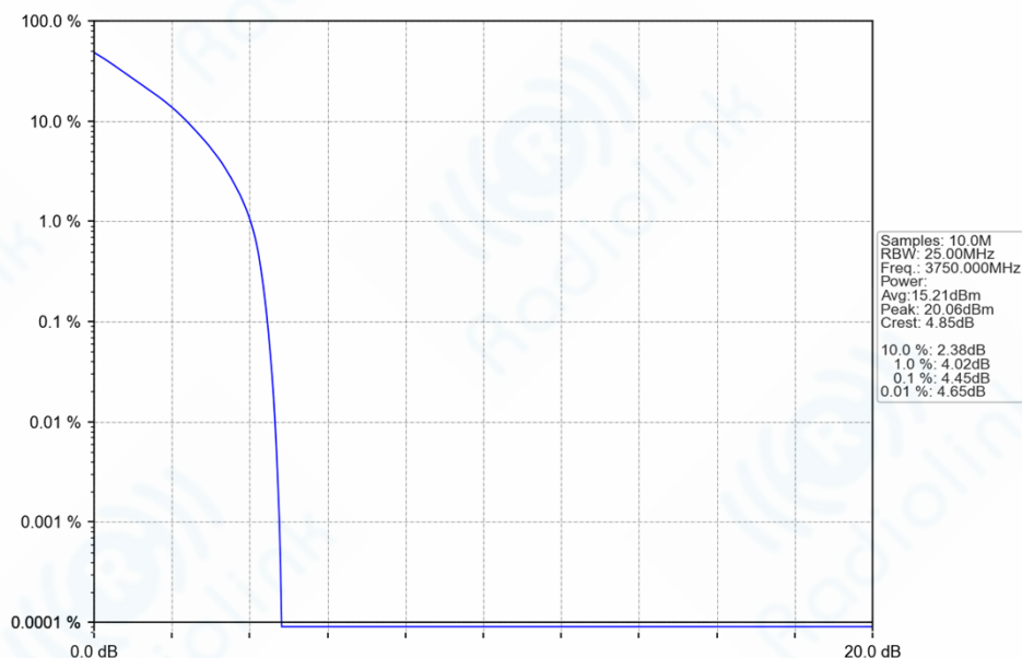
n78a_30kHz_SISO_NTNV_20MHz_DFT-s-OFDM_QPSK_3750MHz_Outer_Full_Ant1
