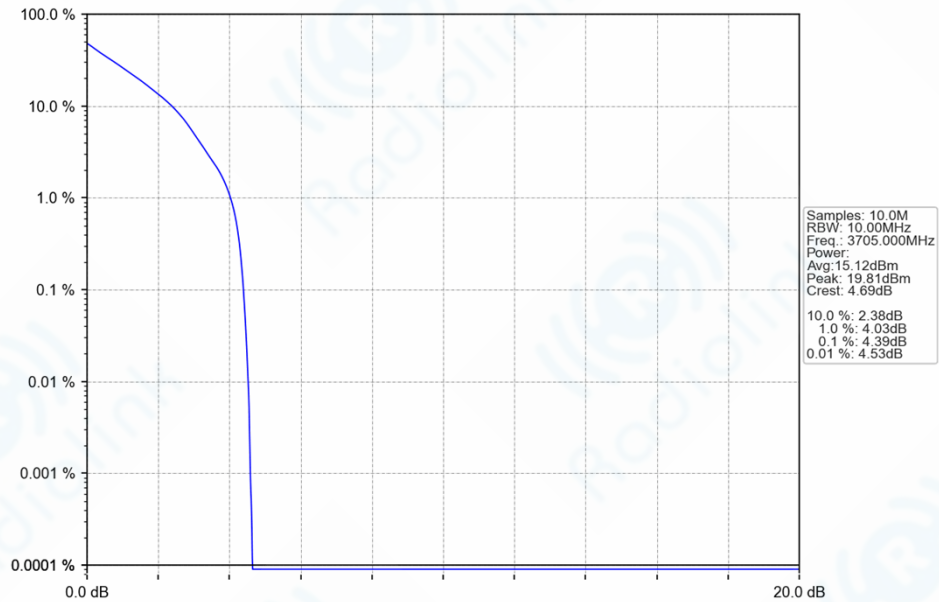
n78a_30kHz_SISO_NTNV_10MHz_DFT-s-OFDM QPSK_3705MHz_Outer_Full_Ant1
