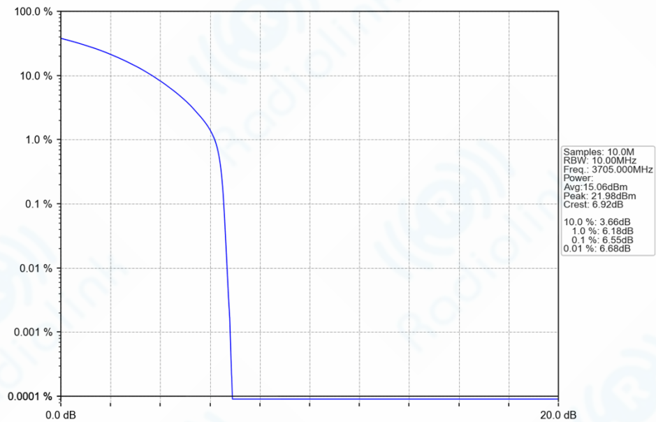
n78a_30kHz_SISO_NTNV_10MHz_CP-OFDM_QPSK_3705MHz_Outer_Full_Ant1
