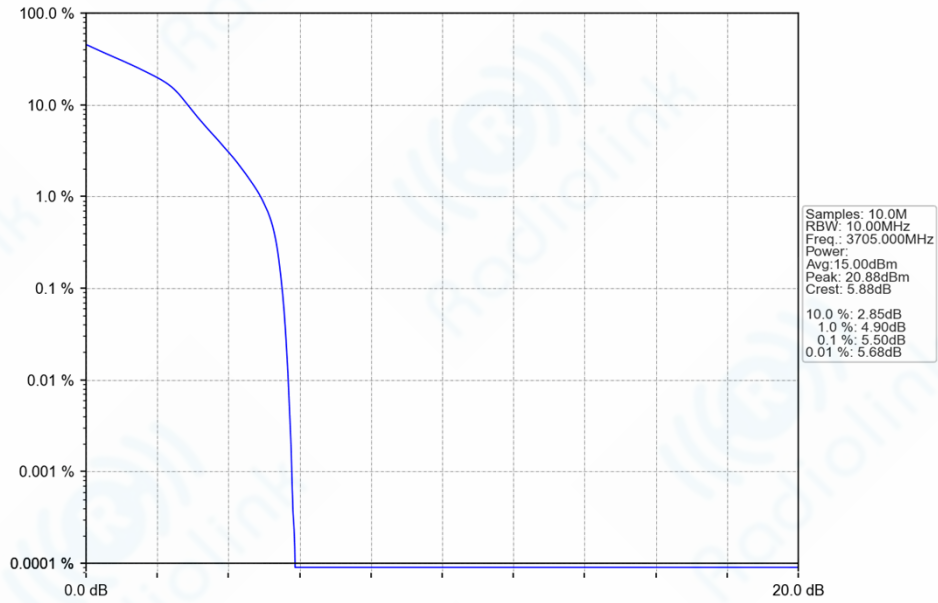
n78a_30kHz_SISO_NTNV_10MHz_DFT-s-OFDM_16_QAM_3705MHz_Outer_Full_Ant1
