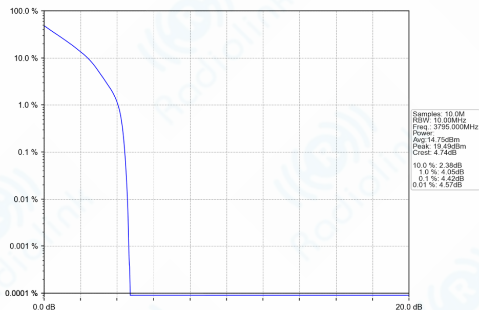
n78a_30kHz_SISO_NTNV_10MHz_DFT-s-OFDM_QPSK_3795MHz_Outer_Full_Ant1
