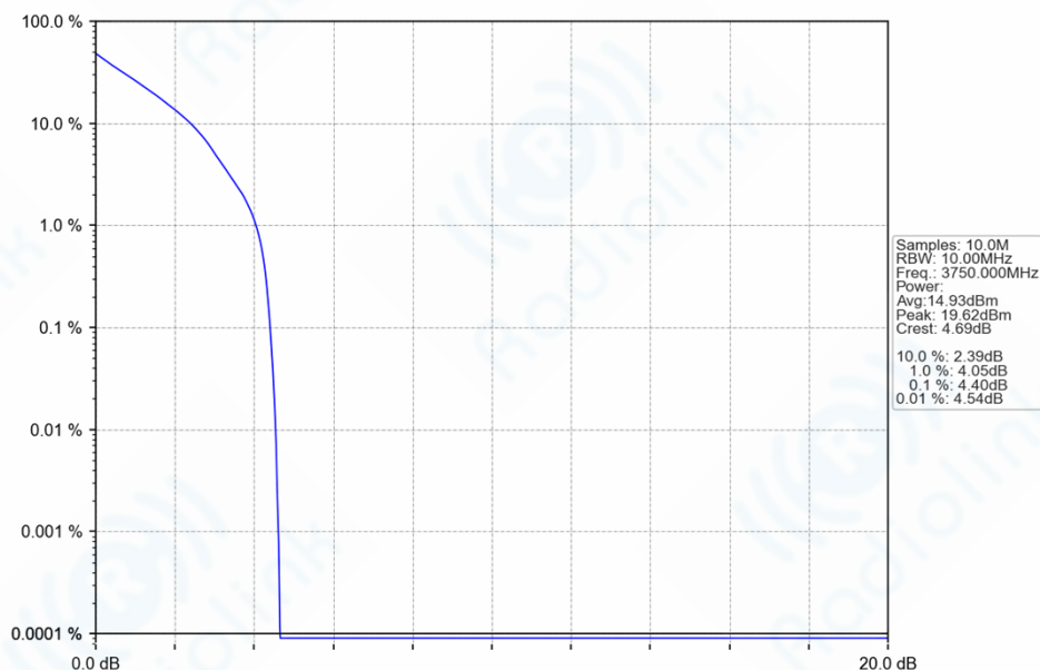
n78a_30kHz_SISO_NTNV_10MHz_DFT-s-OFDM_QPSK_3750MHz_Outer_Full_Ant1
