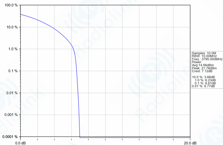
n78a_30kHz_SISO_NTNV_10MHz_CP-OFDM_QPSK_3795MHz_Outer_Full_Ant1
