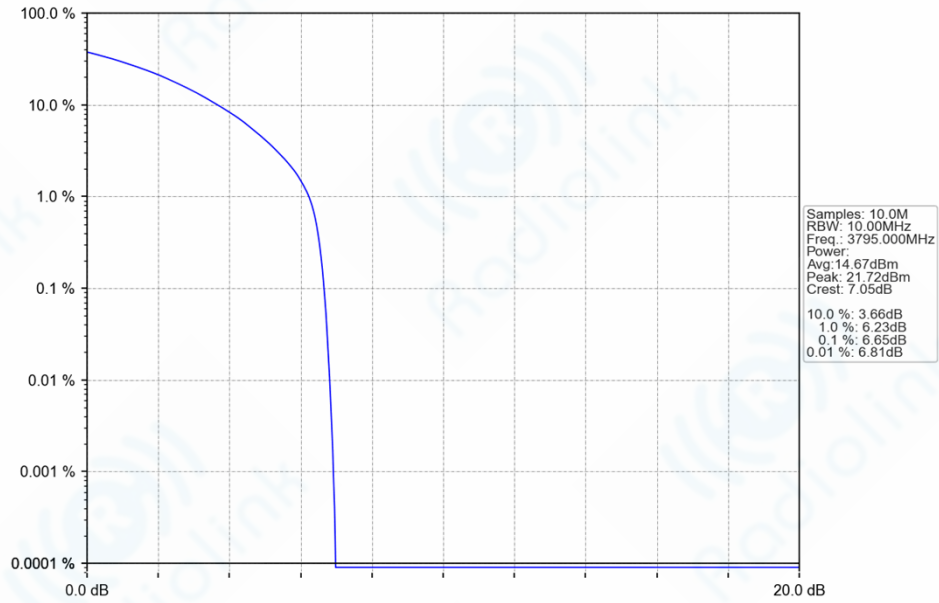
n78a_30kHz_SISO_NTNV_10MHz_CP-OFDM 16 QAM 3795MHz_Outer_Full_Ant1
