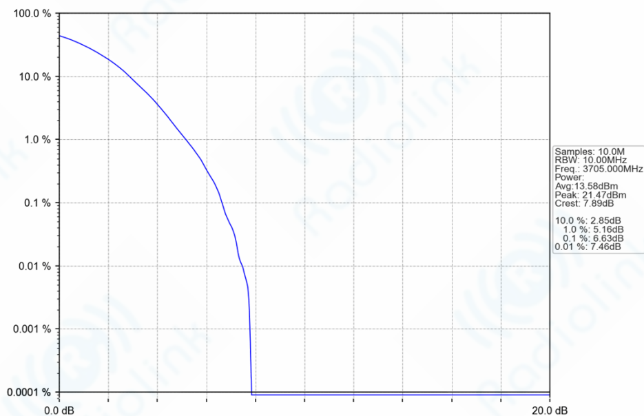
n78a_30kHz_SISO_NTNV_10MHz_DFT-s-OFDM_256_QAM_3705MHz_Outer_Full_Ant1
