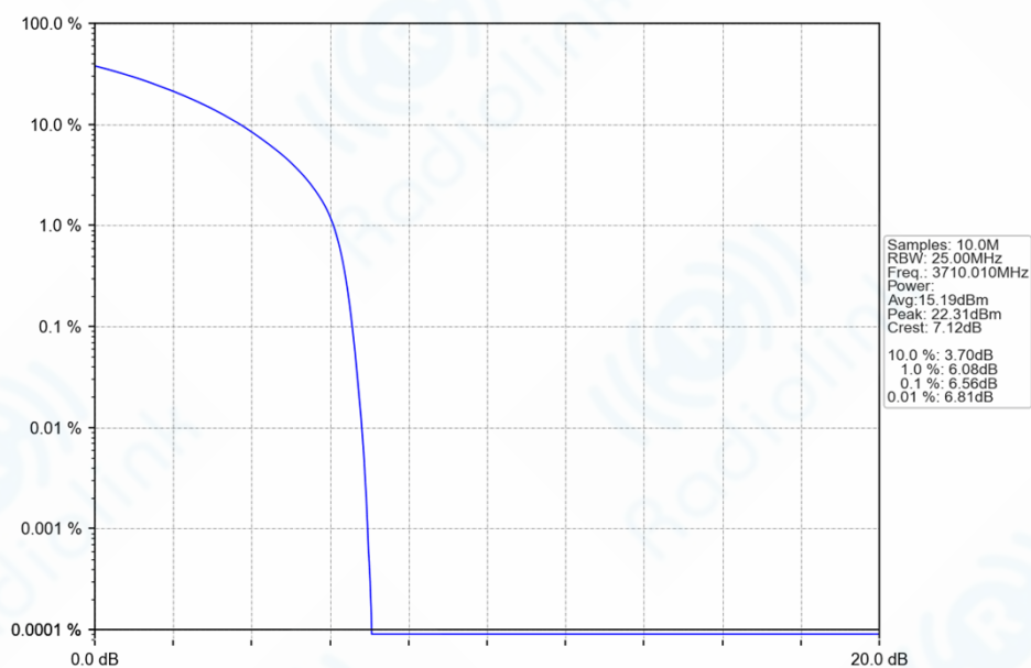
n78a_30kHz_SISO_NTNV_20MHz_CP-OFDM_QPSK_3710.01MHz_Outer_Full_Ant1
