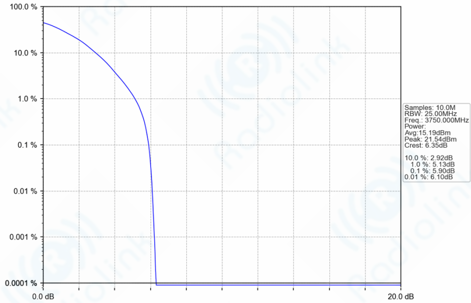
n78a_30kHz_SISO_NTNV_20MHz_DFT-s-OFDM_64_QAM_3750MHz_Outer_Full_Ant1
