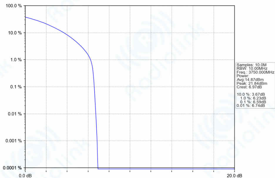
n78a_30kHz_SISO_NTNV_10MHz_CP-OFDM_QPSK_3750MHz_Outer_Full_Ant1
