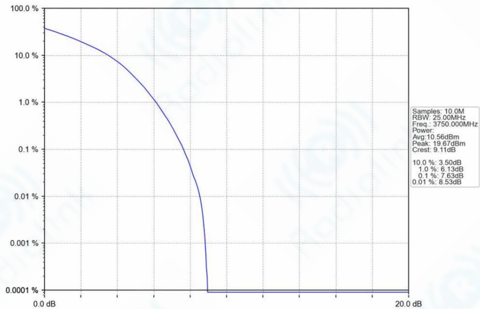
n78a_30kHz_SISO_NTNV_90MHz_DFT-s-OFDM_16_QAM_3750MHz_Outer_Full_Ant1
