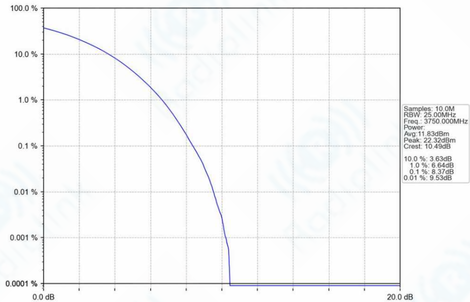
n78a_30kHz_SISO_NTNV_30MHz_CP-OFDM_256_QAM_3750MHz_Outer_Full_Ant1
