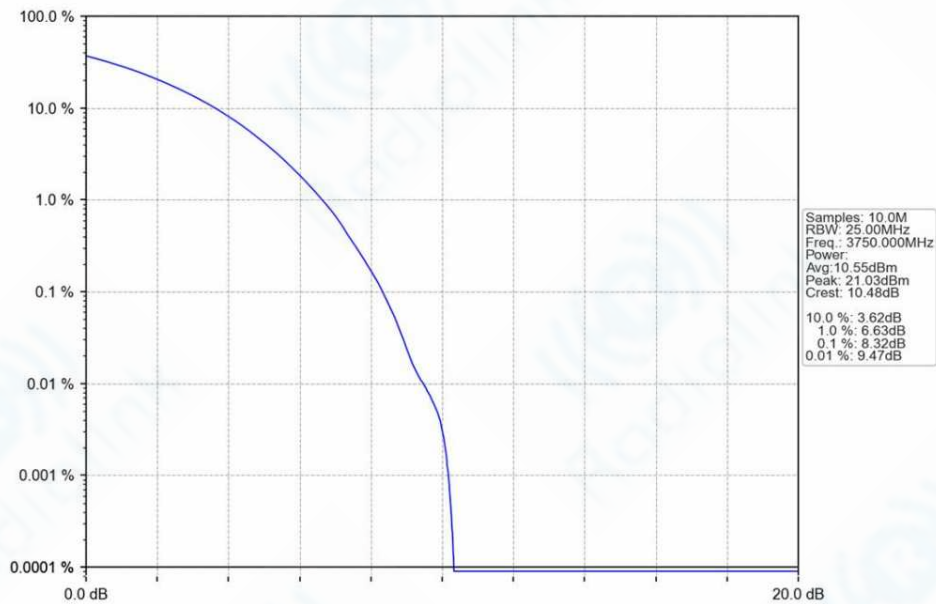
n78a_30kHz_SISO_NTNV_90MHz_CP-OFDM_16_QAM_3750MHz_Outer_Full_Ant1
