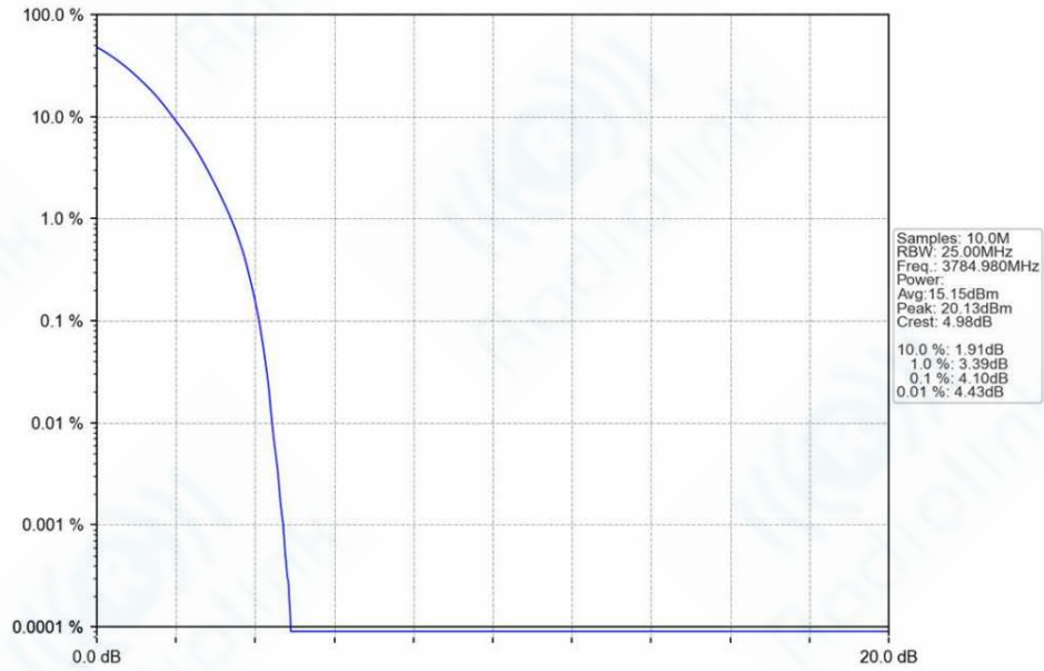
n78a_30kHz_SISO_NTNV_30MHz_DFT-s-OFDM_PI/2_BPSK_3784.98MHz_Outer_Full_Ant1
