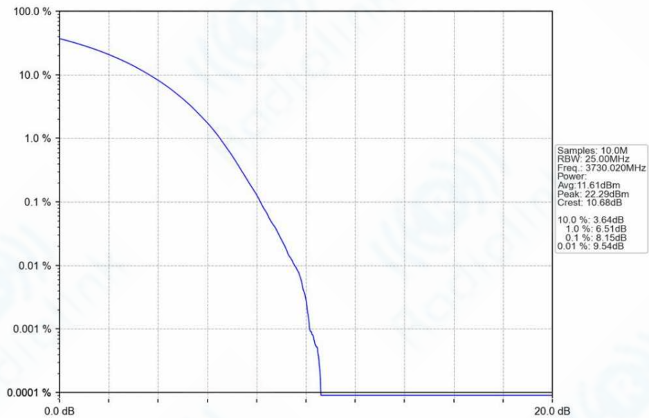
n78a_30kHz_SISO_NTNV_60MHz_CP-OFDM_64_QAM_3730.02MHz_Outer_Full_Ant1
