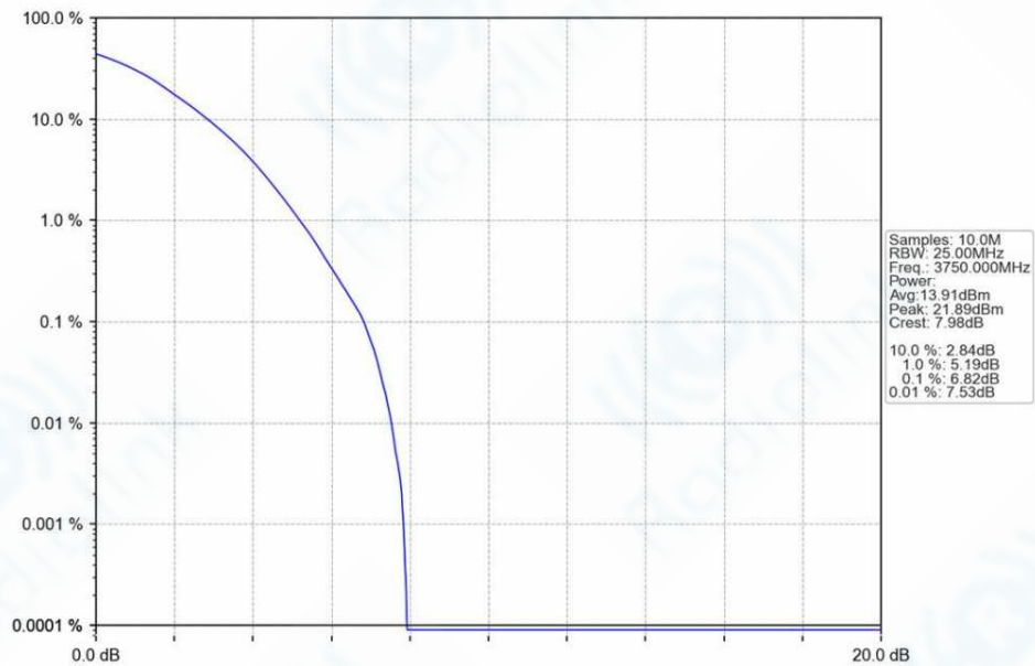
n78a_30kHz_SISO_NTNV_30MHz_DFT-s-OFDM_256_QAM_3750MHz_Outer_Full_Ant1
