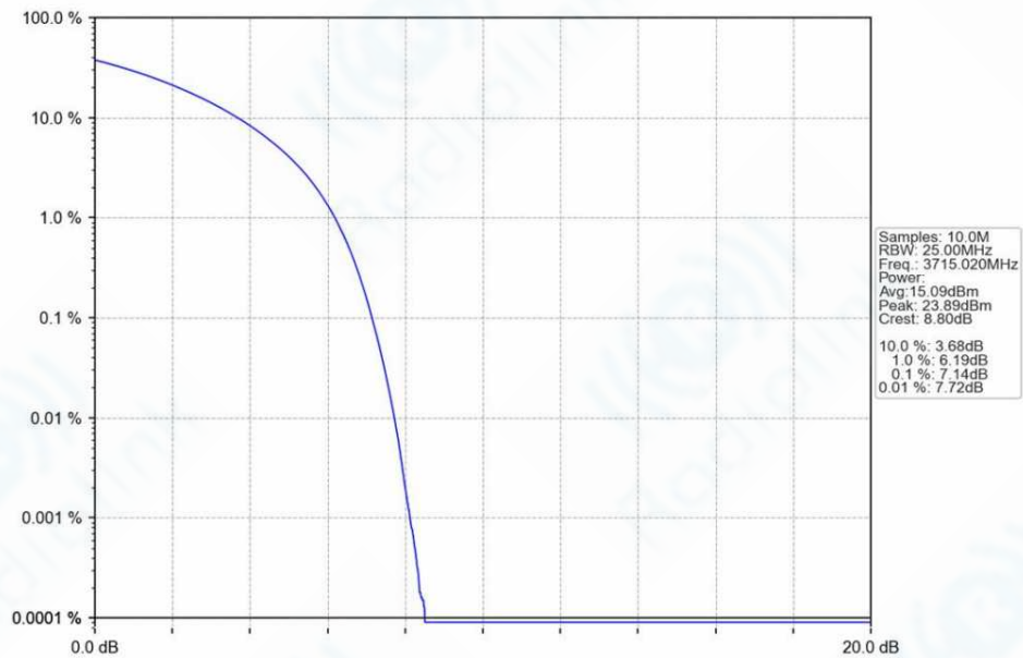
n78a_30kHz_SISO_NTNV_30MHz_CP-OFDM_QPSK_3715.02MHz_Outer_Full_Ant1
