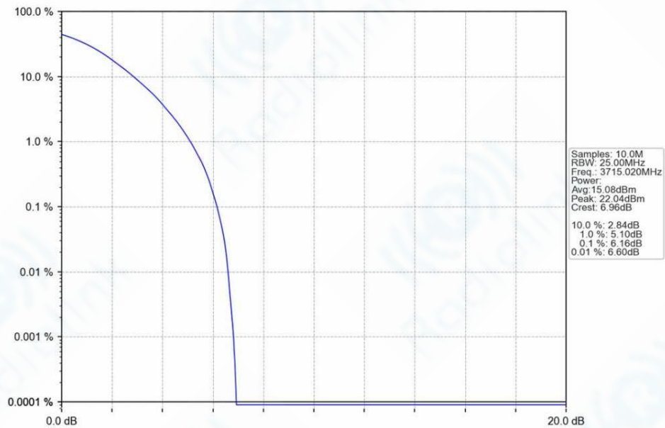
n78a_30kHz_SISO_NTNV_30MHz_DFT-s-OFDM_64_QAM_3715.02MHz_Outer_Full_Ant1
