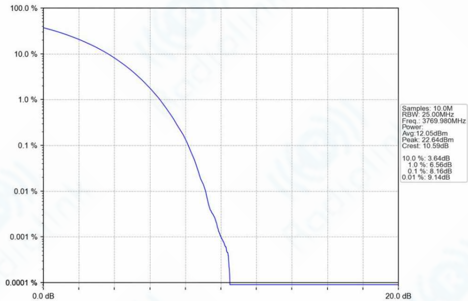
n78a_30kHz_SISO_NTNV_60MHz_CP-OFDM_QPSK_3769.98MHz_Outer_Full_Ant1
