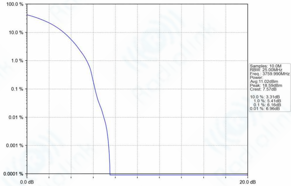
n78a_30kHz_SISO_NTNV_80MHz_DFT-s-OFDM_PI/2_BPSK_3759.99MHz_Outer_Full_Ant1
