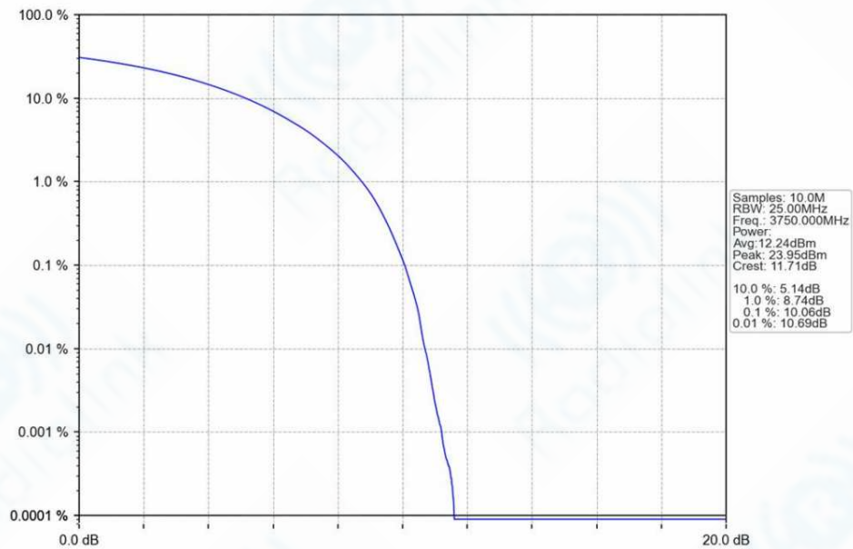
n78a_30kHz_SISO_NTNV_30MHz_CP-OFDM_16_QAM_3750MHz_Outer_Full_Ant1
