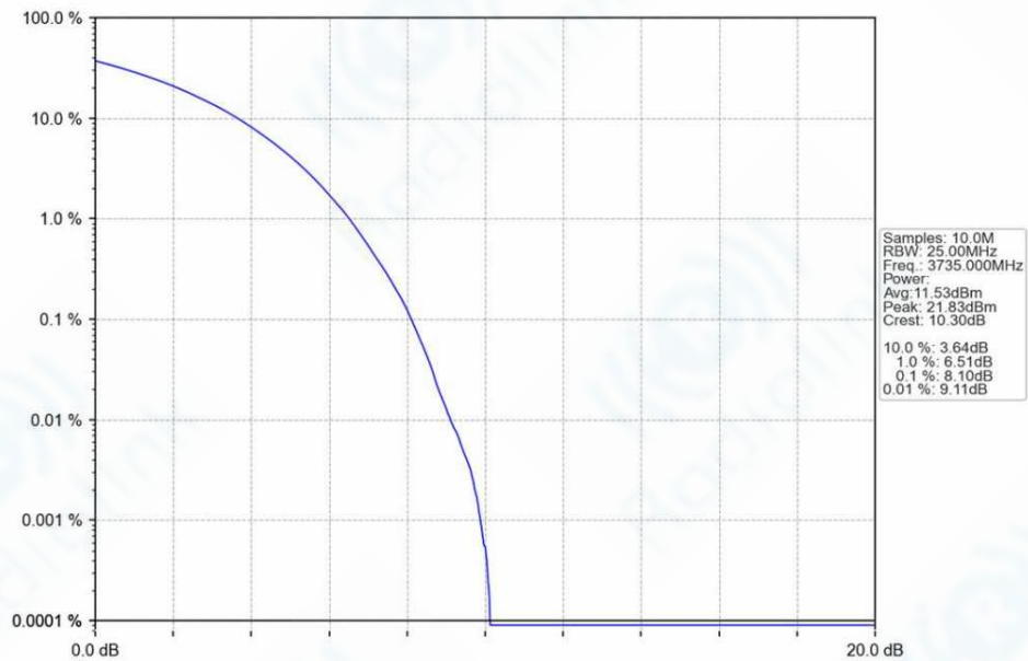
n78a_30kHz_SISO_NTNV_70MHz_CP-OFDM_QPSK_3735MHz_Outer_Full_Ant1
