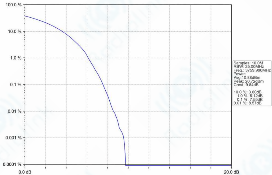
n78a_30kHz_SISO_NTNV_80MHz_DFT-s-OFDM_64_QAM_3759.99MHz_Outer_Full_Ant1
