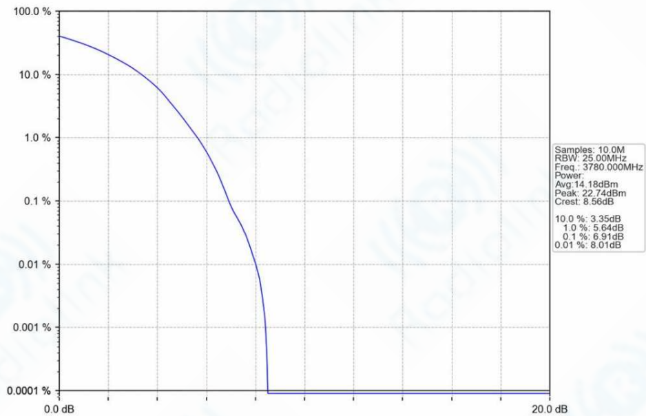
n78a_30kHz_SISO_NTNV_40MHz_DFT-s-OFDM_64_QAM_3780MHz_Outer_Full_Ant1
