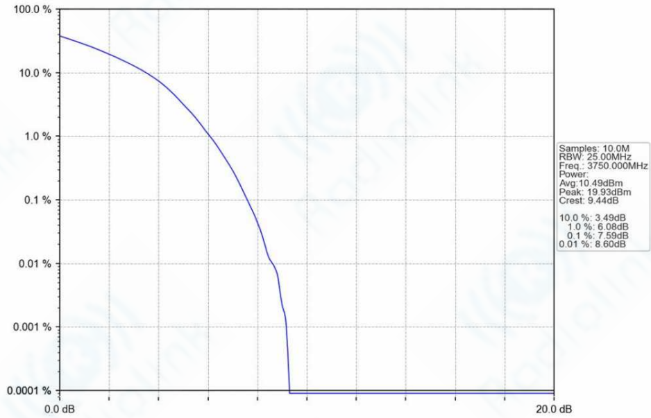
n78a_30kHz_SISO_NTNV_90MHz_DFT-s-OFDM_64_QAM_3750MHz_Outer_Full_Ant1
