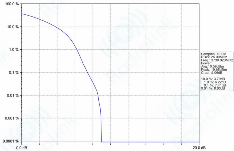
n78a_30kHz_SISO_NTNV_60MHz_DFT-s-OFDM_256_QAM_3730.02MHz_Outer_Full_Ant1
