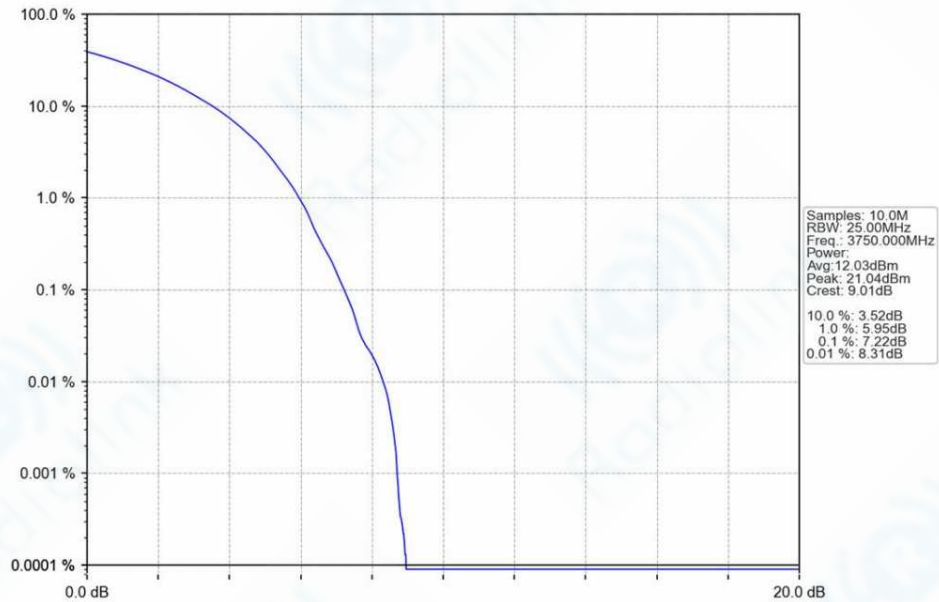
n78a_30kHz_SISO_NTNV_50MHz_DFT-s-OFDM_256_QAM_3750MHz_Outer_Full_Ant1
