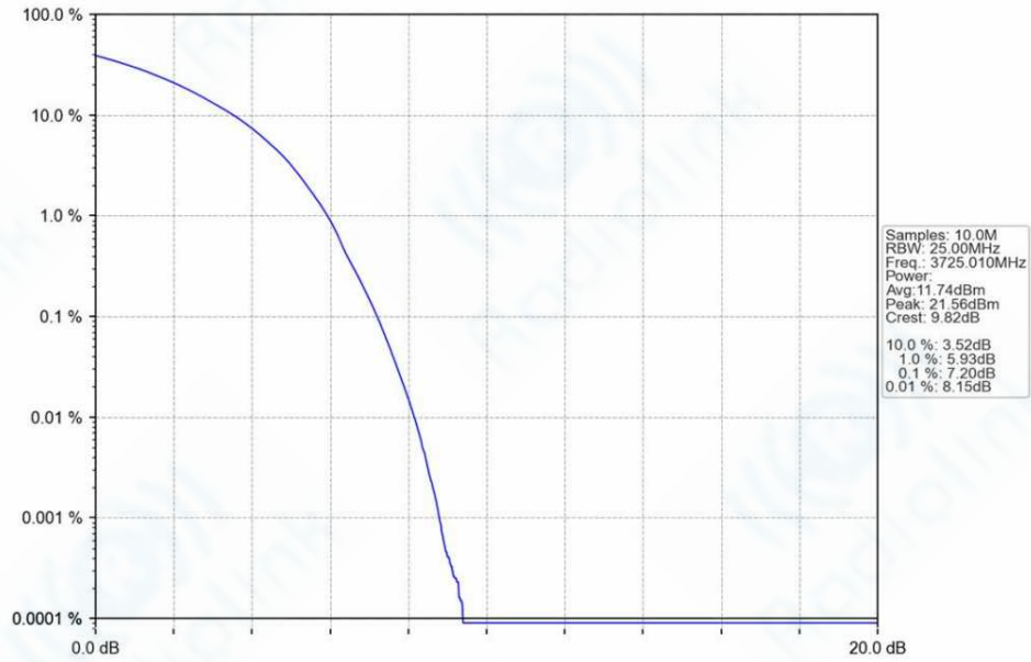
n78a_30kHz_SISO_NTNV_50MHz_DFT-s-OFDM_256_QAM_3725.01MHz_Outer_Full_Ant1
