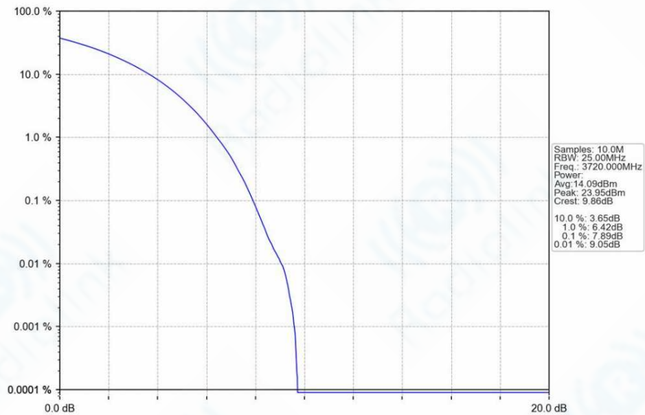
n78a_30kHz_SISO_NTNV_40MHz_CP-OFDM_QPSK_3720MHz_Outer_Full_Ant1
