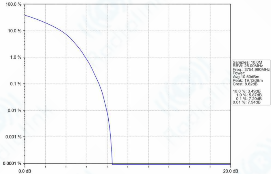
n78a_30kHz_SISO_NTNV_90MHz_DFT-s-OFDM_QPSK_3754.98MHz_Outer_Full_Ant1
