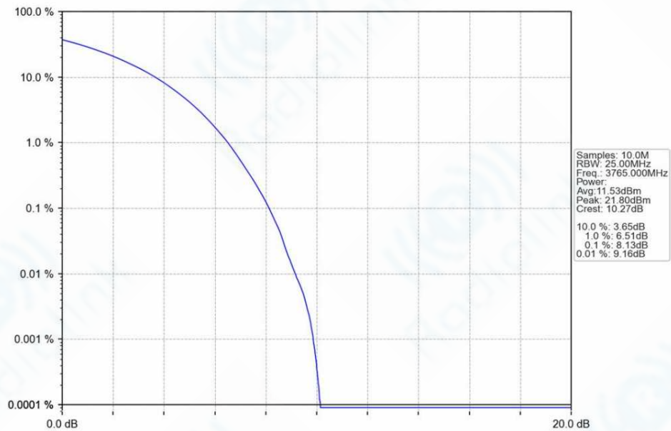
n78a_30kHz_SISO_NTNV_70MHz_CP-OFDM_QPSK_3765MHz_Outer_Full_Ant1
