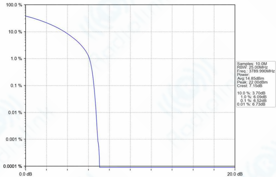
n78a_30kHz_SISO_NTNV_20MHz_CP-OFDM_QPSK_3789.99MHz_Outer_Full_Ant1
