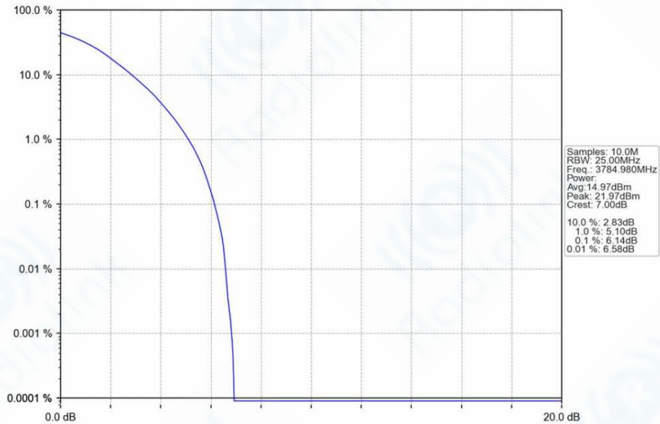
n78a_30kHz_SISO_NTNV_30MHz_DFT-s-OFDM_64_QAM_3784.98MHz_Outer_Full_Ant1
