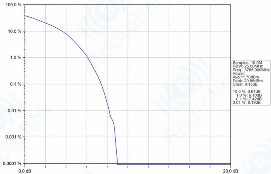
n78a_30kHz_SISO_NTNV_70MHz_DFT-s-OFDM_64_QAM_3765MHz_Outer_Full_Ant1
