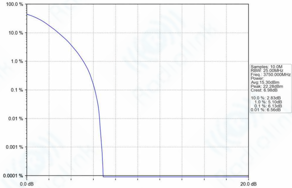
n78a_30kHz_SISO_NTNV_30MHz_DFT-s-OFDM_64_QAM_3750MHz_Outer_Full_Ant1
