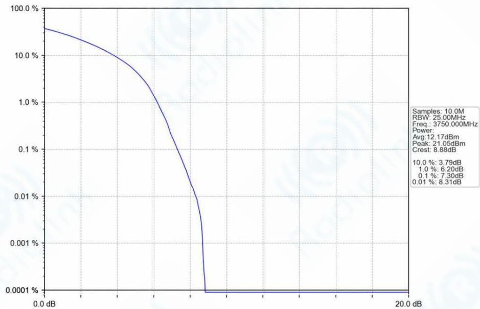
n78a_30kHz_SISO_NTNV_60MHz_DFT-s-OFDM_16_QAM_3750MHz_Outer_Full_Ant1
