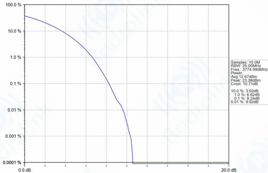
n78a_30kHz_SISO_NTNV_50MHz_CP-OFDM_64_QAM_3774.99MHz_Outer_Full_Ant1
