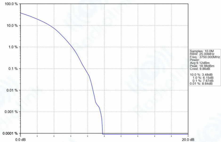
n78a_30kHz_SISO_NTNV_90MHz_DFT-s-OFDM_256_QAM_3750MHz_Outer_Full_Ant1
