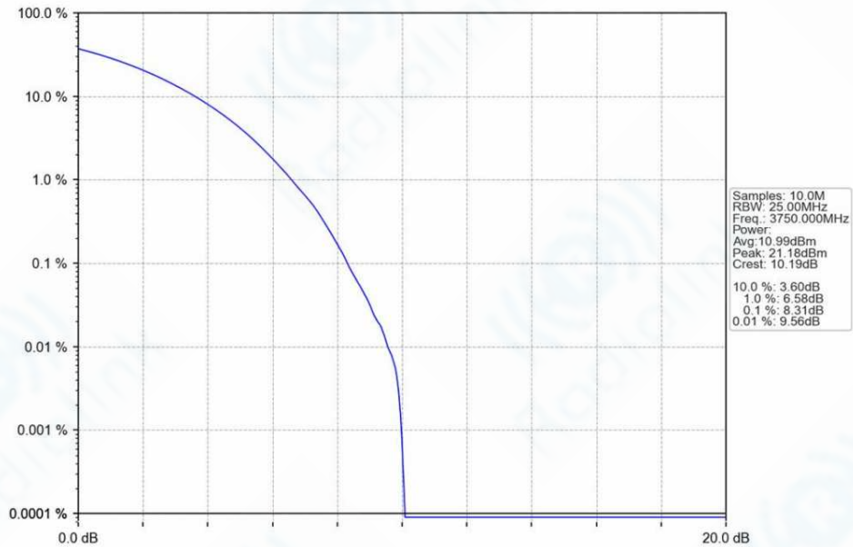
n78a_30kHz_SISO_NTNV_80MHz_CP-OFDM_16_QAM_3750MHz_Outer_Full_Ant1
