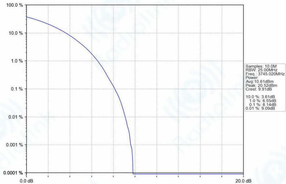
n78a_30kHz_SISO_NTNV_90MHz_CP-OFDM_QPSK_3745.02MHz_Outer_Full_Ant1
