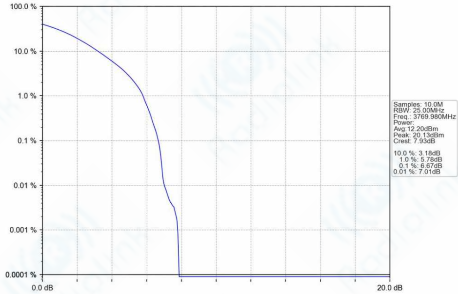
n78a_30kHz_SISO_NTNV_60MHz_DFT-s-OFDM_PI/2_BPSK_3769.98MHz_Outer_Full_Ant1
