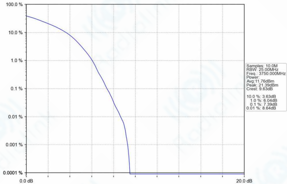
n78a_30kHz_SISO_NTNV_70MHz_DFT-s-OFDM_16_QAM_3750MHz_Outer_Full_Ant1
