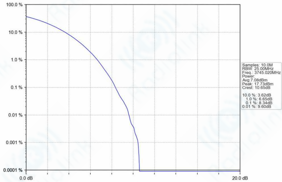
n78a_30kHz_SISO_NTNV_90MHz_CP-OFDM_256_QAM_3745.02MHz_Outer_Full_Ant1
