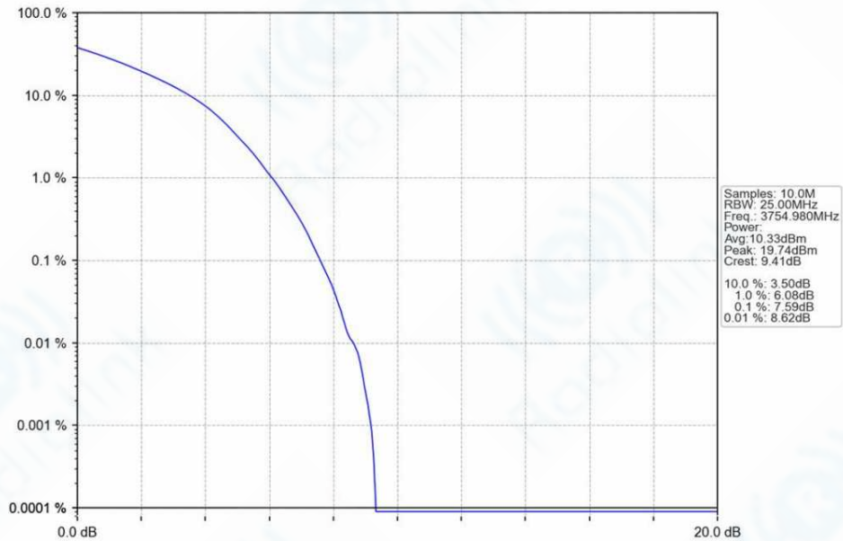
n78a_30kHz_SISO_NTNV_90MHz_DFT-s-OFDM_64_QAM_3754.98MHz_Outer_Full_Ant1
