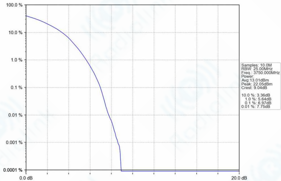
n78a_30kHz_SISO_NTNV_40MHz_DFT-s-OFDM_256_QAM_3750MHz_Outer_Full_Ant1
