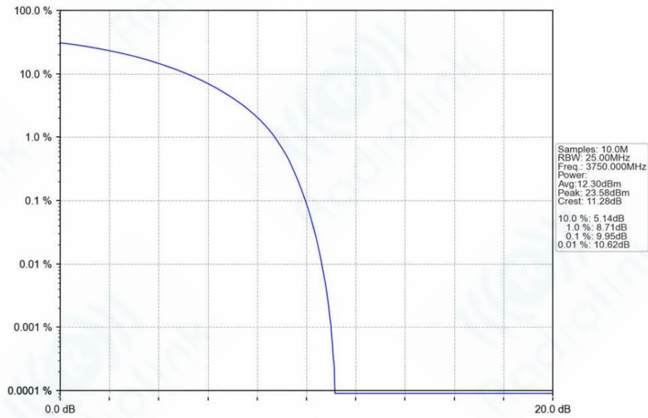
n78a_30kHz_SISO_NTNV_30MHz_CP-OFDM_QPSK_3750MHz_Outer_Full_Ant1
