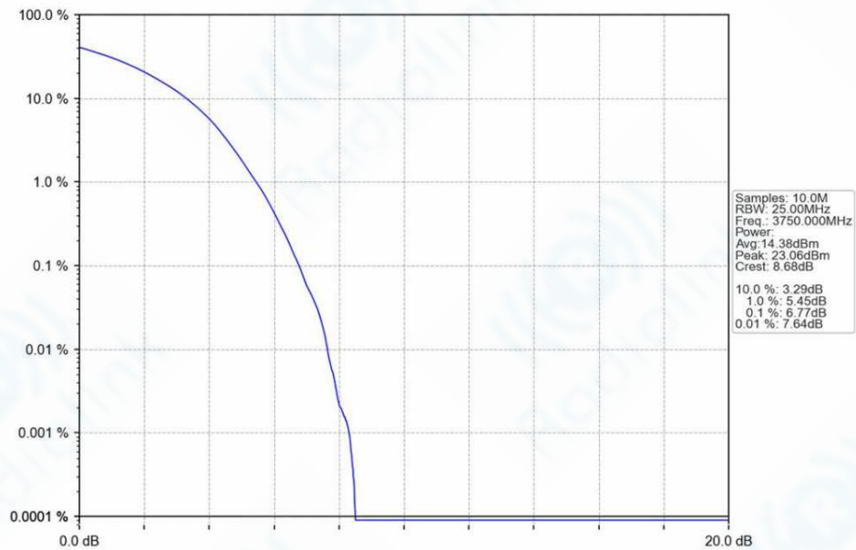
n78a_30kHz_SISO_NTNV_40MHz_DFT-s-OFDM_16_QAM_3750MHz_Outer_Full_Ant1
