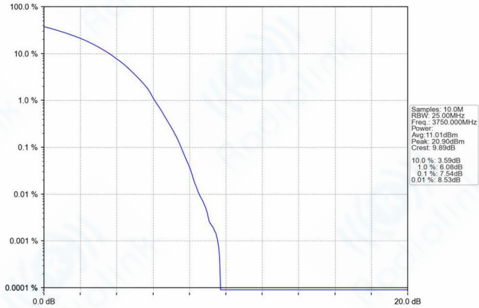
n78a_30kHz_SISO_NTNV_80MHz_DFT-s-OFDM_64_QAM_3750MHz_Outer_Full_Ant1
