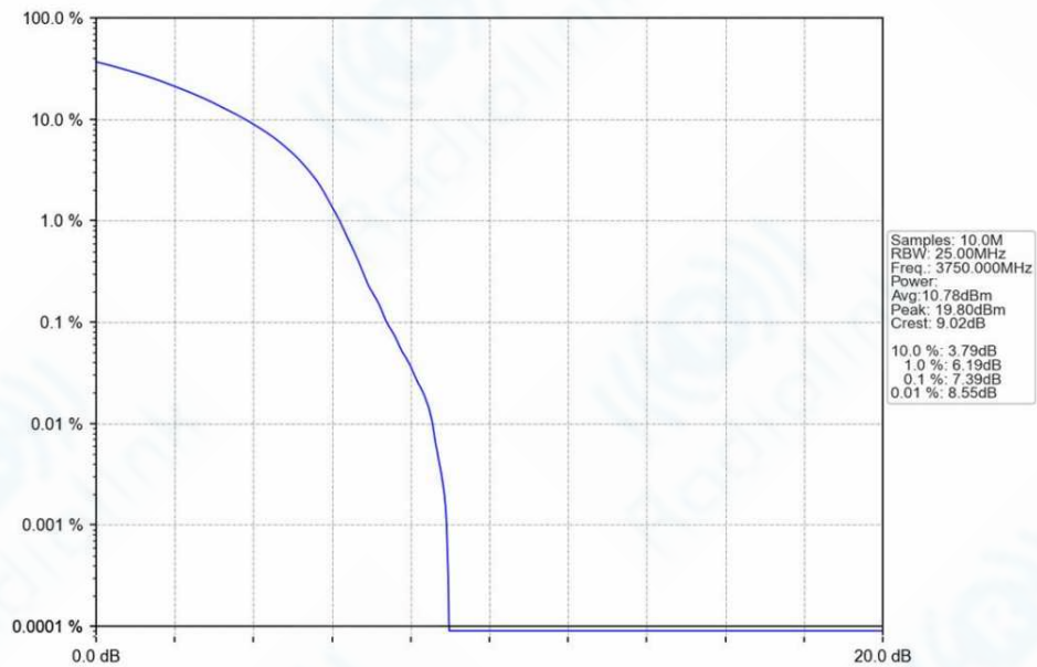
n78a_30kHz_SISO_NTNV_60MHz_DFT-s-OFDM_256_QAM_3750MHz_Outer_Full_Ant1
