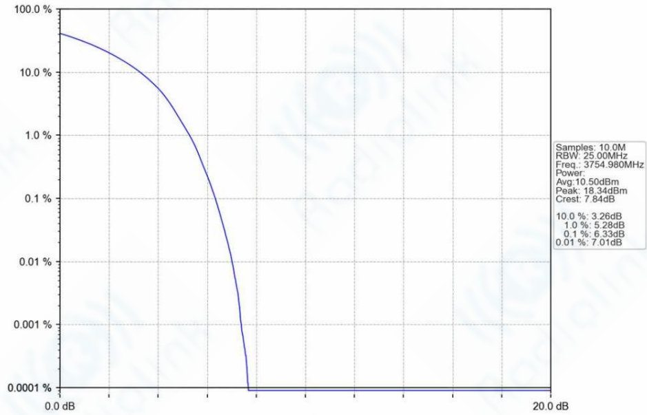
n78a_30kHz_SISO_NTNV_90MHz_DFT-s-OFDM_PI/2_BPSK_3754.98MHz_Outer_Full_Ant1
