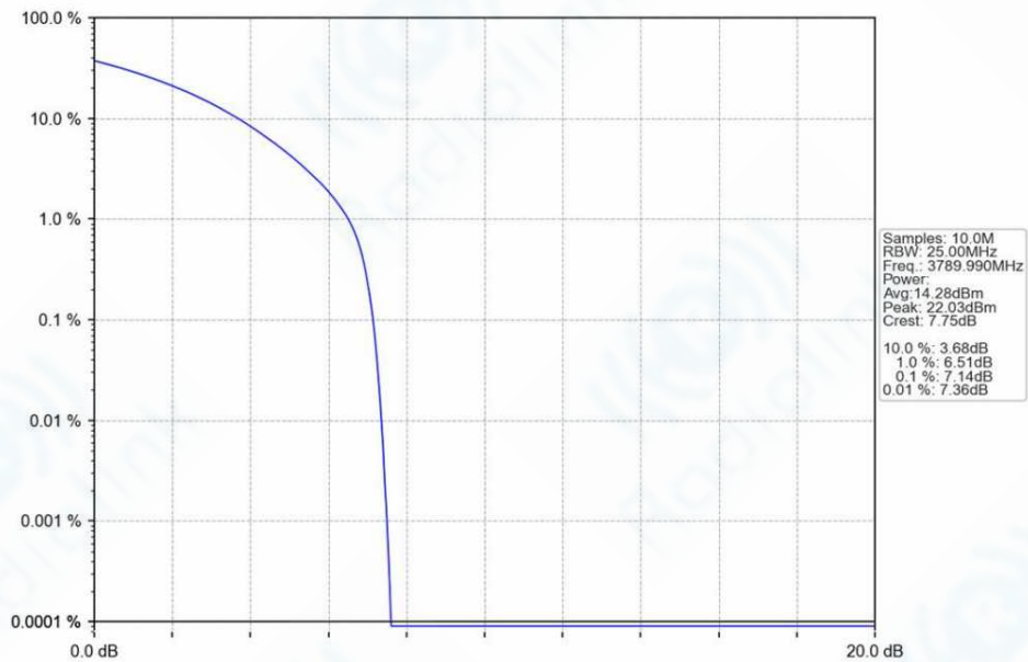
n78a_30kHz_SISO_NTNV_20MHz_CP-OFDM_64_QAM_3789.99MHz_Outer_Full_Ant1
