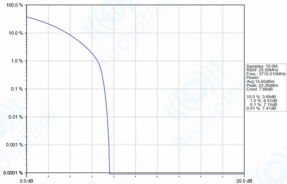
n78a_30kHz_SISO_NTNV_20MHz_CP-OFDM_64_QAM_3710.01MHz_Outer_Full_Ant1
