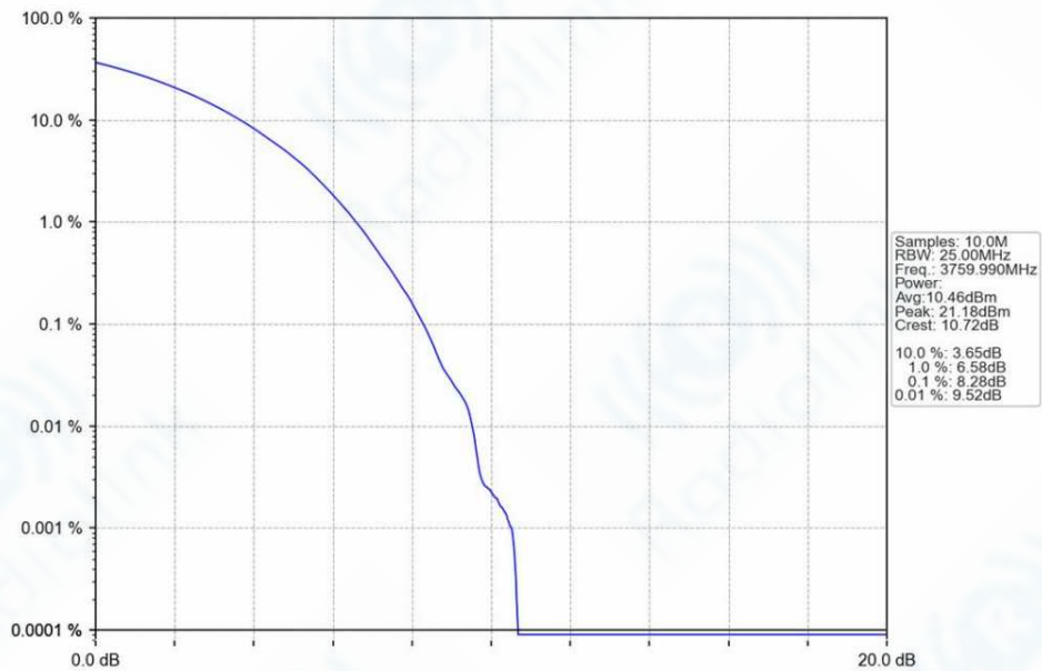
n78a_30kHz_SISO_NTNV_80MHz_CP-OFDM_64_QAM_3759.99MHz_Outer_Full_Ant1
