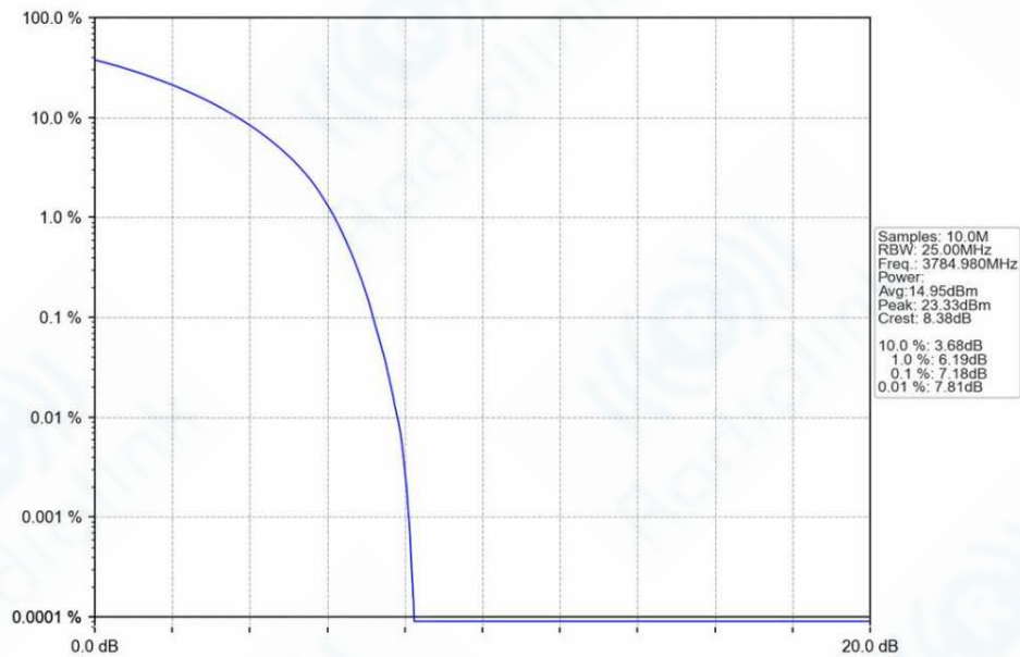
n78a_30kHz_SISO_NTNV_30MHz_CP-OFDM_QPSK_3784.98MHz_Outer_Full_Ant1
