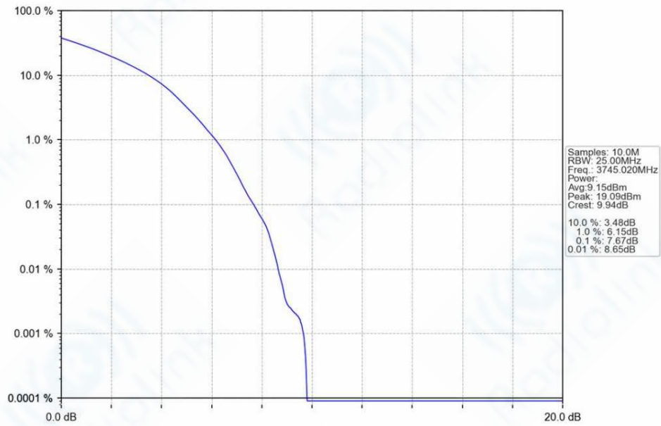
n78a_30kHz_SISO_NTNV_90MHz_DFT-s-OFDM_256_QAM_3745.02MHz_Outer_Full_Ant1
