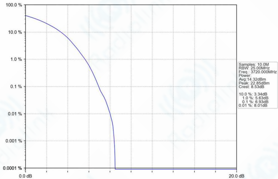
n78a_30kHz_SISO_NTNV_40MHz_DFT-s-OFDM_64_QAM_3720MHz_Outer_Full_Ant1
