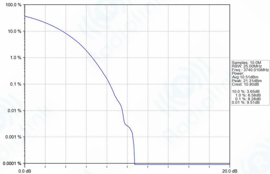
n78a_30kHz_SISO_NTNV_80MHz_CP-OFDM_64_QAM_3740.01MHz_Outer_Full_Ant1
