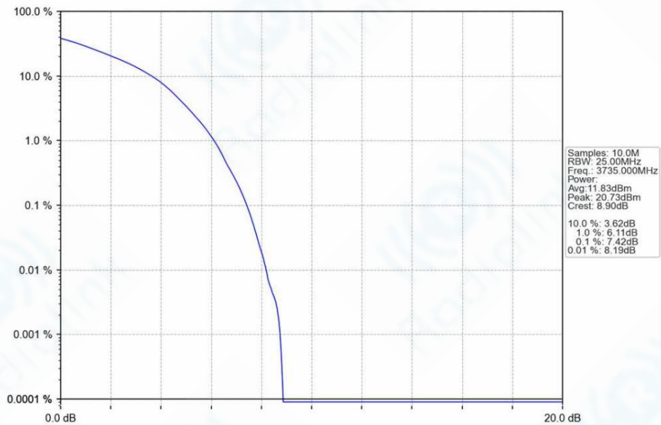
n78a_30kHz_SISO_NTNV_70MHz_DFT-s-OFDM_64_QAM_3735MHz_Outer_Full_Ant1
