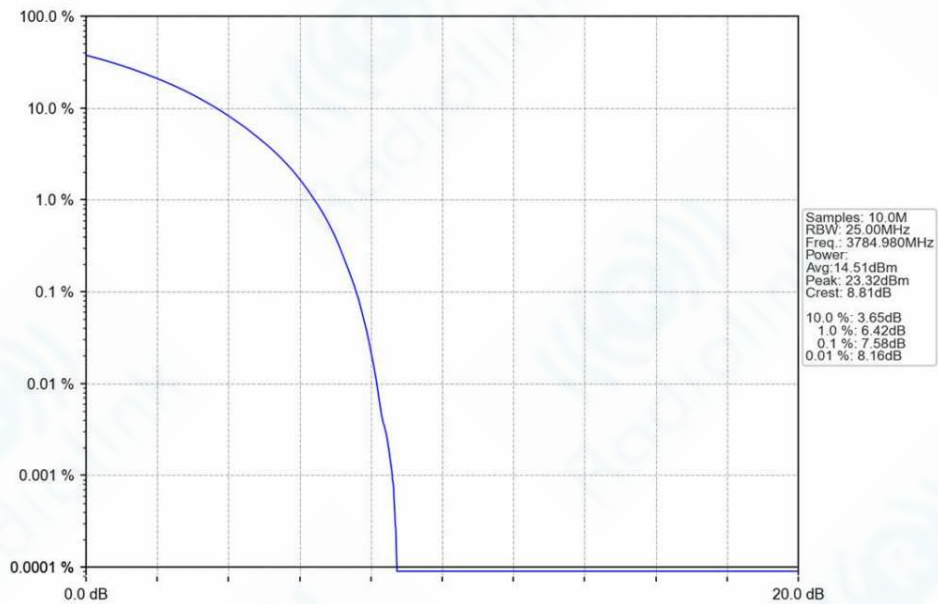
n78a_30kHz_SISO_NTNV_30MHz_CP-OFDM_64_QAM_3784.98MHz_Outer_Full_Ant1
