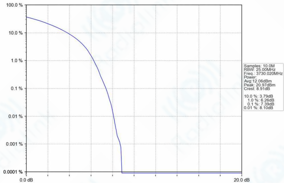
n78a_30kHz_SISO_NTNV_60MHz_DFT-s-OFDM_64_QAM_3730.02MHz_Outer_Full_Ant1
