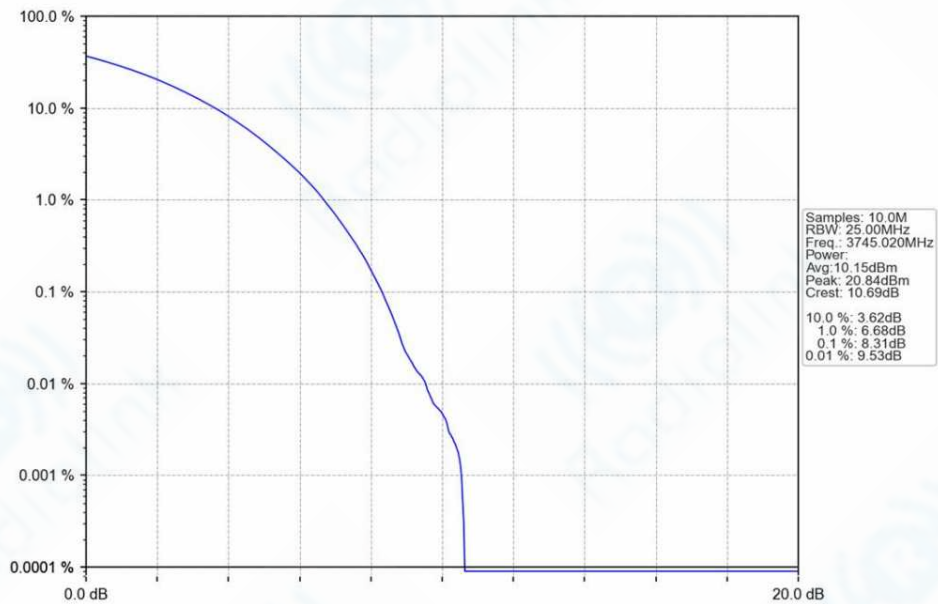
n78a_30kHz_SISO_NTNV_90MHz_CP-OFDM_64_QAM_3745.02MHz_Outer_Full_Ant1
