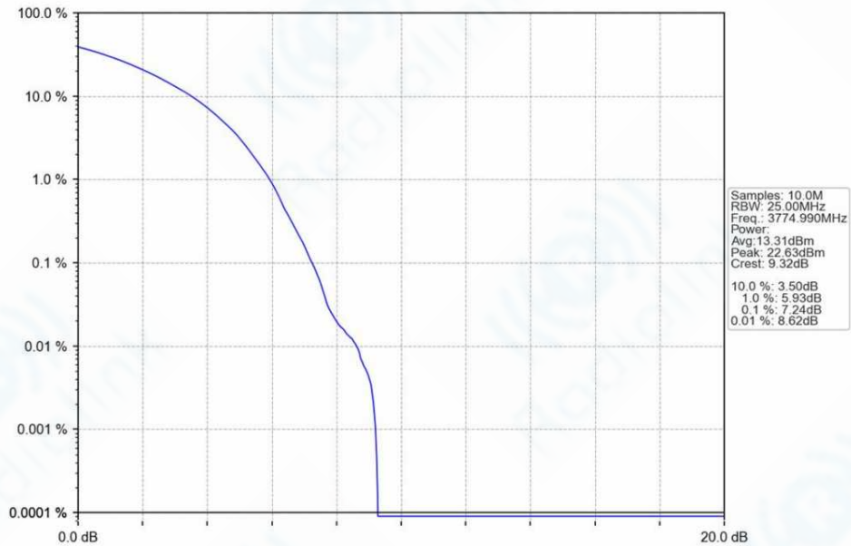
n78a_30kHz_SISO_NTNV_50MHz_DFT-s-OFDM_64_QAM_3774.99MHz_Outer_Full_Ant1
