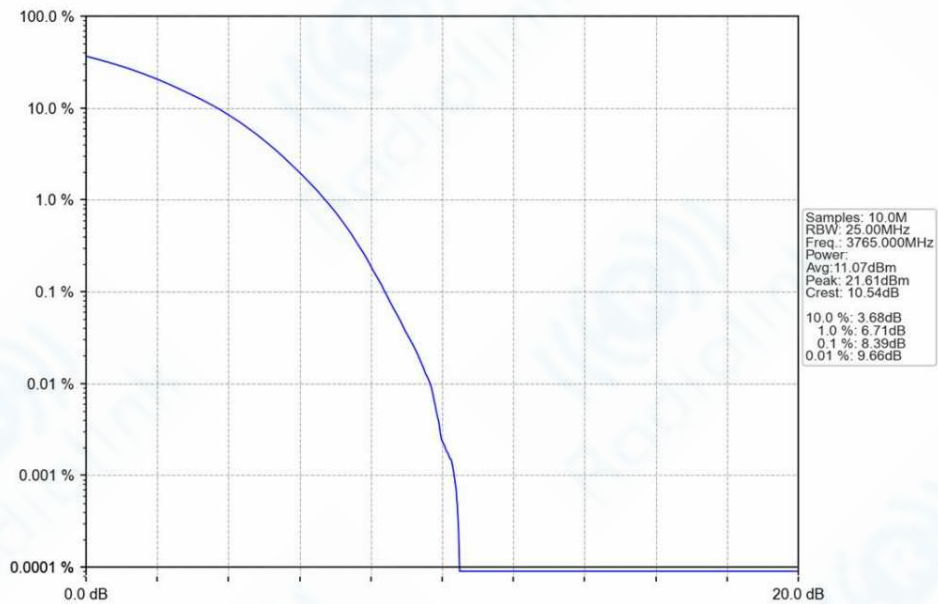
n78a_30kHz_SISO_NTNV_70MHz_CP-OFDM_64_QAM_3765MHz_Outer_Full_Ant1
