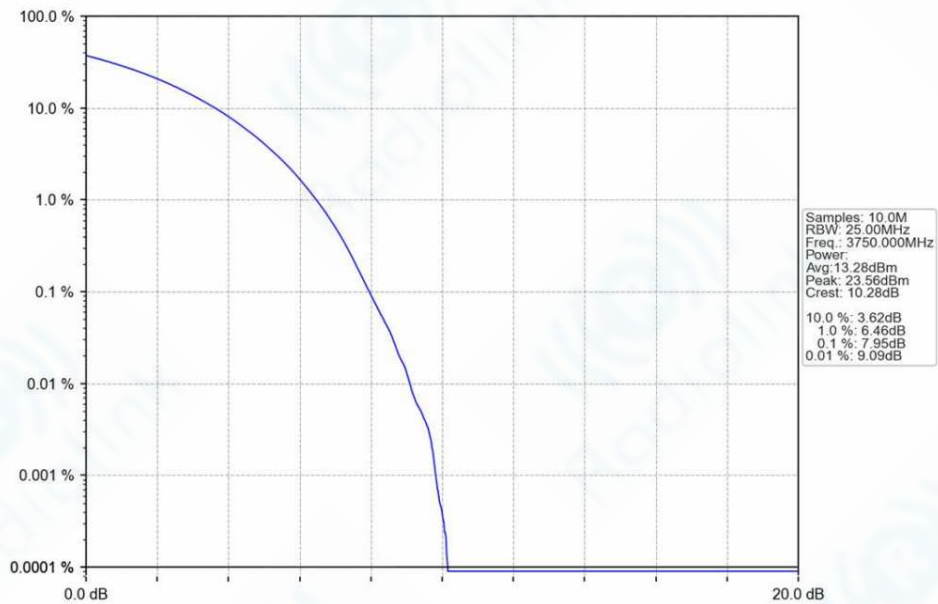
n78a_30kHz_SISO_NTNV_50MHz_CP-OFDM_16_QAM_3750MHz_Outer_Full_Ant1
