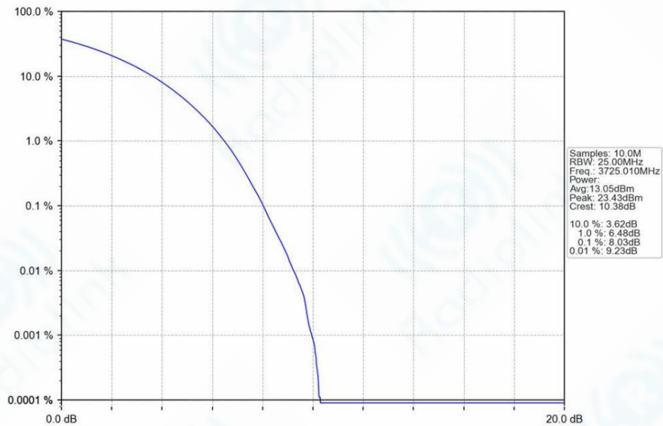
n78a_30kHz_SISO_NTNV_50MHz_CP-OFDM_QPSK_3725.01MHz_Outer_Full_Ant1
