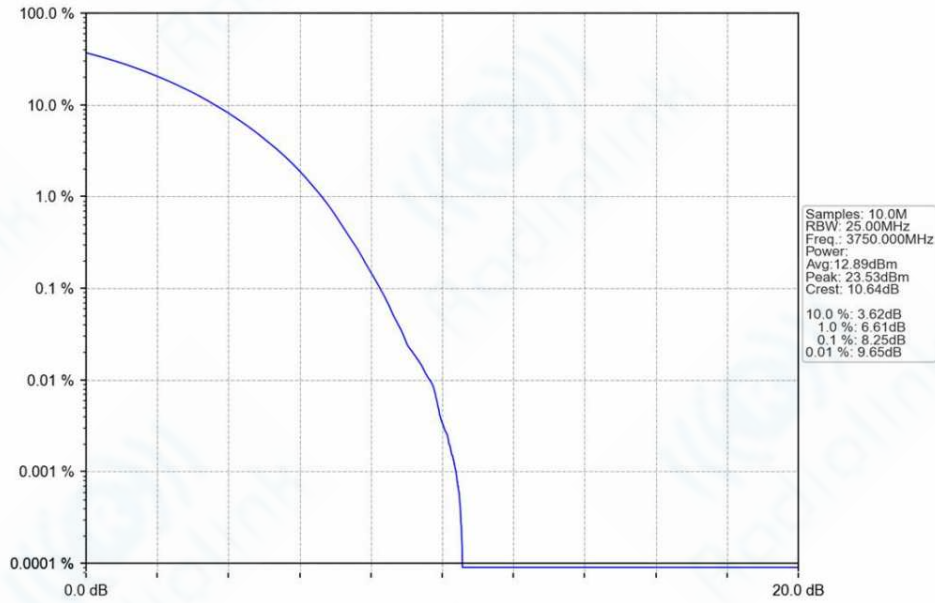
n78a_30kHz_SISO_NTNV_50MHz_CP-OFDM_64_QAM_3750MHz_Outer_Full_Ant1
