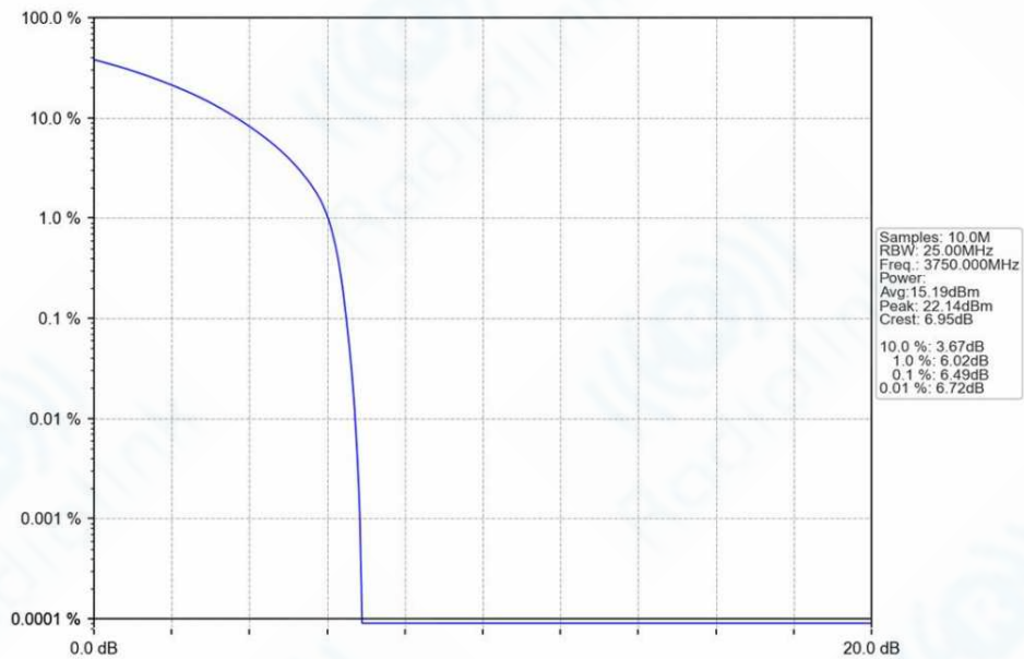
n78a_30kHz_SISO_NTNV_20MHz_CP-OFDM_16_QAM_3750MHz_Outer_Full_Ant1
