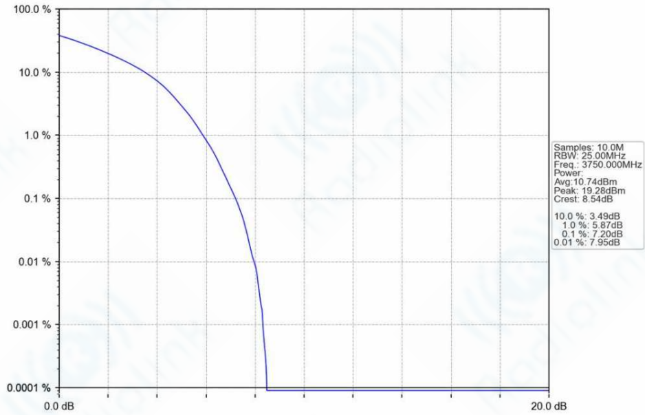
n78a_30kHz_SISO_NTNV_90MHz_DFT-s-OFDM_QPSK_3750MHz_Outer_Full_Ant1
