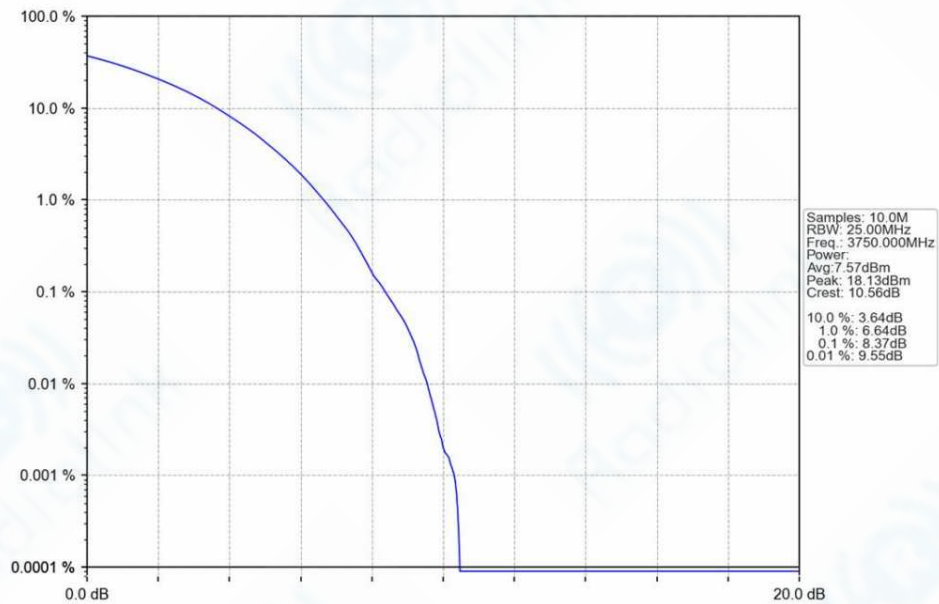
n78a_30kHz_SISO_NTNV_80MHz_CP-OFDM_256_QAM_3750MHz_Outer_Full_Ant1
