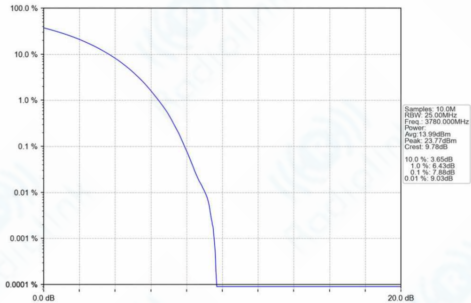
n78a_30kHz_SISO_NTNV_40MHz_CP-OFDM_QPSK_3780MHz_Outer_Full_Ant1
