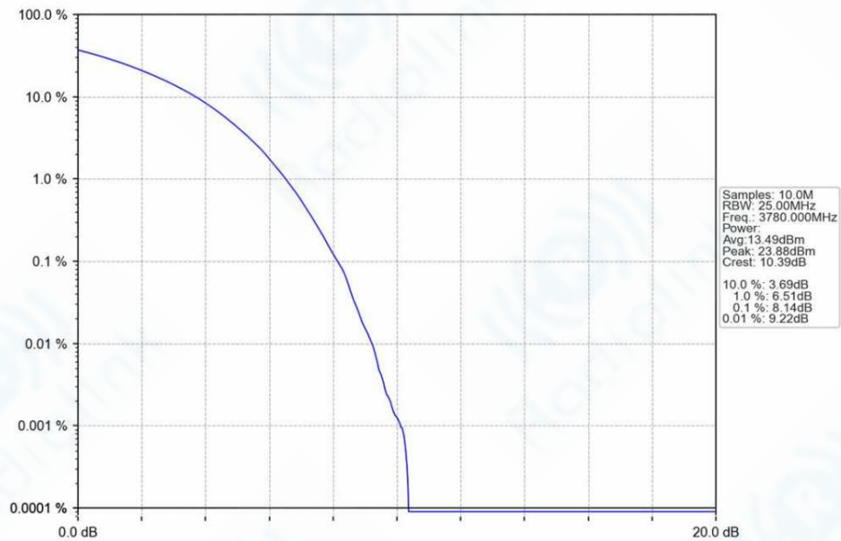
n78a_30kHz_SISO_NTNV_40MHz_CP-OFDM_64_QAM_3780MHz_Outer_Full_Ant1
