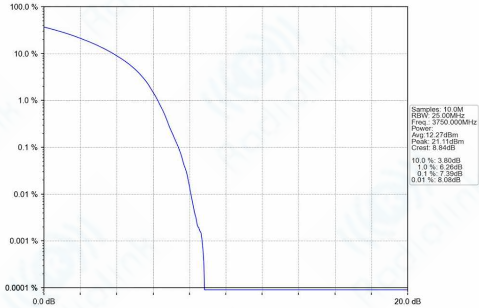
n78a_30kHz_SISO_NTNV_60MHz_DFT-s-OFDM_64_QAM_3750MHz_Outer_Full_Ant1
