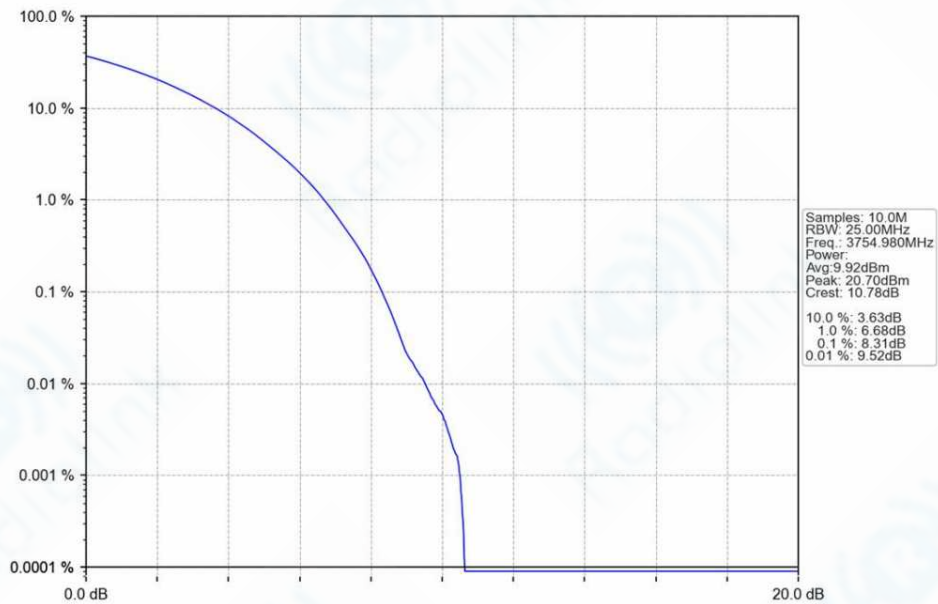
n78a_30kHz_SISO_NTNV_90MHz_CP-OFDM_64_QAM_3754.98MHz_Outer_Full_Ant1
