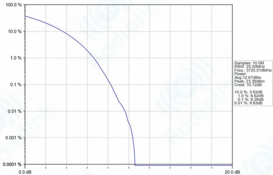
n78a_30kHz_SISO_NTNV_50MHz_CP-OFDM_64_QAM_3725.01MHz_Outer_Full_Ant1
