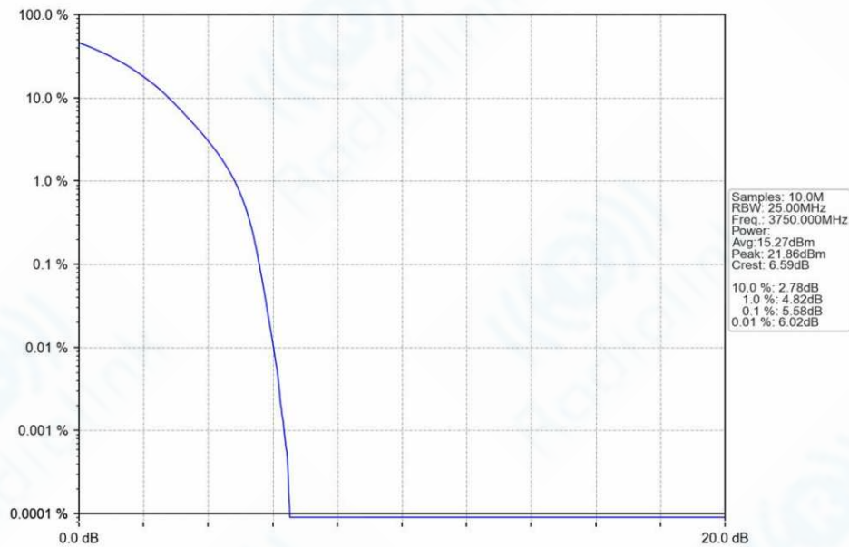
n78a_30kHz_SISO_NTNV_30MHz_DFT-s-OFDM_16_QAM_3750MHz_Outer_Full_Ant1
