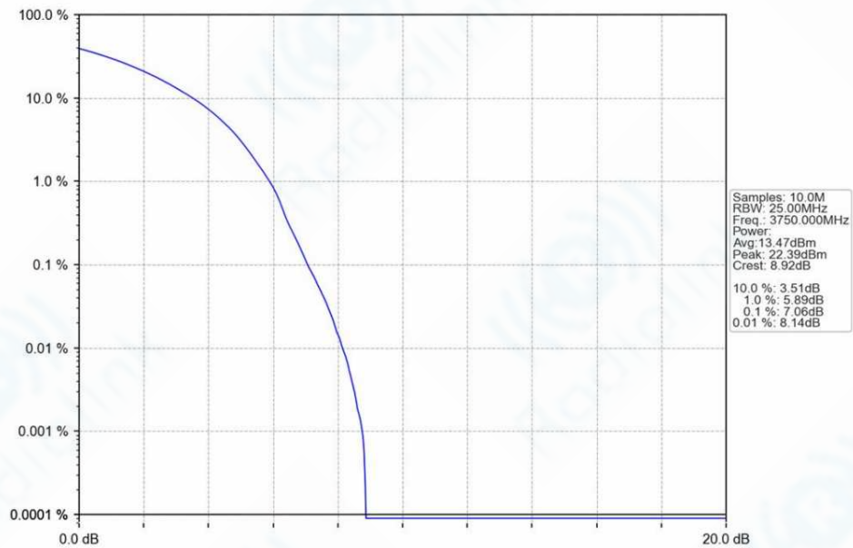
n78a_30kHz_SISO_NTNV_50MHz_DFT-s-OFDM_16_QAM_3750MHz_Outer_Full_Ant1
