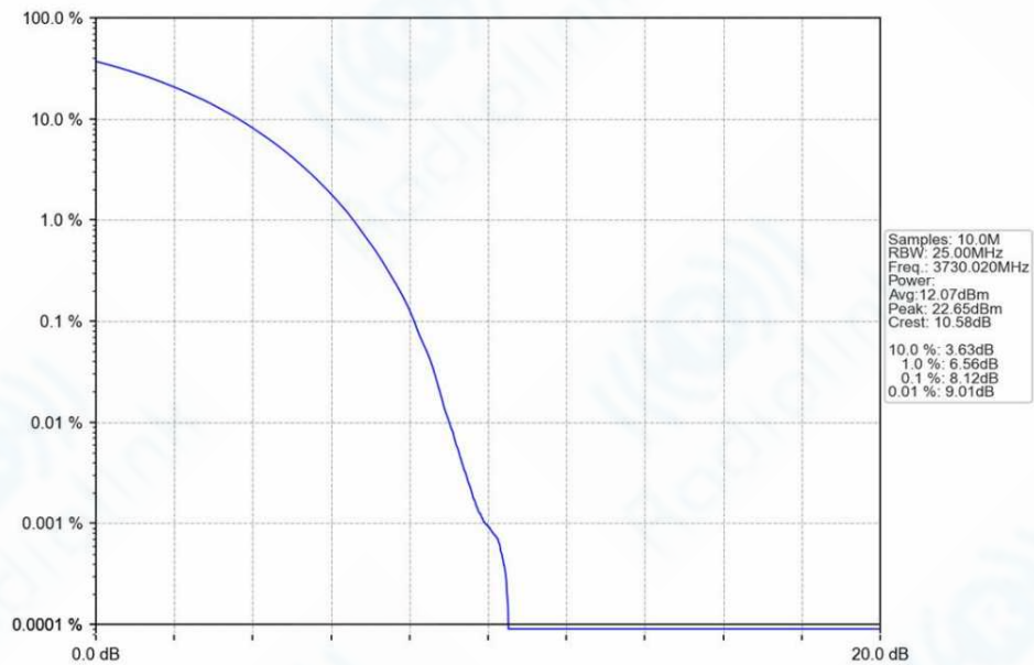
n78a_30kHz_SISO_NTNV_60MHz_CP-OFDM_QPSK_3730.02MHz_Outer_Full_Ant1
