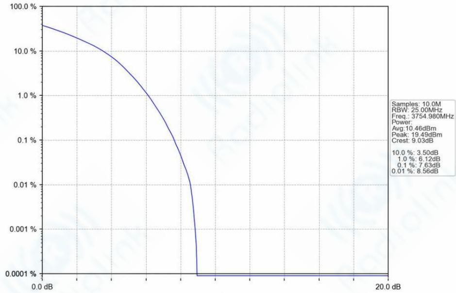
n78a_30kHz_SISO_NTNV_90MHz_DFT-s-OFDM_16_QAM_3754.98MHz_Outer_Full_Ant1
