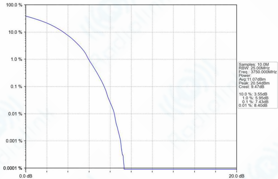
n78a_30kHz_SISO_NTNV_80MHz_DFT-s-OFDM_16_QAM_3750MHz_Outer_Full_Ant1
