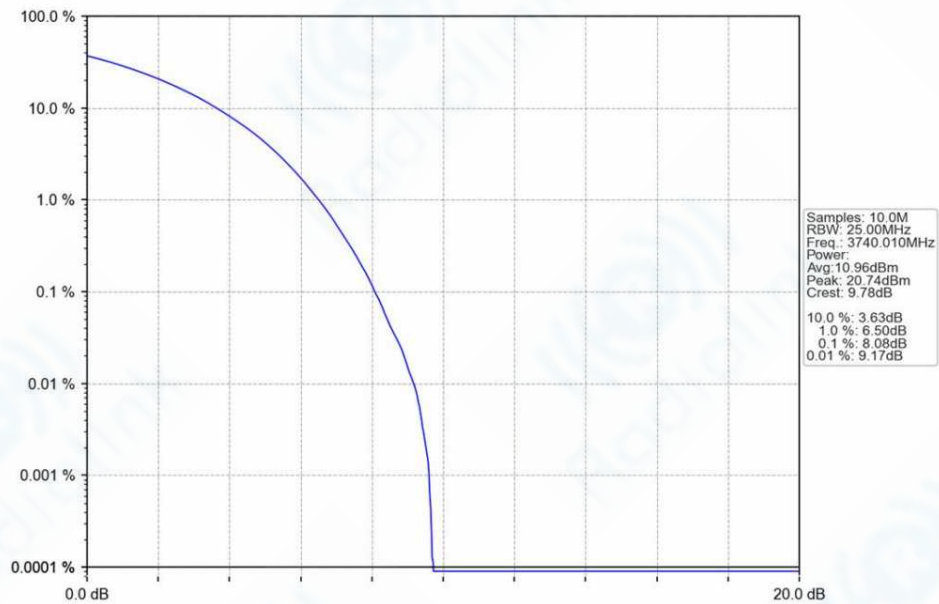
n78a_30kHz_SISO_NTNV_80MHz_CP-OFDM_QPSK_3740.01MHz_Outer_Full_Ant1
