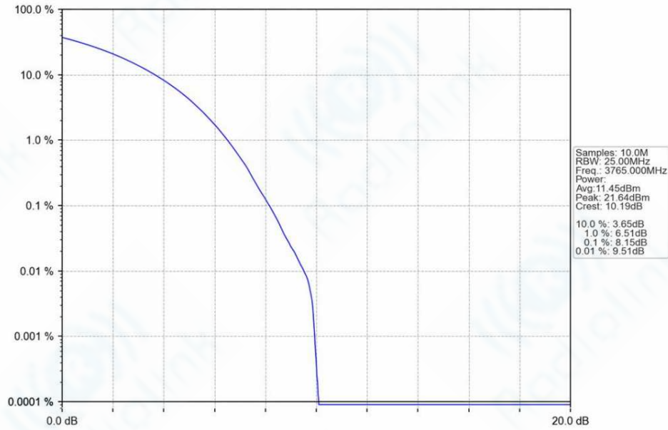
n78a_30kHz_SISO_NTNV_70MHz_CP-OFDM 16 QAM 3765MHz_Outer_Full_Ant1
