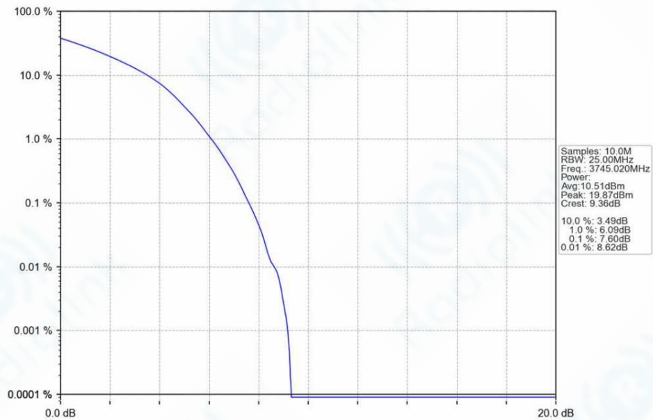
n78a_30kHz_SISO_NTNV_90MHz_DFT-s-OFDM_64_QAM_3745.02MHz_Outer_Full_Ant1
