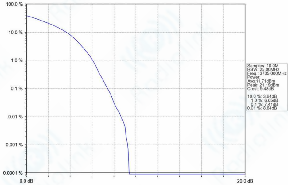
n78a_30kHz_SISO_NTNV_70MHz_DFT-s-OFDM_16_QAM_3735MHz_Outer_Full_Ant1
