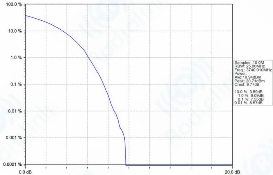
n78a_30kHz_SISO_NTNV_80MHz_DFT-s-OFDM_64_QAM_3740.01MHz_Outer_Full_Ant1
