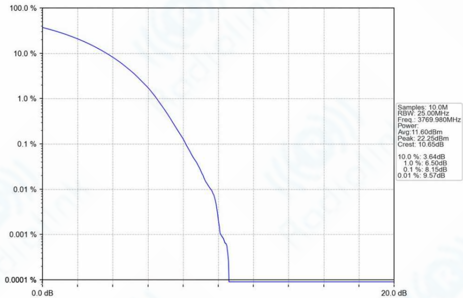
n78a_30kHz_SISO_NTNV_60MHz_CP-OFDM_64_QAM_3769.98MHz_Outer_Full_Ant1
