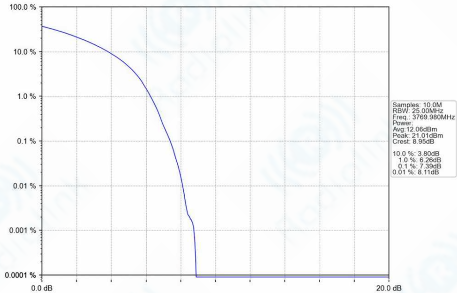
n78a_30kHz_SISO_NTNV_60MHz_DFT-s-OFDM_64_QAM_3769.98MHz_Outer_Full_Ant1
