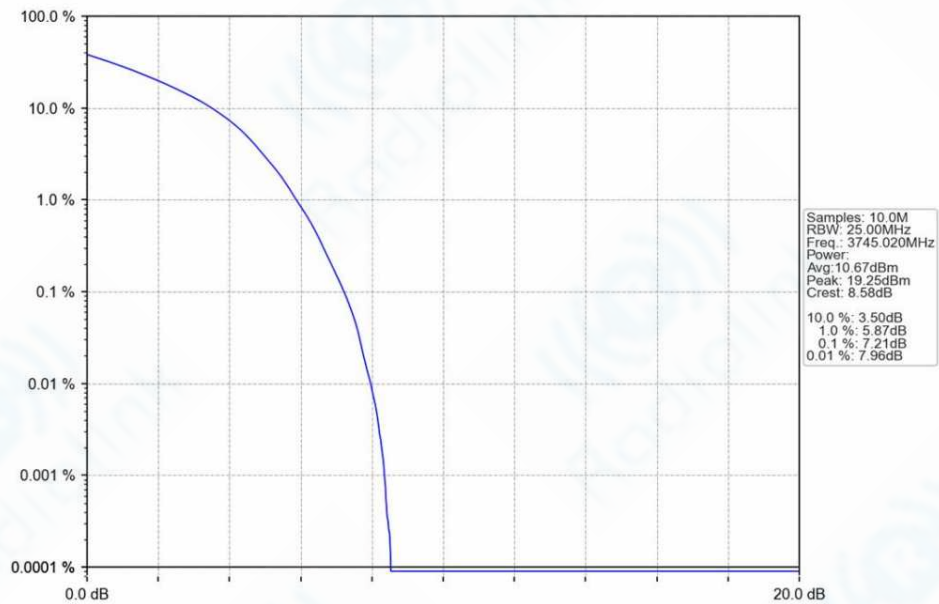
n78a_30kHz_SISO_NTNV_90MHz_DFT-s-OFDM_QPSK_3745.02MHz_Outer_Full_Ant1
