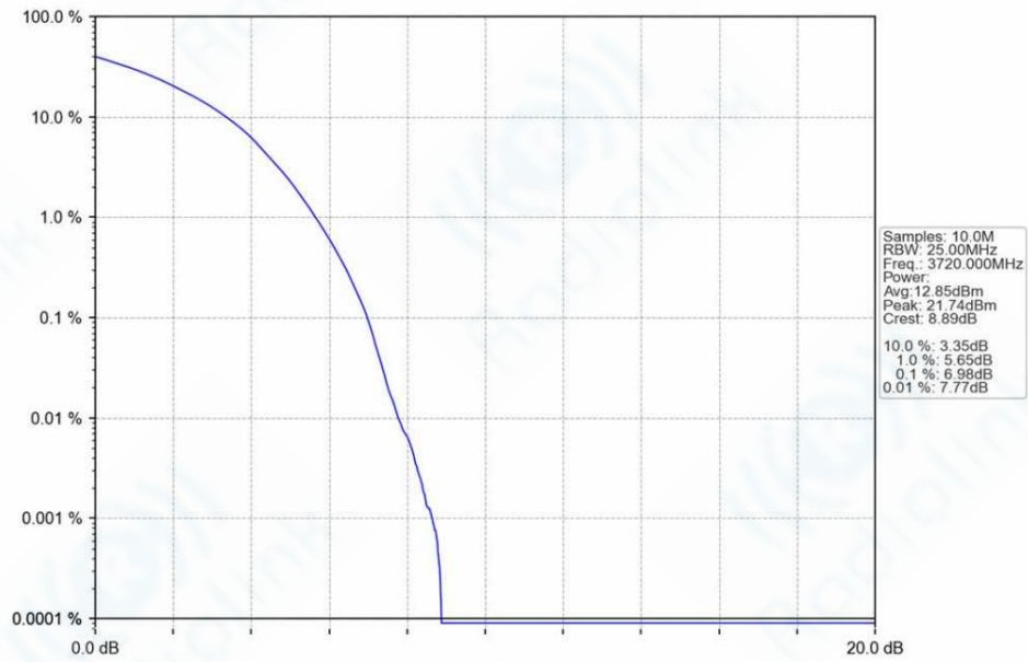
n78a_30kHz_SISO_NTNV_40MHz_DFT-s-OFDM_256_QAM_3720MHz_Outer_Full_Ant1
