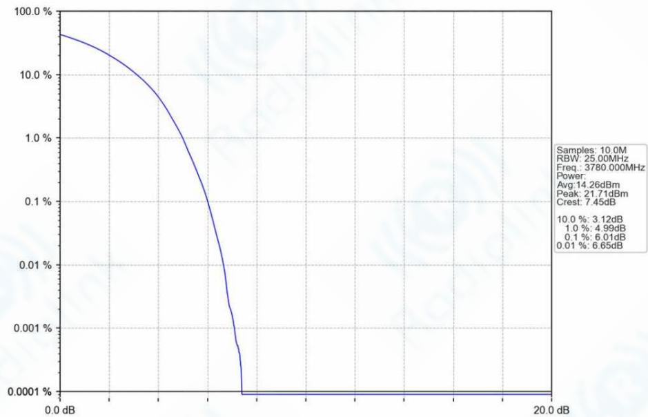
n78a_30kHz_SISO_NTNV_40MHz_DFT-s-OFDM_QPSK_3780MHz_Outer_Full_Ant1
