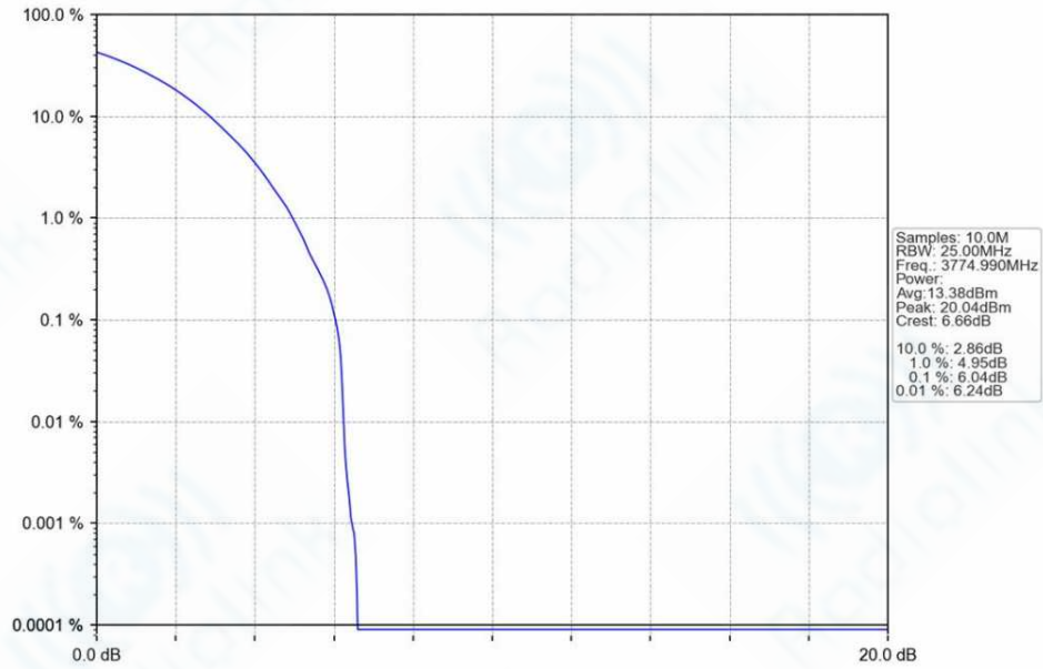
n78a_30kHz_SISO_NTNV_50MHz_DFT-s-OFDM_PI/2_BPSK_3774.99MHz_Outer_Full_Ant1
