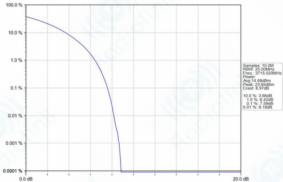
n78a_30kHz_SISO_NTNV_30MHz_CP-OFDM_64_QAM_3715.02MHz_Outer_Full_Ant1
