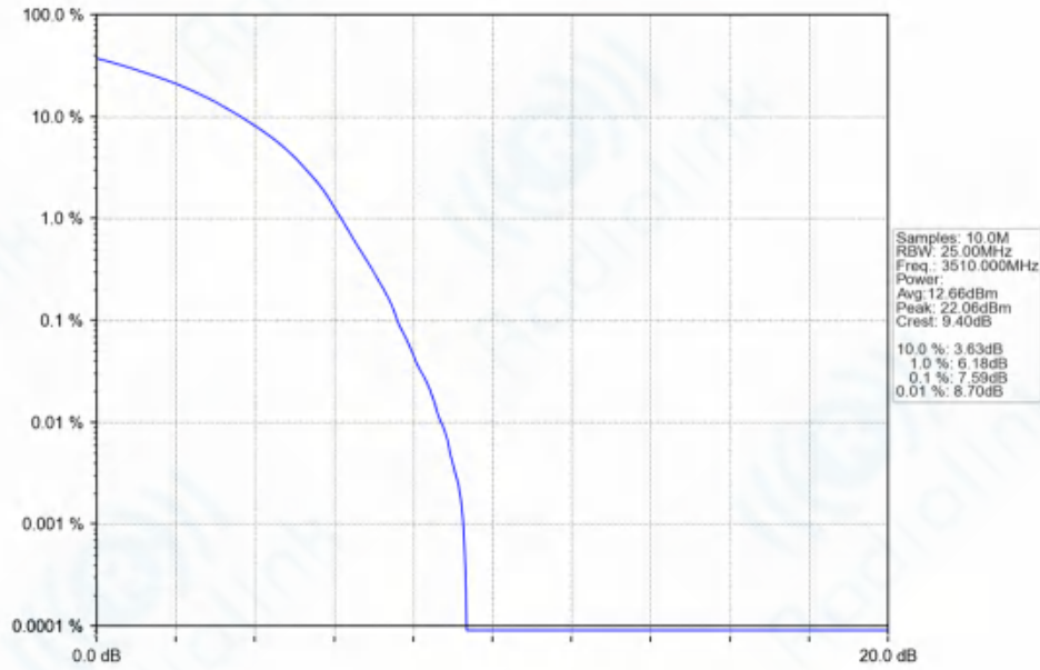
n77d_30kHz_SISO_NTNV_80MHz_DFT-s-OFDM_256_QAM_3510MHz_Outer_Full_Ant1
