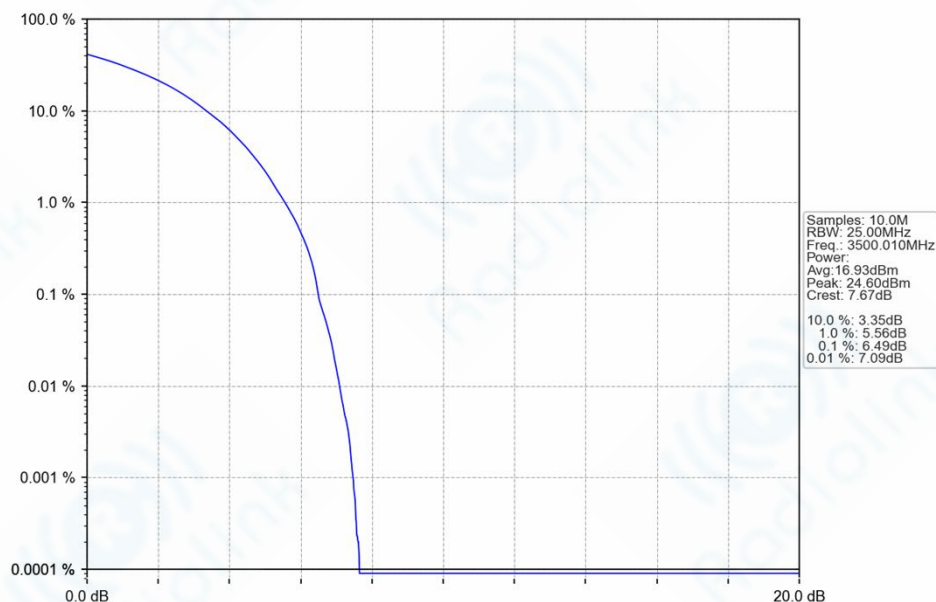
n77d_30kHz_SISO_NTNV_50MHz_DFT-s-OFDM_QPSK_3500.01MHz_Outer_Full_Ant1
