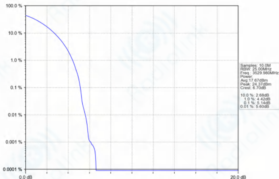
n77d_30kHz_SISO_NTNV_40MHz_DFT-s-OFDM_PI/2_BPSK_3529.98MHz_Outer_Full_Ant1
