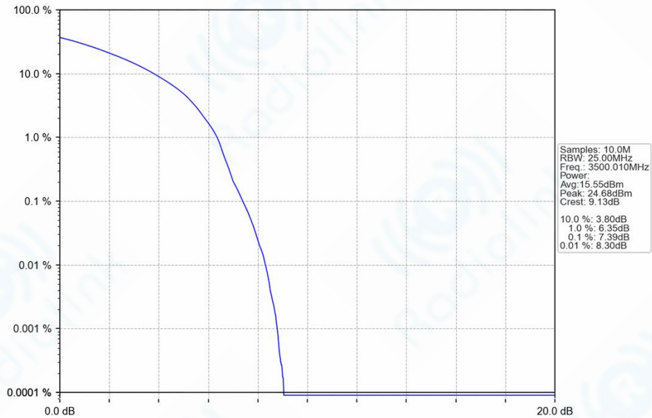
n77d_30kHz_SISO_NTNV_60MHz_DFT-s-OFDM_16_QAM_3500.01MHz_Outer_Full_Ant1
