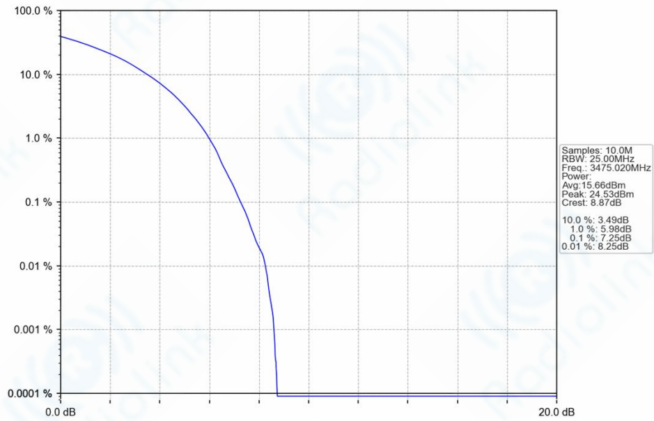
n77d_30kHz_SISO_NTNV_50MHz_DFT-s-OFDM_256_QAM_3475.02MHz_Outer_Full_Ant1
