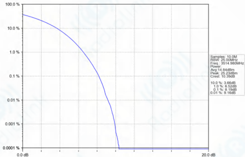
n77d_30kHz_SISO_NTNV_70MHz_CP-OFDM_QPSK_3514.98MHz_Outer_Full_Ant1
