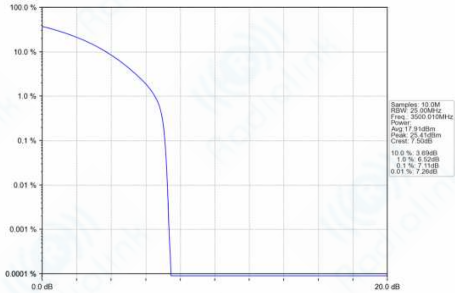
n77d_30kHz_SISO_NTNV_20MHz_CP-OFDM_64_QAM_3500.01MHz_Outer_Full_Ant1
