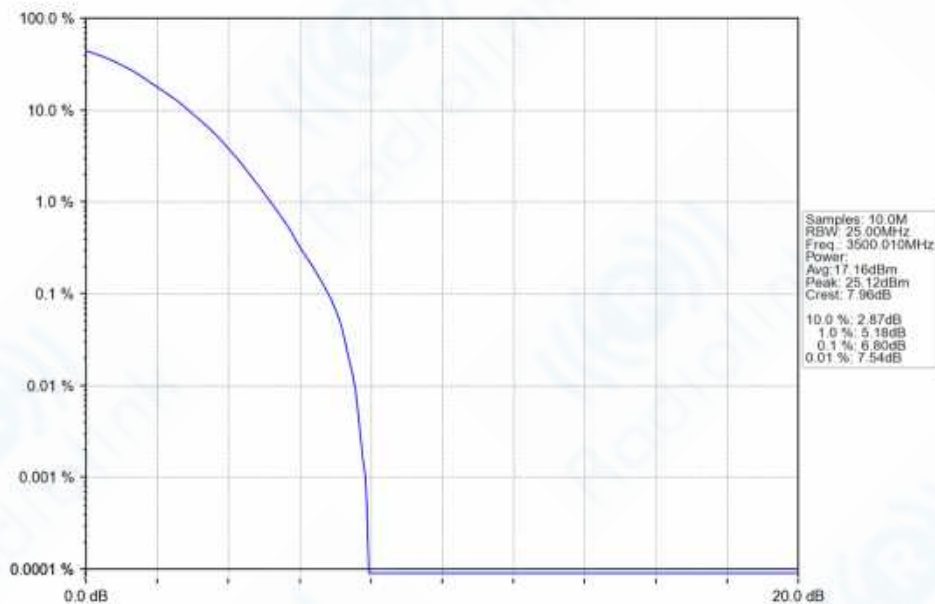
n77d_30kHz_SISO_NTNV_30MHz_DFT-s-OFDM_256_QAM_3500.01MHz_Outer_Full_Ant1
