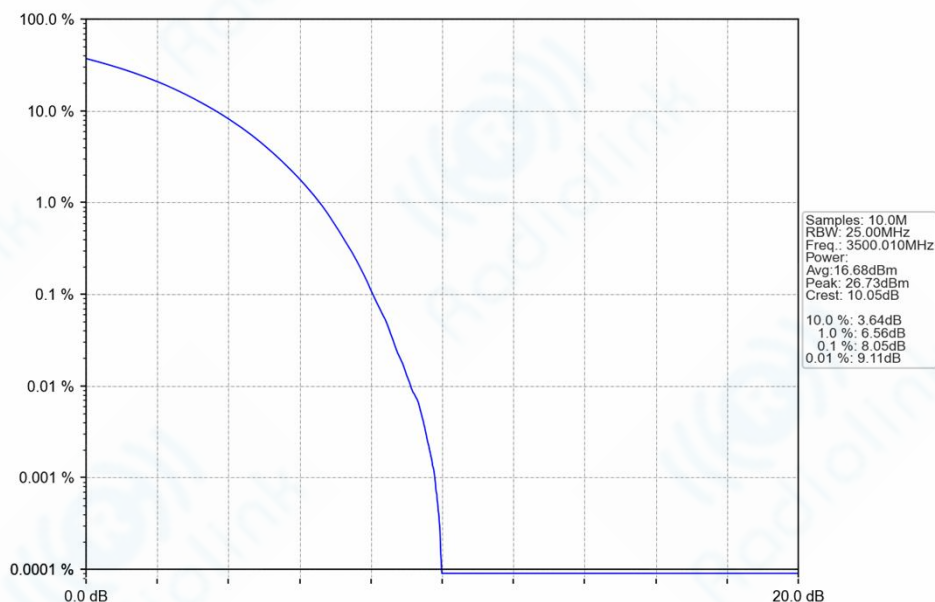
n77d_30kHz_SISO_NTNV_50MHz_CP-OFDM_QPSK_3500.01MHz_Outer_Full_Ant1
