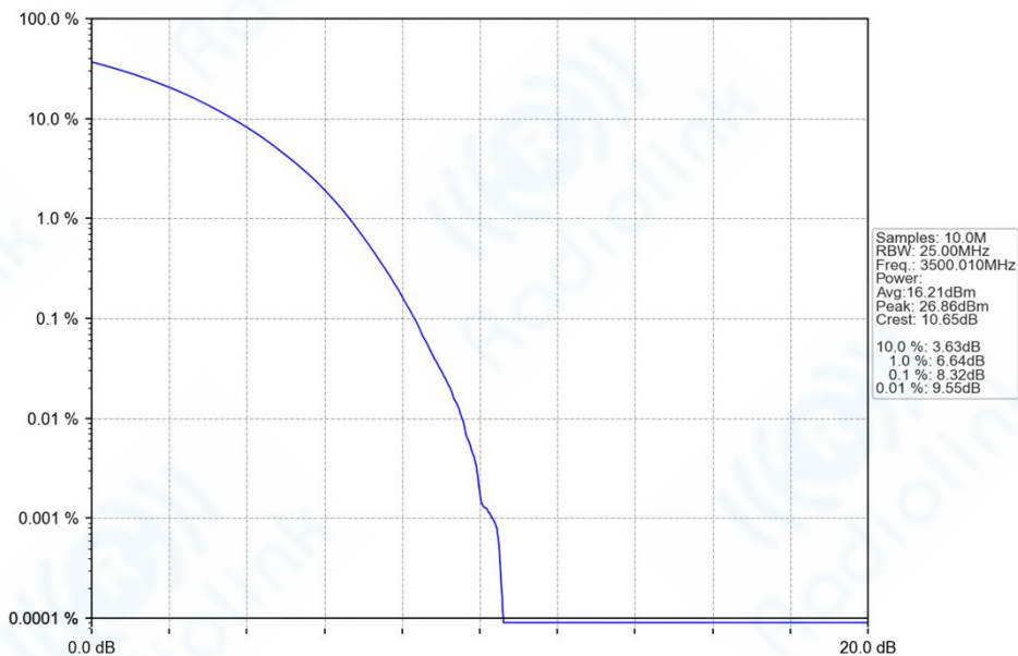
n77d_30kHz_SISO_NTNV_50MHz_CP-OFDM_64_QAM_3500.01MHz_Outer_Full_Ant1
