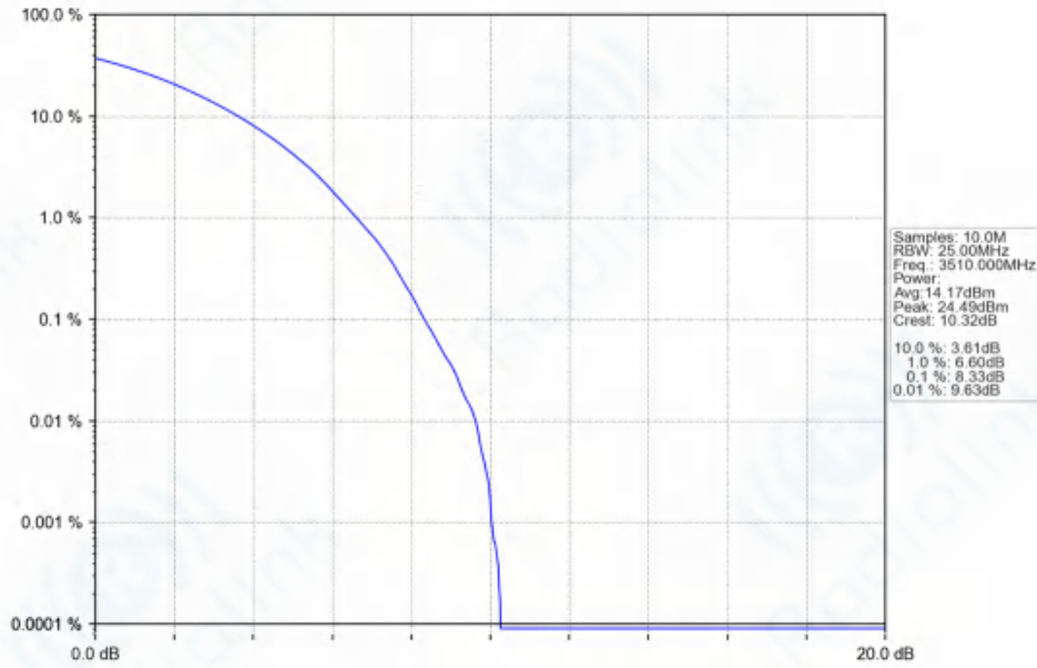
n77d_30kHz_SISO_NTNV_80MHz_CP-OFDM_16_QAM_3510MHz_Outer_Full_Ant1
