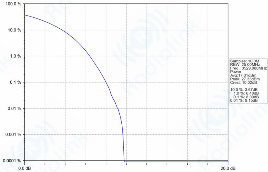
n77d_30kHz_SISO_NTNV_40MHz_CP-OFDM_16_QAM_3529.98MHz_Outer_Full_Ant1
