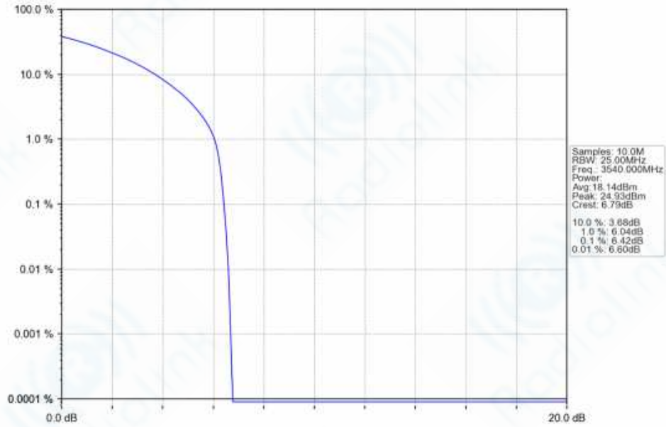
n77d_30kHz_SISO_NTNV_20MHz_CP-OFDM_16_QAM_3540MHz_Outer_Full_Ant1
