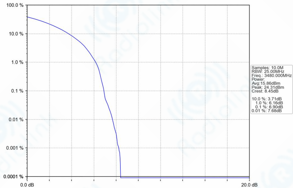
n77d_30kHz_SISO_NTNV_60MHz_DFT-s-OFDM QPSK_3480MHz_Outer_Full_Ant1
