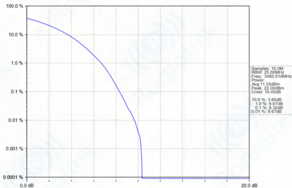
n77d_30kHz_SISO_NTNV_70MHz_CP-OFDM_256_QAM_3485.01MHz_Outer_Full_Ant1
