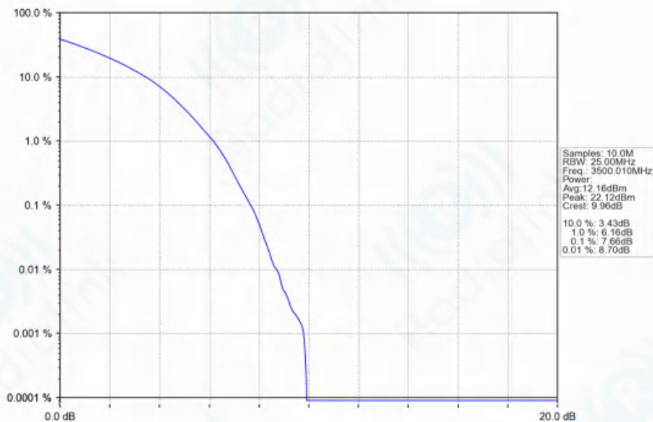
n77d_30kHz_SISO_NTNV_90MHz_DFT-s-OFDM_256_QAM_3500.01MHz_Outer_Full_Ant1
