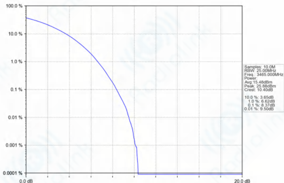
n77d_30kHz_SISO_NTNV_30MHz_CP-OFDM_256_QAM_3465MHz_Outer_Full_Ant1
