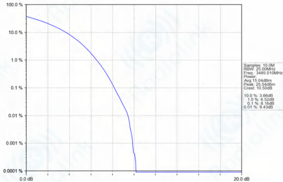
n77d_30kHz_SISO_NTNV_70MHz_CP-OFDM_16_QAM_3485.01MHz_Outer_Full_Ant1
