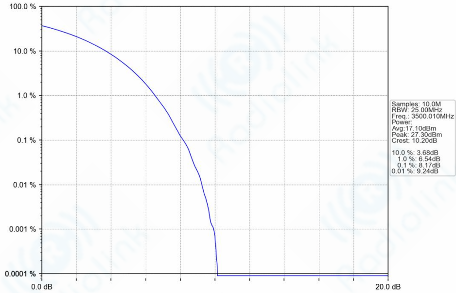
n77d_30kHz_SISO_NTNV_40MHz_CP-OFDM_64_QAM_3500.01MHz_Outer_Full_Ant1
