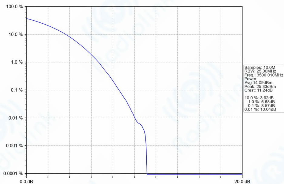
n77d_30kHz_SISO_NTNV_40MHz_CP-OFDM_256_QAM_3500.01MHz_Outer_Full_Ant1
