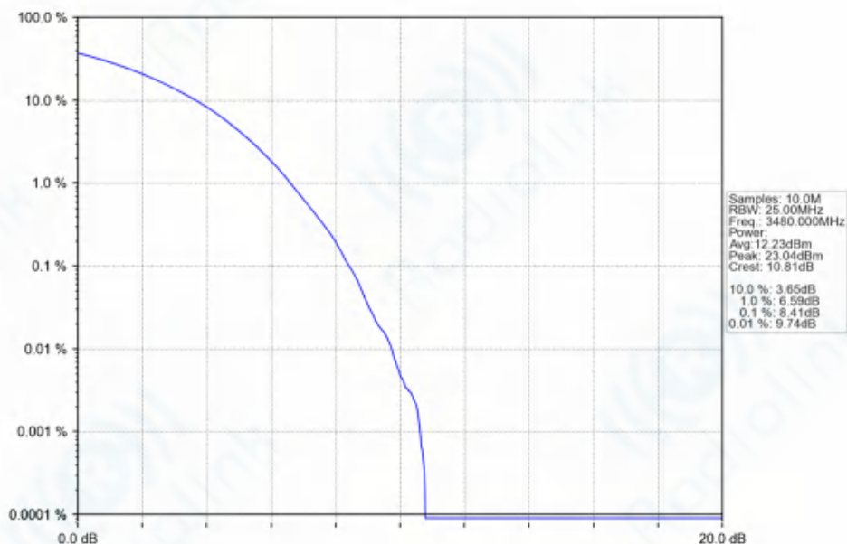
n77d_30kHz_SISO_NTNV_60MHz_CP-OFDM_256_QAM_3480MHz_Outer_Full_Ant1
