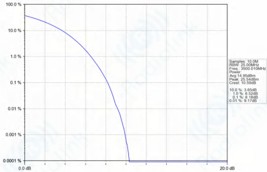
n77d_30kHz_SISO_NTNV_70MHz_CP-OFDM_QPSK_3500.01MHz_Outer_Full_Ant1
