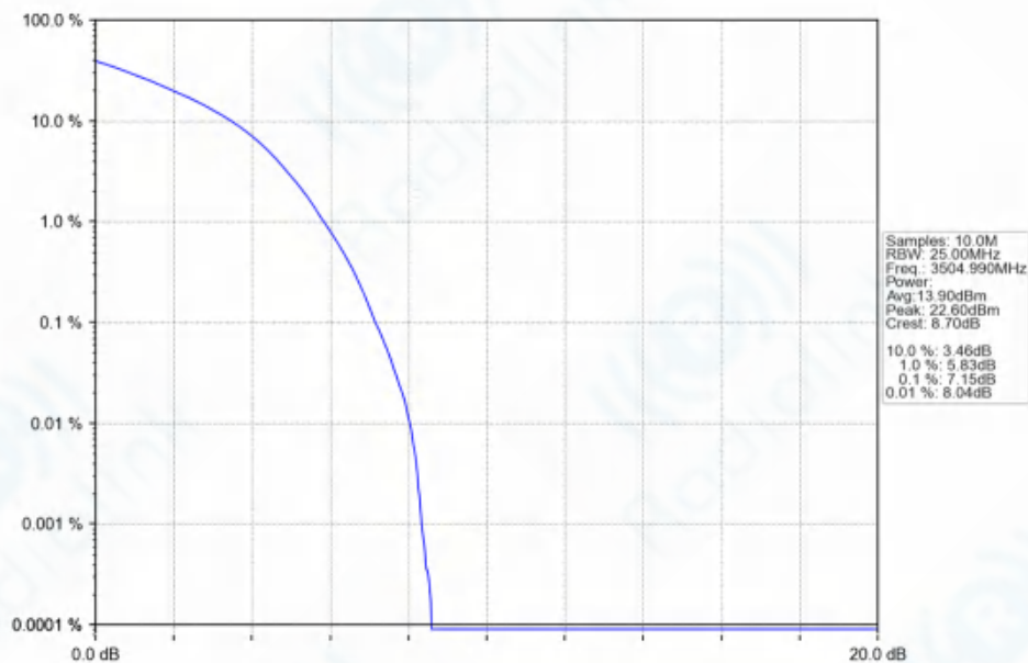
n77d_30kHz_SISO_NTNV_90MHz_DFT-s-OFDM_QPSK_3504.99MHz_Outer_Full_Ant1
