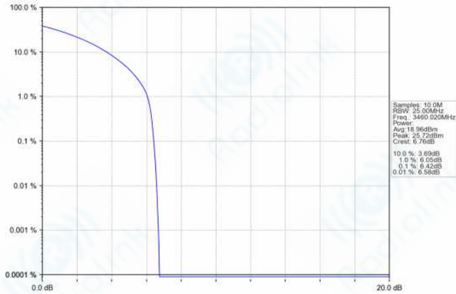
n77d_30kHz_SISO_NTNV_20MHz_CP-OFDM_16_QAM_3460.02MHz_Outer_Full_Ant1
