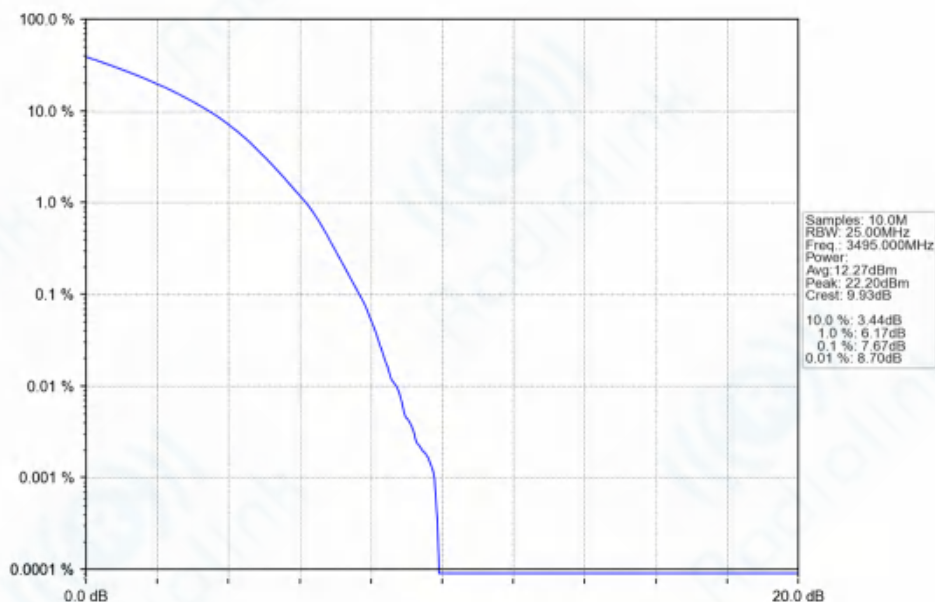
n77d_30kHz_SISO_NTNV_90MHz_DFT-s-OFDM_256_QAM_3495MHz_Outer_Full_Ant1
