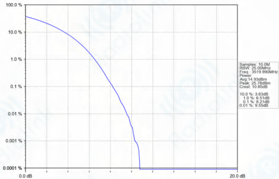
n77d_30kHz_SISO_NTNV_60MHz_CP-OFDM_64_QAM_3519.99MHz_Outer_Full_Ant1
