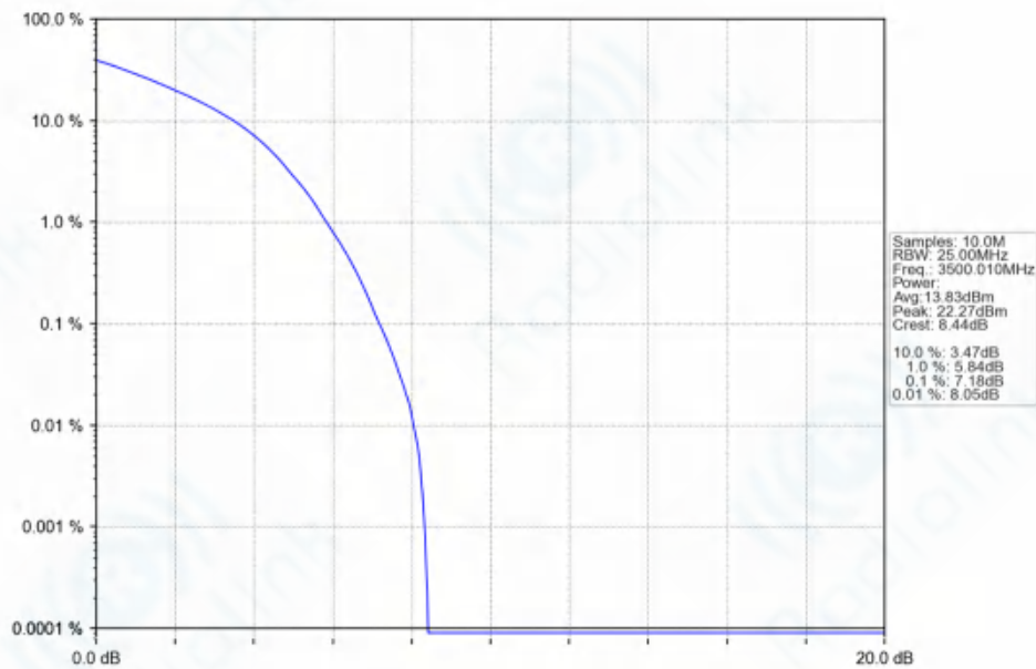
n77d_30kHz_SISO_NTNV_90MHz_DFT-s-OFDM_QPSK_3500.01MHz_Outer_Full_Ant1
