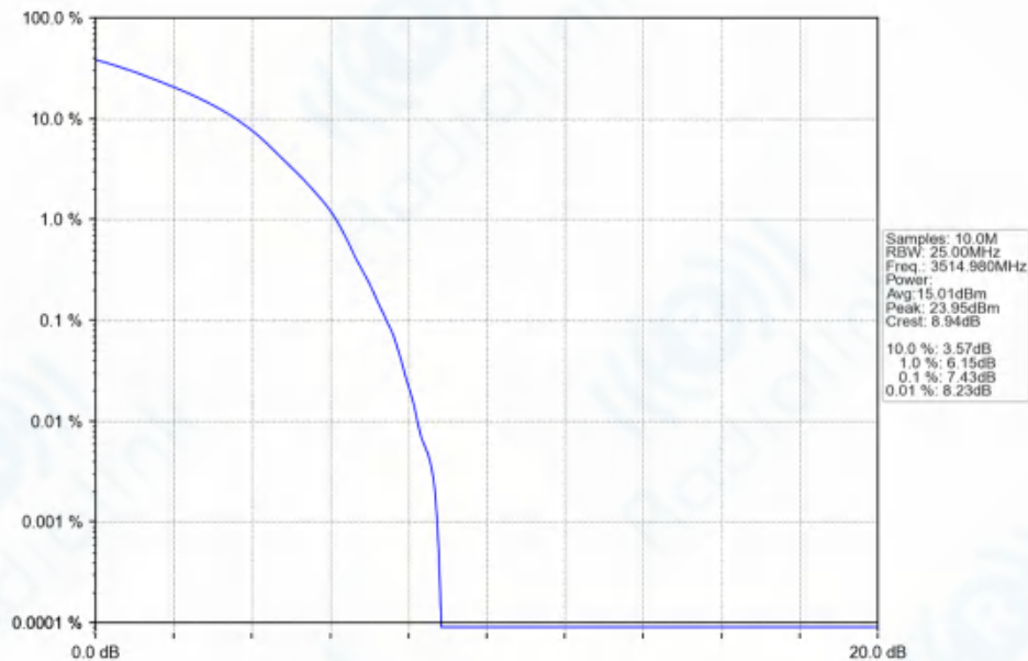
n77d_30kHz_SISO_NTNV_70MHz_DFT-s-OFDM_64_QAM_3514.98MHz_Outer_Full_Ant1
