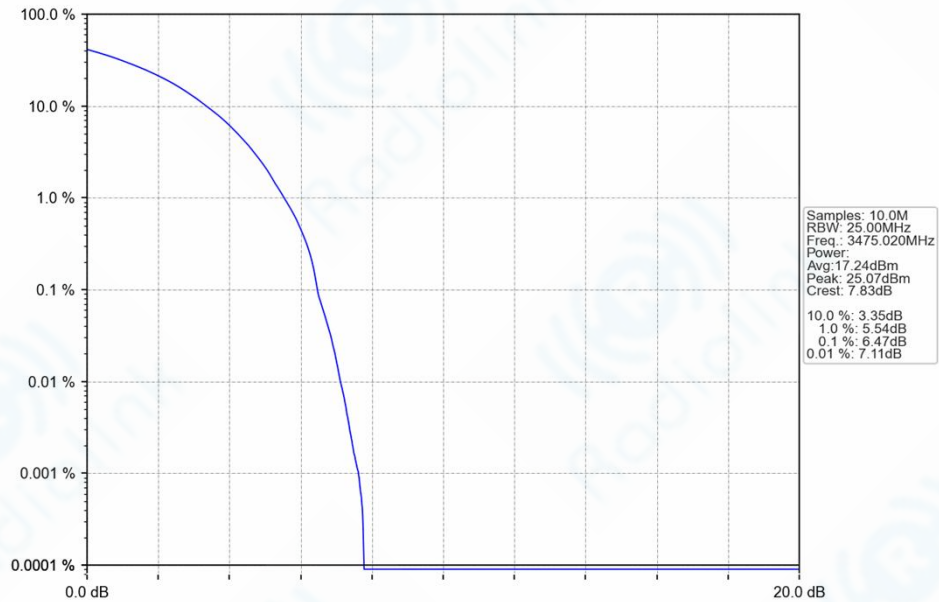
n77d_30kHz_SISO_NTNV_50MHz_DFT-s-OFDM_QPSK_3475.02MHz_Outer_Full_Ant1
