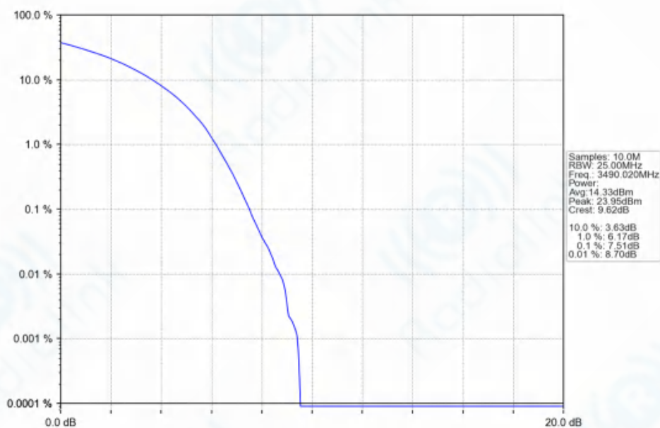
n77d_30kHz_SISO_NTNV_80MHz_DFT-s-OFDM_64_QAM_3490.02MHz_Outer_Full_Ant1
