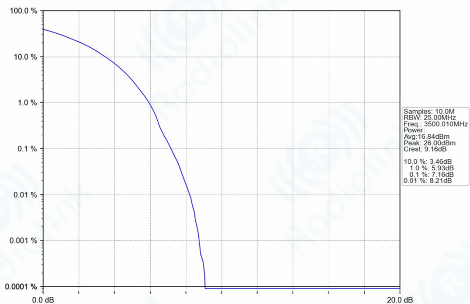
n77d_30kHz_SISO_NTNV_50MHz_DFT-s-OFDM_16_QAM_3500.01MHz_Outer_Full_Ant1
