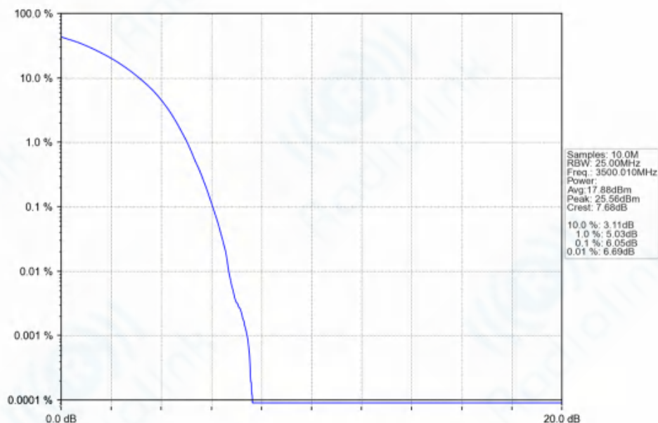
n77d_30kHz_SISO_NTNV_40MHz_DFT-s-OFDM_QPSK_3500.01MHz_Outer_Full_Ant1
