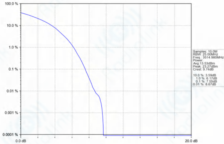
n77d_30kHz_SISO_NTNV_70MHz_DFT-s-OFDM_256_QAM_3514.98MHz_Outer_Full_Ant1
