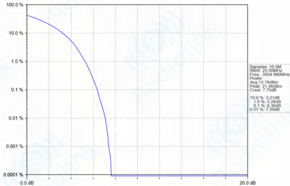
n77d_30kHz_SISO_NTNV_90MHz_DFT-s-OFDM PI/2 BPSK_3504.99MHz_Outer_Full_Ant1
