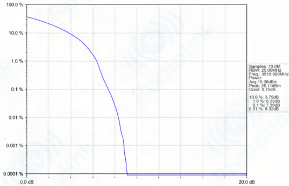
n77d_30kHz_SISO_NTNV_60MHz_DFT-s-OFDM_16_QAM_3519.99MHz_Outer_Full_Ant1
