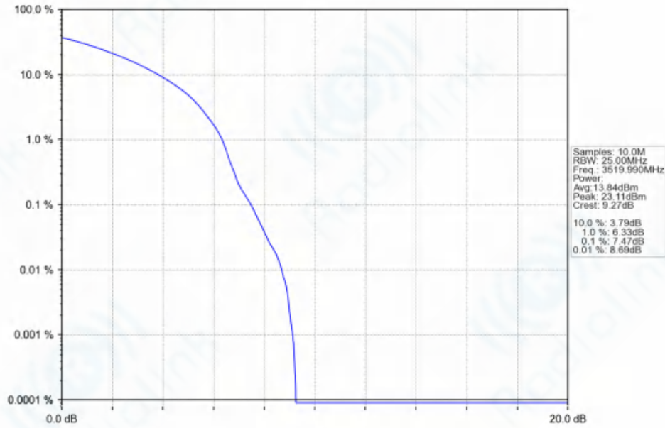
n77d_30kHz_SISO_NTNV_60MHz_DFT-s-OFDM_256_QAM_3519.99MHz_Outer_Full_Ant1
