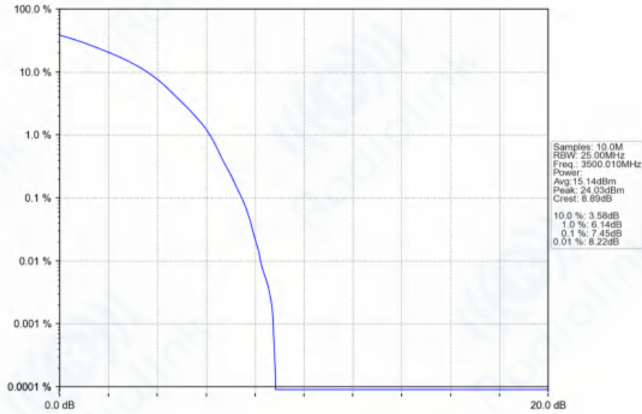
n77d_30kHz_SISO_NTNV_70MHz_DFT-s-OFDM_64_QAM_3500.01MHz_Outer_Full_Ant1
