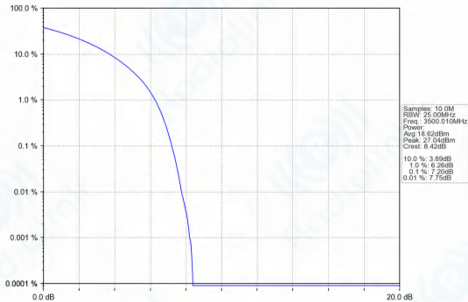
n77d_30kHz_SISO_NTNV_30MHz_CP-OFDM_16_QAM_3500.01MHz_Outer_Full_Ant1
