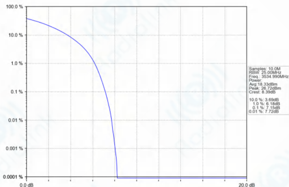
n77d_30kHz_SISO_NTNV_30MHz_CP-OFDM_QPSK_3534.99MHz_Outer_Full_Ant1
