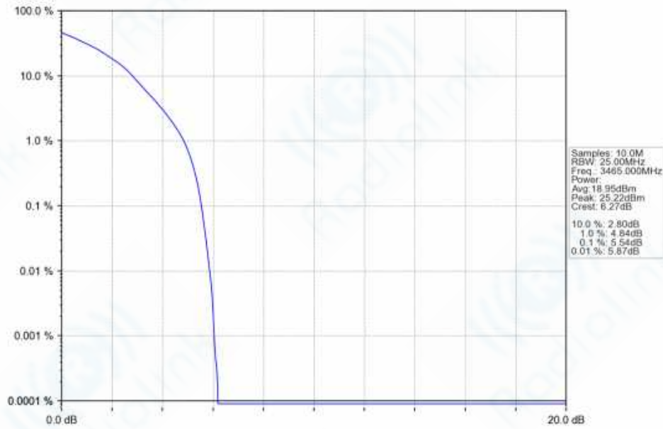
n77d_30kHz_SISO_NTNV_30MHz_DFT-s-OFDM_16_QAM_3465MHz_Outer_Full_Ant1
