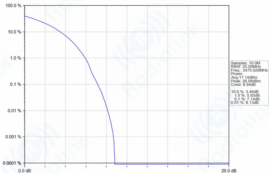
n77d_30kHz_SISO_NTNV_50MHz_DFT-s-OFDM_16_QAM_3475.02MHz_Outer_Full_Ant1
