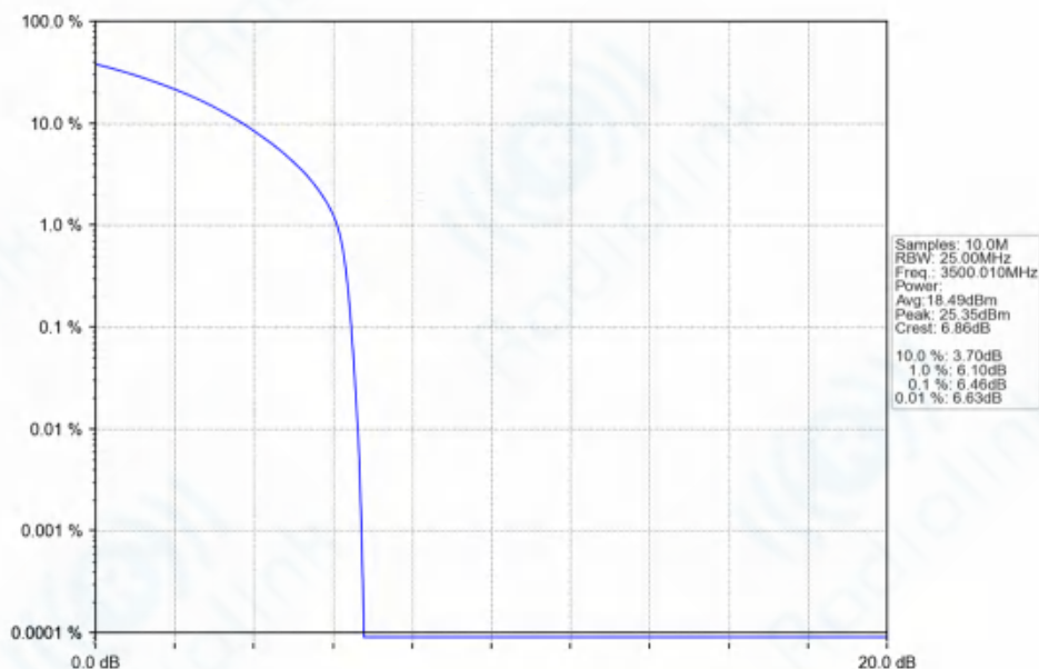
n77d_30kHz_SISO_NTNV_20MHz_CP-OFDM_QPSK_3500.01MHz_Outer_Full_Ant1
