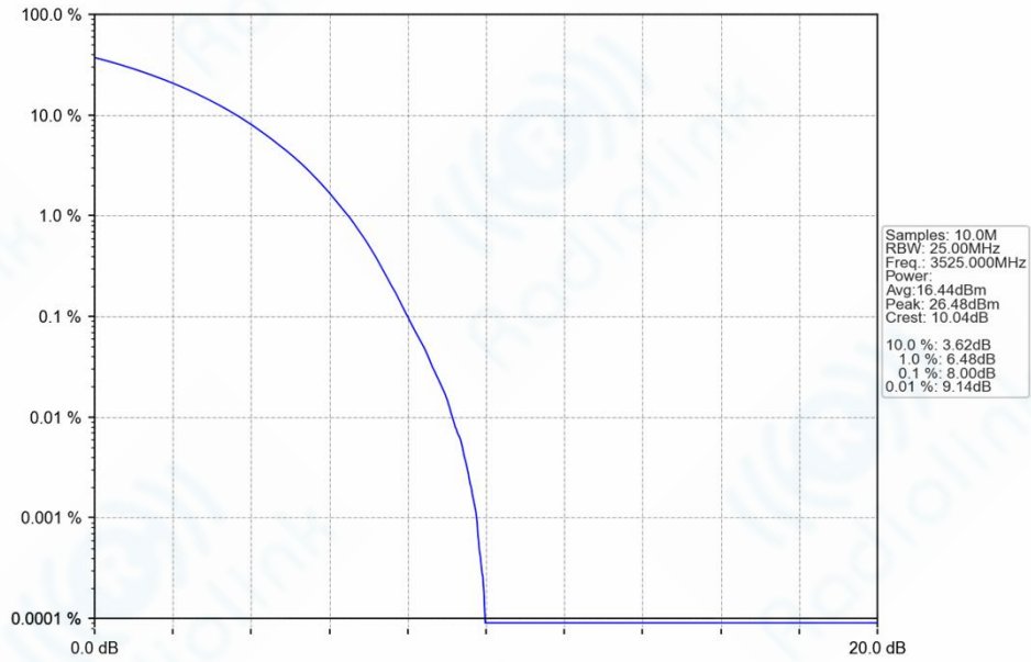
n77d_30kHz_SISO_NTNV_50MHz_CP-OFDM_16_QAM_3525MHz_Outer_Full_Ant1
