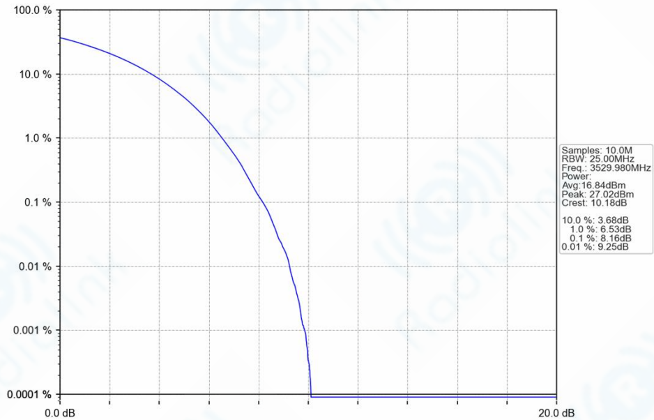
n77d_30kHz_SISO_NTNV_40MHz_CP-OFDM_64_QAM_3529.98MHz_Outer_Full_Ant1
