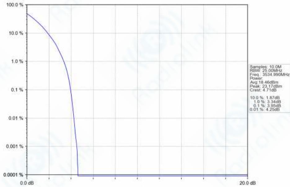
n77d_30kHz_SISO_NTNV_30MHz_DFT-s-OFDM PI/2 BPSK_3534.99MHz_Outer_Full_Ant1
