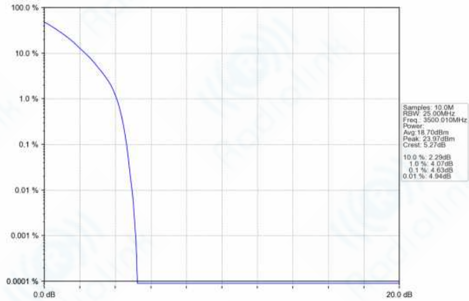
n77d_30kHz_SISO_NTNV_30MHz_DFT-s-OFDM_QPSK_3500.01MHz_Outer_Full_Ant1
