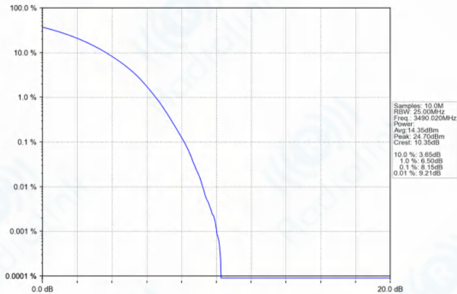
n77d_30kHz_SISO_NTNV_80MHz_CP-OFDM_QPSK_3490.02MHz_Outer_Full_Ant1
