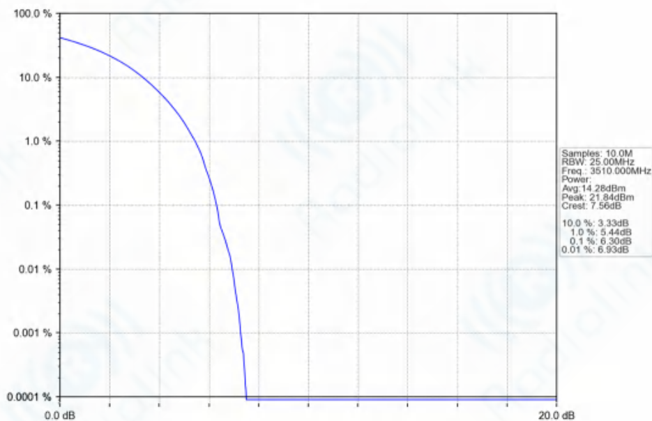
n77d_30kHz_SISO_NTNV_80MHz_DFT-s-OFDM PI/2 BPSK_3510MHz_Outer_Full_Ant1
