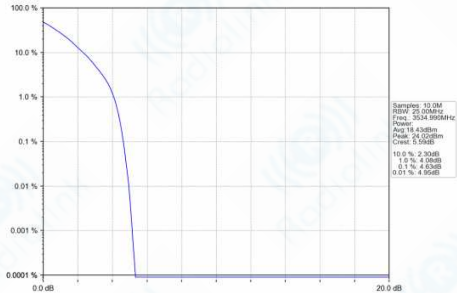
n77d_30kHz_SISO_NTNV_30MHz_DFT-s-OFDM_QPSK_3534.99MHz_Outer_Full_Ant1
