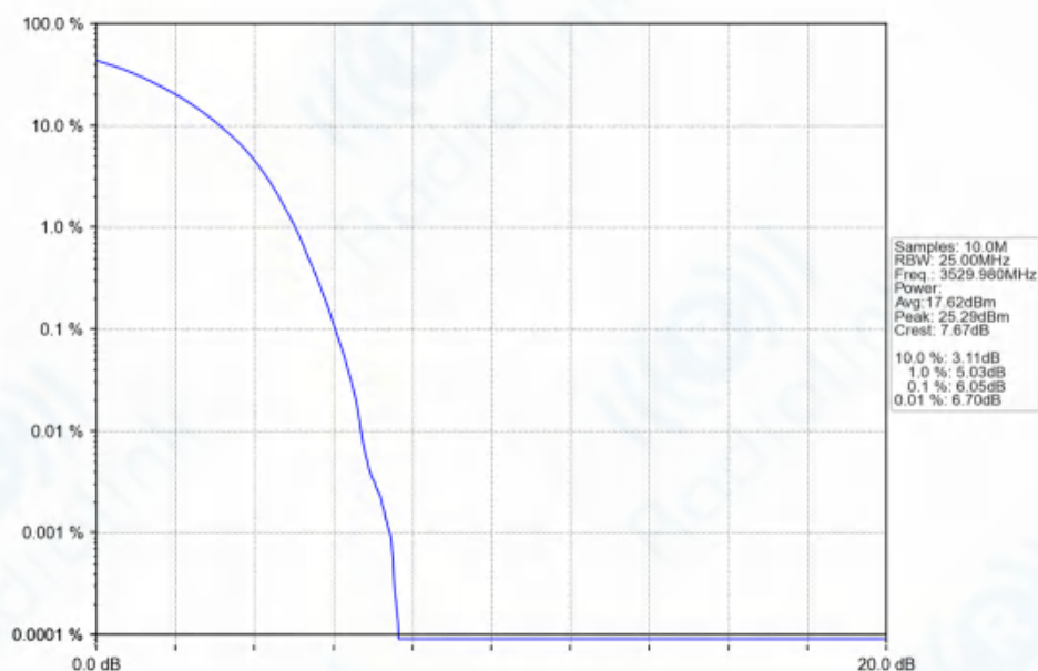
n77d_30kHz_SISO_NTNV_40MHz_DFT-s-OFDM_QPSK_3529.98MHz_Outer_Full_Ant1
