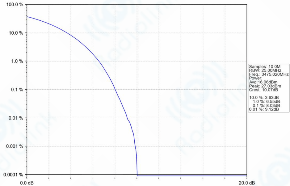
n77d_30kHz_SISO_NTNV_50MHz_CP-OFDM_QPSK_3475.02MHz_Outer_Full_Ant1
