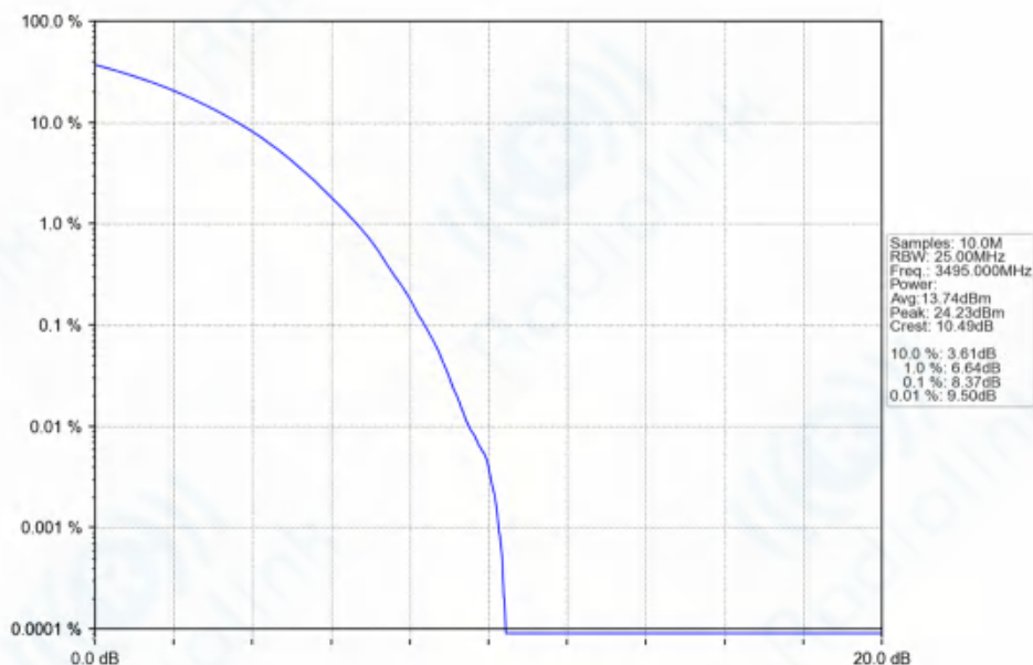
n77d_30kHz_SISO_NTNV_90MHz_CP-OFDM_16_QAM_3495MHz_Outer_Full_Ant1
