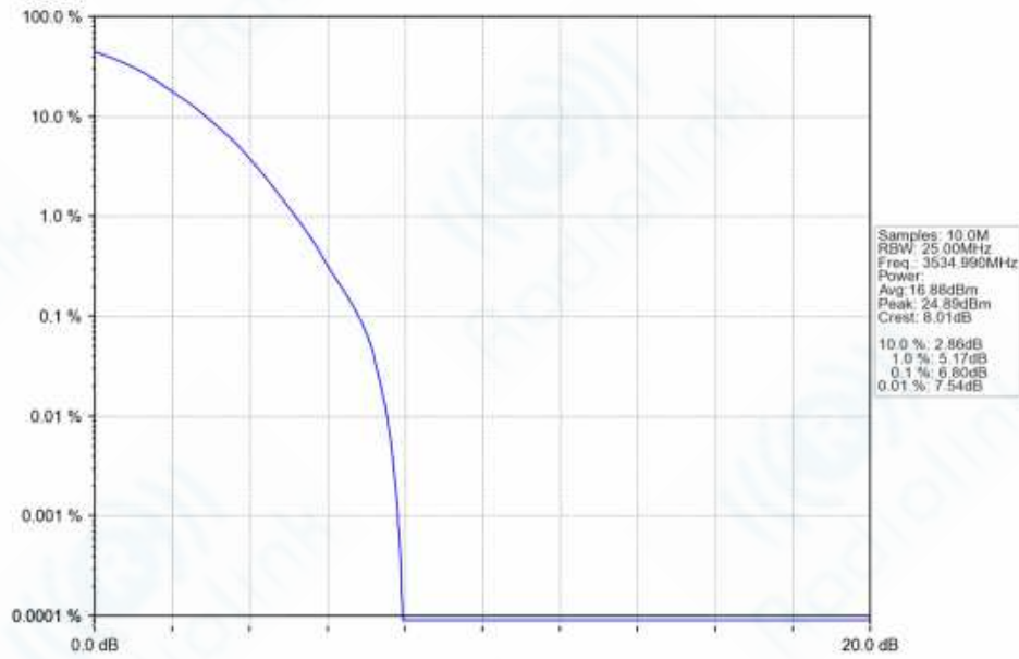
n77d_30kHz_SISO_NTNV_30MHz_DFT-s-OFDM_256_QAM_3534.99MHz_Outer_Full_Ant1
