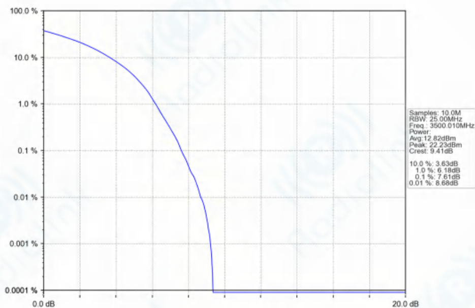
n77d_30kHz_SISO_NTNV_80MHz_DFT-s-OFDM_256_QAM_3500.01MHz_Outer_Full_Ant1
