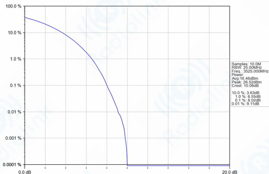
n77d_30kHz_SISO_NTNV_50MHz_CP-OFDM_QPSK_3525MHz_Outer_Full_Ant1
