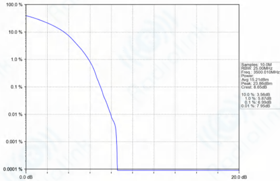
n77d_30kHz_SISO_NTNV_70MHz_DFT-s-OFDM_QPSK_3500.01MHz_Outer_Full_Ant1
