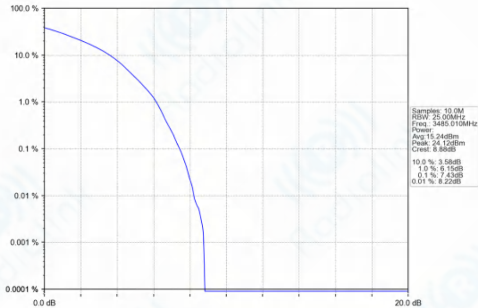
n77d_30kHz_SISO_NTNV_70MHz_DFT-s-OFDM_64_QAM_3485.01MHz_Outer_Full_Ant1
