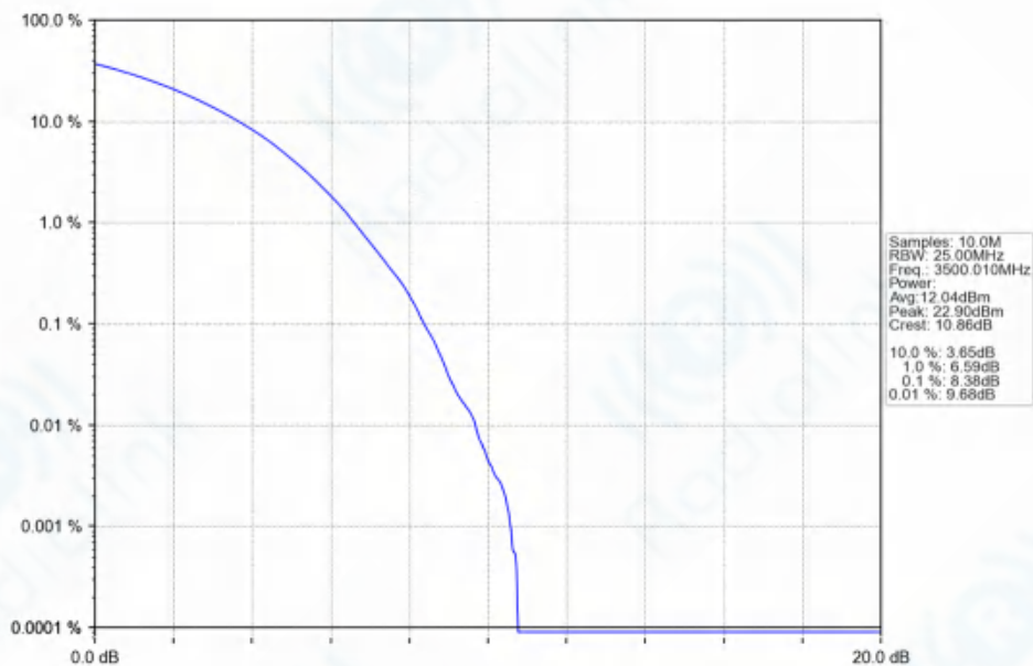
n77d_30kHz_SISO_NTNV_60MHz_CP-OFDM_256_QAM_3500.01MHz_Outer_Full_Ant1
