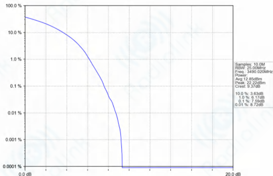
n77d_30kHz_SISO_NTNV_80MHz_DFT-s-OFDM_256_QAM_3490.02MHz_Outer_Full_Ant1
