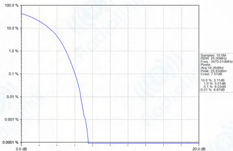
n77d_30kHz_SISO_NTNV_40MHz_DFT-s-OFDM_QPSK_3470.01MHz_Outer_Full_Ant1
