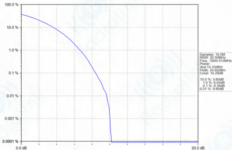
n77d_30kHz_SISO_NTNV_80MHz_CP-OFDM_16_QAM_3500.01MHz_Outer_Full_Ant1
