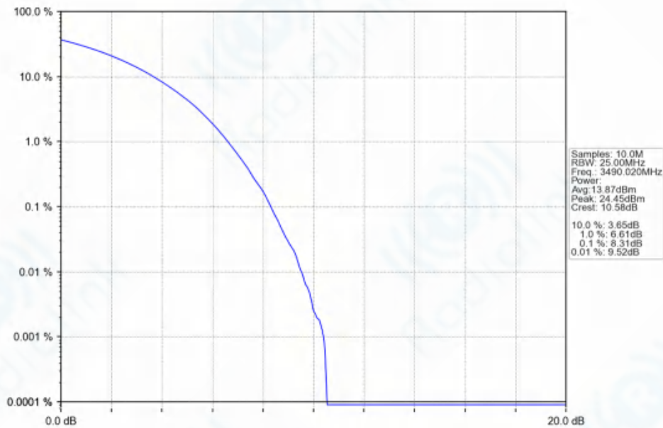
n77d_30kHz_SISO_NTNV_80MHz_CP-OFDM_64_QAM_3490.02MHz_Outer_Full_Ant1
