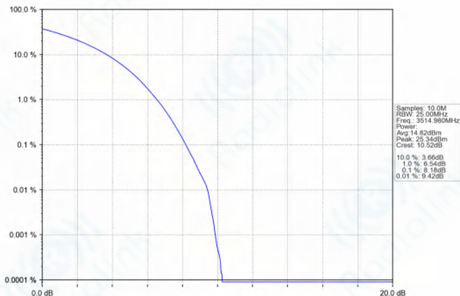
n77d_30kHz_SISO_NTNV_70MHz_CP-OFDM_16_QAM_3514.98MHz_Outer_Full_Ant1
