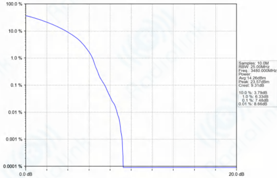
n77d_30kHz_SISO_NTNV_60MHz_DFT-s-OFDM_256_QAM_3480MHz_Outer_Full_Ant1
