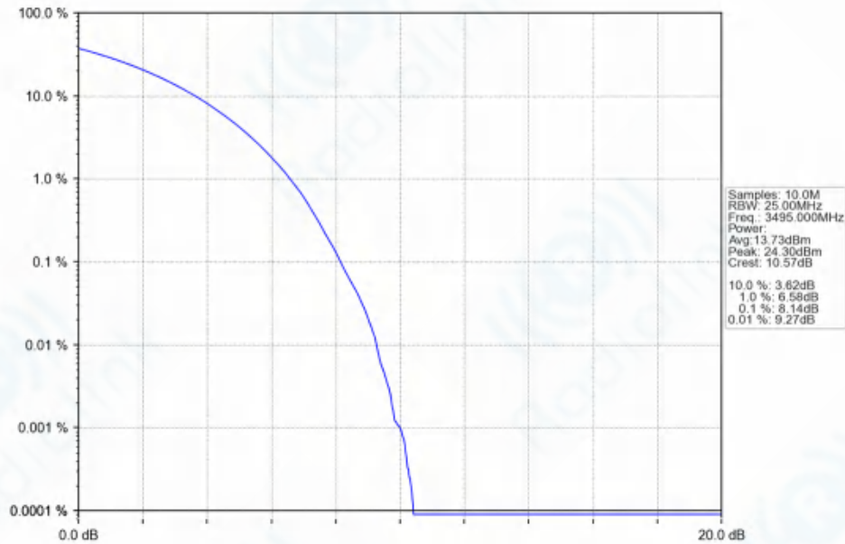
n77d_30kHz_SISO_NTNV_90MHz_CP-OFDM_QPSK_3495MHz_Outer_Full_Ant1
