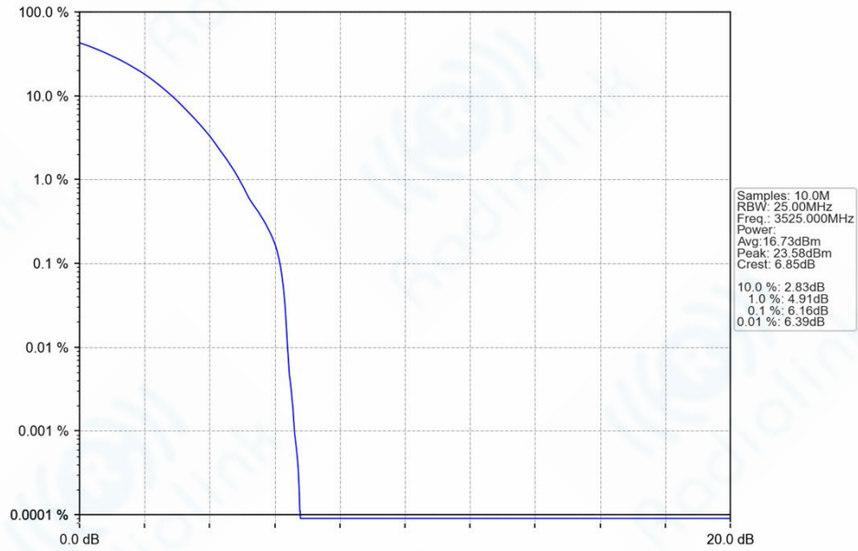
n77d_30kHz_SISO_NTNV_50MHz_DFT-s-OFDM_PI/2_BPSK_3525MHz_Outer_Full_Ant1
