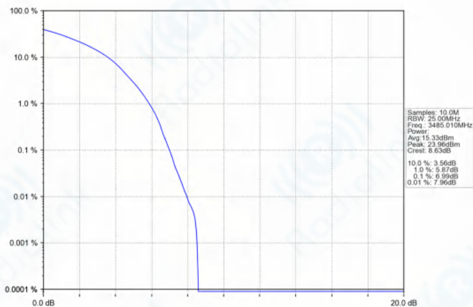
n77d_30kHz_SISO_NTNV_70MHz_DFT-s-OFDM_QPSK_3485.01MHz_Outer_Full_Ant1
