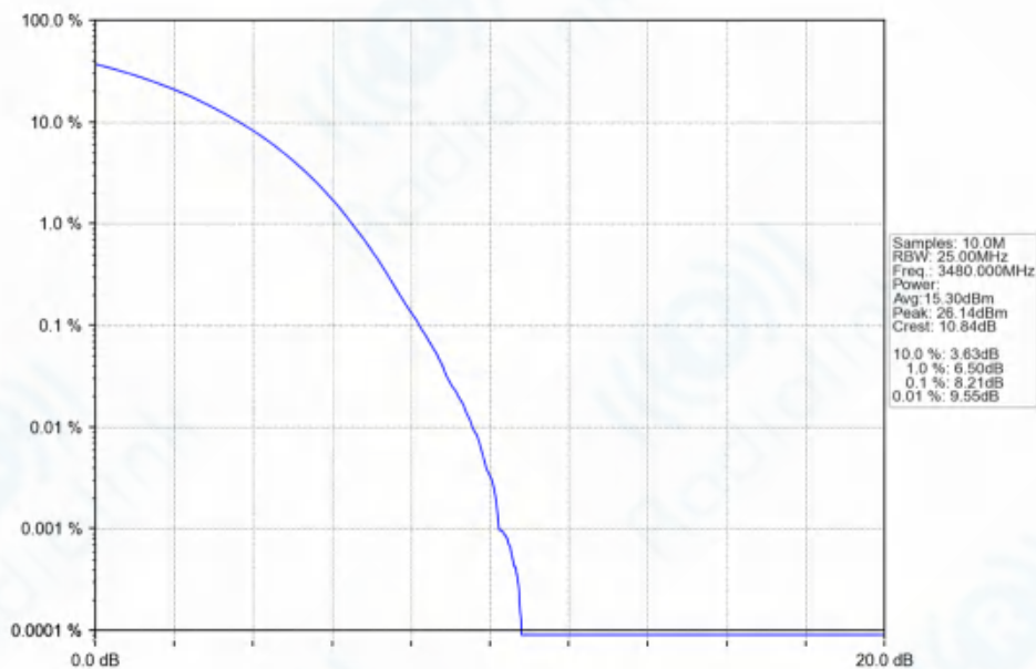
n77d_30kHz_SISO_NTNV_60MHz_CP-OFDM_64_QAM_3480MHz_Outer_Full_Ant1
