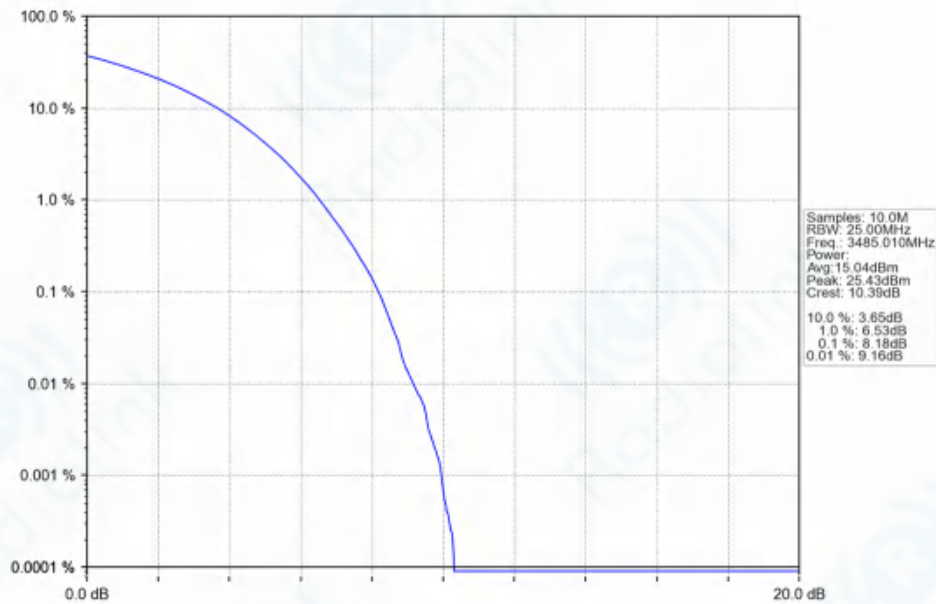
n77d_30kHz_SISO_NTNV_70MHz_CP-OFDM_QPSK_3485.01MHz_Outer_Full_Ant1
