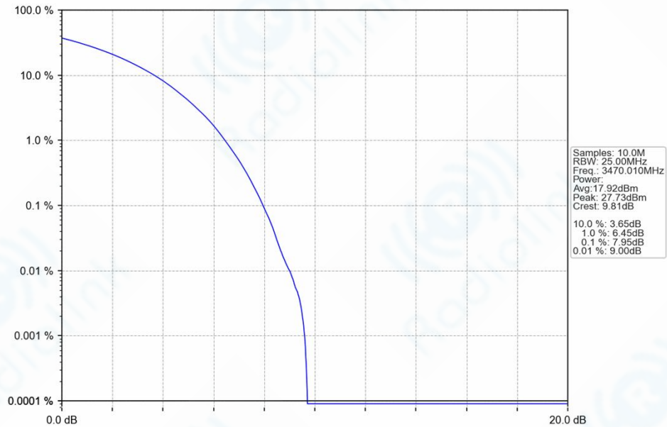
n77d_30kHz_SISO_NTNV_40MHz_CP-OFDM_QPSK_3470.01MHz_Outer_Full_Ant1
