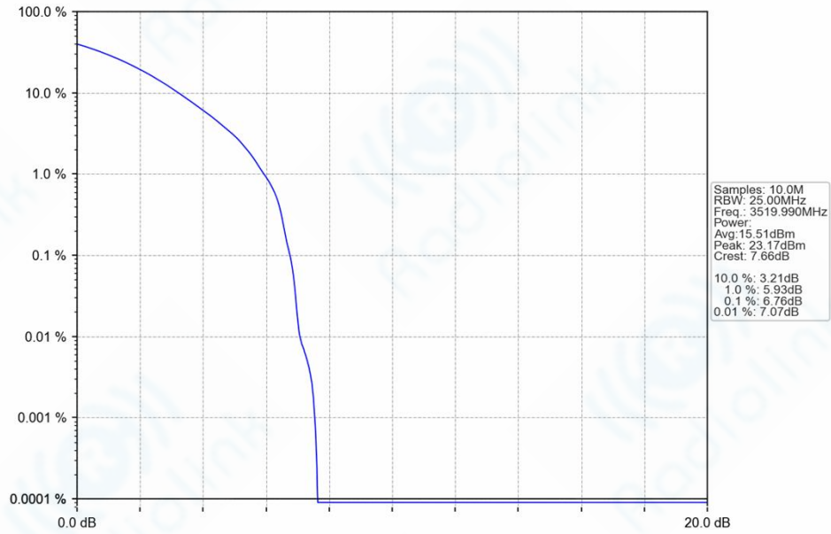
n77d_30kHz_SISO_NTNV_60MHz_DFT-s-OFDM PI/2 BPSK_3519.99MHz_Outer_Full_Ant1
