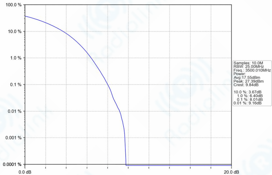
n77d_30kHz_SISO_NTNV_40MHz_CP-OFDM_16_QAM_3500.01MHz_Outer_Full_Ant1
