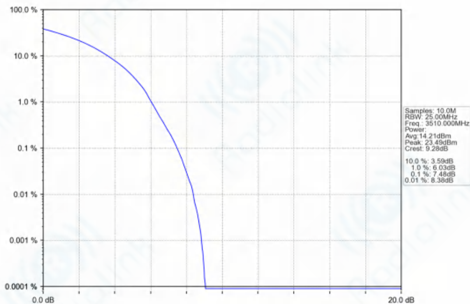
n77d_30kHz_SISO_NTNV_80MHz_DFT-s-OFDM_16_QAM_3510MHz_Outer_Full_Ant1
