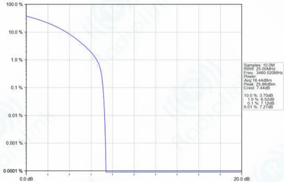
n77d_30kHz_SISO_NTNV_20MHz_CP-OFDM_64_QAM_3460.02MHz_Outer_Full_Ant1
