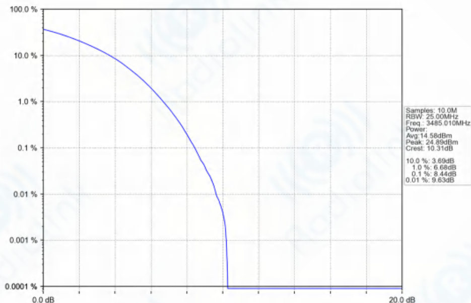
n77d_30kHz_SISO_NTNV_70MHz_CP-OFDM_64_QAM_3485.01MHz_Outer_Full_Ant1
