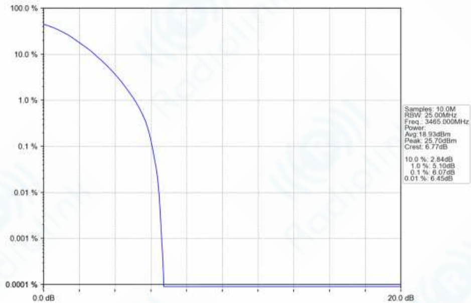
n77d_30kHz_SISO_NTNV_30MHz_DFT-s-OFDM_64_QAM_3465MHz_Outer_Full_Ant1
