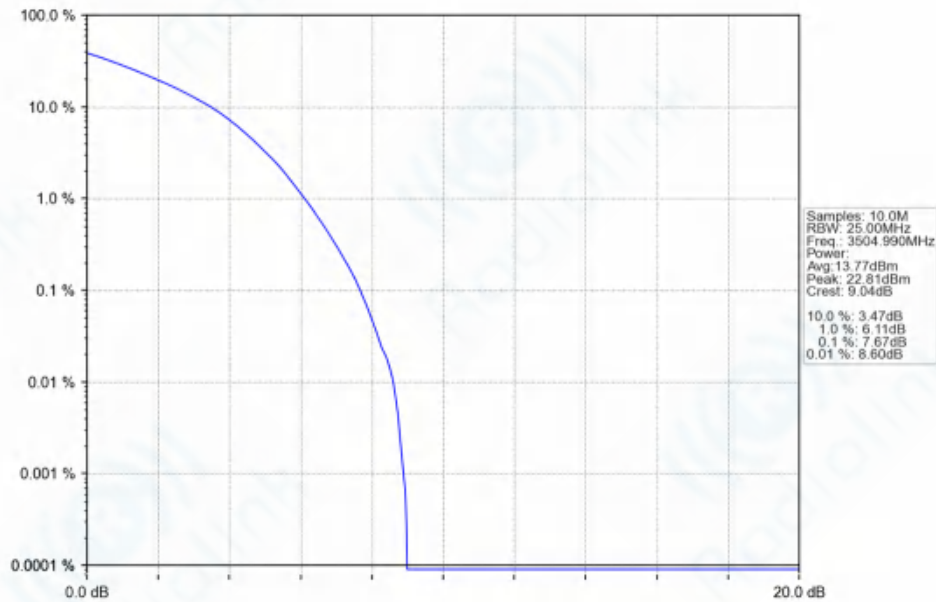
n77d_30kHz_SISO_NTNV_90MHz_DFT-s-OFDM_16_QAM_3504.99MHz_Outer_Full_Ant1
