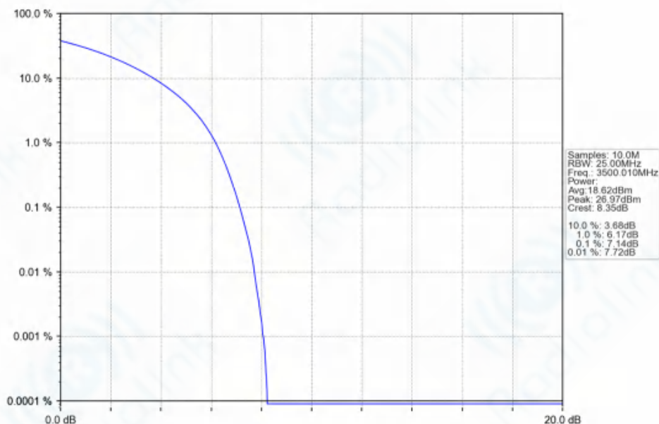
n77d_30kHz_SISO_NTNV_30MHz_CP-OFDM_QPSK_3500.01MHz_Outer_Full_Ant1
