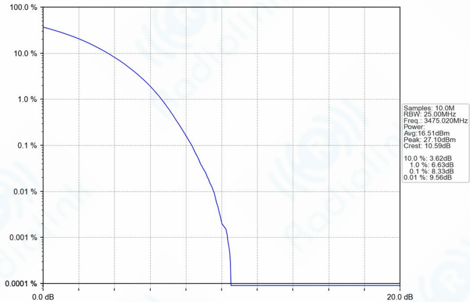
n77d_30kHz_SISO_NTNV_50MHz_CP-OFDM_64_QAM_3475.02MHz_Outer_Full_Ant1
