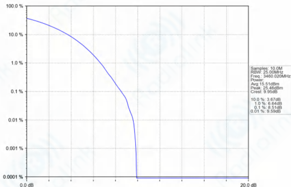
n77d_30kHz_SISO_NTNV_20MHz_CP-OFDM_256_QAM_3460.02MHz_Outer_Full_Ant1
