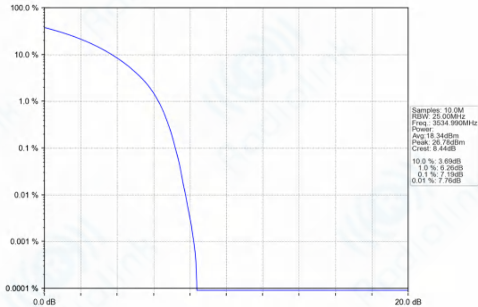
n77d_30kHz_SISO_NTNV_30MHz_CP-OFDM 16 QAM_3534.99MHz_Outer_Full_Ant1
