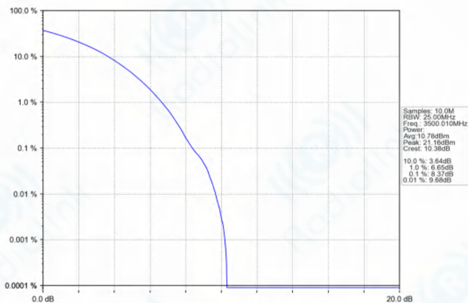
n77d_30kHz_SISO_NTNV_80MHz_CP-OFDM_256_QAM_3500.01MHz_Outer_Full_Ant1
