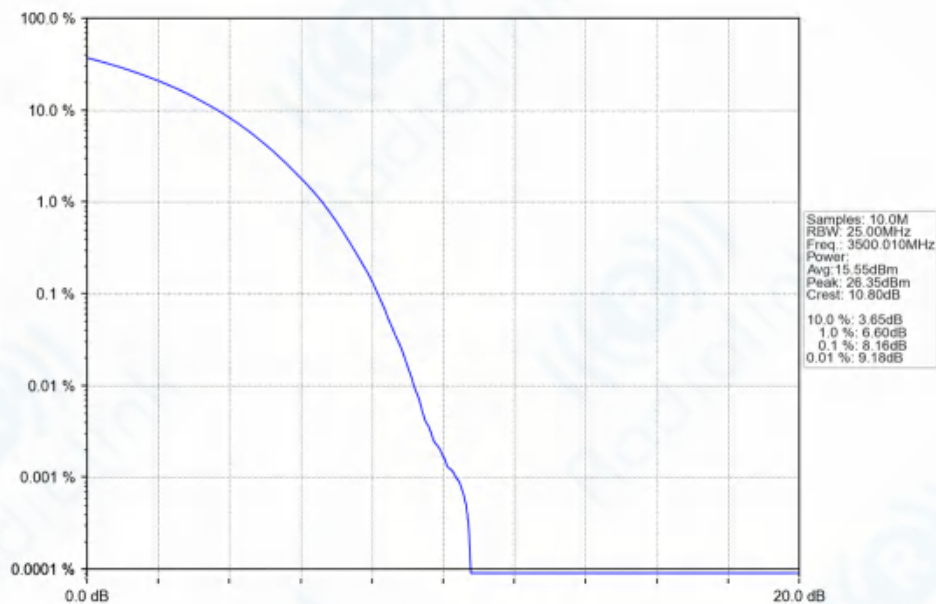
n77d_30kHz_SISO_NTNV_60MHz_CP-OFDM_16_QAM_3500.01MHz_Outer_Full_Ant1
