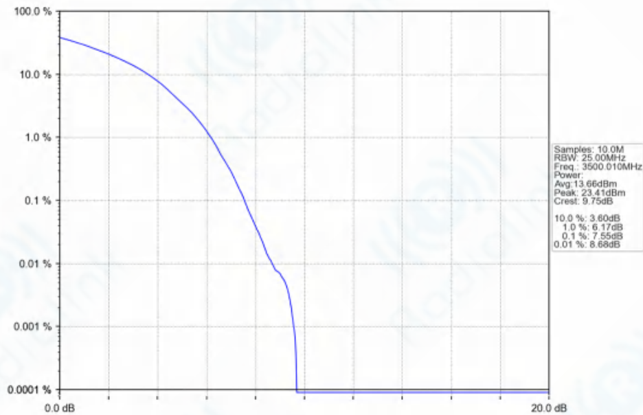
n77d_30kHz_SISO_NTNV_70MHz_DFT-s-OFDM_256_QAM_3500.01MHz_Outer_Full_Ant1
