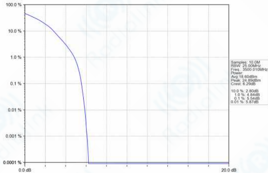
n77d_30kHz_SISO_NTNV_30MHz_DFT-s-OFDM_16_QAM_3500.01MHz_Outer_Full_Ant1
