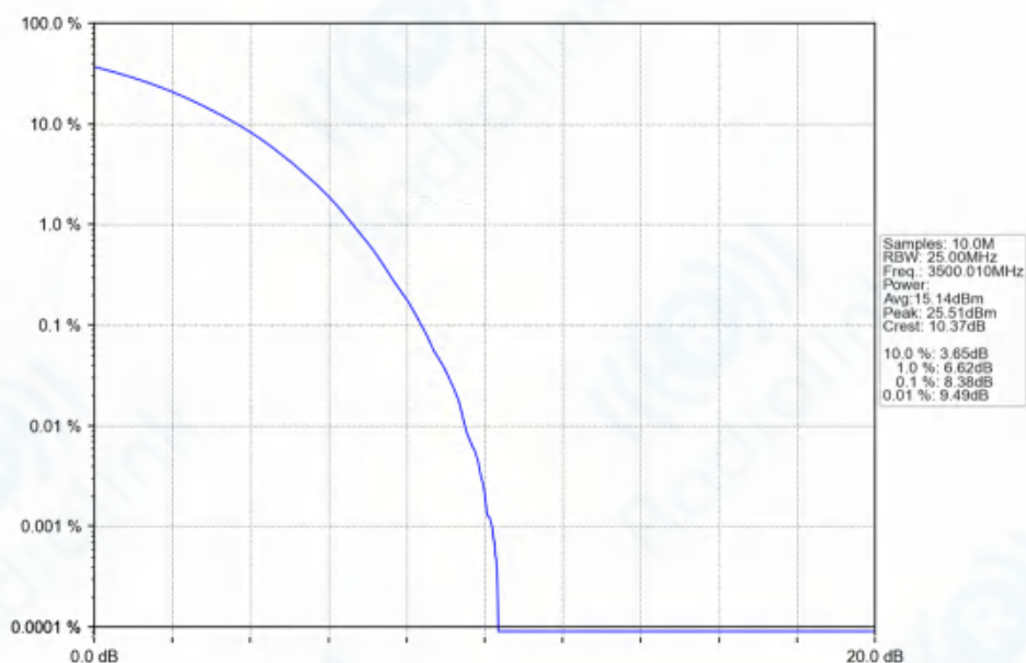
n77d_30kHz_SISO_NTNV_30MHz_CP-OFDM_256_QAM_3500.01MHz_Outer_Full_Ant1
