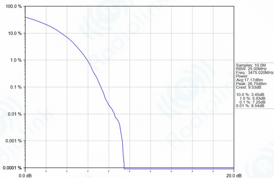
n77d_30kHz_SISO_NTNV_50MHz_DFT-s-OFDM_64_QAM_3475.02MHz_Outer_Full_Ant1
