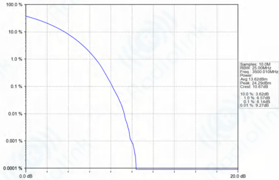
n77d_30kHz_SISO_NTNV_90MHz_CP-OFDM_QPSK_3500.01MHz_Outer_Full_Ant1
