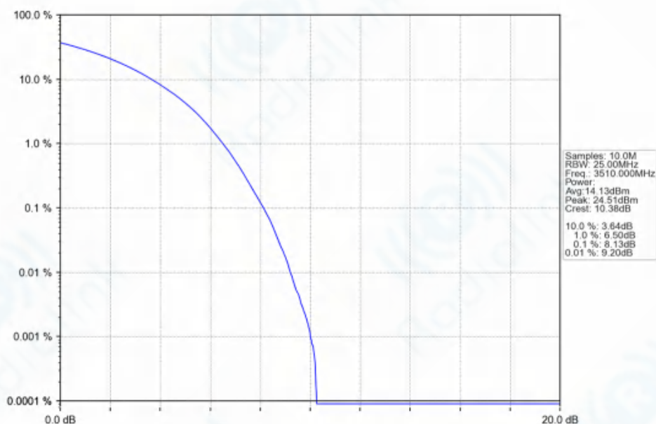
n77d_30kHz_SISO_NTNV_80MHz_CP-OFDM_QPSK_3510MHz_Outer_Full_Ant1
