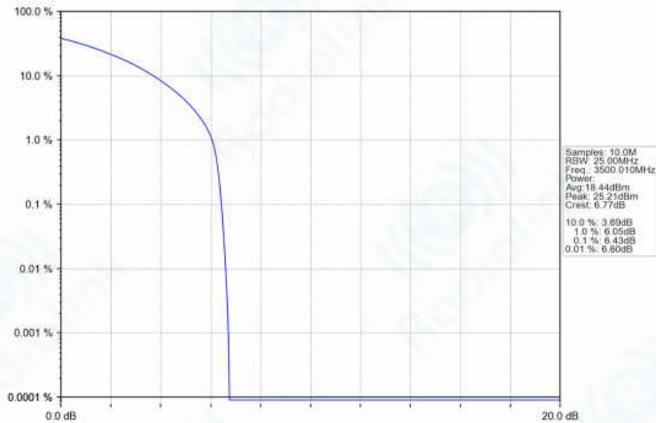
n77d_30kHz_SISO_NTNV_20MHz_CP-OFDM_16_QAM_3500.01MHz_Outer_Full_Ant1
