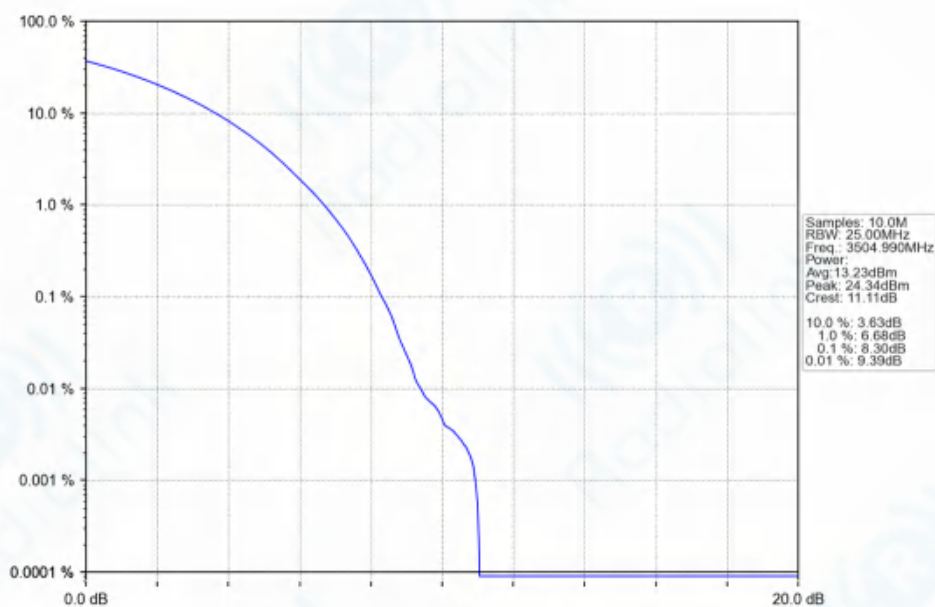
n77d_30kHz_SISO_NTNV_90MHz_CP-OFDM_64_QAM_3504.99MHz_Outer_Full_Ant1
