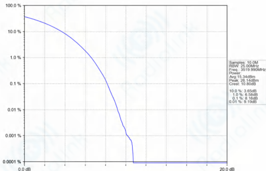
n77d_30kHz_SISO_NTNV_60MHz_CP-OFDM_16_QAM_3519.99MHz_Outer_Full_Ant1
