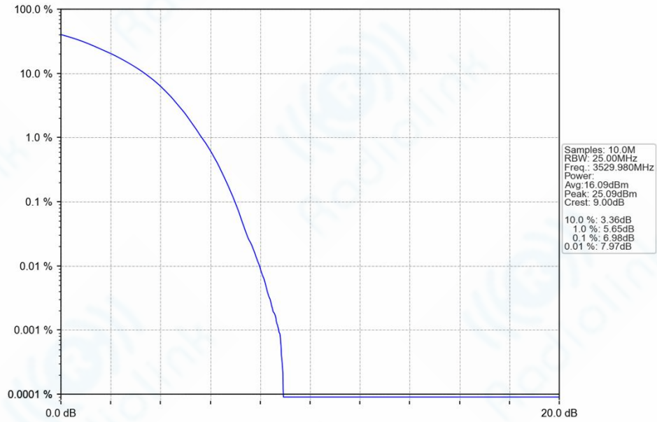
n77d_30kHz_SISO_NTNV_40MHz_DFT-s-OFDM_256_QAM_3529.98MHz_Outer_Full_Ant1
