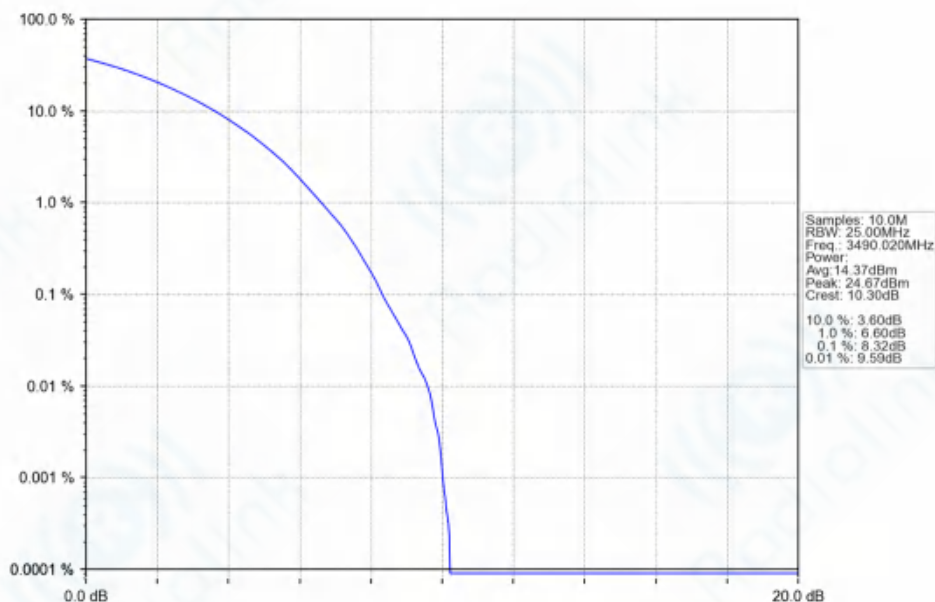
n77d_30kHz_SISO_NTNV_80MHz_CP-OFDM_16_QAM_3490.02MHz_Outer_Full_Ant1
