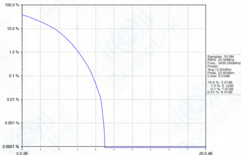
n77d_30kHz_SISO_NTNV_90MHz_DFT-s-OFDM_16_QAM_3495MHz_Outer_Full_Ant1
