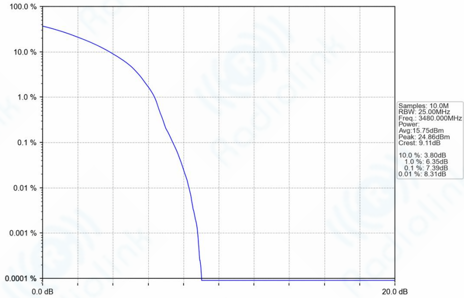
n77d_30kHz_SISO_NTNV_60MHz_DFT-s-OFDM_16_QAM_3480MHz_Outer_Full_Ant1
