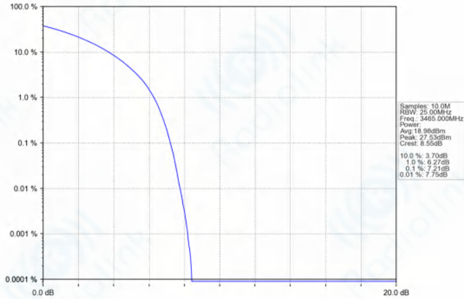
n77d_30kHz_SISO_NTNV_30MHz_CP-OFDM_16_QAM_3465MHz_Outer_Full_Ant1
