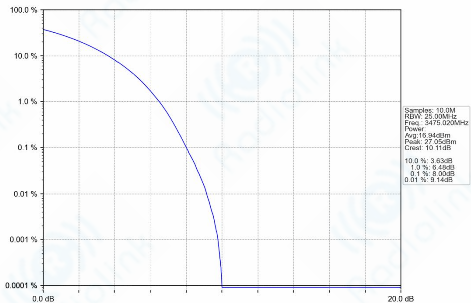
n77d_30kHz_SISO_NTNV_50MHz_CP-OFDM_16_QAM_3475.02MHz_Outer_Full_Ant1
