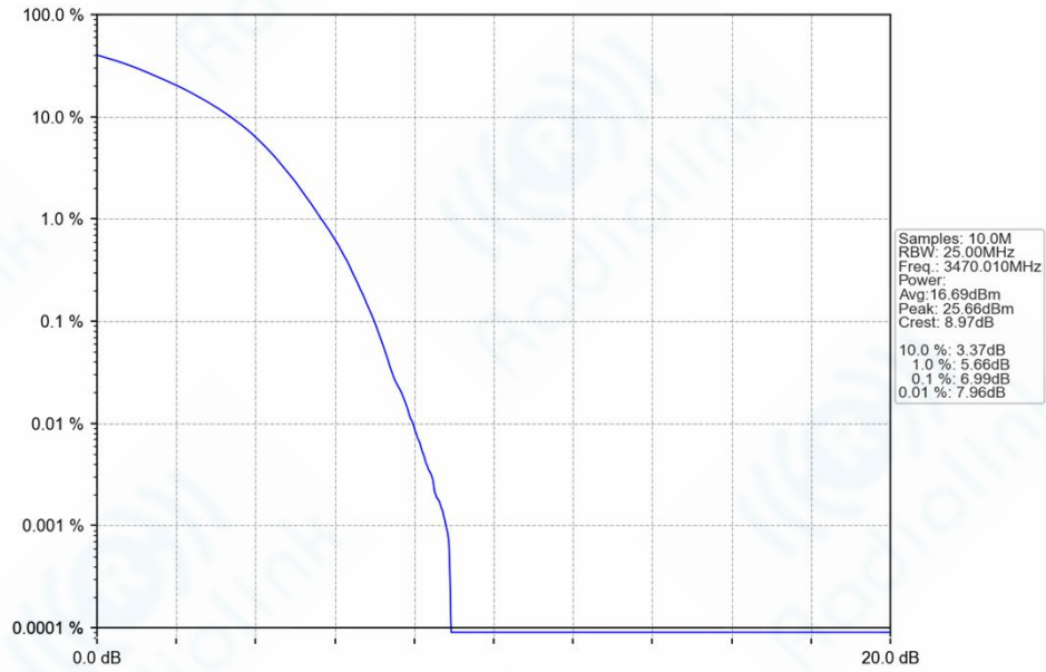
n77d_30kHz_SISO_NTNV_40MHz_DFT-s-OFDM_256_QAM_3470.01MHz_Outer_Full_Ant1
