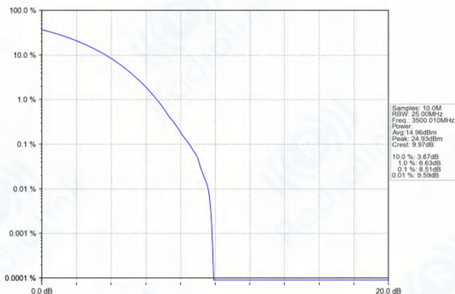
n77d_30kHz_SISO_NTNV_20MHz_CP-OFDM_256_QAM_3500.01MHz_Outer_Full_Ant1
