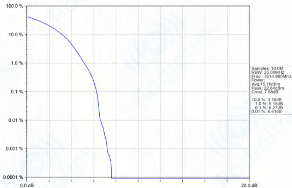
n77d_30kHz_SISO_NTNV_70MHz_DFT-s-OFDM_PI/2_BPSK_3514.98MHz_Outer_Full_Ant1
