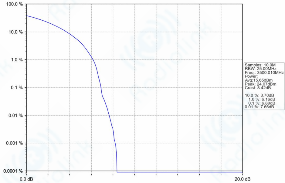
n77d_30kHz_SISO_NTNV_60MHz_DFT-s-OFDM_QPSK_3500.01MHz_Outer_Full_Ant1
