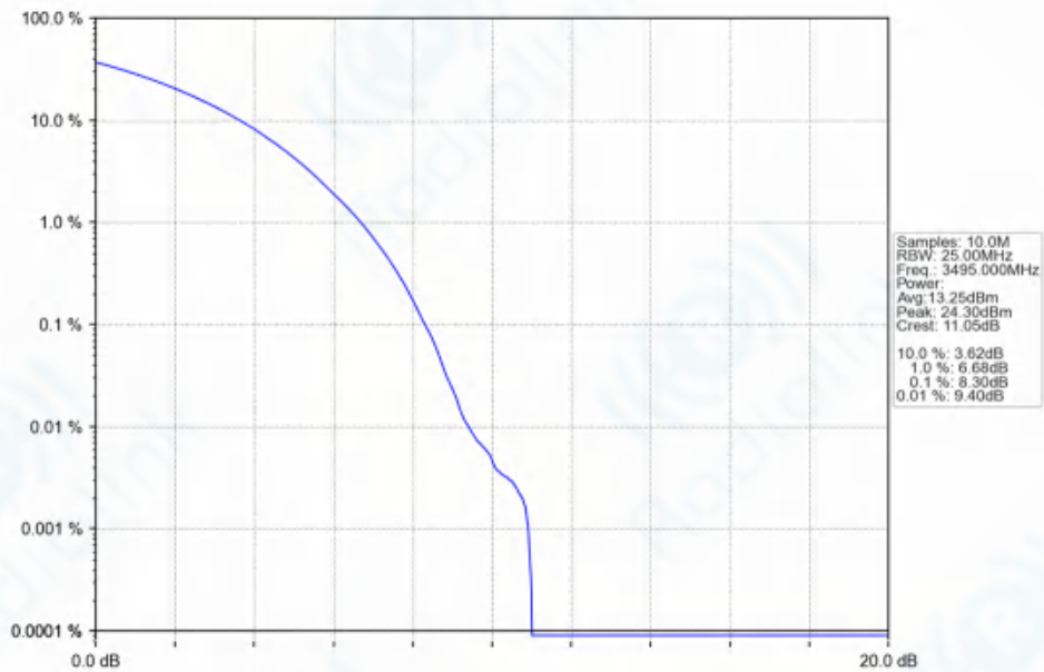
n77d_30kHz_SISO_NTNV_90MHz_CP-OFDM_64_QAM_3495MHz_Outer_Full_Ant1
