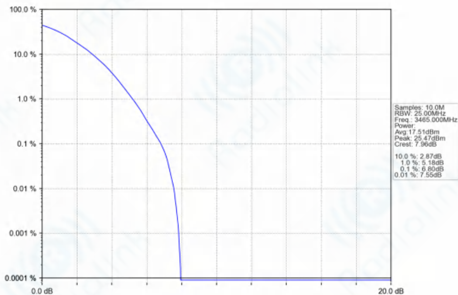
n77d_30kHz_SISO_NTNV_30MHz_DFT-s-OFDM_256_QAM_3465MHz_Outer_Full_Ant1
