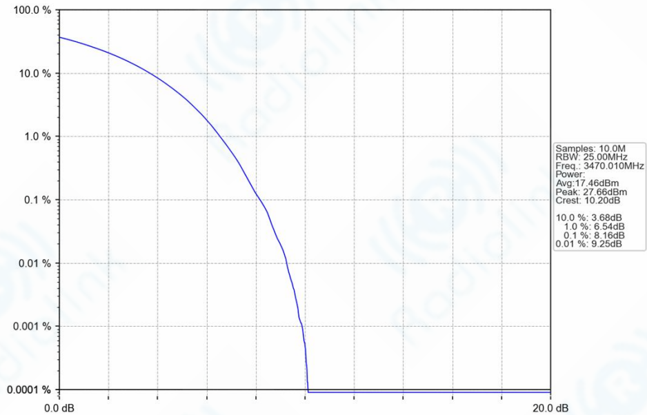
n77d_30kHz_SISO_NTNV_40MHz_CP-OFDM_64_QAM_3470.01MHz_Outer_Full_Ant1
