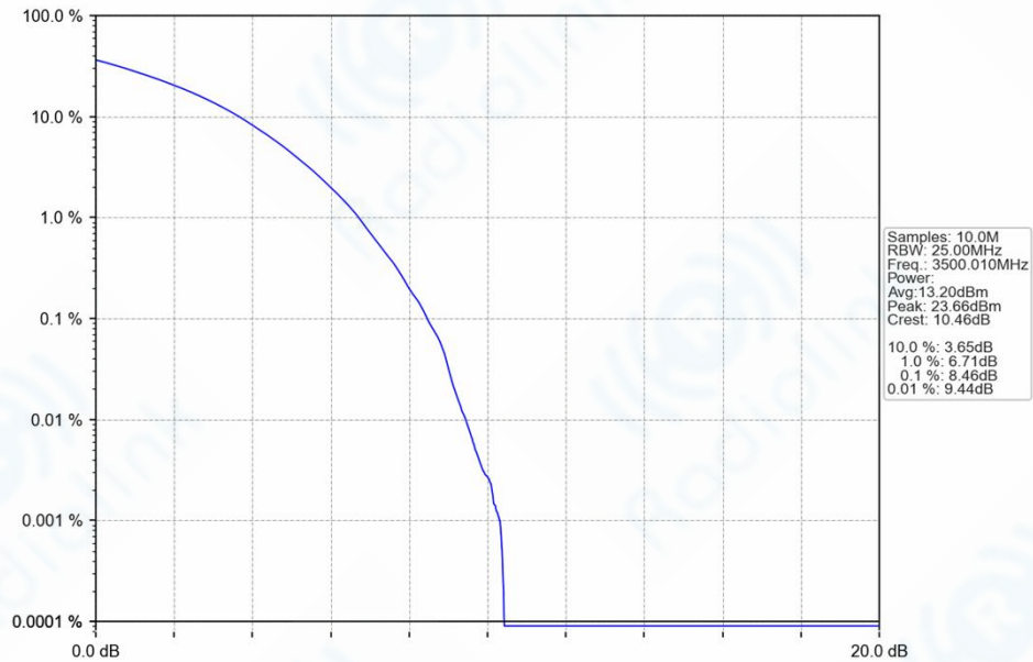
n77d_30kHz_SISO_NTNV_50MHz_CP-OFDM_256_QAM_3500.01MHz_Outer_Full_Ant1
