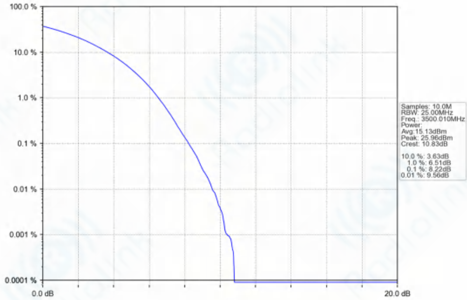
n77d_30kHz_SISO_NTNV_60MHz_CP-OFDM_64_QAM_3500.01MHz_Outer_Full_Ant1
