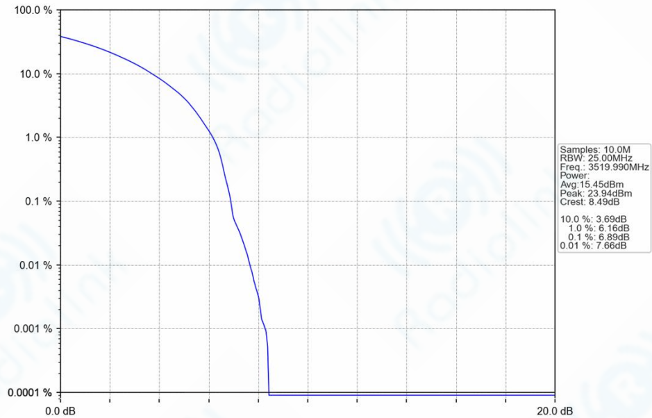
n77d_30kHz_SISO_NTNV_60MHz_DFT-s-OFDM_QPSK_3519.99MHz_Outer_Full_Ant1
