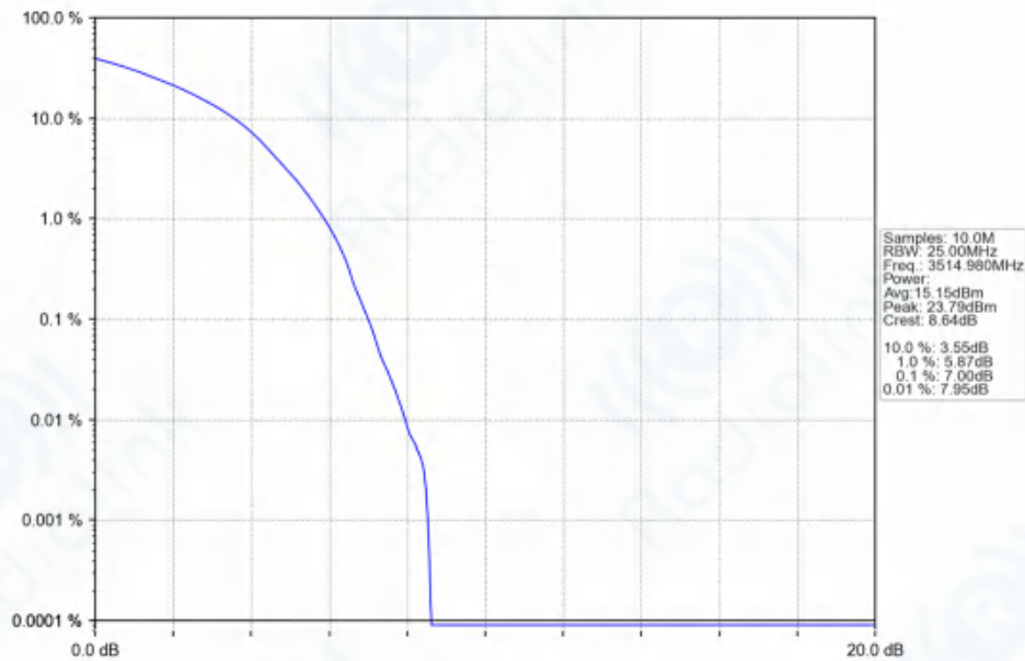
n77d_30kHz_SISO_NTNV_70MHz_DFT-s-OFDM_QPSK_3514.98MHz_Outer_Full_Ant1
