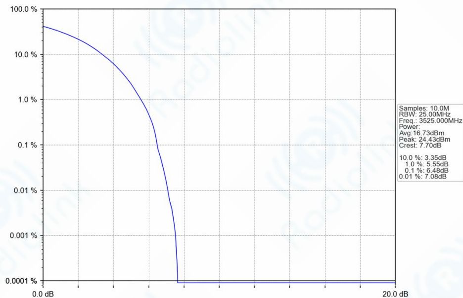
n77d_30kHz_SISO_NTNV_50MHz_DFT-s-OFDM_QPSK_3525MHz_Outer_Full_Ant1
