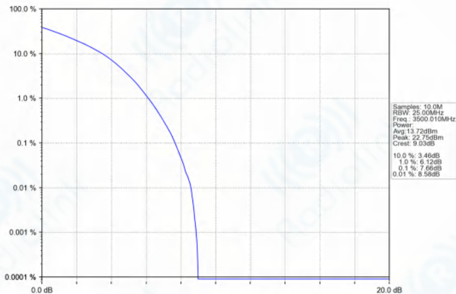
n77d_30kHz_SISO_NTNV_90MHz_DFT-s-OFDM_16_QAM_3500.01MHz_Outer_Full_Ant1
