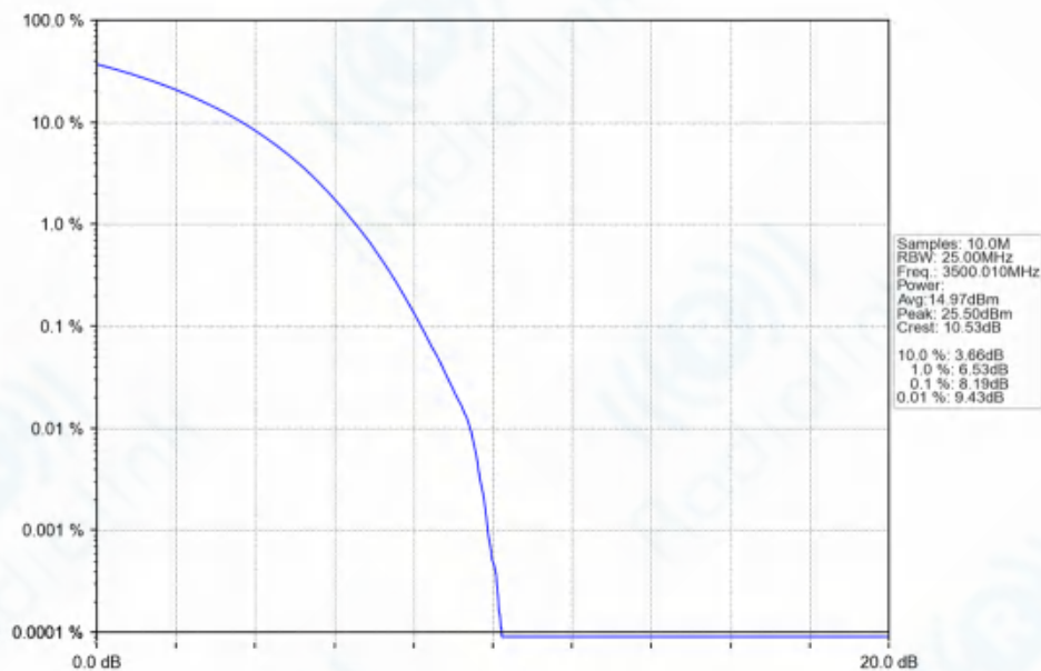
n77d_30kHz_SISO_NTNV_70MHz_CP-OFDM_16_QAM_3500.01MHz_Outer_Full_Ant1
