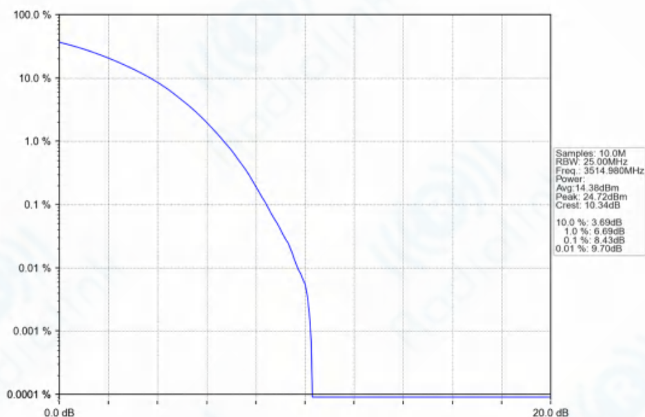
n77d_30kHz_SISO_NTNV_70MHz_CP-OFDM_64_QAM_3514.98MHz_Outer_Full_Ant1
