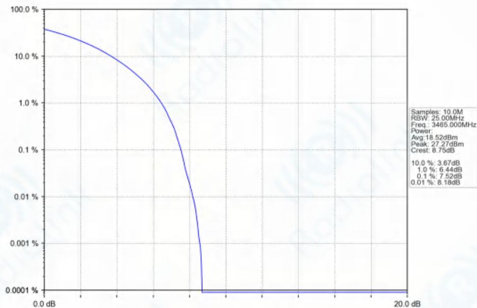
n77d_30kHz_SISO_NTNV_30MHz_CP-OFDM 64 QAM_3465MHz_Outer_Full_Ant1
