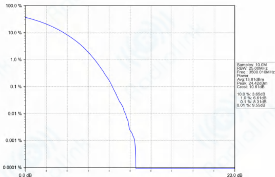
n77d_30kHz_SISO_NTNV_80MHz_CP-OFDM_64_QAM_3500.01MHz_Outer_Full_Ant1
