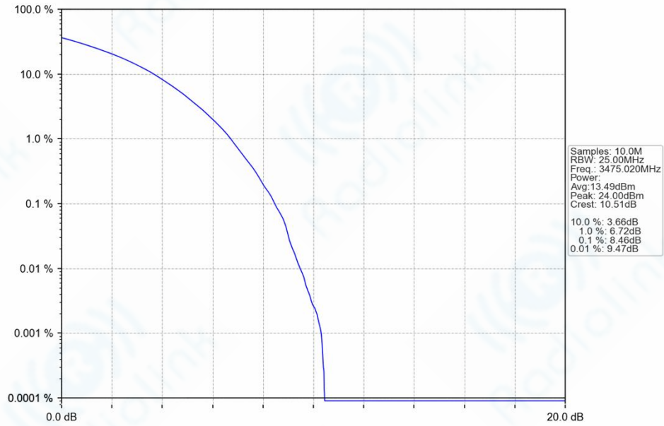
n77d_30kHz_SISO_NTNV_50MHz_CP-OFDM_256_QAM_3475.02MHz_Outer_Full_Ant1
