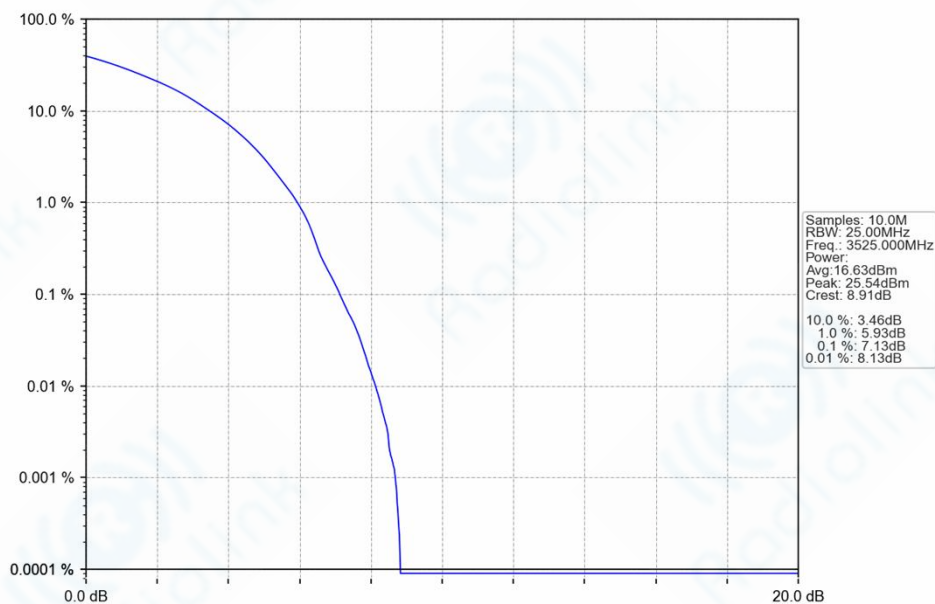
n77d_30kHz_SISO_NTNV_50MHz_DFT-s-OFDM_16_QAM_3525MHz_Outer_Full_Ant1
