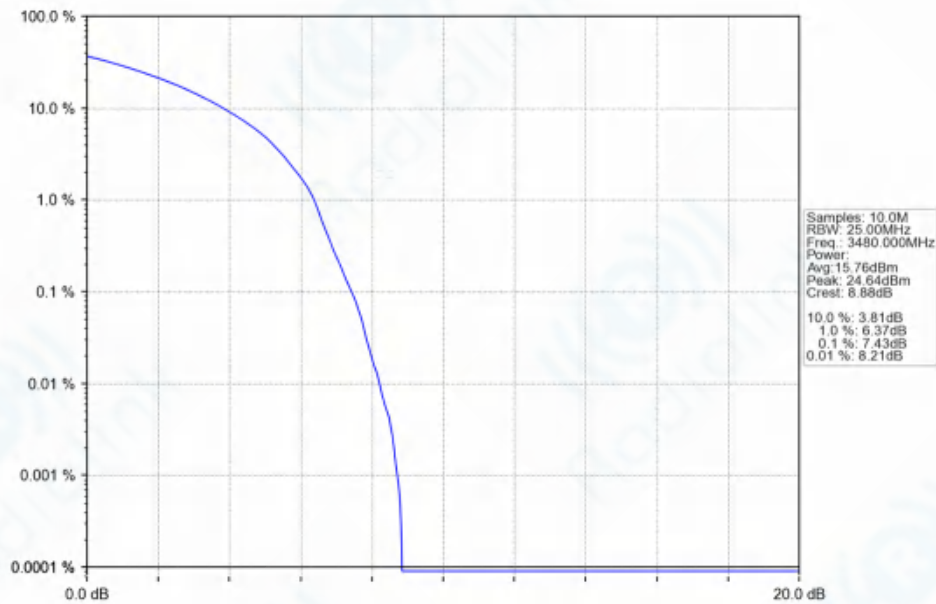
n77d_30kHz_SISO_NTNV_60MHz_DFT-s-OFDM_64_QAM_3480MHz_Outer_Full_Ant1
