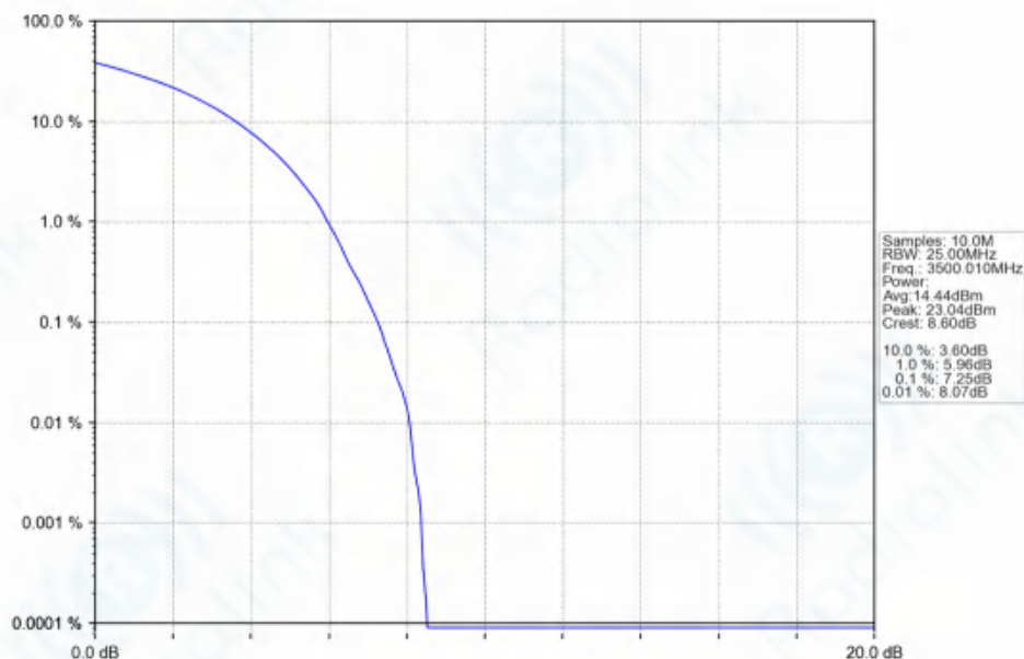
n77d_30kHz_SISO_NTNV_80MHz_DFT-s-OFDM_QPSK_3500.01MHz_Outer_Full_Ant1
