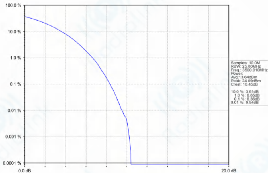
n77d_30kHz_SISO_NTNV_90MHz_CP-OFDM_16_QAM_3500.01MHz_Outer_Full_Ant1
