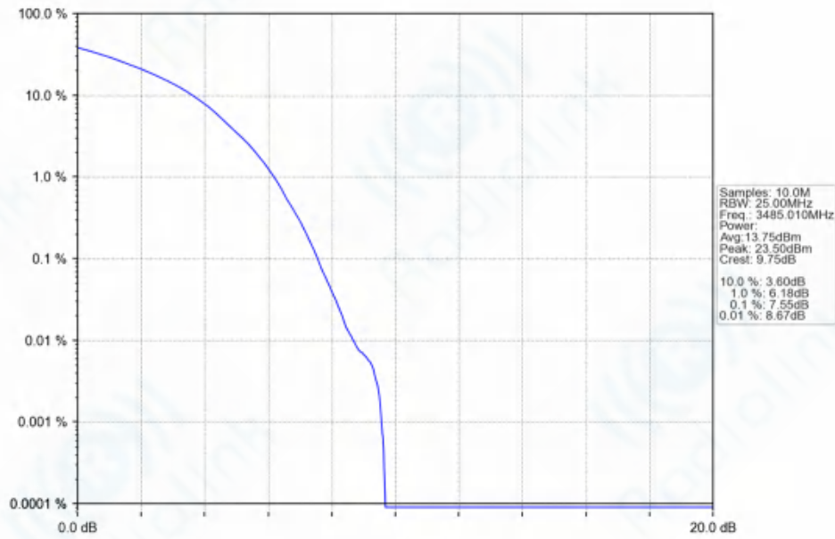
n77d_30kHz_SISO_NTNV_70MHz_DFT-s-OFDM_256_QAM_3485.01MHz_Outer_Full_Ant1
