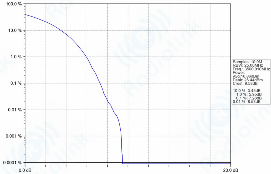
n77d_30kHz_SISO_NTNV_50MHz_DFT-s-OFDM_64_QAM_3500.01MHz_Outer_Full_Ant1
