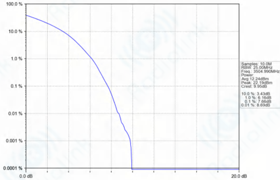
n77d_30kHz_SISO_NTNV_90MHz_DFT-s-OFDM_256_QAM_3504.99MHz_Outer_Full_Ant1
