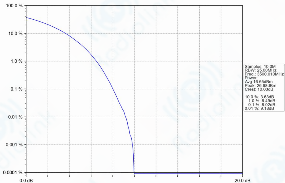
n77d_30kHz_SISO_NTNV_50MHz_CP-OFDM_16_QAM_3500.01MHz_Outer_Full_Ant1
