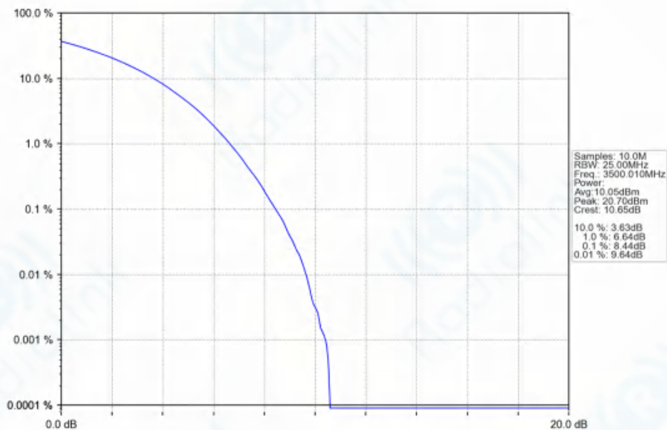
n77d_30kHz_SISO_NTNV_90MHz_CP-OFDM_256_QAM_3500.01MHz_Outer_Full_Ant1
