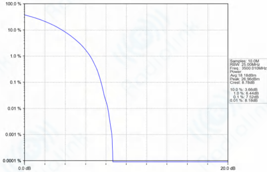
n77d_30kHz_SISO_NTNV_30MHz_CP-OFDM_64_QAM_3500.01MHz_Outer_Full_Ant1
