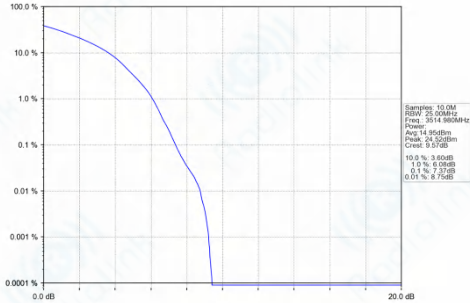
n77d_30kHz_SISO_NTNV_70MHz_DFT-s-OFDM_16_QAM_3514.98MHz_Outer_Full_Ant1
