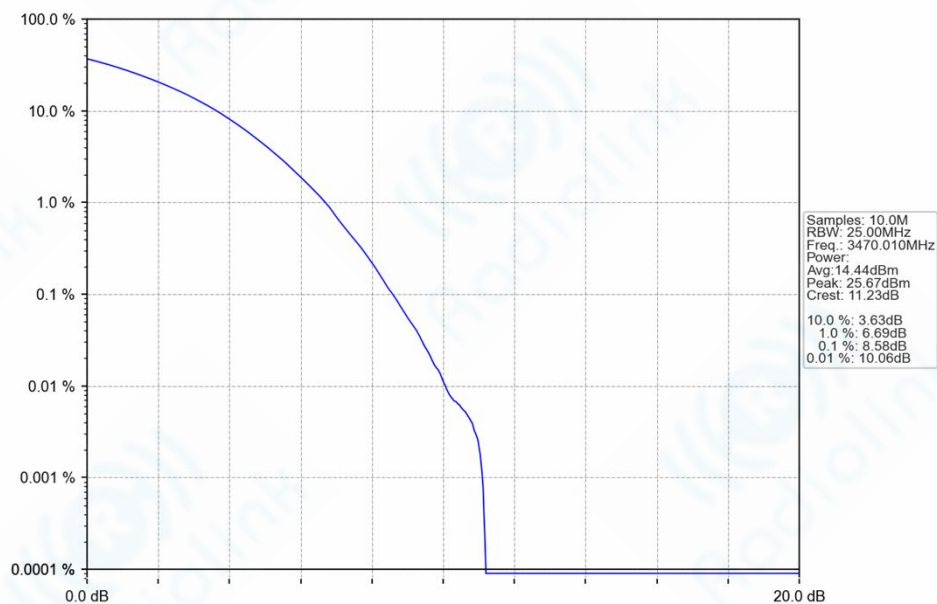
n77d_30kHz_SISO_NTNV_40MHz_CP-OFDM_256_QAM_3470.01MHz_Outer_Full_Ant1
