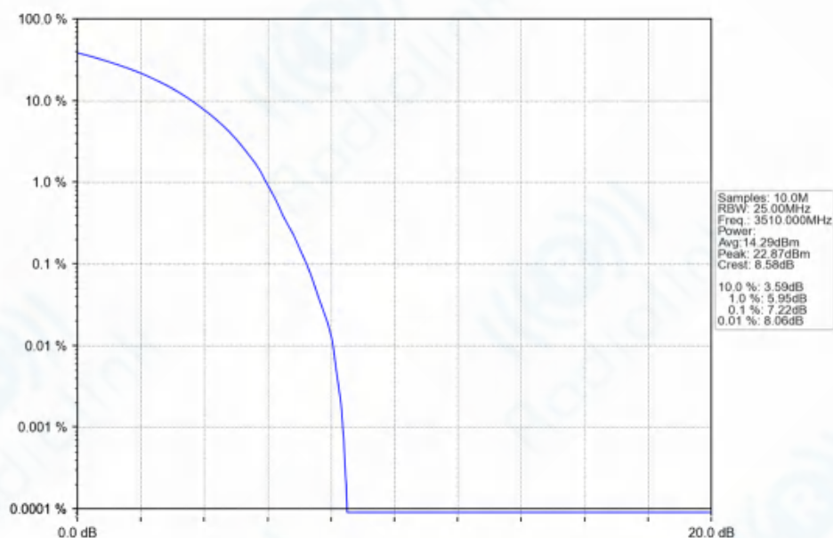
n77d_30kHz_SISO_NTNV_80MHz_DFT-s-OFDM_QPSK_3510MHz_Outer_Full_Ant1
