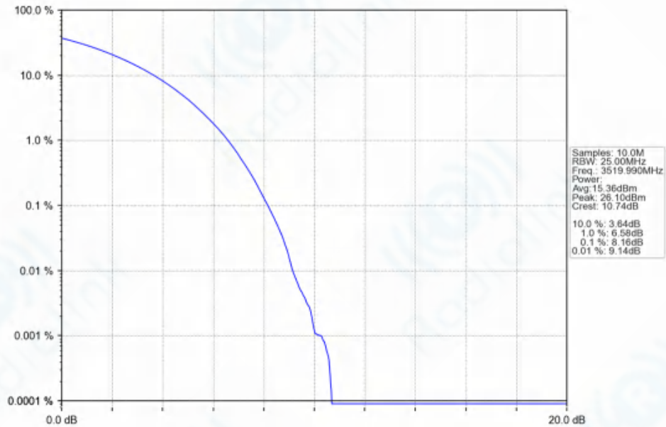
n77d_30kHz_SISO_NTNV_60MHz_CP-OFDM_QPSK_3519.99MHz_Outer_Full_Ant1
