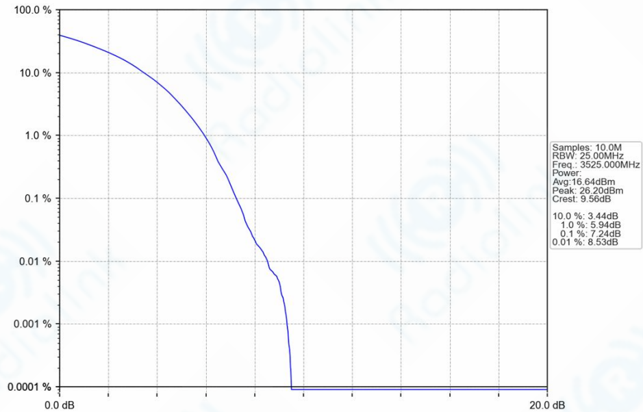
n77d_30kHz_SISO_NTNV_50MHz_DFT-s-OFDM_64_QAM_3525MHz_Outer_Full_Ant1
