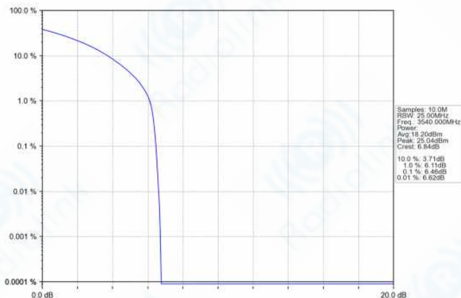
n77d_30kHz_SISO_NTNV_20MHz_CP-OFDM_QPSK_3540MHz_Outer_Full_Ant1
