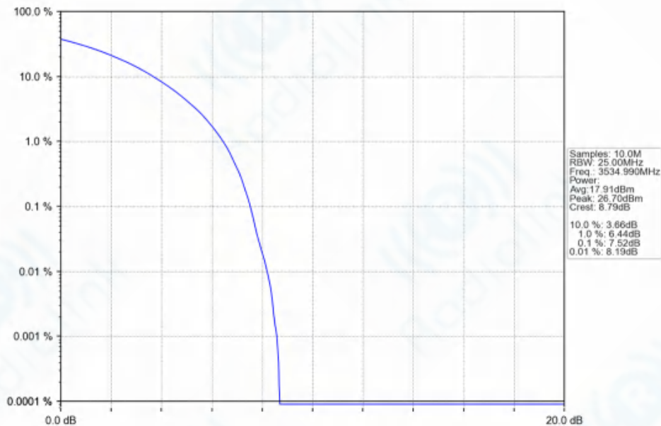
n77d_30kHz_SISO_NTNV_30MHz_CP-OFDM_64_QAM_3534.99MHz_Outer_Full_Ant1
