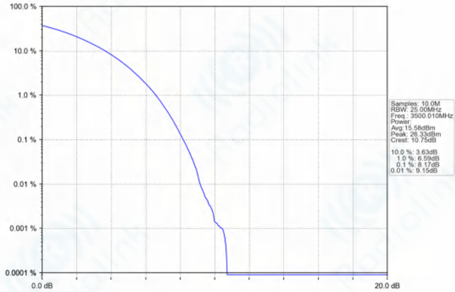
n77d_30kHz_SISO_NTNV_60MHz_CP-OFDM_QPSK_3500.01MHz_Outer_Full_Ant1
