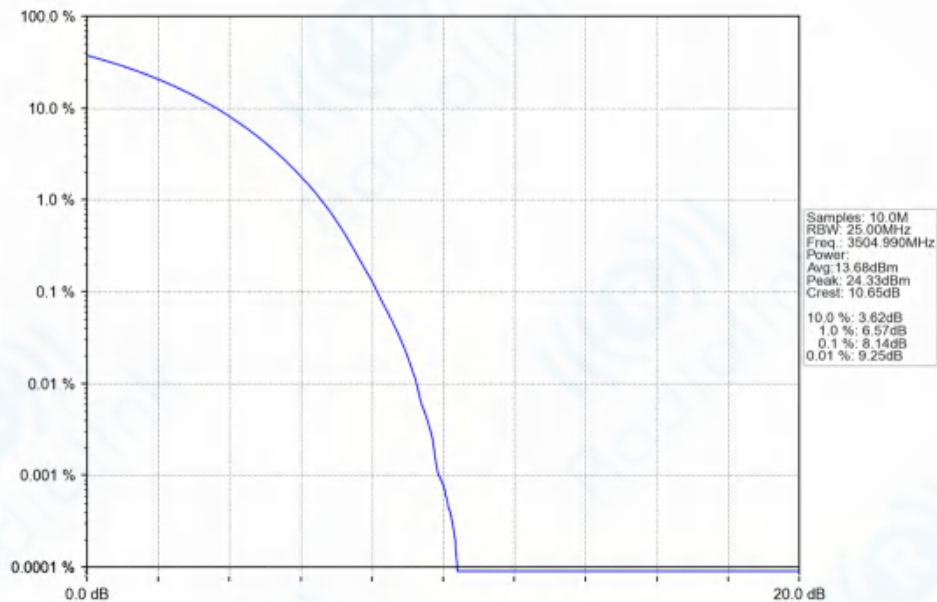
n77d_30kHz_SISO_NTNV_90MHz_CP-OFDM_QPSK_3504.99MHz_Outer_Full_Ant1
