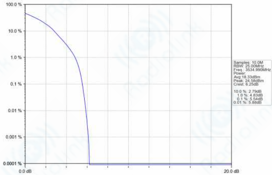
n77d_30kHz_SISO_NTNV_30MHz_DFT-s-OFDM_16_QAM_3534.99MHz_Outer_Full_Ant1
