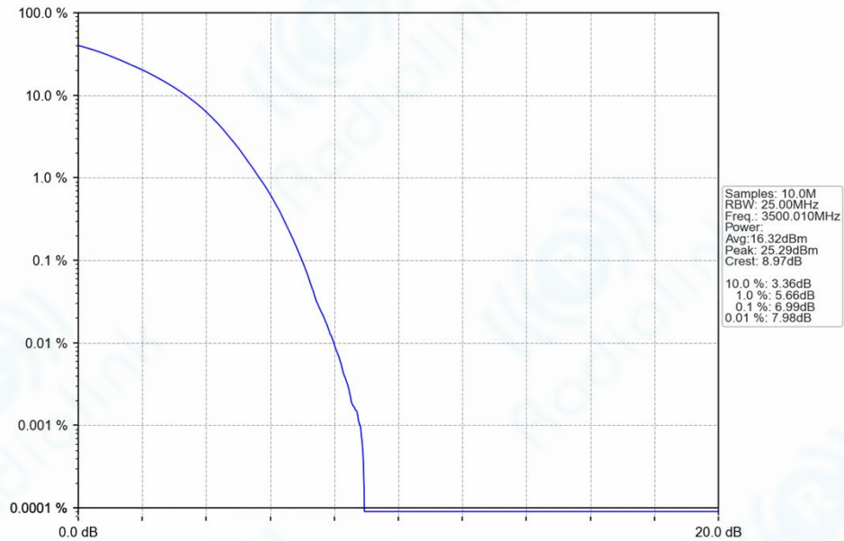
n77d_30kHz_SISO_NTNV_40MHz_DFT-s-OFDM_256_QAM_3500.01MHz_Outer_Full_Ant1
