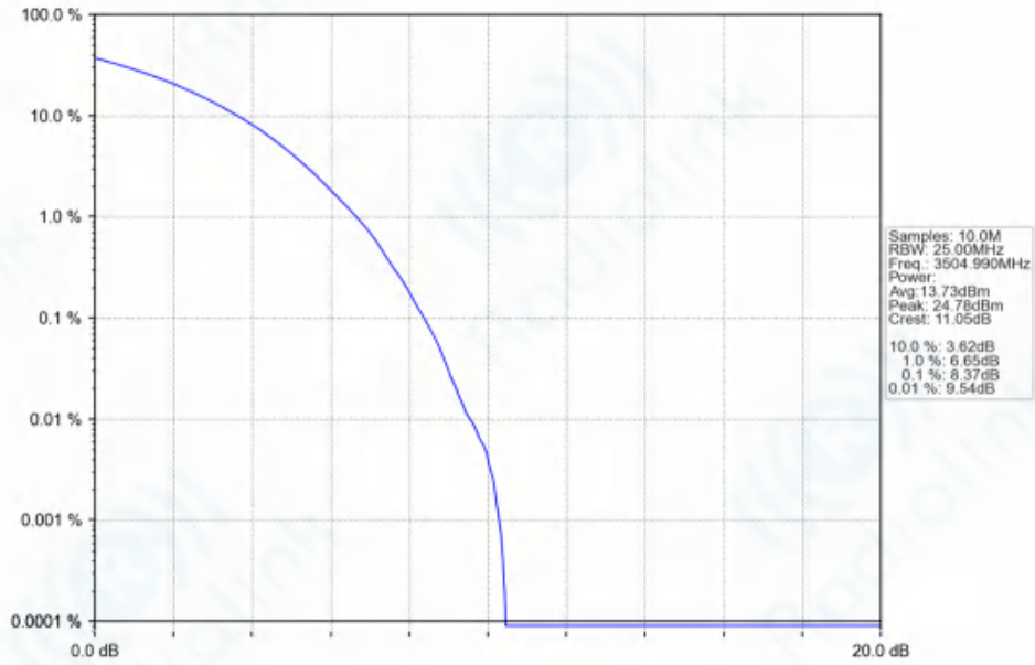
n77d_30kHz_SISO_NTNV_90MHz_CP-OFDM_16_QAM_3504.99MHz_Outer_Full_Ant1
