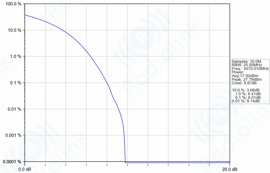
n77d_30kHz_SISO_NTNV_40MHz_CP-OFDM_16_QAM_3470.01MHz_Outer_Full_Ant1
