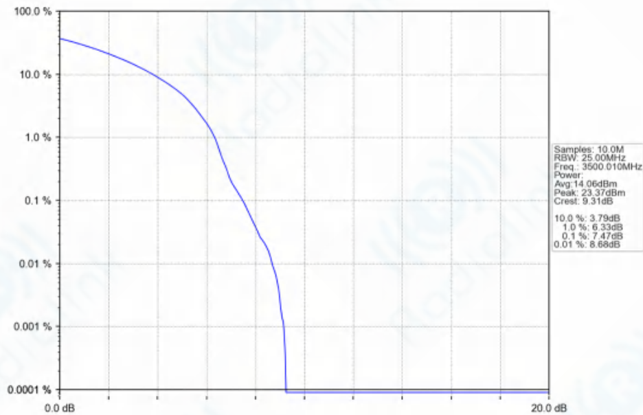
n77d_30kHz_SISO_NTNV_60MHz_DFT-s-OFDM_256_QAM_3500.01MHz_Outer_Full_Ant1
