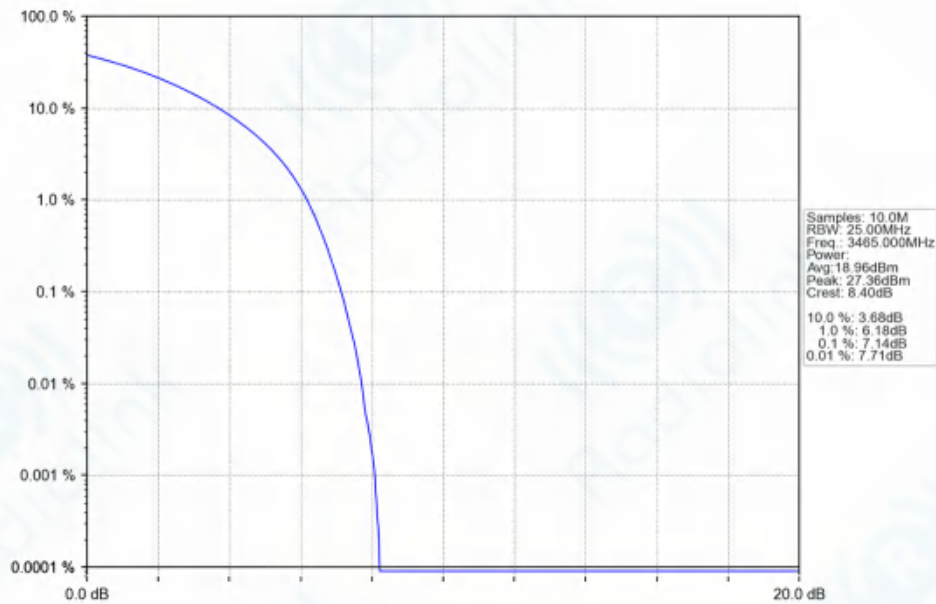
n77d_30kHz_SISO_NTNV_30MHz_CP-OFDM_QPSK_3465MHz_Outer_Full_Ant1
