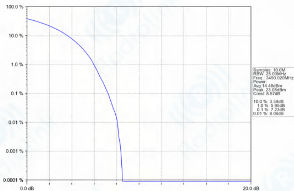
n77d_30kHz_SISO_NTNV_80MHz_DFT-s-OFDM QPSK_3490.02MHz_Outer_Full_Ant1
