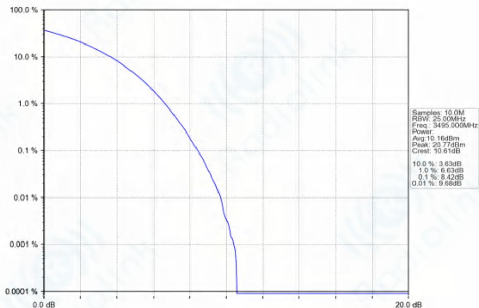
n77d_30kHz_SISO_NTNV_90MHz_CP-OFDM_256_QAM_3495MHz_Outer_Full_Ant1
