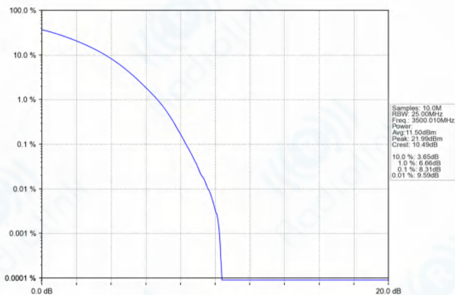
n77d_30kHz_SISO_NTNV_70MHz_CP-OFDM_256_QAM_3500.01MHz_Outer_Full_Ant1
