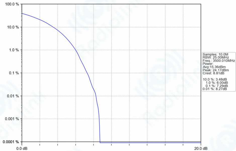
n77d_30kHz_SISO_NTNV_50MHz_DFT-s-OFDM_256_QAM_3500.01MHz_Outer_Full_Ant1
