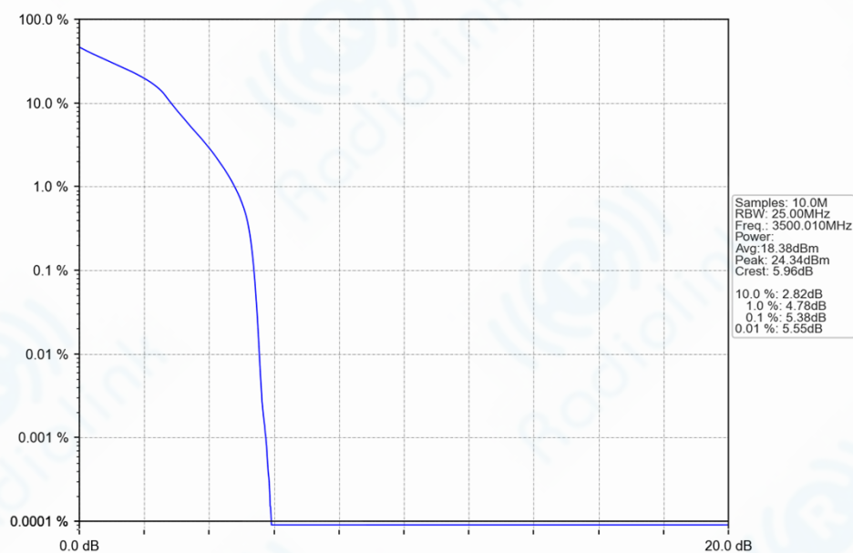
n77d_30kHz_SISO_NTNV_20MHz_DFT-s-OFDM_16_QAM_3500.01MHz_Outer_Full_Ant1
