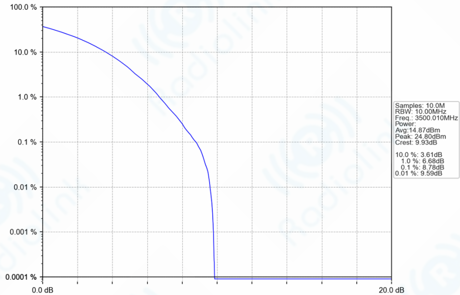
n77d_30kHz_SISO_NTNV_10MHz_CP-OFDM_256_QAM_3500.01MHz_Outer_Full_Ant1
