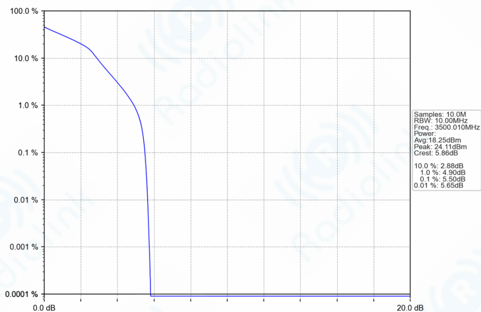
n77d_30kHz_SISO_NTNV_10MHz_DFT-s-OFDM_16_QAM_3500.01MHz_Outer_Full_Ant1
