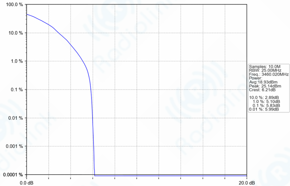
n77d_30kHz_SISO_NTNV_20MHz_DFT-s-OFDM_64_QAM_3460.02MHz_Outer_Full_Ant1
