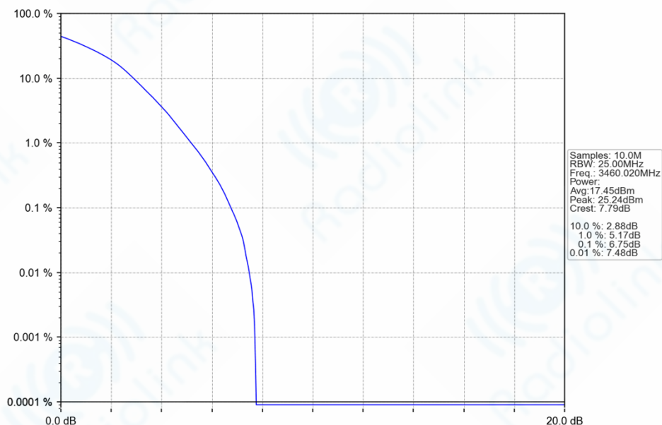
n77d_30kHz_SISO_NTNV_20MHz_DFT-s-OFDM_256_QAM_3460.02MHz_Outer_Full_Ant1
