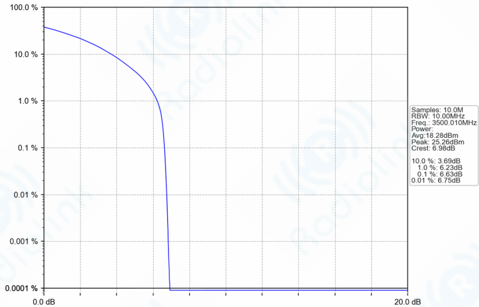
n77d_30kHz_SISO_NTNV_10MHz_CP-OFDM_16_QAM_3500.01MHz_Outer_Full_Ant1
