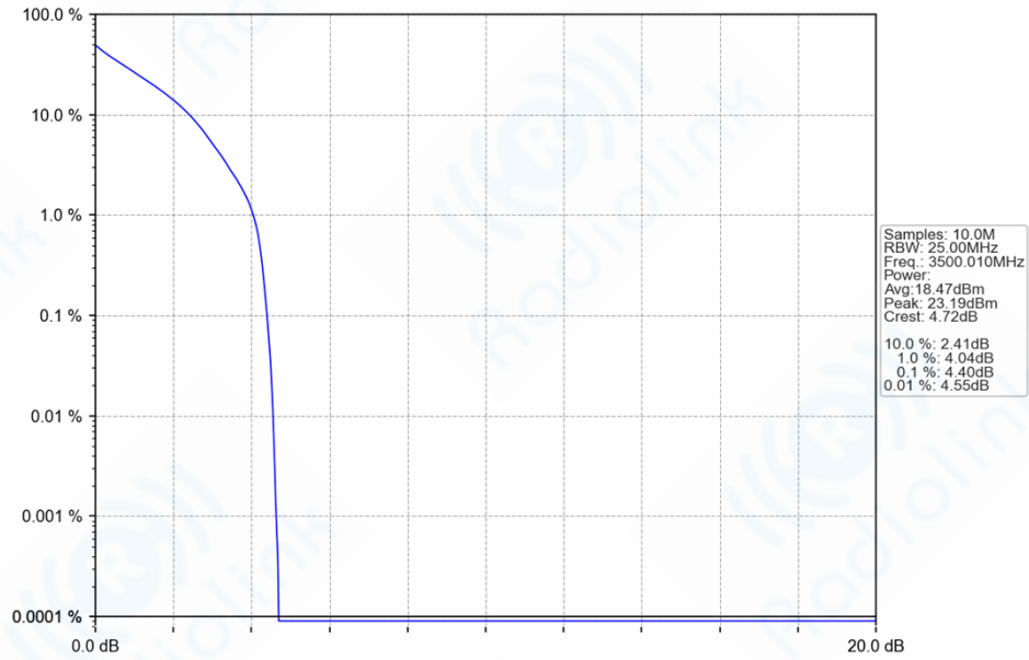
n77d_30kHz_SISO_NTNV_20MHz_DFT-s-OFDM_QPSK_3500.01MHz_Outer_Full_Ant1
