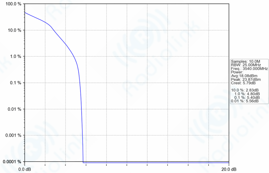
n77d_30kHz_SISO_NTNV_20MHz_DFT-s-OFDM_16_QAM_3540MHz_Outer_Full_Ant1
