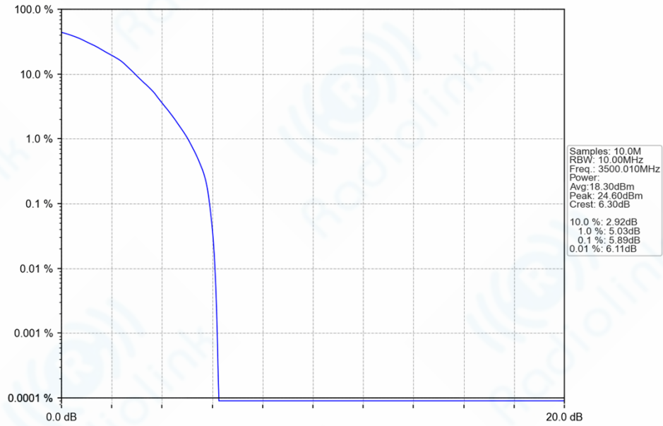
n77d_30kHz_SISO_NTNV_10MHz_DFT-s-OFDM_64_QAM_3500.01MHz_Outer_Full_Ant1
