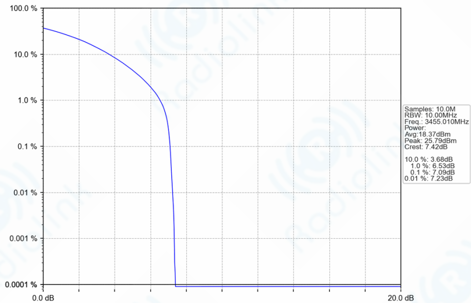
n77d_30kHz_SISO_NTNV_10MHz_CP-OFDM_64_QAM_3455.01MHz_Outer_Full_Ant1
