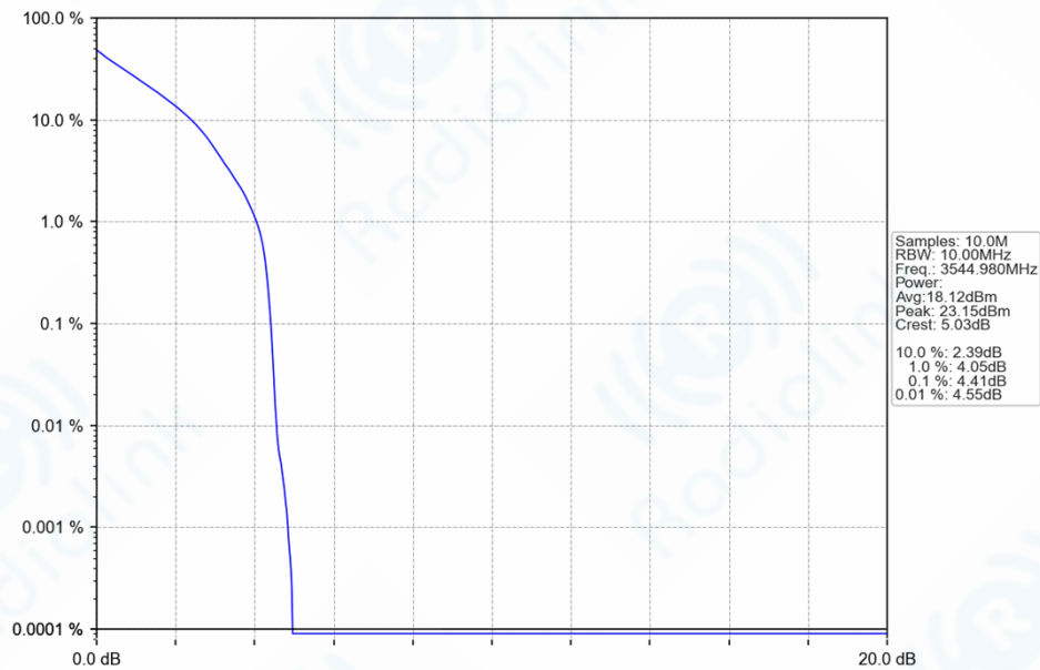
n77d_30kHz_SISO_NTNV_10MHz_DFT-s-OFDM_QPSK_3544.98MHz_Outer_Full_Ant1
