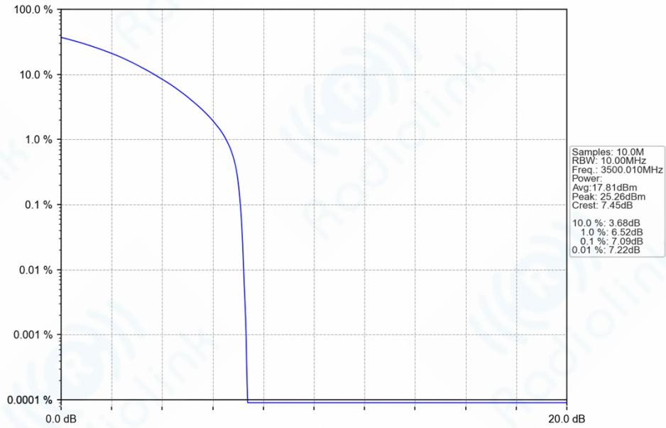
n77d_30kHz_SISO_NTNV_10MHz_CP-OFDM_64_QAM_3500.01MHz_Outer_Full_Ant1
