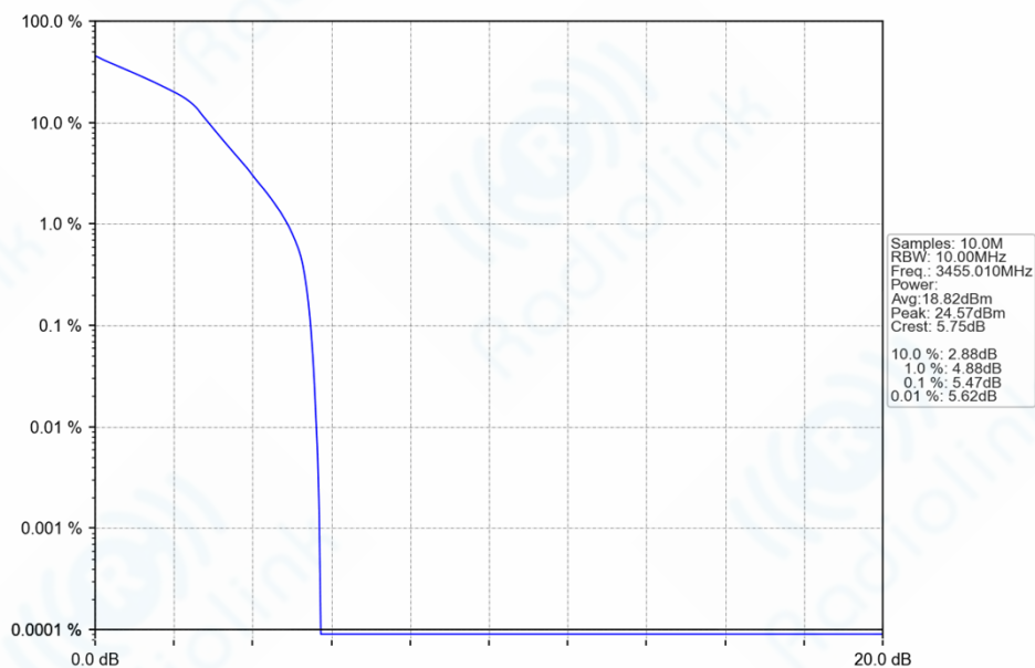
n77d_30kHz_SISO_NTNV_10MHz_DFT-s-OFDM_16_QAM_3455.01MHz_Outer_Full_Ant1
