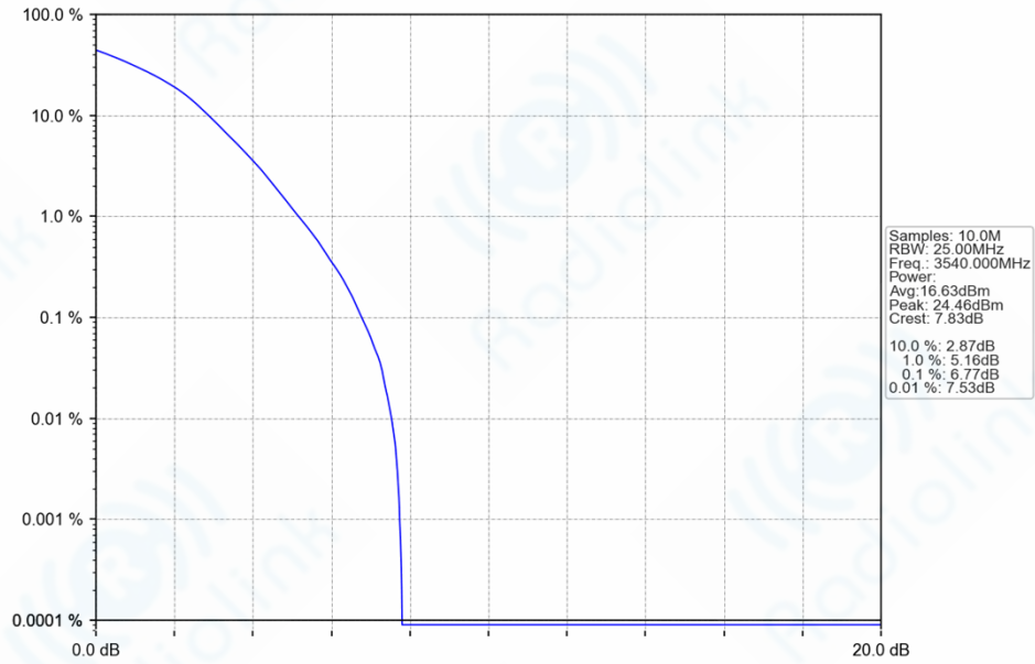
n77d_30kHz_SISO_NTNV_20MHz_DFT-s-OFDM_256_QAM_3540MHz_Outer_Full_Ant1
