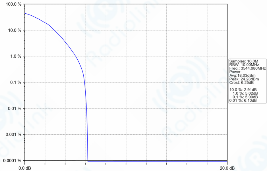
n77d_30kHz_SISO_NTNV_10MHz_DFT-s-OFDM_64_QAM_3544.98MHz_Outer_Full_Ant1
