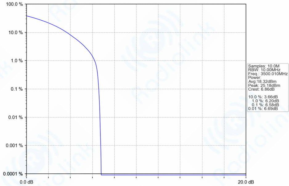
n77d_30kHz_SISO_NTNV_10MHz_CP-OFDM_QPSK_3500.01MHz_Outer_Full_Ant1
