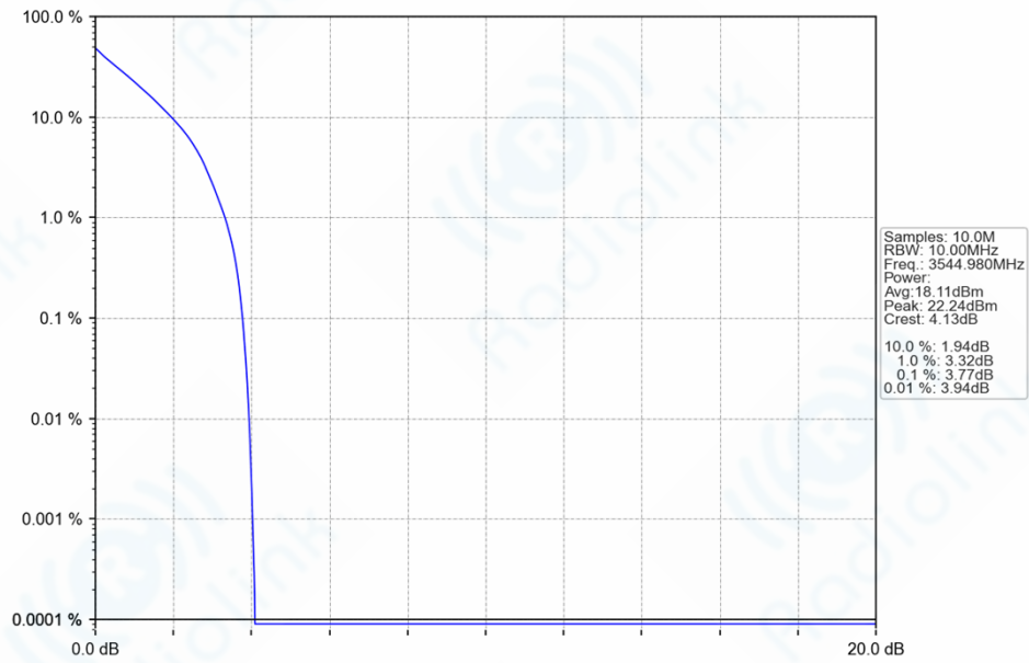
n77d_30kHz_SISO_NTNV_10MHz_DFT-s-OFDM_PI/2_BPSK_3544.98MHz_Outer_Full_Ant1
