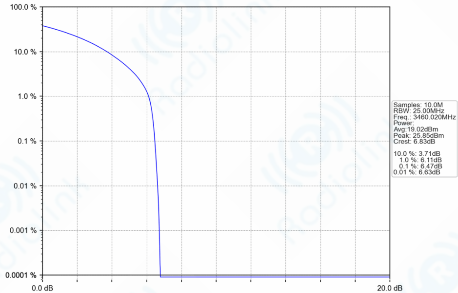
n77d_30kHz_SISO_NTNV_20MHz_CP-OFDM_QPSK_3460.02MHz_Outer_Full_Ant1
