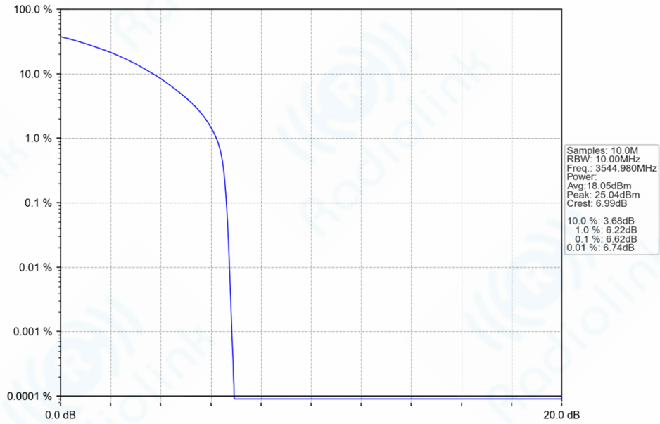
n77d_30kHz_SISO_NTNV_10MHz_CP-OFDM_16_QAM_3544.98MHz_Outer_Full_Ant1
