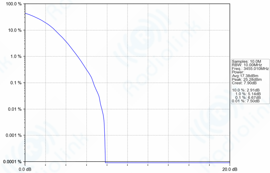
n77d_30kHz_SISO_NTNV_10MHz_DFT-s-OFDM_256_QAM_3455.01MHz_Outer_Full_Ant1
