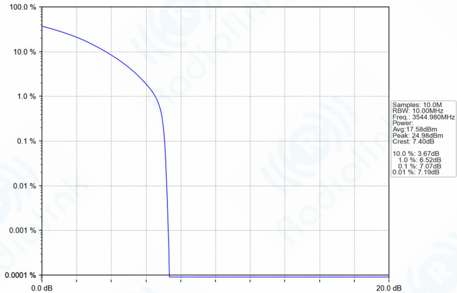
n77d_30kHz_SISO_NTNV_10MHz_CP-OFDM_64_QAM_3544.98MHz_Outer_Full_Ant1
