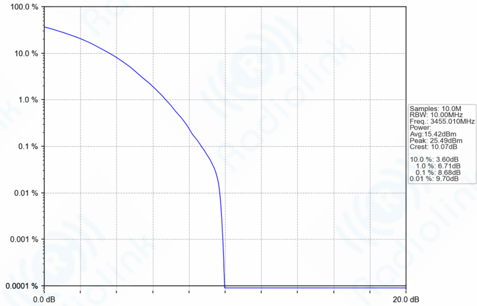
n77d_30kHz_SISO_NTNV_10MHz_CP-OFDM_256_QAM_3455.01MHz_Outer_Full_Ant1
