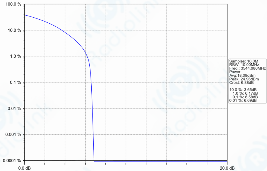
n77d_30kHz_SISO_NTNV_10MHz_CP-OFDM_QPSK_3544.98MHz_Outer_Full_Ant1
