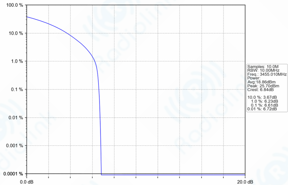
n77d_30kHz_SISO_NTNV_10MHz_CP-OFDM_QPSK_3455.01MHz_Outer_Full_Ant1
