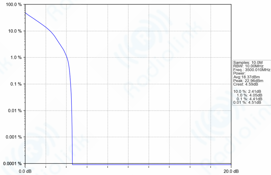
n77d_30kHz_SISO_NTNV_10MHz_DFT-s-OFDM_QPSK_3500.01MHz_Outer_Full_Ant1
