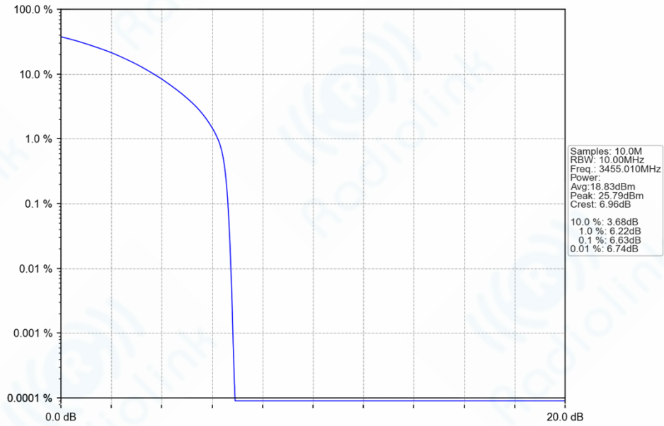
n77d_30kHz_SISO_NTNV_10MHz_CP-OFDM_16_QAM_3455.01MHz_Outer_Full_Ant1
