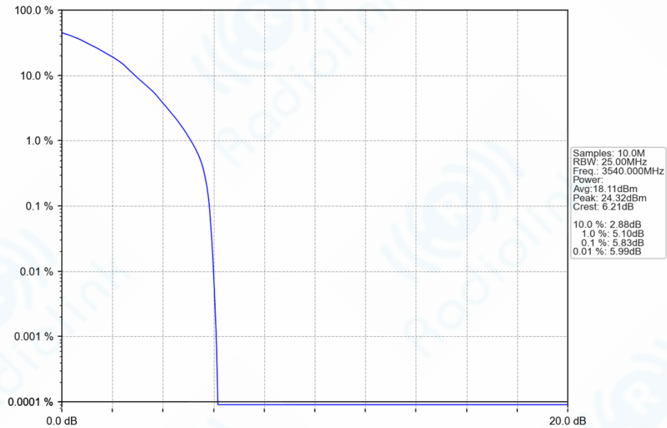
n77d_30kHz_SISO_NTNV_20MHz_DFT-s-OFDM_64_QAM_3540MHz_Outer_Full_Ant1
