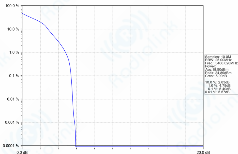
n77d_30kHz_SISO_NTNV_20MHz_DFT-s-OFDM_16_QAM_3460.02MHz_Outer_Full_Ant1
