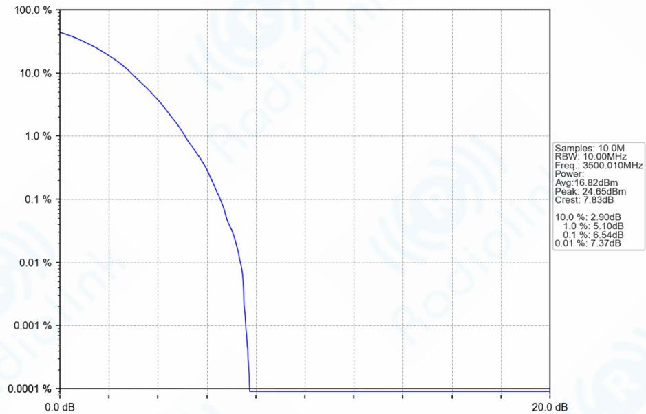
n77d_30kHz_SISO_NTNV_10MHz_DFT-s-OFDM_256_QAM_3500.01MHz_Outer_Full_Ant1
