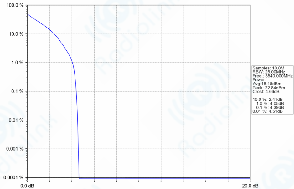
n77d_30kHz_SISO_NTNV_20MHz_DFT-s-OFDM_QPSK_3540MHz_Outer_Full_Ant1
