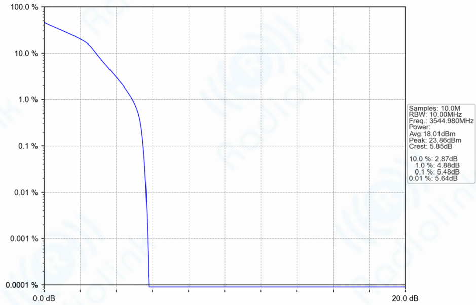
n77d_30kHz_SISO_NTNV_10MHz_DFT-s-OFDM_16_QAM_3544.98MHz_Outer_Full_Ant1
