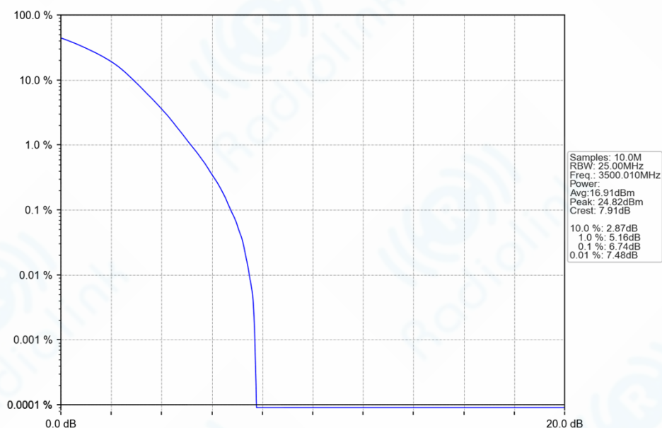
n77d_30kHz_SISO_NTNV_20MHz_DFT-s-OFDM_256_QAM_3500.01MHz_Outer_Full_Ant1
