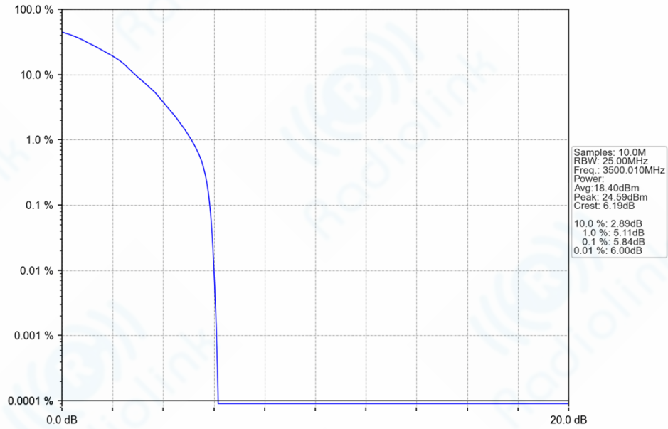
n77d_30kHz_SISO_NTNV_20MHz_DFT-s-OFDM_64_QAM_3500.01MHz_Outer_Full_Ant1
