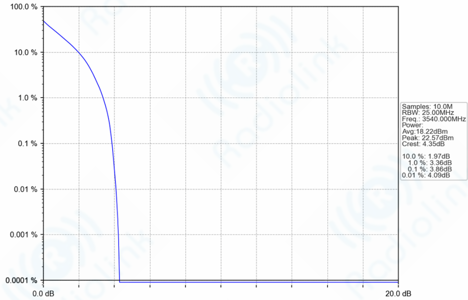
n77d_30kHz_SISO_NTNV_20MHz_DFT-s-OFDM_PI/2_BPSK_3540MHz_Outer_Full_Ant1
