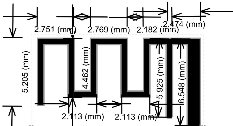
Figure 3: Antenna Dimensions
