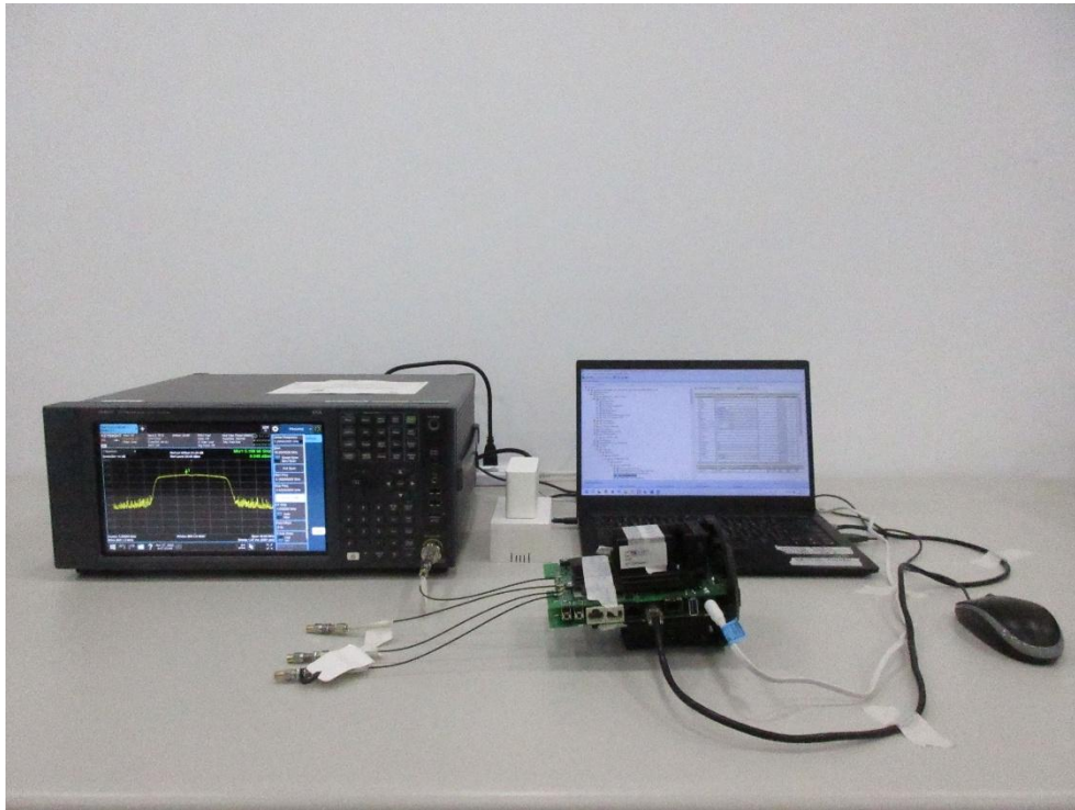
Description: Conducted Measurement Test Setup - BLE
